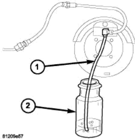
Fig. 71: Bleed Hose Set Up Courtesy of CHRYSLER LLC
