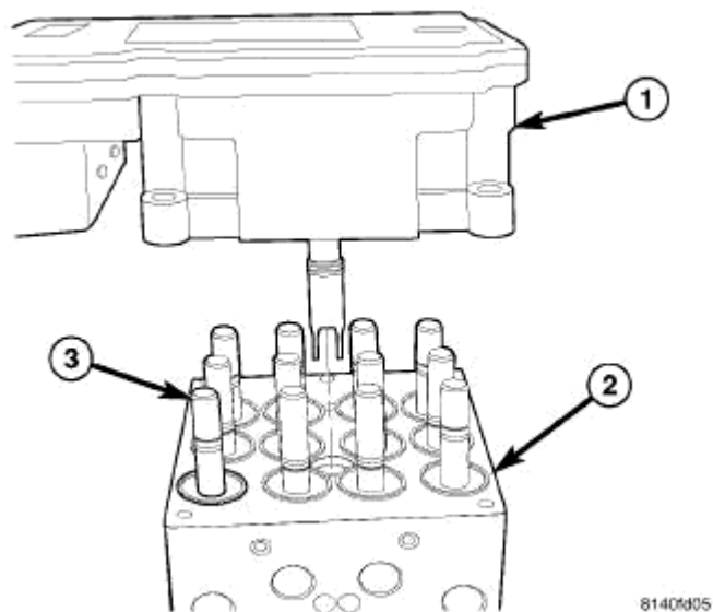
Fig. 54: Identifying ABM, HCU, & Solenoid Valve Stem Courtesy of CHRYSLER LLC
