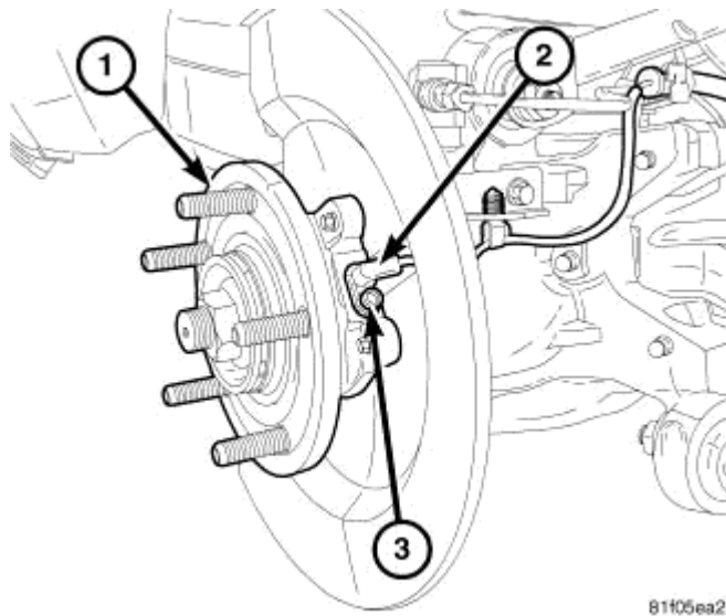
Fig. 21: Hub And Bearing Courtesy of CHRYSLER LLC
