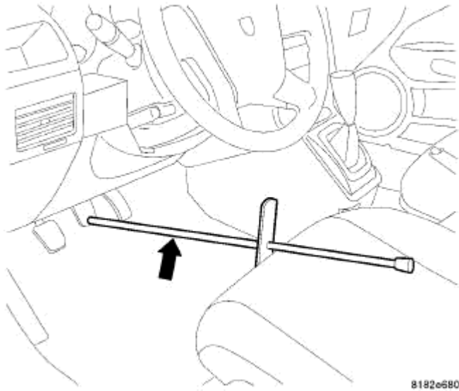
Fig. 36: BRAKE PEDAL HOLDING TOOL Courtesy of CHRYSLER LLC
