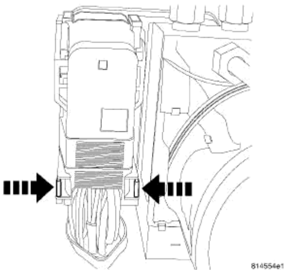
Fig. 46: ABM Connector Release Tabs
