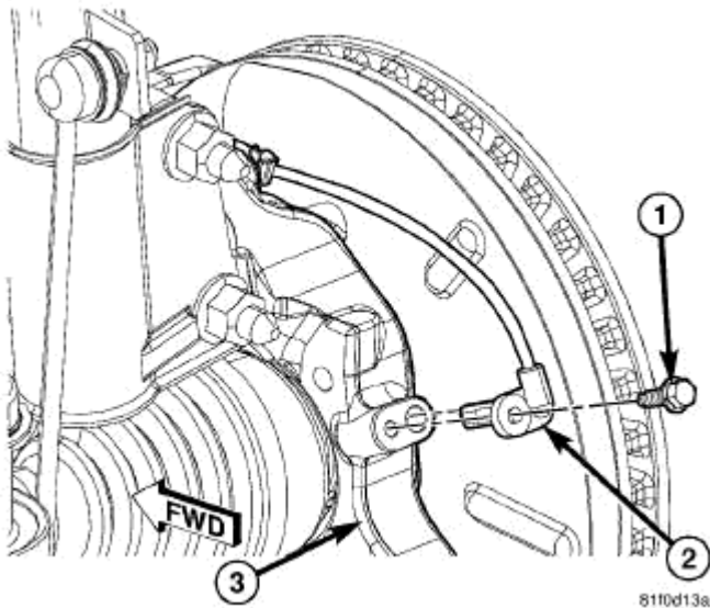
Fig. 16: Front Wheel Speed Sensor
