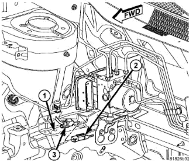
Fig. 12: Front Wheel Speed Sensor Wiring Connector Courtesy of CHRYSLER LLC
