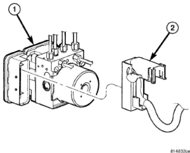
Fig. 47: Wiring Harness Connector At ABM
