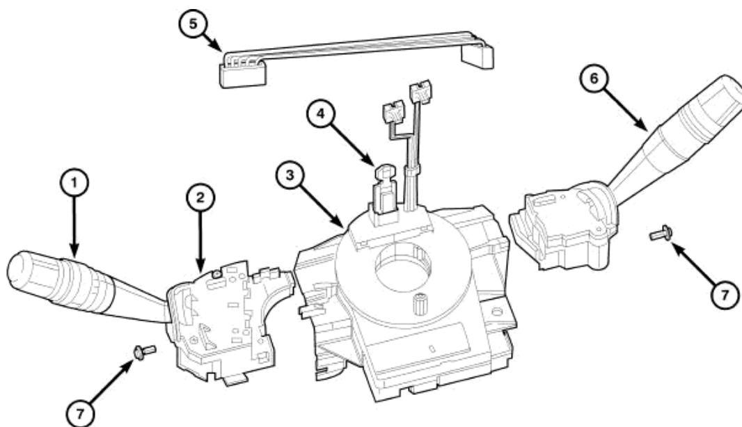
Fig. 10: Steering Control Module Courtesy of CHRYSLER LLC
