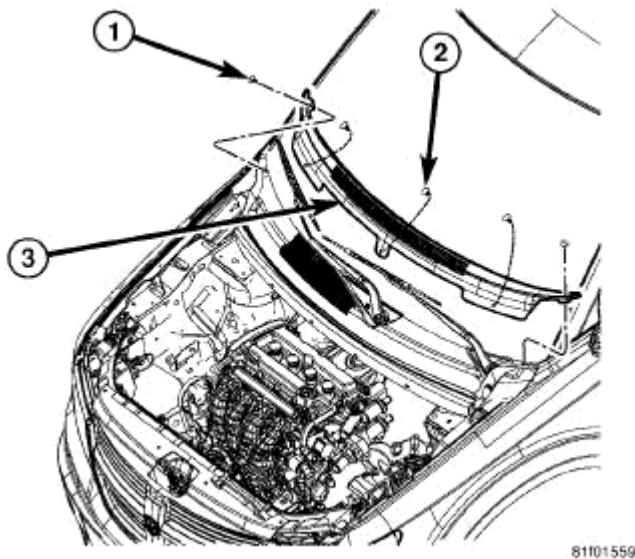
Fig. 37: Cowl Top Screen Courtesy of CHRYSLER LLC
