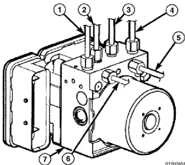
Fig. 45: Identifying Brake Tubes At Hydraulic Control Unit Courtesy of CHRYSLER LLC
