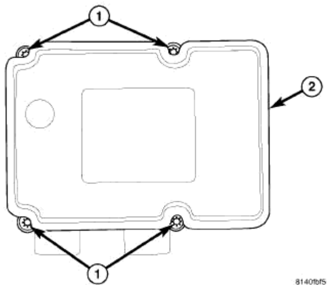
Fig. 55: ABM Mounting Screws - With Traction Control Courtesy of CHRYSLER LLC
