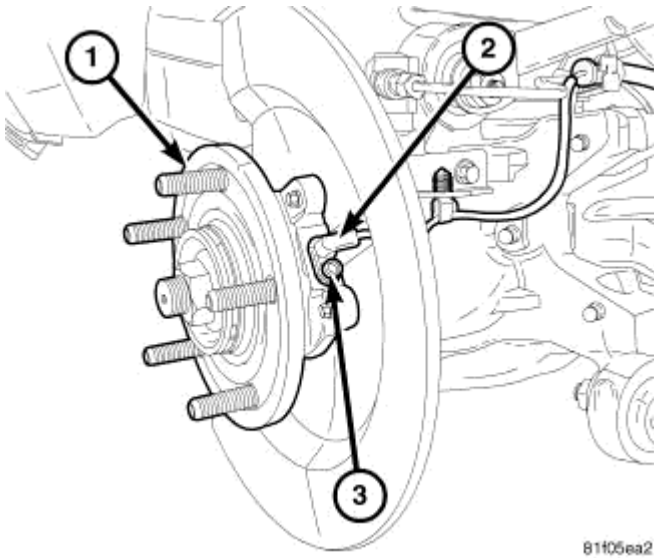
Fig. 20: Hub And Bearing Courtesy of CHRYSLER LLC
