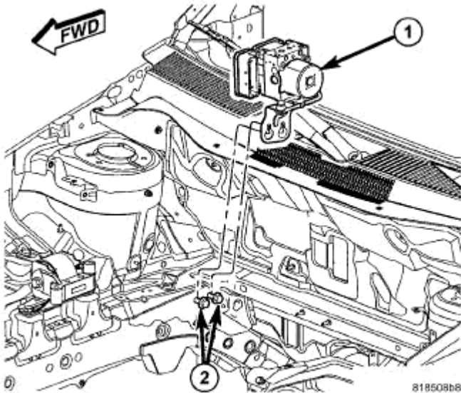
Fig. 57: Locating Integrated Control Unit (ICU) Courtesy of CHRYSLER LLC
