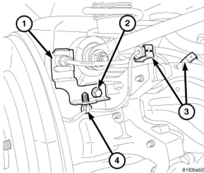
Fig. 22: Brake Tube Routing Bracket Courtesy of CHRYSLER LLC
