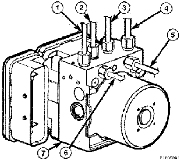
Fig. 40: Identifying Brake Tubes At Hydraulic Control Unit Courtesy of CHRYSLER LLC
