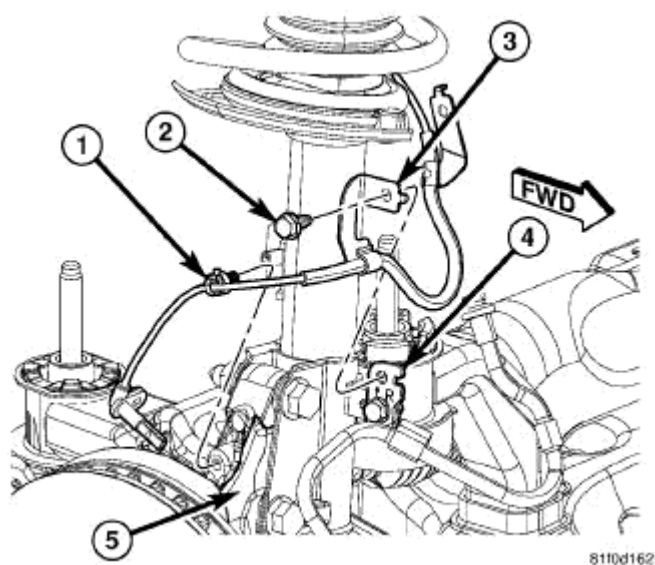
Fig. 17: Wheel Speed Sensor Routing & Brake Flex Hose Bracket Courtesy of CHRYSLER LLC
