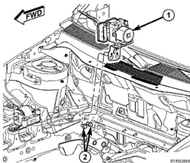
Fig. 43: Locating Integrated Control Unit (ICU)
