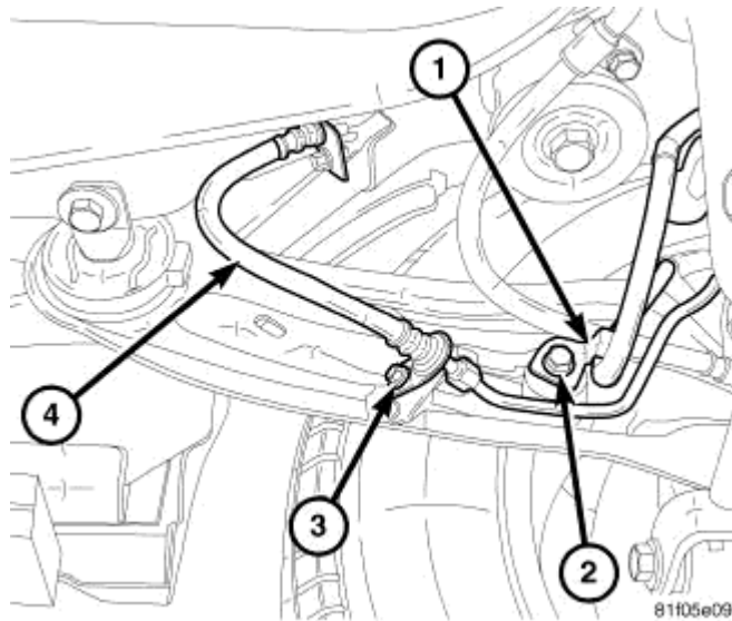
Fig. 25: Brake Flex Hose And Tube Bracket Courtesy of CHRYSLER LLC
