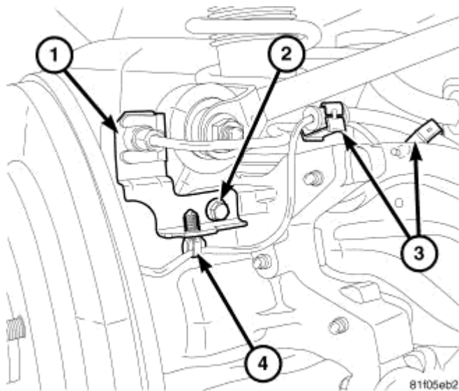
Fig. 31: Brake Tube Routing Bracket Courtesy of CHRYSLER LLC
