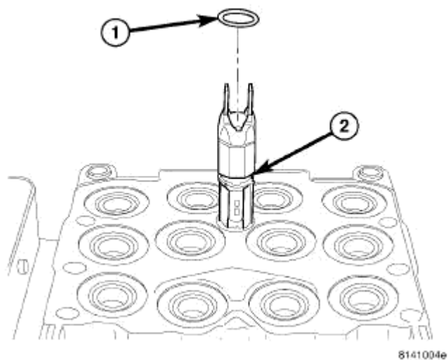
Fig. 53: Internal Pump Connector O-Ring Courtesy of CHRYSLER LLC
