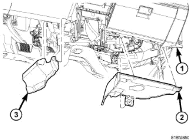
Fig. 6: Lower Instrument Panel Silencer Courtesy of CHRYSLER LLC
