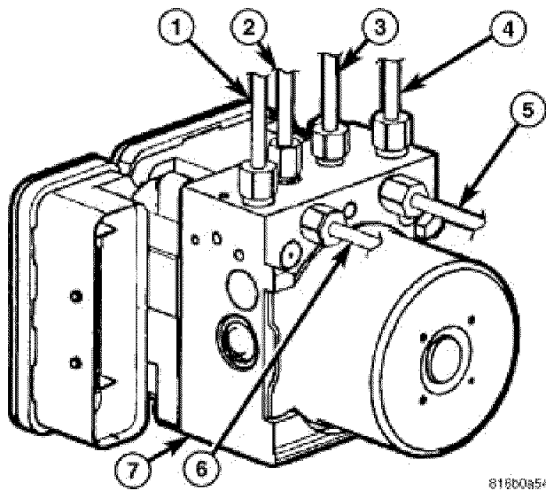
Fig. 69: Identifying Brake Tubes At Hydraulic Control Unit Courtesy of CHRYSLER LLC
