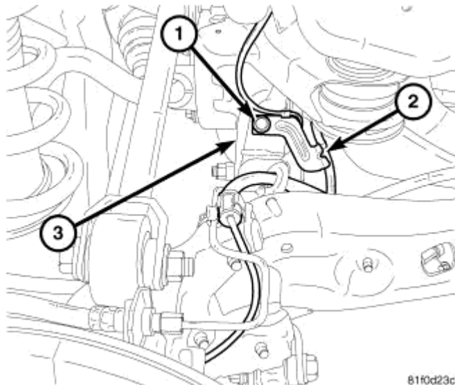
Fig. 28: Wheel Speed Sensor Routing Clamp Courtesy of CHRYSLER LLC
