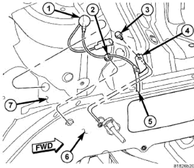
Fig. 13: Front Wheel Speed Sensor Mounting To Body Courtesy of CHRYSLER LLC
