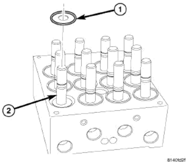
Fig. 52: Solenoid Valve Seal Courtesy of CHRYSLER LLC
