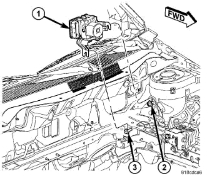
Fig. 66: Integrated Control Unit Mounting - RHD Courtesy of CHRYSLER LLC
