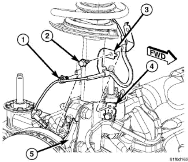
Fig. 14: Wheel Speed Sensor Routing & Brake Flex Hose Bracket Courtesy of CHRYSLER LLC
