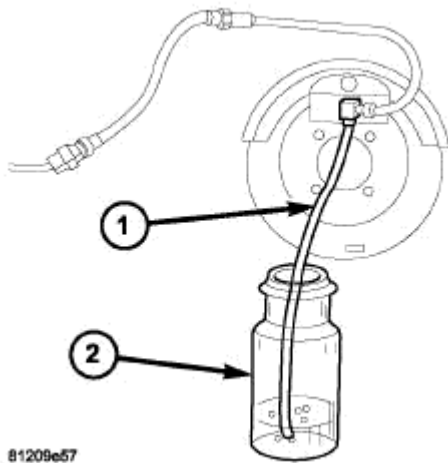
Fig. 65: Bleed Hose Set Up Courtesy of CHRYSLER LLC
