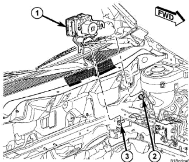
Fig. 48: Integrated Control Unit Mounting - RHD Courtesy of CHRYSLER LLC
