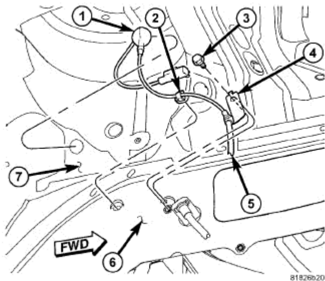
Fig. 18: Front Wheel Speed Sensor Mounting To Body Courtesy of CHRYSLER LLC
