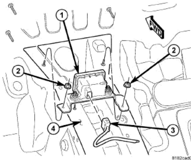
Fig. 7: Dynamics Sensor Courtesy of CHRYSLER LLC
