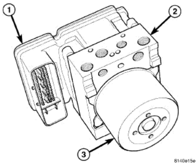
Fig. 33: Integrated Control Unit Courtesy of CHRYSLER LLC
