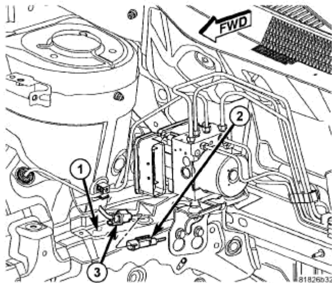
Fig. 19: Front Wheel Speed Sensor Wiring Connector Courtesy of CHRYSLER LLC
