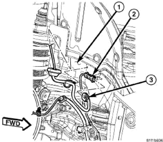
Fig. 27: Wheel Speed Sensor Wiring Connector Courtesy of CHRYSLER LLC
