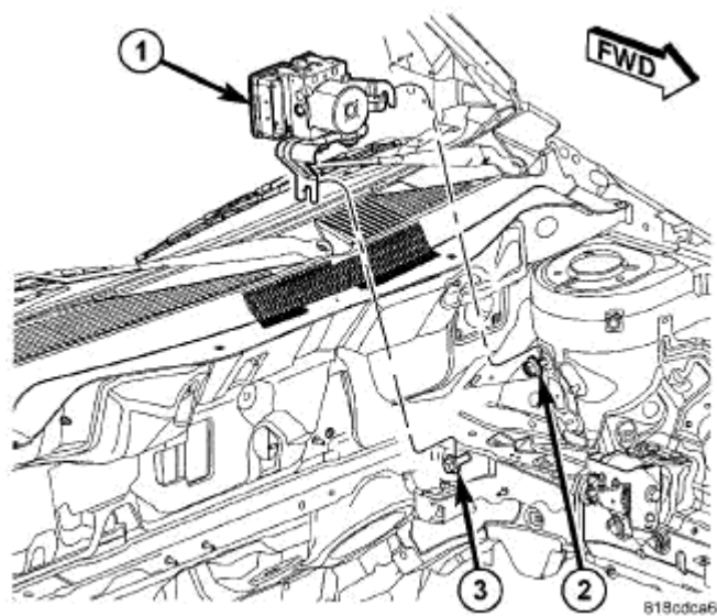
Fig. 35: Integrated Control Unit Mounting - RHD Courtesy of CHRYSLER LLC
