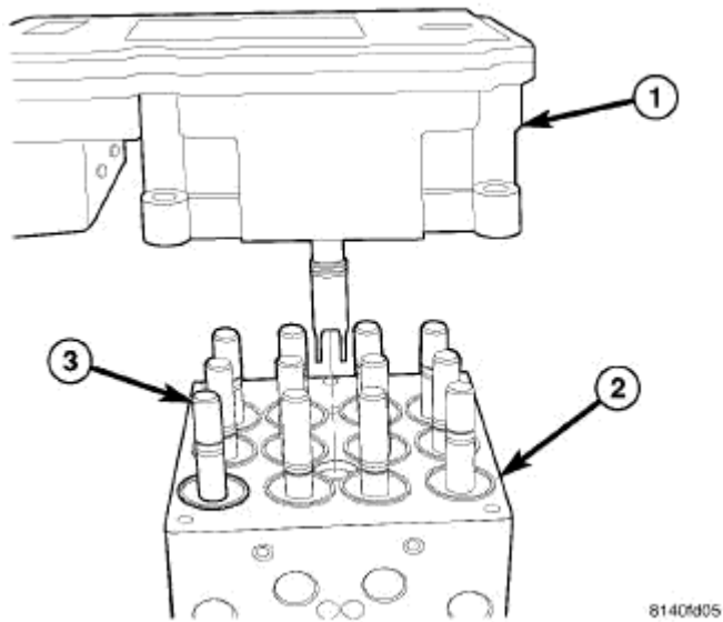
Fig. 51: Identifying ABM, HCU, & Solenoid Valve Stem Courtesy of CHRYSLER LLC
