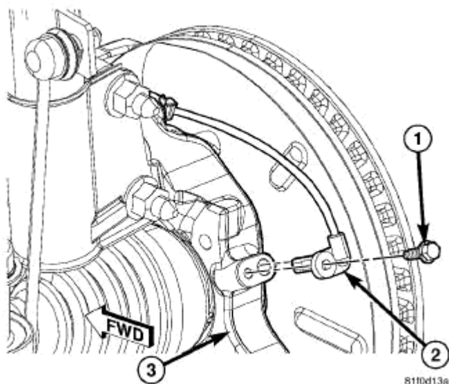
Fig. 11: Front Wheel Speed Sensor
