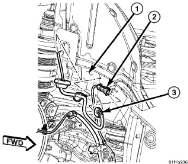
Fig. 26: Wheel Speed Sensor Wiring Connector Courtesy of CHRYSLER LLC
