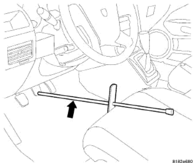
Fig. 44: BRAKE PEDAL HOLDING TOOL Courtesy of CHRYSLER LLC
