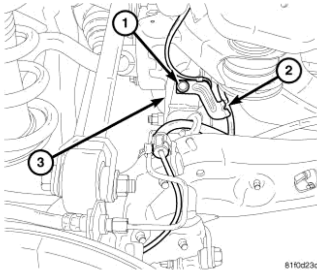
Fig. 24: Wheel Speed Sensor Routing Clamp Courtesy of CHRYSLER LLC
