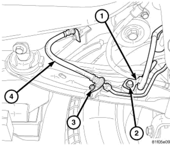
Fig. 29: Brake Flex Hose And Tube Bracket Courtesy of CHRYSLER LLC
