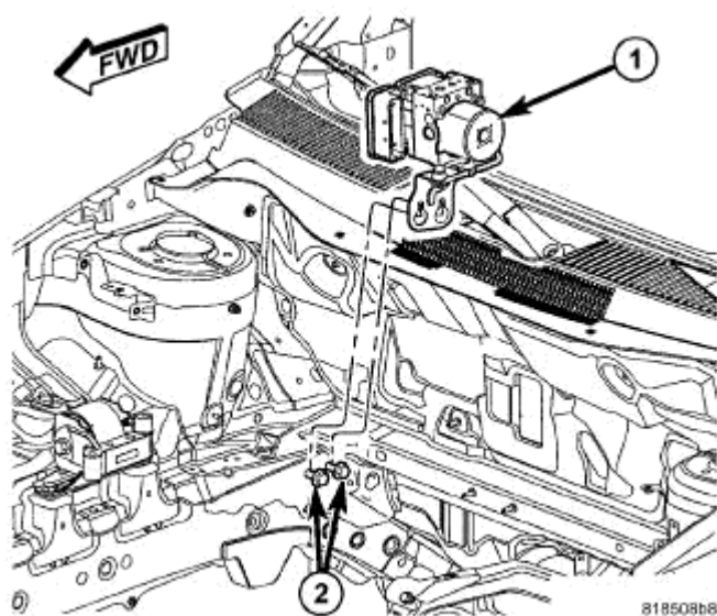
Fig. 34: Locating Integrated Control Unit (ICU) Courtesy of CHRYSLER LLC
