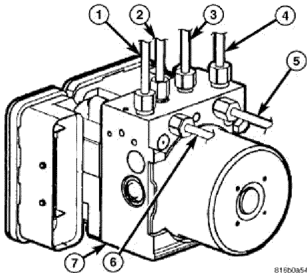
Fig. 68: Identifying Brake Tubes At Hydraulic Control Unit Courtesy of CHRYSLER LLC
