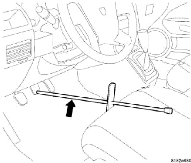
Fig. 64: BRAKE PEDAL HOLDING TOOL Courtesy of CHRYSLER LLC
