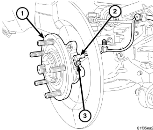
Fig. 23: Hub And Bearing Courtesy of CHRYSLER LLC
