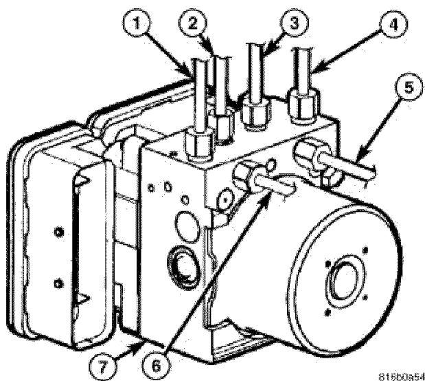
Fig. 60: Identifying Brake Tubes At Hydraulic Control Unit Courtesy of CHRYSLER LLC
