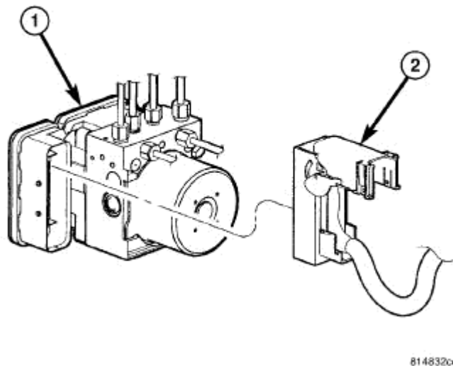
Fig. 58: Wiring Harness Connector At ABM Courtesy of CHRYSLER LLC
