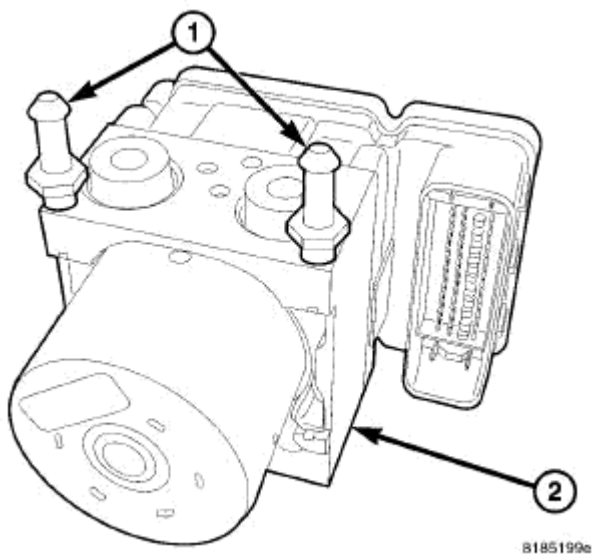
Fig. 56: ICU Mounting Pins Courtesy of CHRYSLER LLC
