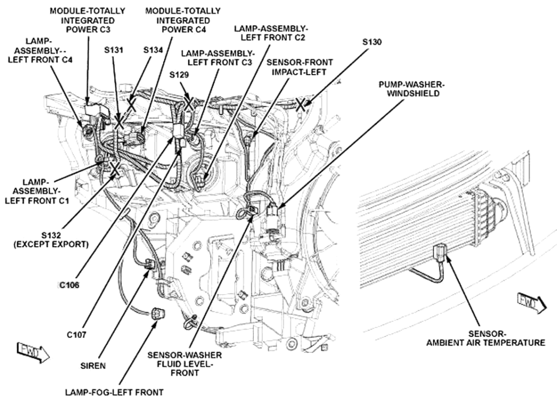
Fig. 1: Locating Totally Integrated Power Module Courtesy of CHRYSLER CORP.
