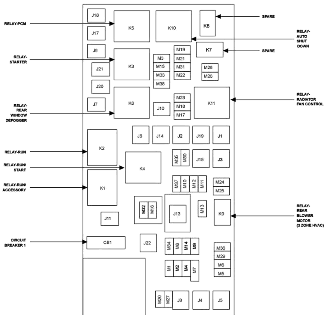
Fig. 2: Identifying Totally Integrated Power Module Components Courtesy of CHRYSLER CORP.
