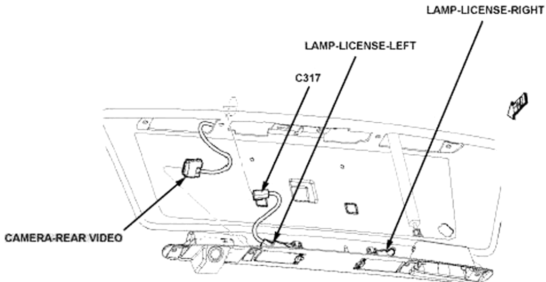
Fig. 38: Liftgate Courtesy of CHRYSLER LLC
