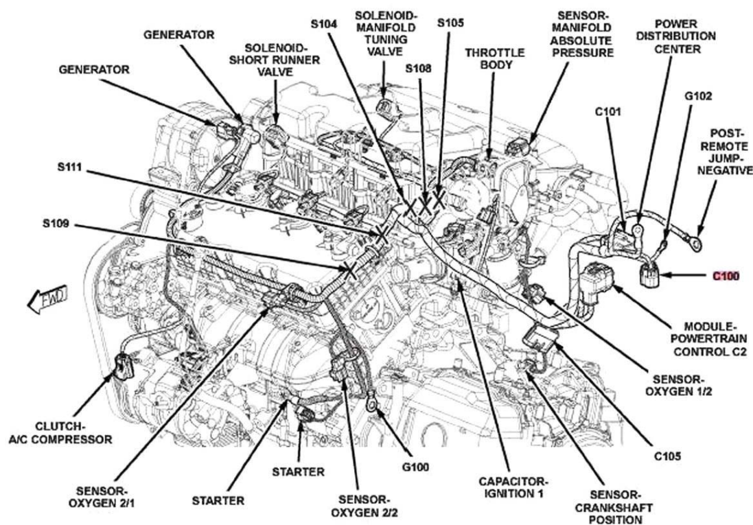
Fig. 19: Left Side & Rear Of Engine (3.5L)
