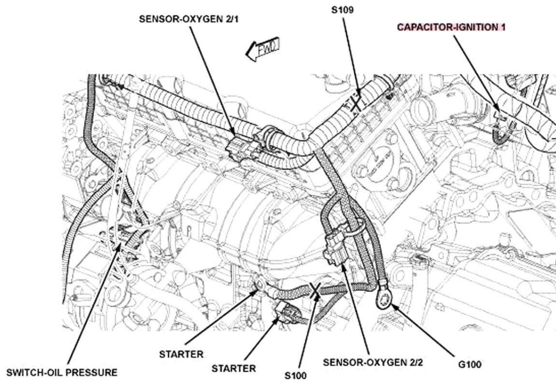
Fig. 41: Left Rear Of Engine (3.5L) Courtesy of CHRYSLER LLC
