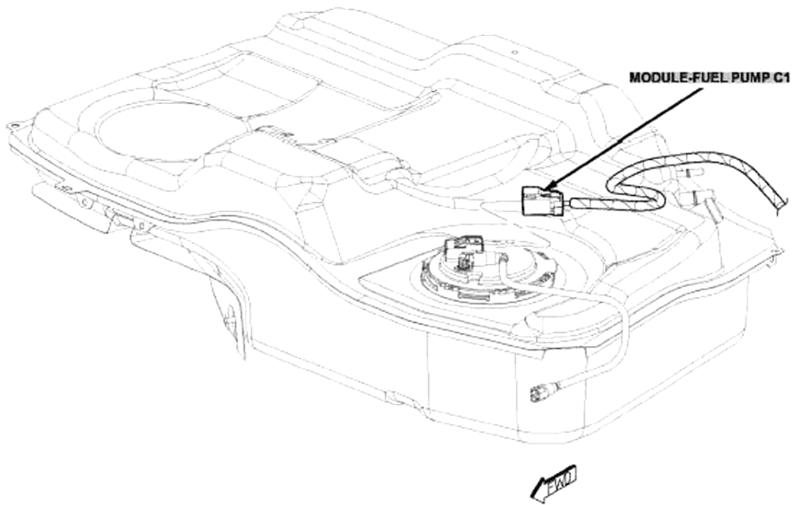
Fig. 50: Top Of Fuel Tank (Except AWD) Courtesy of CHRYSLER LLC
