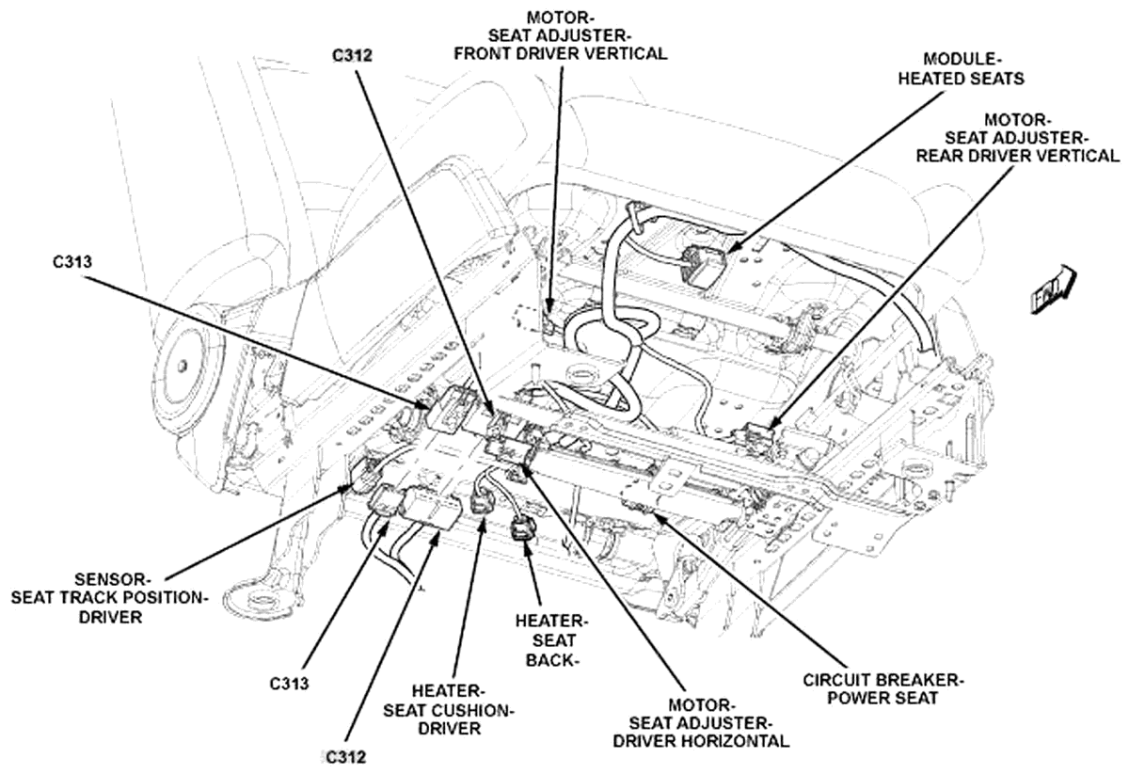
Fig. 34: Driver's Seat
