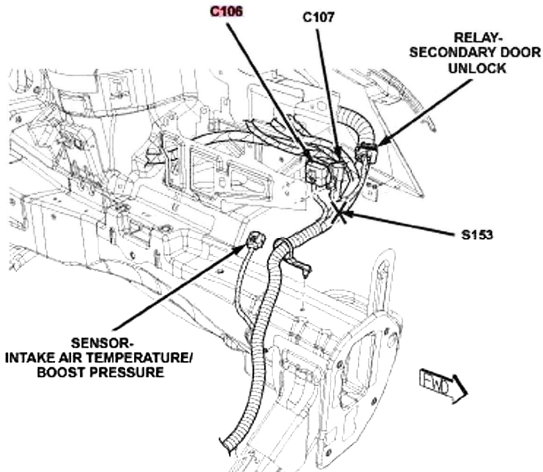
Fig. 21: Left Side Of Engine Compartment Courtesy of CHRYSLER LLC
