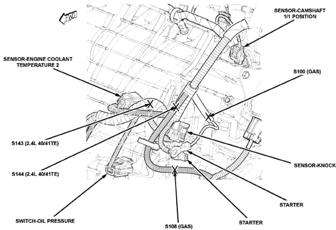
Fig. 47: Left Rear Of Engine (2.4L & 3.5L)
