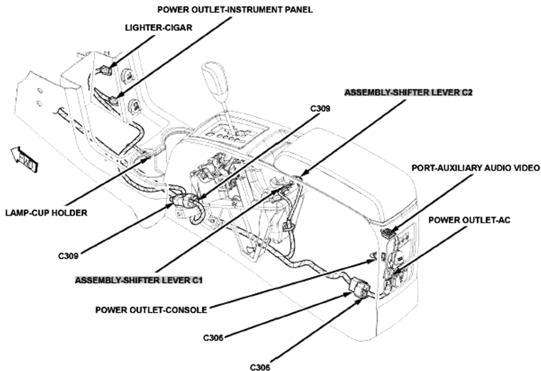
Fig. 15: Center Console
