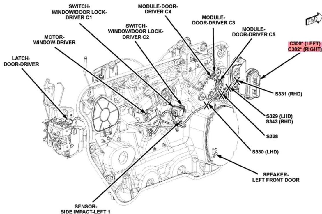
Fig. 26: Driver's Door (Front Passenger's Similar)
