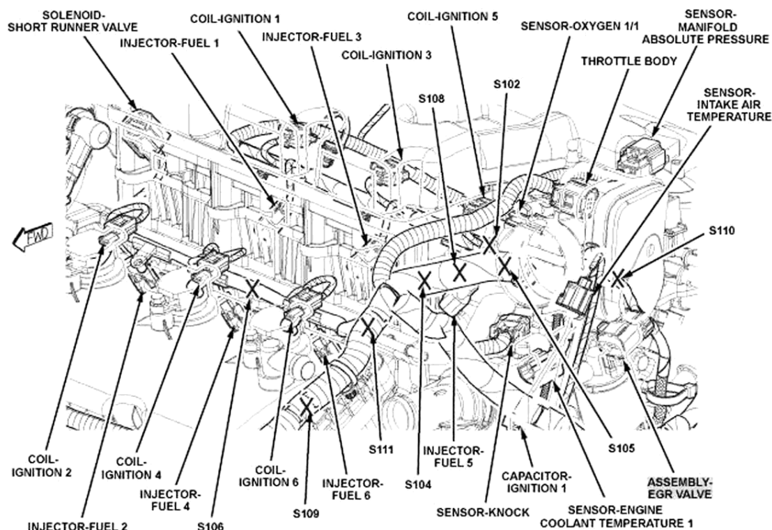
Fig. 13: Top Of Engine (3.5L) Courtesy of CHRYSLER LLC
