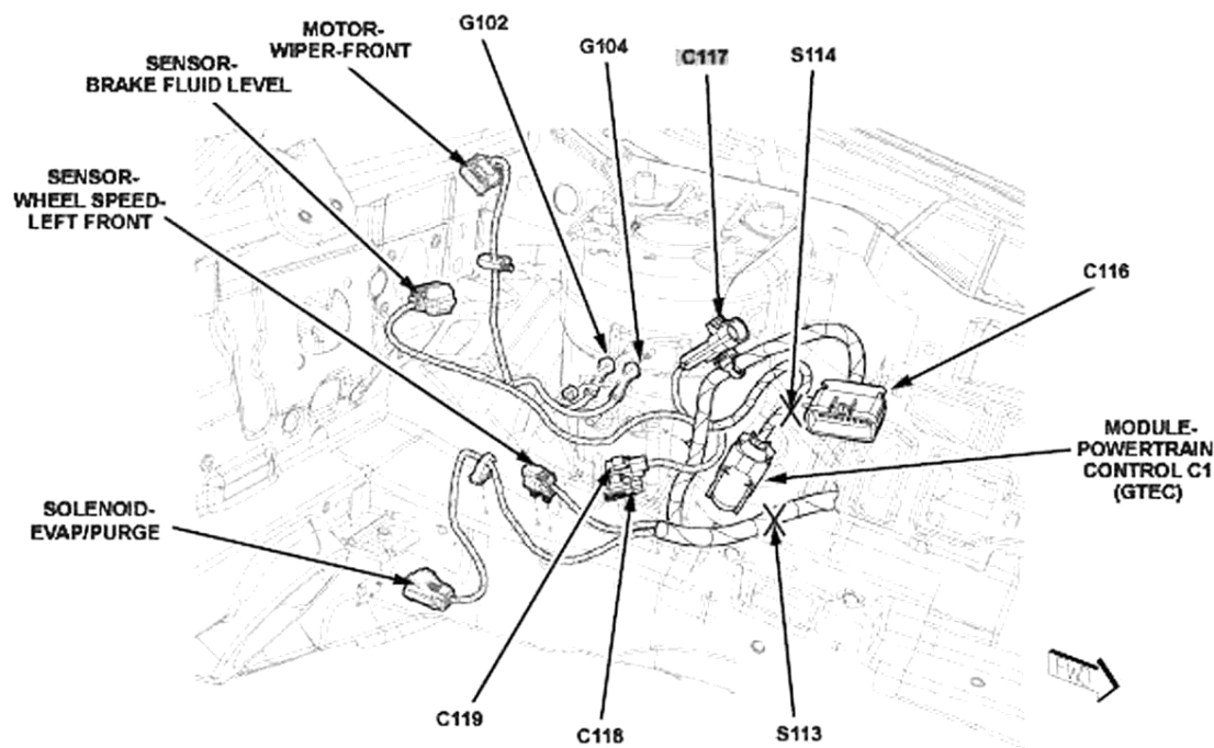
Fig. 22: Left Side Of Engine Compartment Courtesy of CHRYSLER LLC
