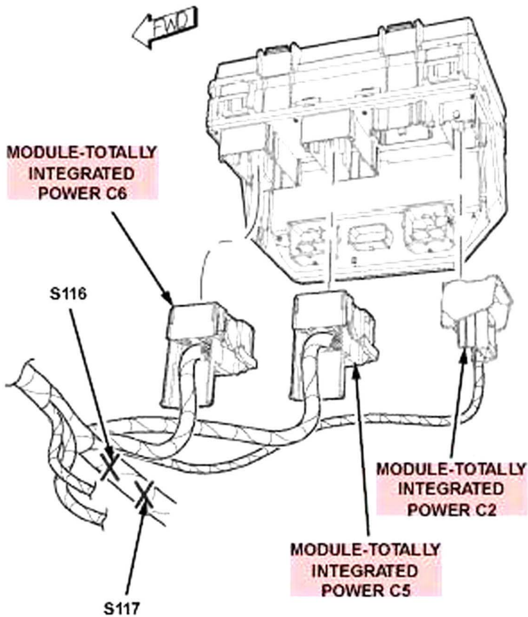
Fig. 51: Totally Integrated Power Module Courtesy of CHRYSLER LLC
