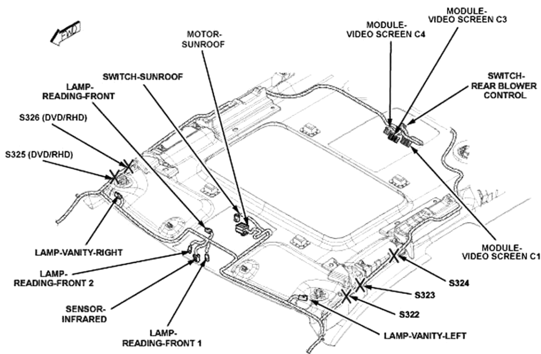
Fig. 44: Roof
