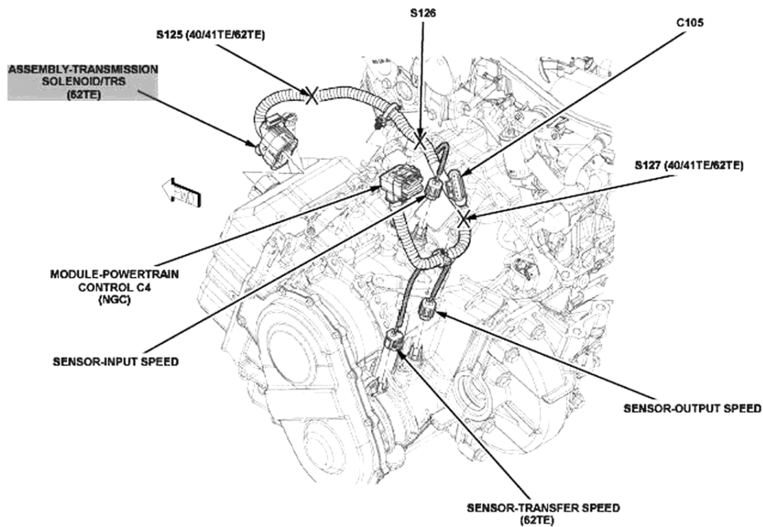
Fig. 17: Transmission (3.5L)
