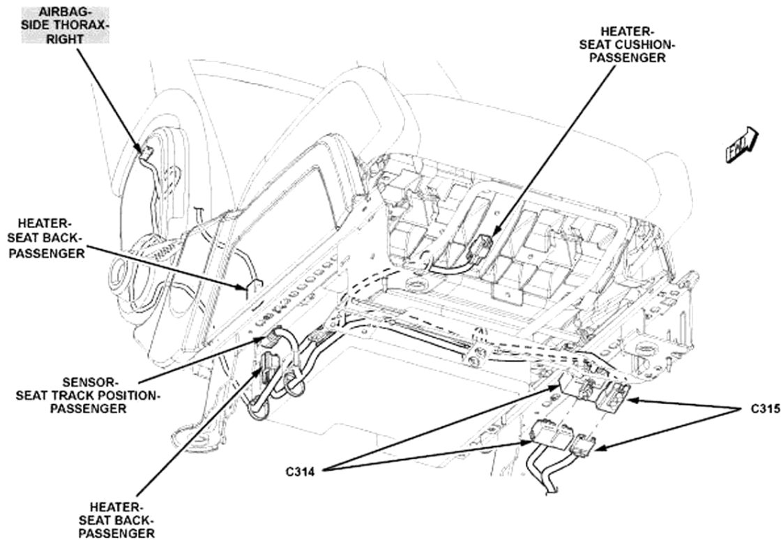
Fig. 9: Front Passenger's Seat
