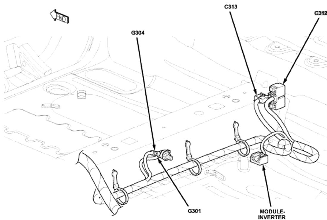
Fig. 35: Floor Under Driver's Seat Courtesy of CHRYSLER LLC
