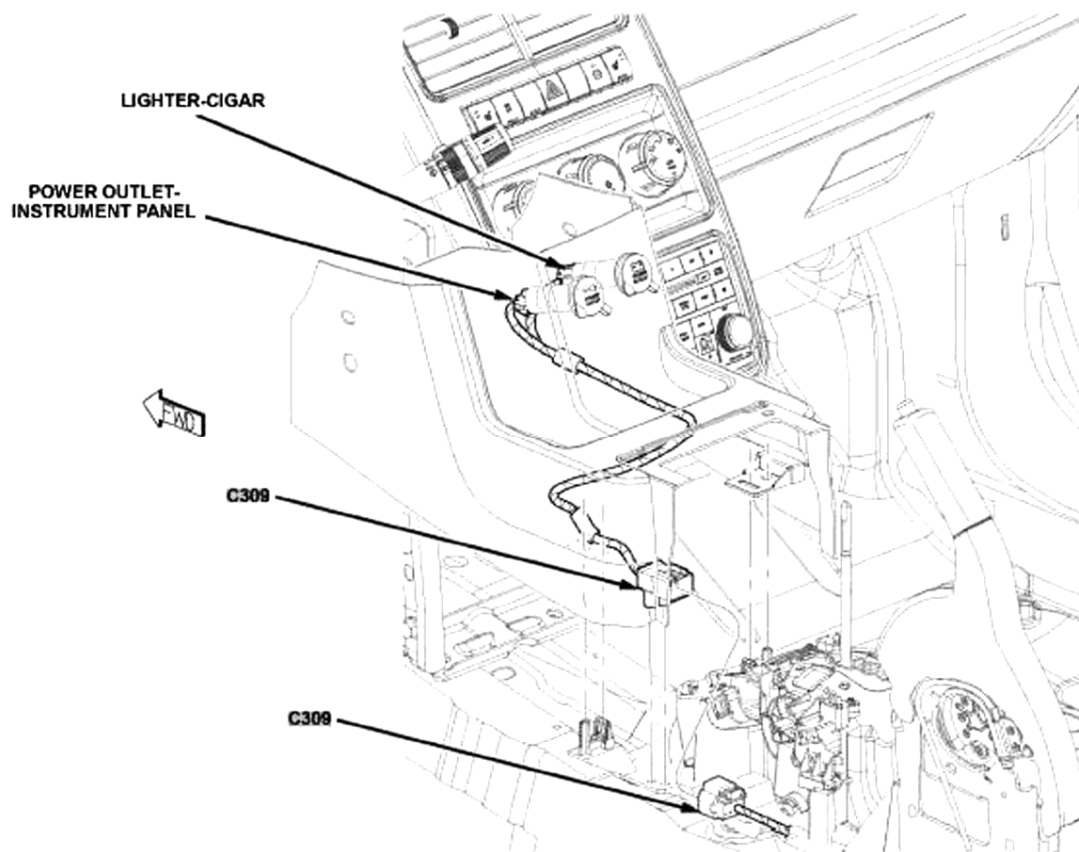
Fig. 31: Under Center Of Dash Courtesy of CHRYSLER LLC
