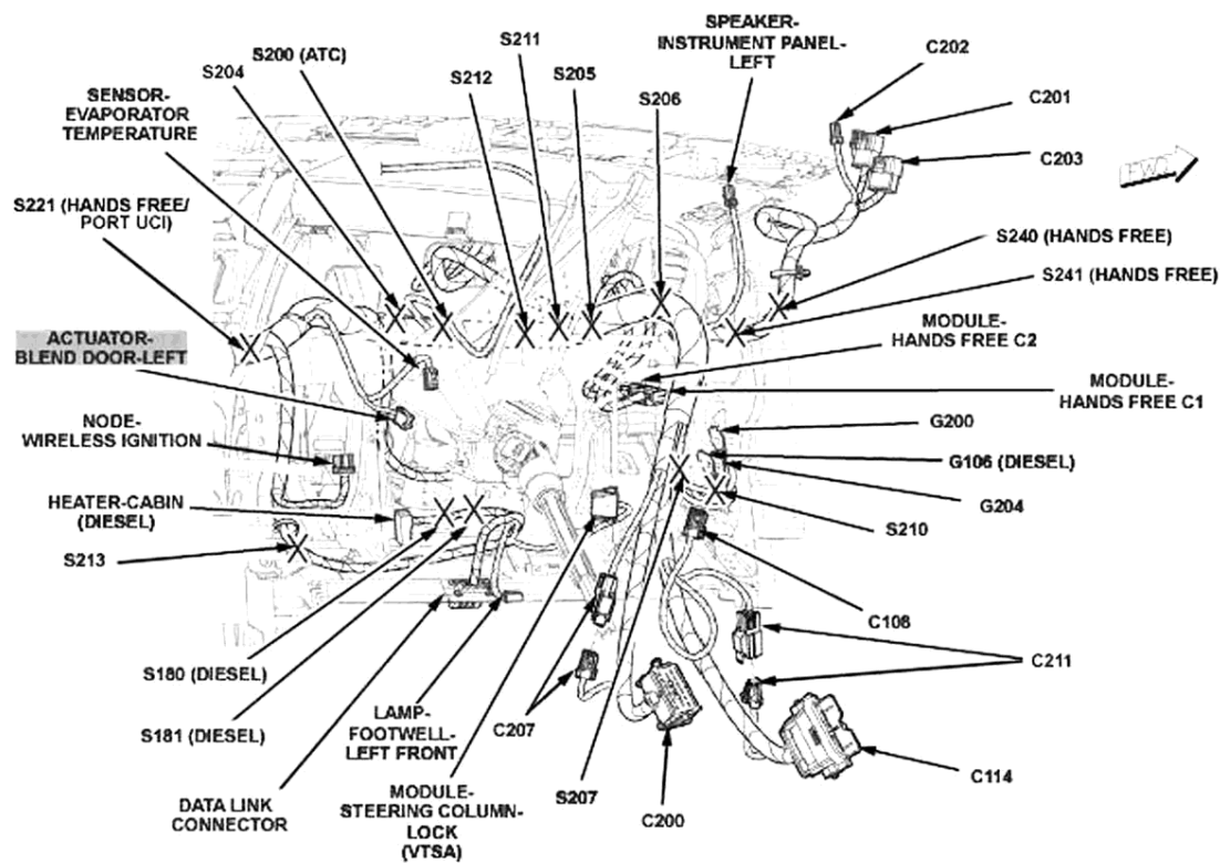
Fig. 2: Left Side Of Dash
