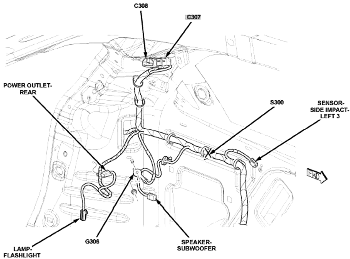
Fig. 30: Left Quarterpanel Courtesy of CHRYSLER LLC
