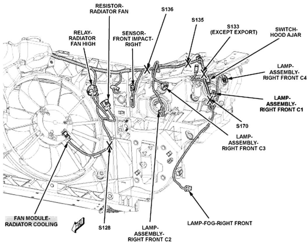
Fig. 46: Right Front Of Engine Compartment Courtesy of CHRYSLER LLC
