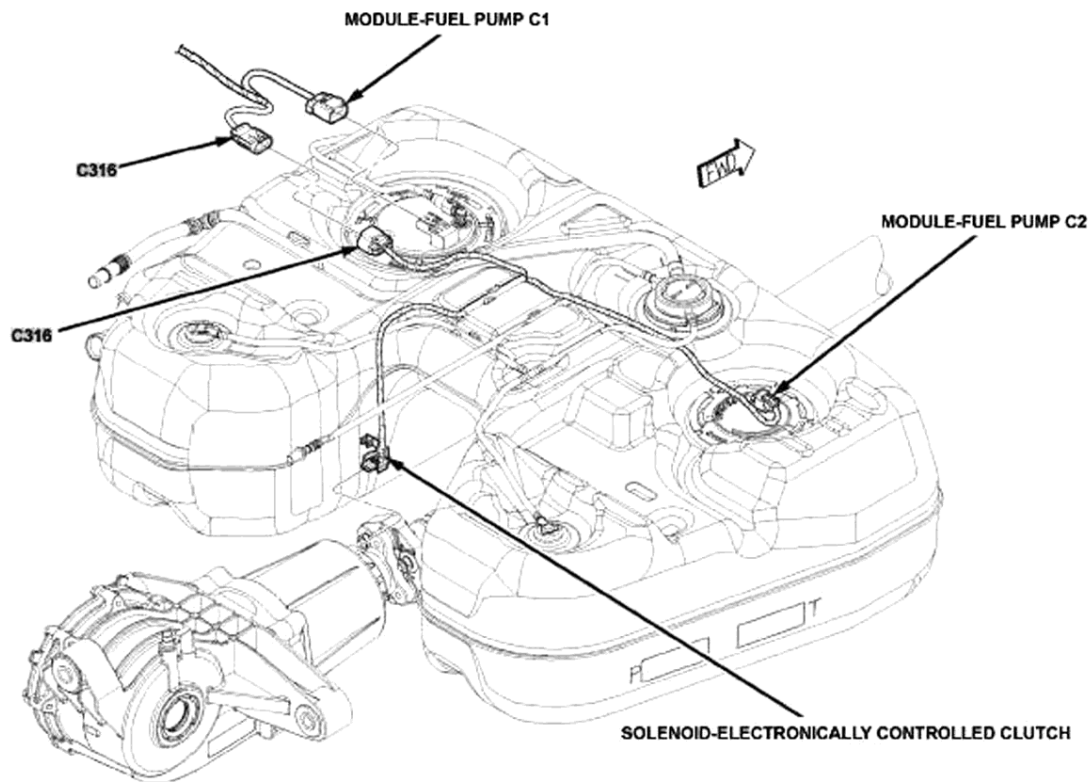
Fig. 37: Top Of Fuel Tank (AWD) Courtesy of CHRYSLER LLC
