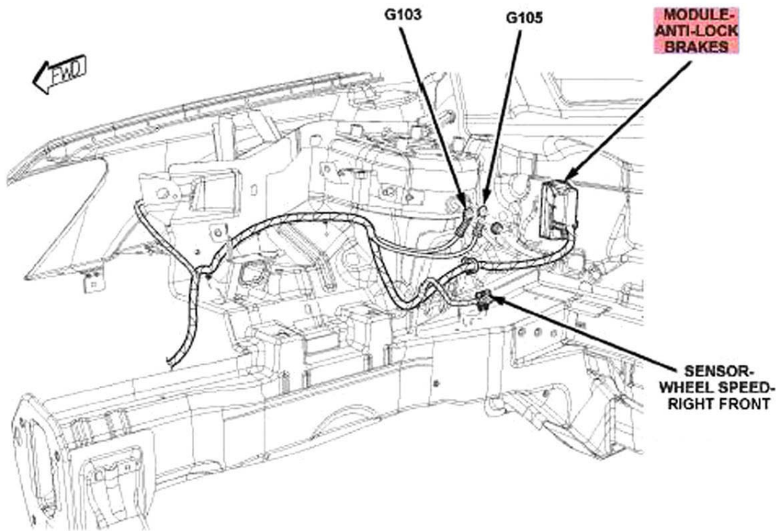
Fig. 49: Right Rear Of Engine Compartment
