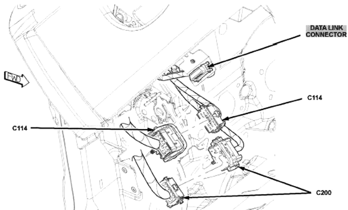
Fig. 45: Lower Left Side Of Dash Courtesy of CHRYSLER LLC
