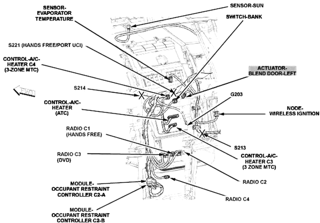
Fig. 1: Center Of Dash Courtesy of CHRYSLER LLC
