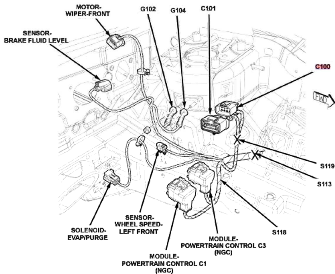
Fig. 18: Left Rear Of Engine Compartment Courtesy of CHRYSLER LLC
