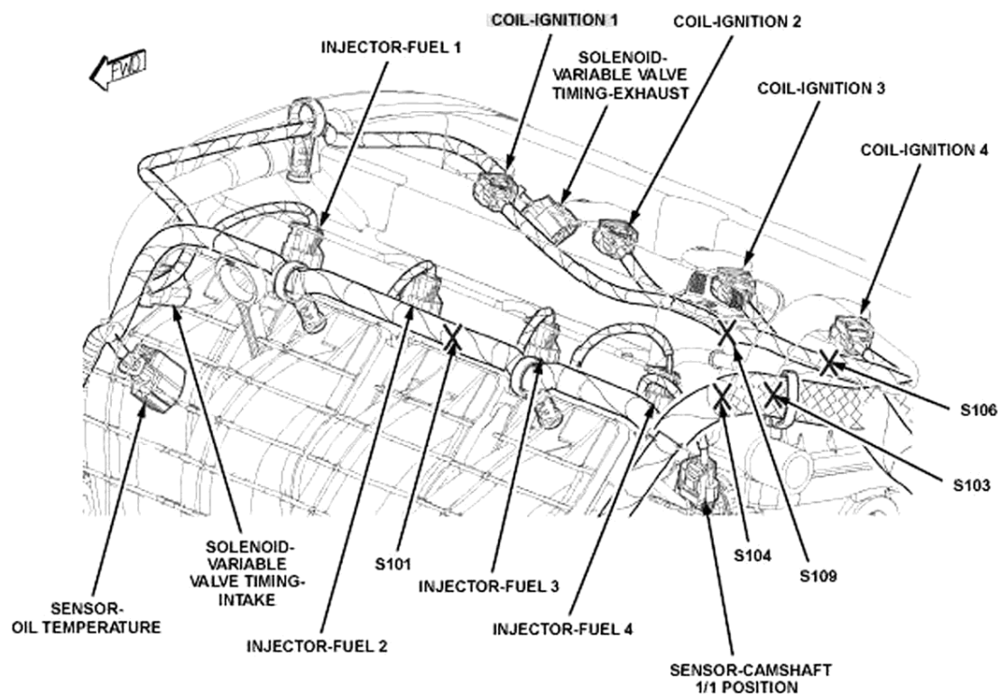
Fig. 43: Top Of Engine (2.4L) Courtesy of CHRYSLER LLC
