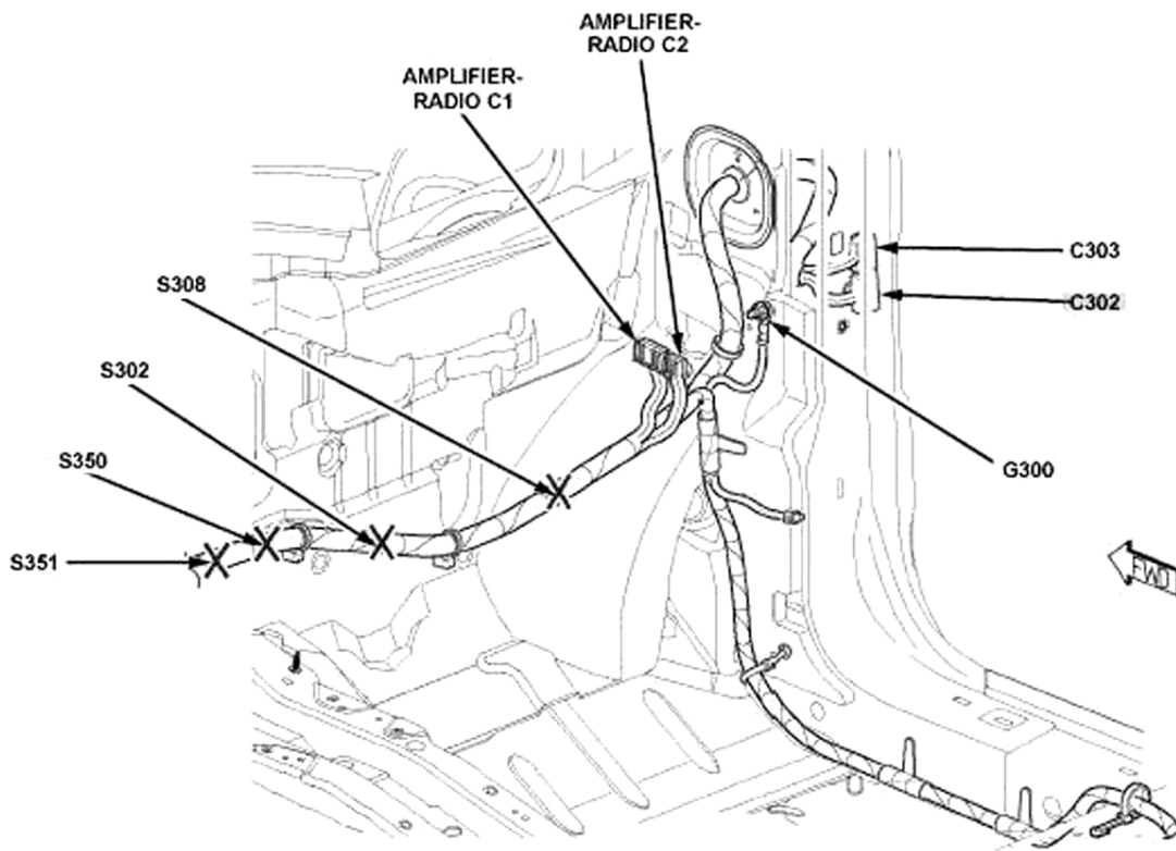
Fig. 10: Right Kick Panel Courtesy of CHRYSLER LLC
