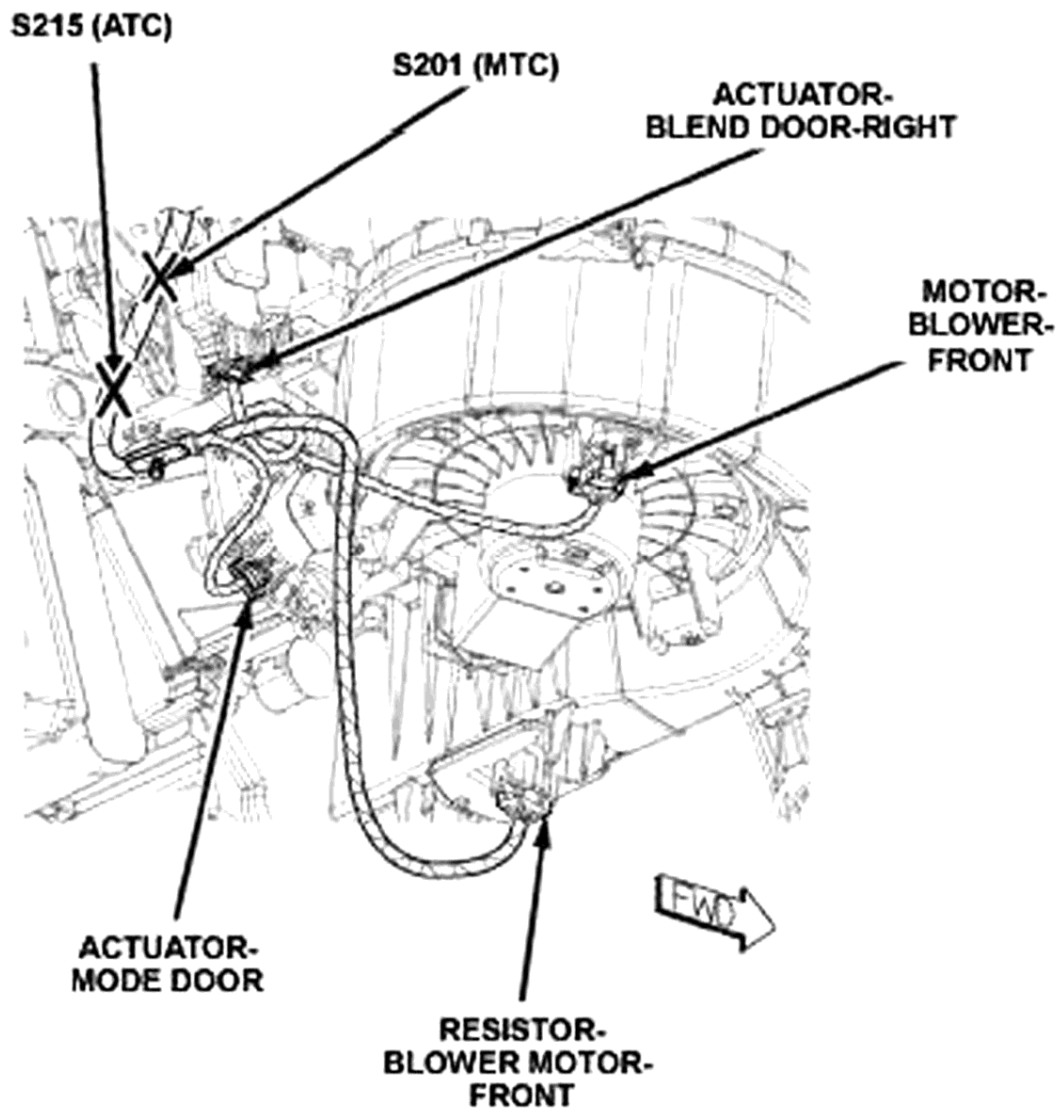
Fig. 3: Right Side Of Dash Courtesy of CHRYSLER LLC
