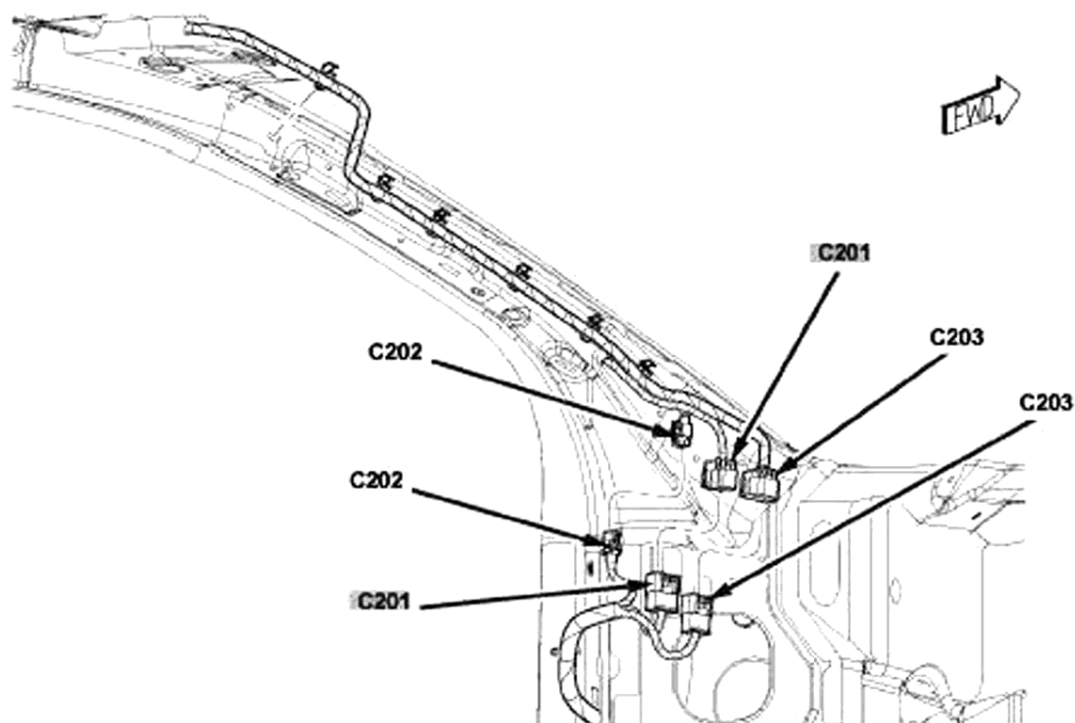
Fig. 24: Left "A" Pillar Courtesy of CHRYSLER LLC
