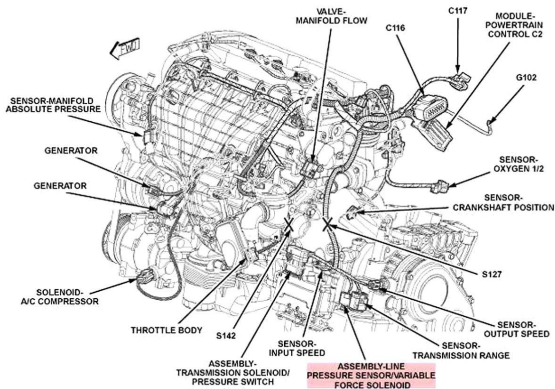
Fig. 13: Top Of Engine (3.5L) Courtesy of CHRYSLER LLC
