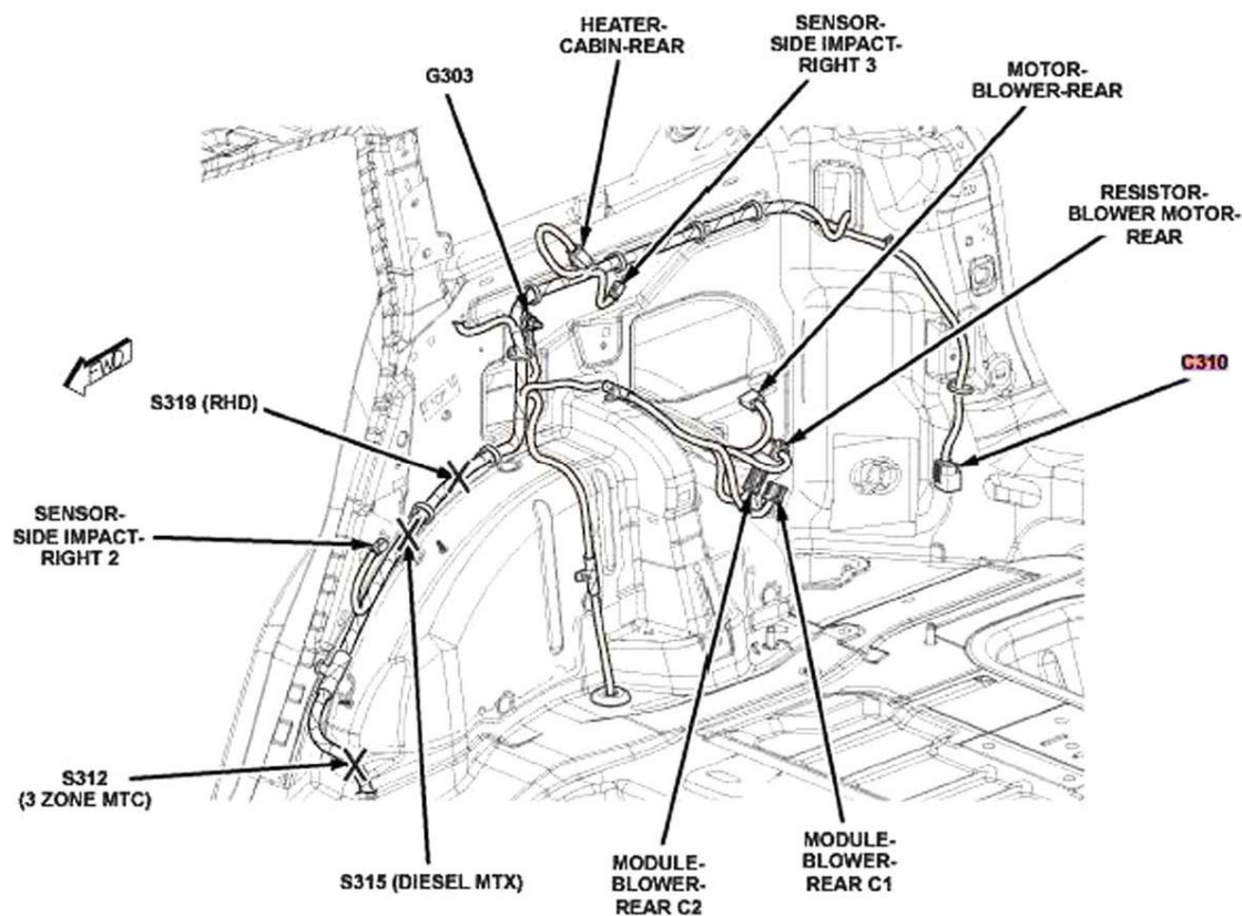
Fig. 32: Right Quarterpanel Courtesy of CHRYSLER LLC
