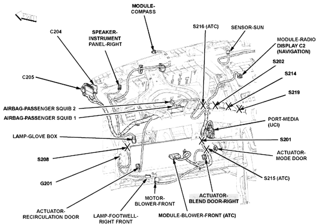
Fig. 4: Right Side Of Dash Courtesy of CHRYSLER LLC
