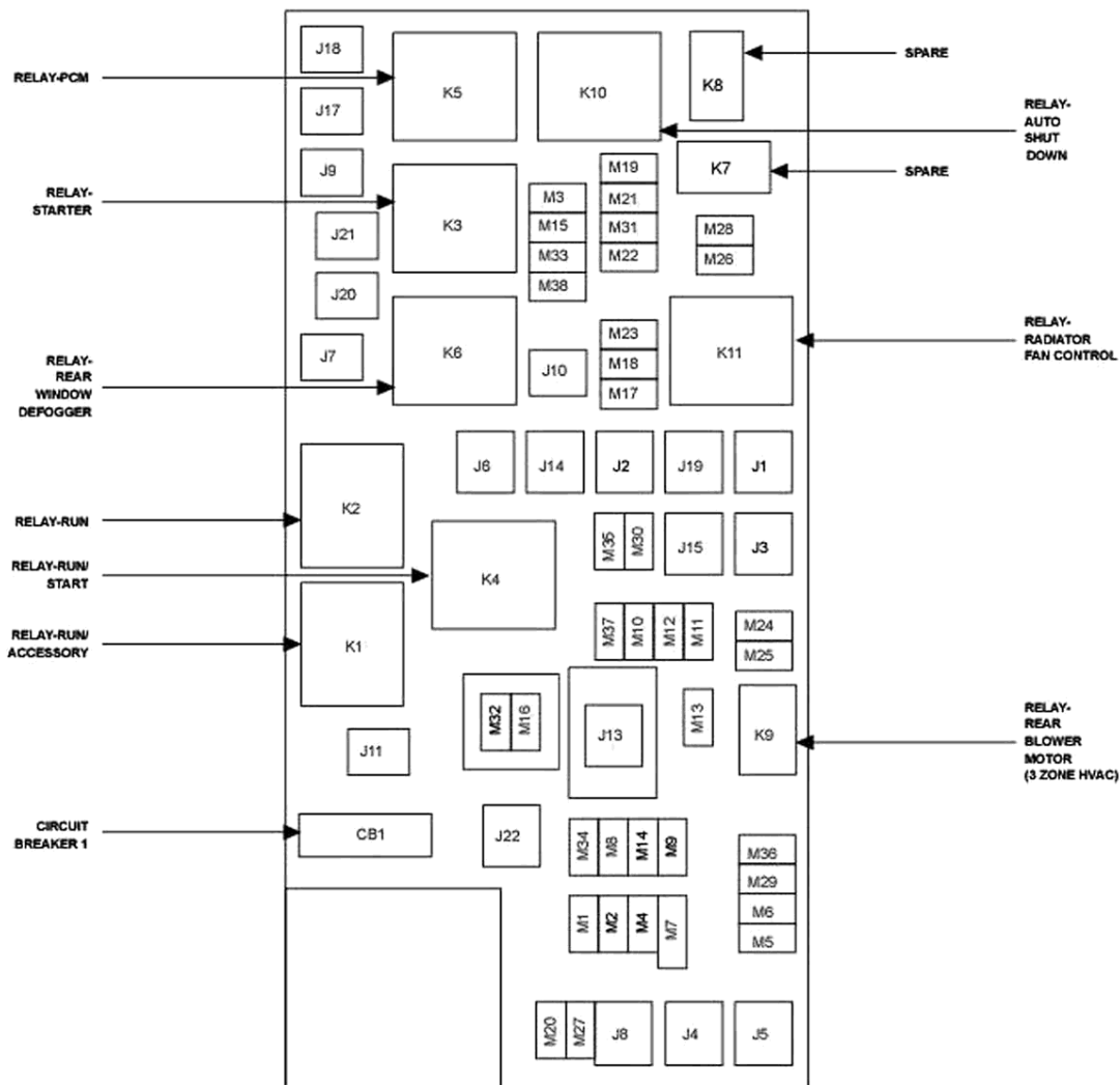
Fig. 42: Totally Integrated Power Module Courtesy of CHRYSLER LLC
