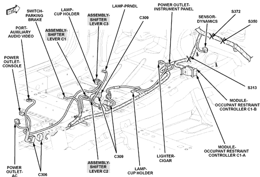
Fig. 16: Left Front Floor Courtesy of CHRYSLER LLC
