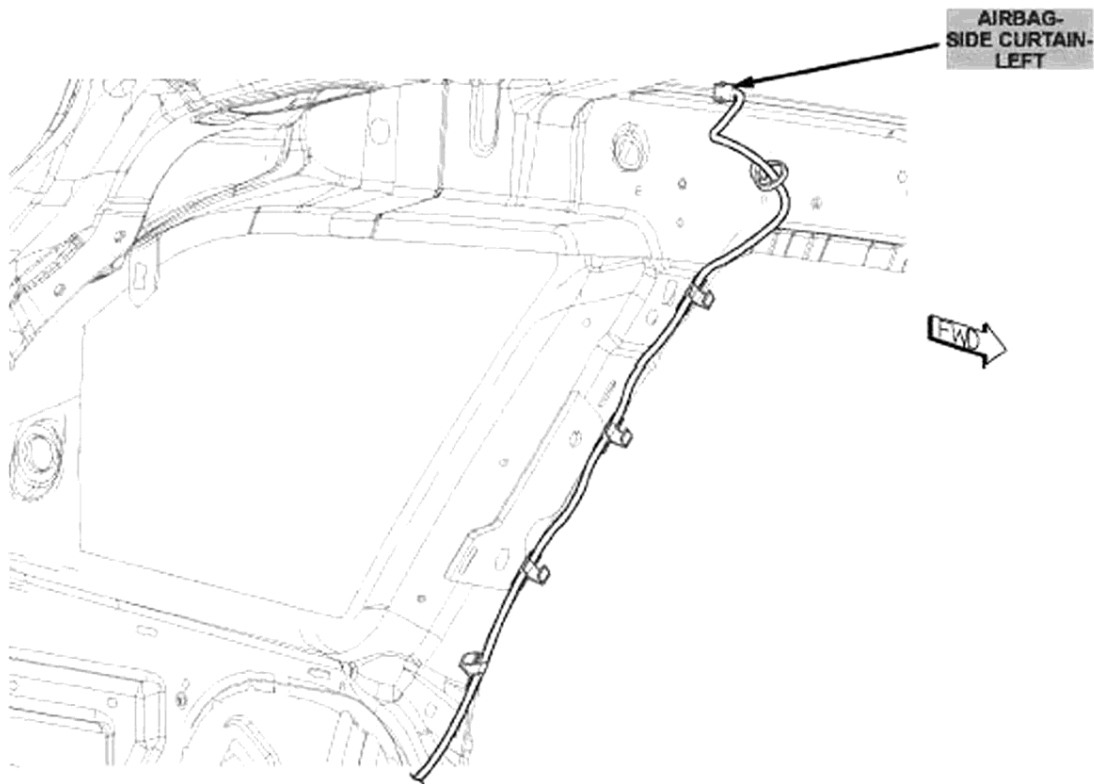
Fig. 6: Left "C" Pillar Courtesy of CHRYSLER LLC
