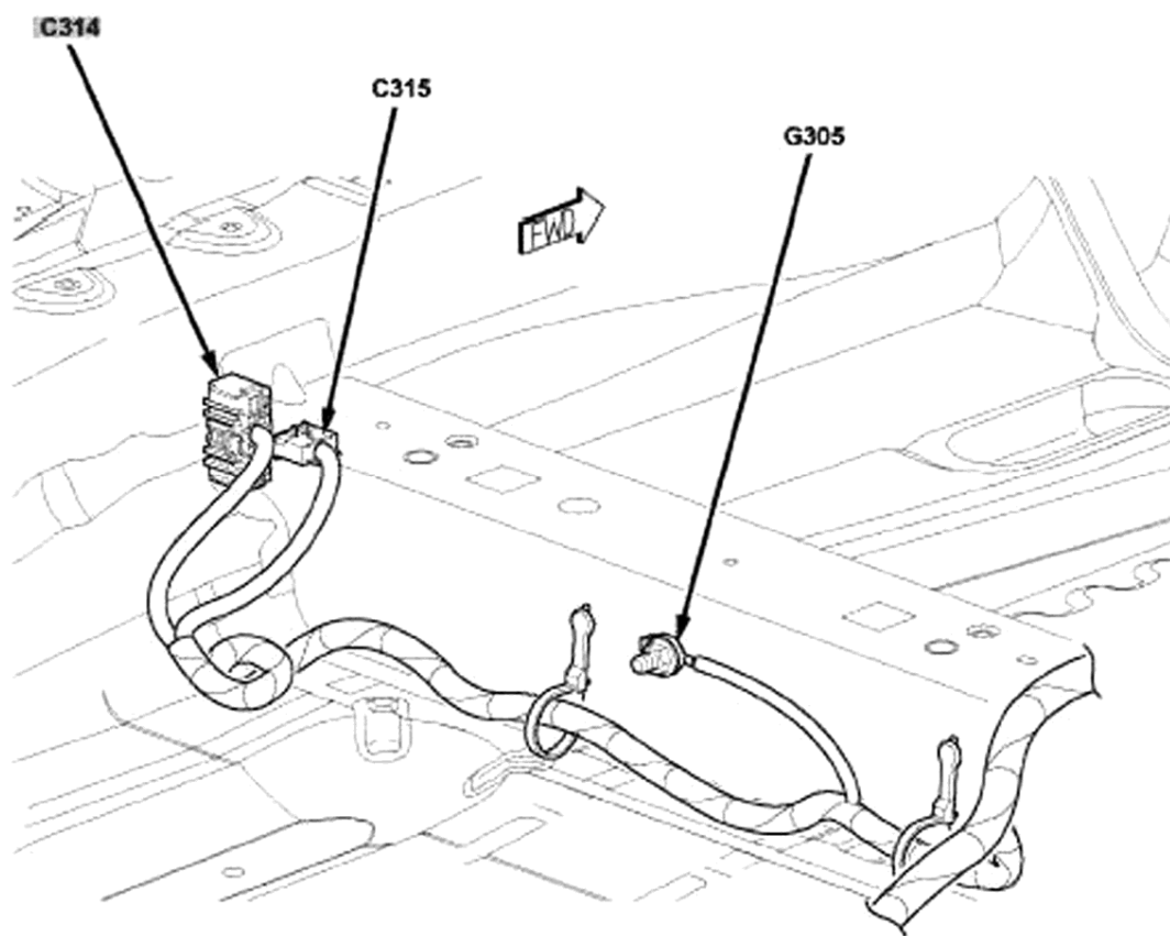
Fig. 36: Floor Under Front Passenger's Seat Courtesy of CHRYSLER LLC
