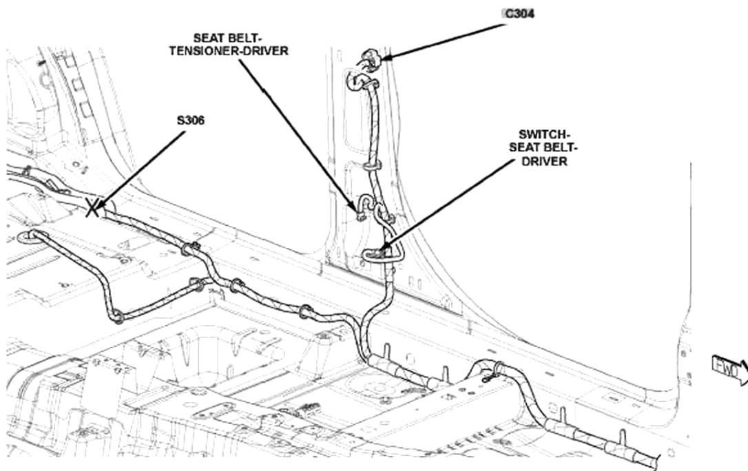
Fig. 28: Left "B" & "C" Pillars
