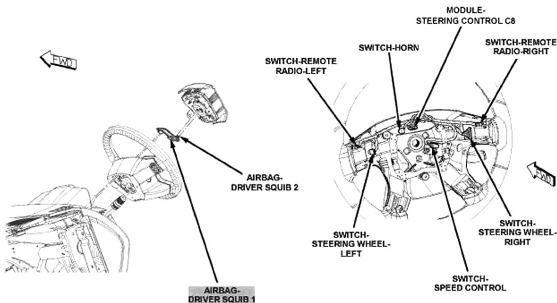
Fig. 5: Steering Wheel Courtesy of CHRYSLER LLC
