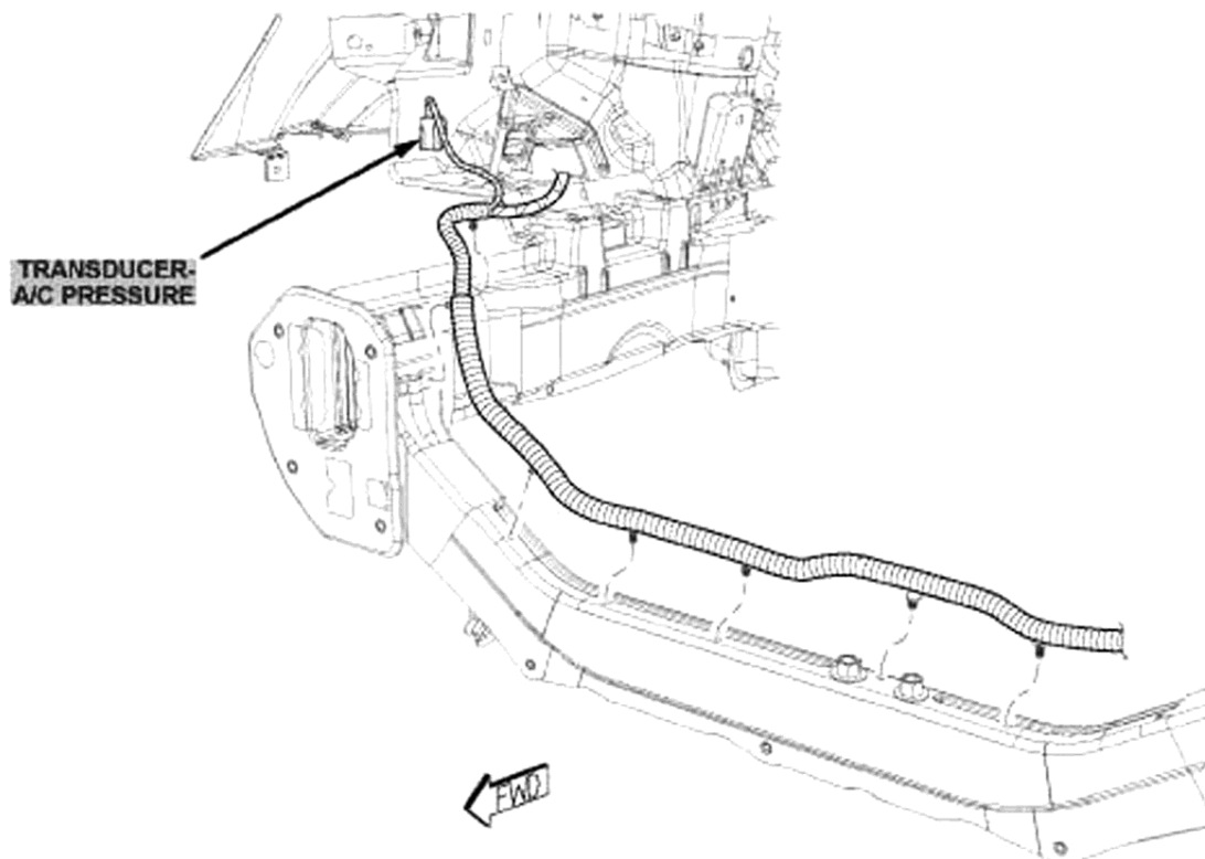
Fig. 53: Right Front Of Engine Compartment
