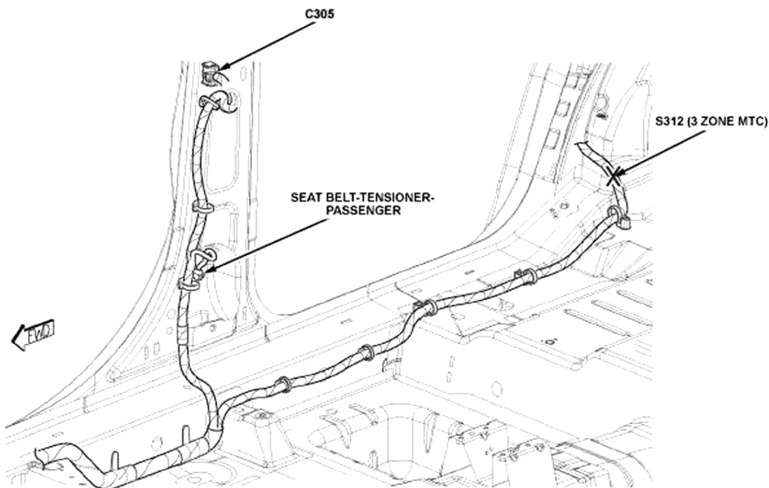
Fig. 29: Right "B" & "C" Pillars
