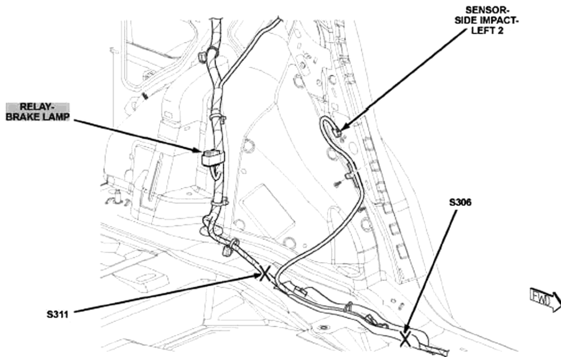
Fig. 52: Left "C" Pillar Courtesy of CHRYSLER LLC
