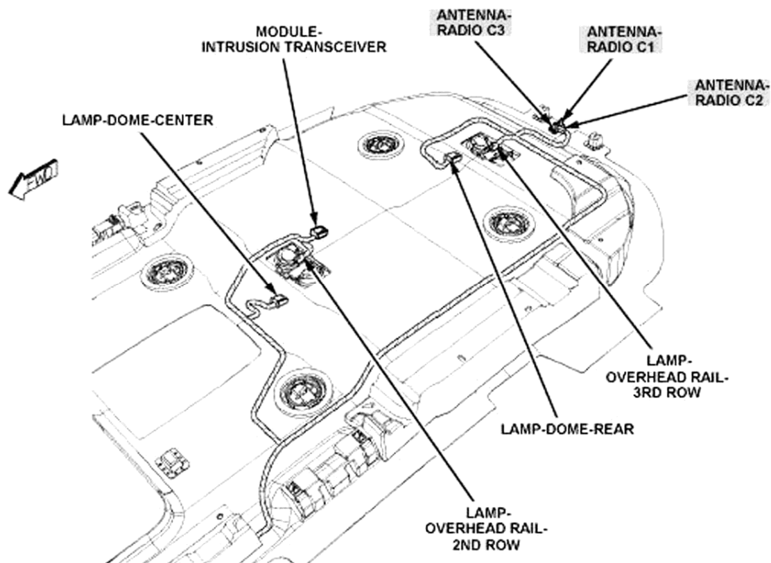
Fig. 12: Overhead Rail
