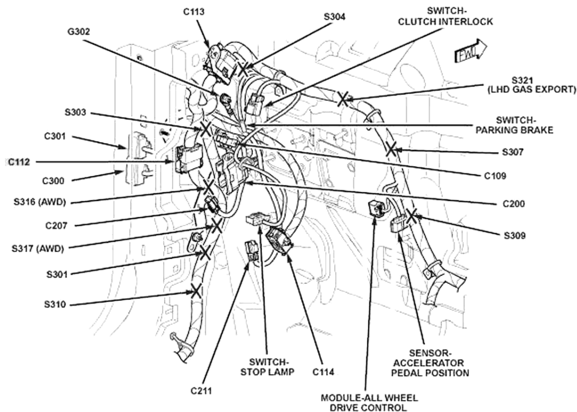
Fig. 54: Left Side Of Dash & Kick Panel
