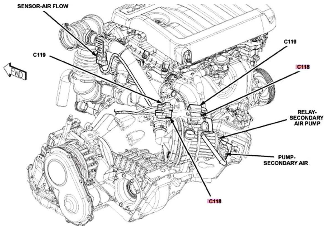
Fig. 23: Right Side Of Engine (2.4L) Courtesy of CHRYSLER LLC
