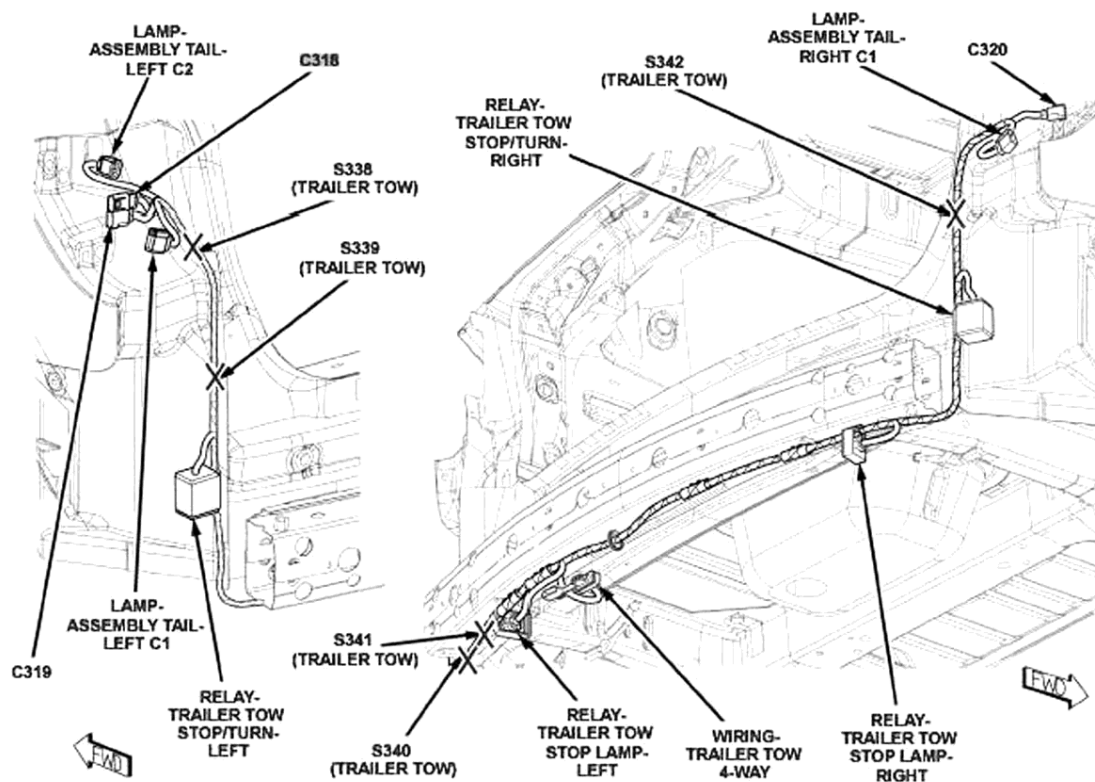
Fig. 39: Rear Of Vehicle Courtesy of CHRYSLER LLC
