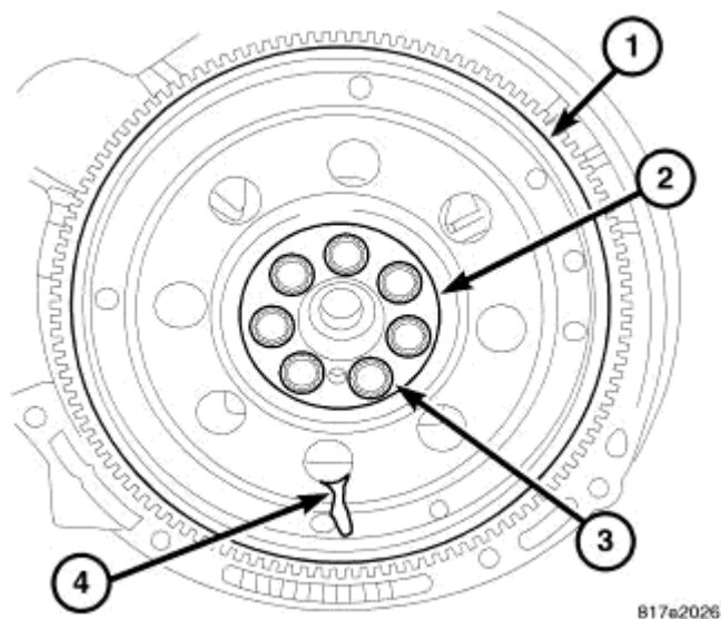
Fig. 230: FLEX PLATE Courtesy of CHRYSLER LLC
