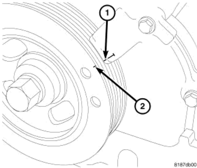
Fig. 345: Top Dead Center Courtesy of CHRYSLER LLC
