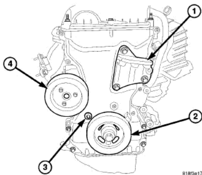
Fig. 368: Right Side Engine Mount Bracket Bolt Courtesy of CHRYSLER LLC
