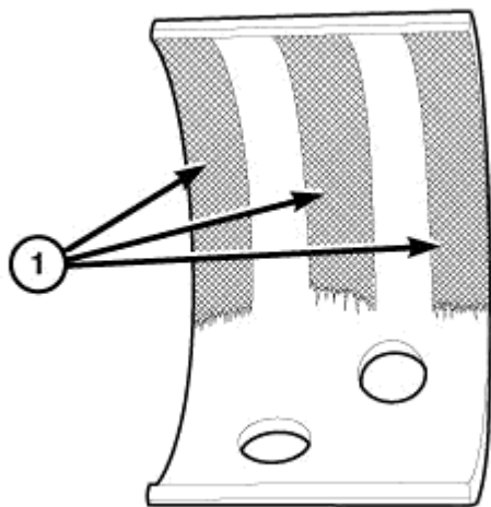
Fig. 123: Camshaft Bearing Caps Courtesy of CHRYSLER LLC
