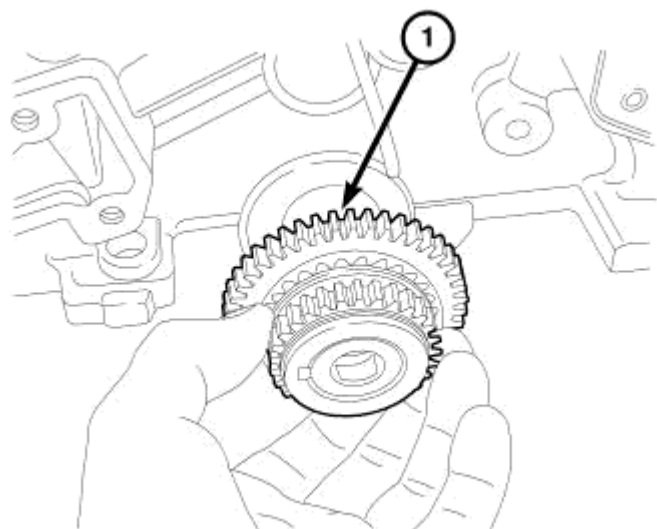
Fig. 192: CRANKSHAFT SPROCKET Courtesy of CHRYSLER LLC
