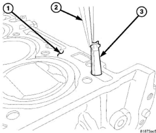
Fig. 89: Variable Valve Timing Filter Screen Courtesy of CHRYSLER LLC
