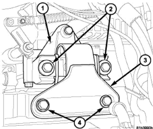
Fig. 235: LEFT MOUNT Courtesy of CHRYSLER LLC
