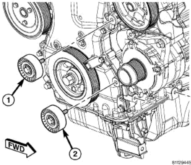
Fig. 381: Accessory Drive Belt Idler Pulley Courtesy of CHRYSLER LLC
