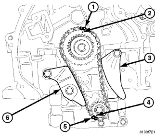
Fig. 305: Balance Shaft Module Timing Courtesy of CHRYSLER LLC
