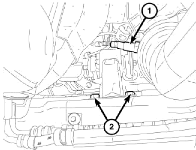
Fig. 252: Rear Mount Retaining Bolts & Oxygen Sensor Courtesy of CHRYSLER LLC
