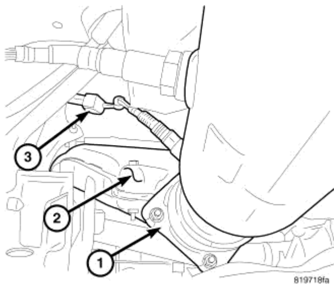
Fig. 327: Catalytic Converter At Exhaust Manifold Courtesy of CHRYSLER LLC
