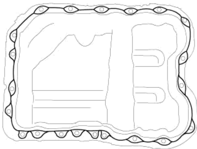
Fig. 293: SEALING OIL PAN Courtesy of CHRYSLER LLC
