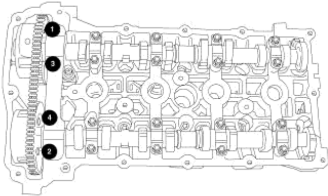
Fig. 102: Front Camshaft Cap Torque Sequence
