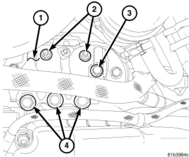
Fig. 362: Right Engine Mount Bracket Retaining Bolts
