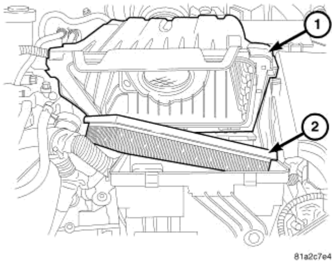
Fig. 56: AIR FILTER ELEMENT
