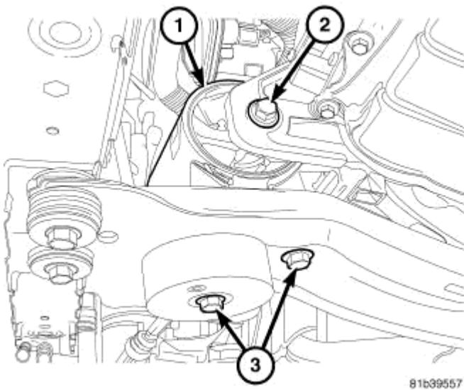
Fig. 245: FRONT MOUNT
