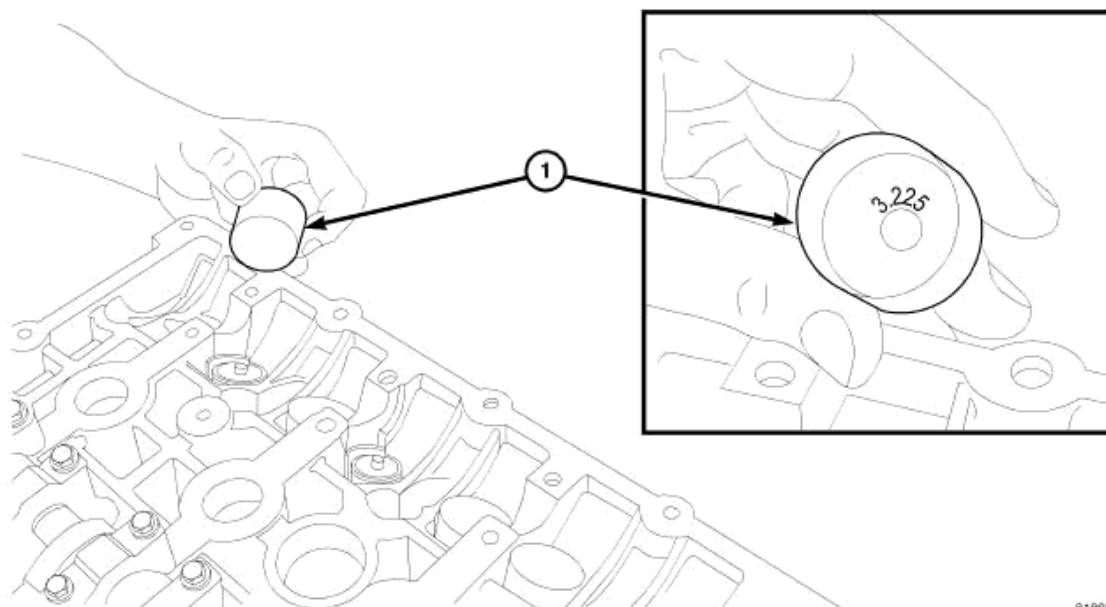
Fig. 120: TAPPET IDENTIFICATION Courtesy of CHRYSLER LLC
