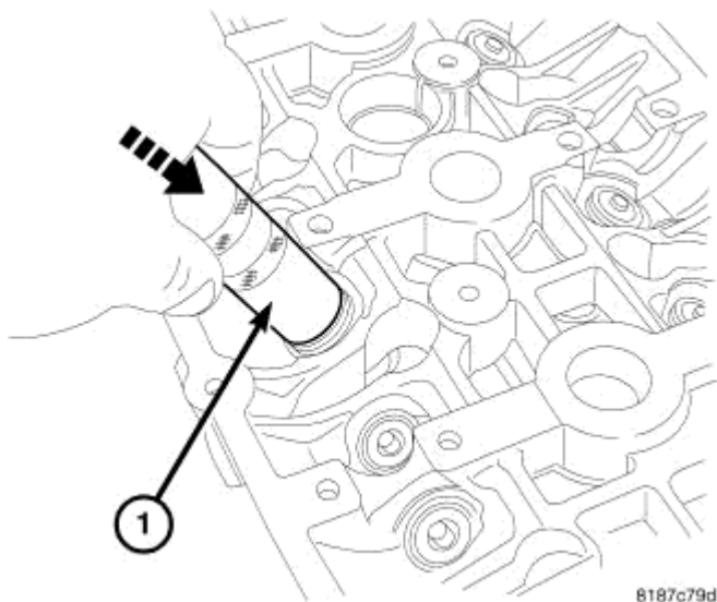
Fig. 159: VALVE REMOVAL
