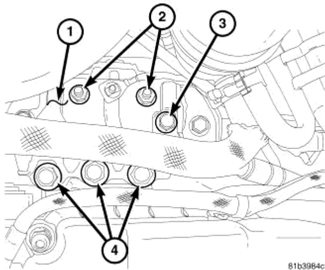
Fig. 241: Power Steering Line Support Bracket Courtesy of CHRYSLER LLC
