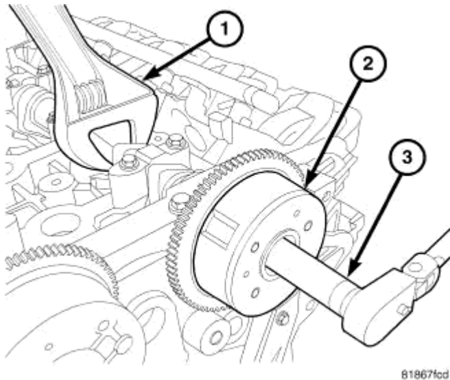
Fig. 355: Camshaft Phaser Installation Courtesy of CHRYSLER LLC
