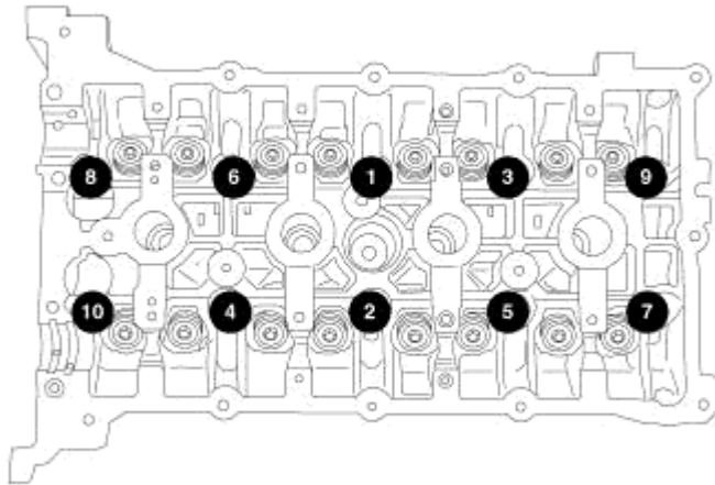
Fig. 95: CYLINDER HEAD TORQUE SEQUENCE
