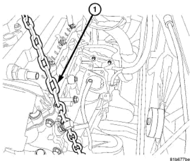
Fig. 212: LIFT CHAIN
