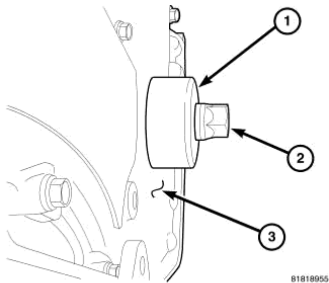
Fig. 225: FRONT SEAL INSTALLED Courtesy of CHRYSLER LLC
