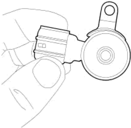
Fig. 275: SOLENOID MOUNTING TAB 1/2 Courtesy of CHRYSLER LLC
