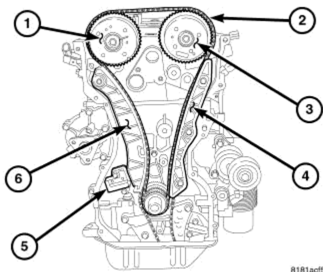
Fig. 348: Timing Drive
