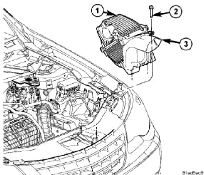
Fig. 331: Air Cleaner Housing Courtesy of CHRYSLER LLC
