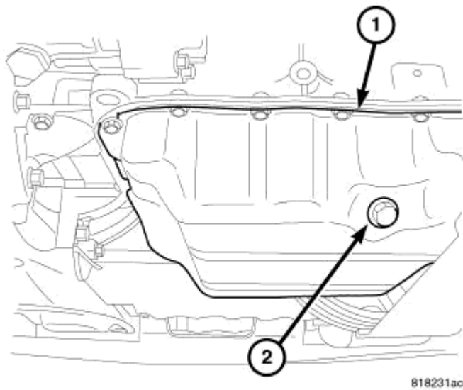
Fig. 287: OIL DRAIN PLUG Courtesy of CHRYSLER LLC
