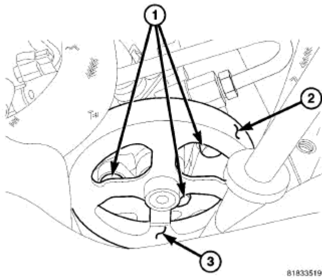
Fig. 388: POWER STEERING PUMP - GAS Courtesy of CHRYSLER LLC
