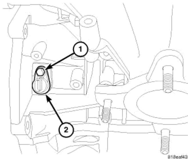
Fig. 191: CRANKSHAFT POSITION SENSOR Courtesy of CHRYSLER LLC
