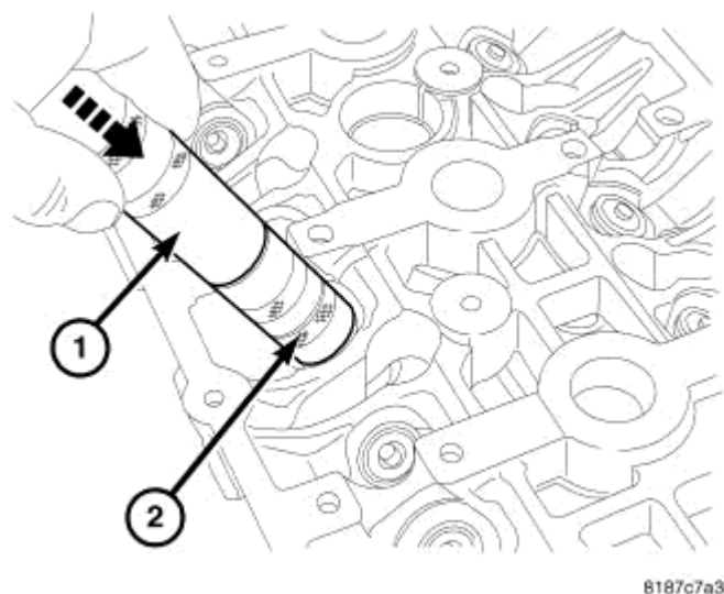
Fig. 164: VALVE INSTALLATION Courtesy of CHRYSLER LLC
