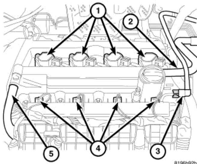
Fig. 9: Coil Connector Courtesy of CHRYSLER LLC
