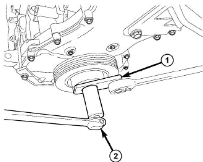
Fig. 226: Damper Removal Courtesy of CHRYSLER LLC
