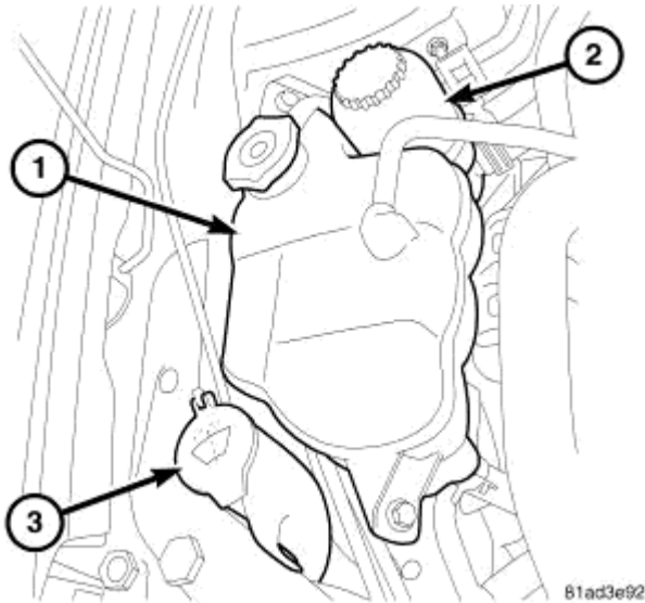
Fig. 361: COOLANT RESERVOIR
