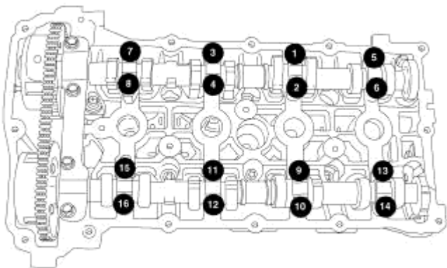
Fig. 101: Camshaft Cap Torque Sequence
