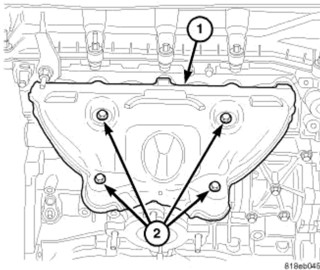
Fig. 320: EXHAUST MANIFOLD HEAT SHIELD Courtesy of CHRYSLER LLC
