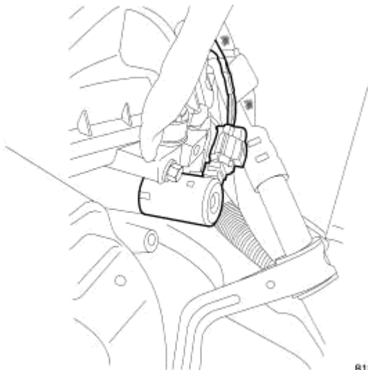
Fig. 276: SOLENOID LOCATION 1/2 Courtesy of CHRYSLER LLC
