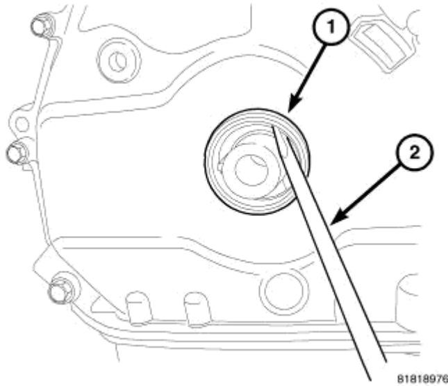
Fig. 222: FRONT CRANKSHAFT SEAL REMOVAL Courtesy of CHRYSLER LLC
