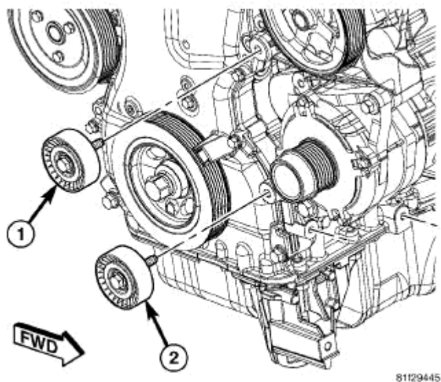
Fig. 371: Accessory Drive Belt Idler Pulley Courtesy of CHRYSLER LLC
