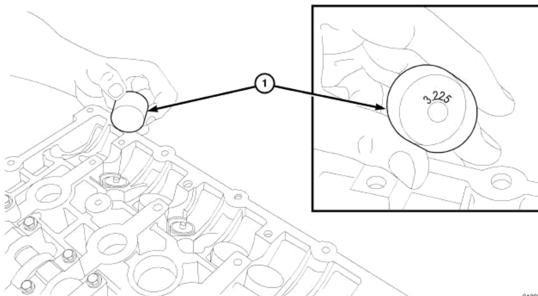
Fig. 117: TAPPET IDENTIFICATION
