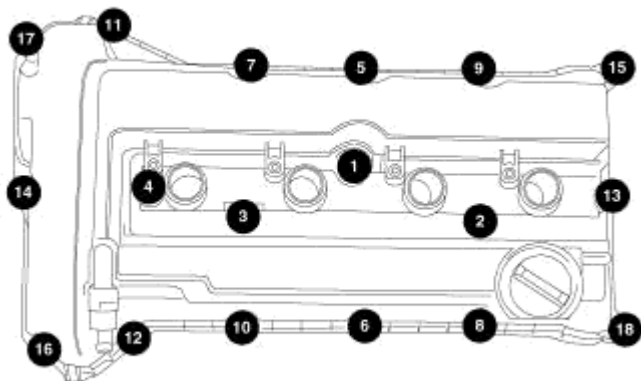
Fig. 115: Cylinder Head Cover Torque Sequence Courtesy of CHRYSLER LLC
