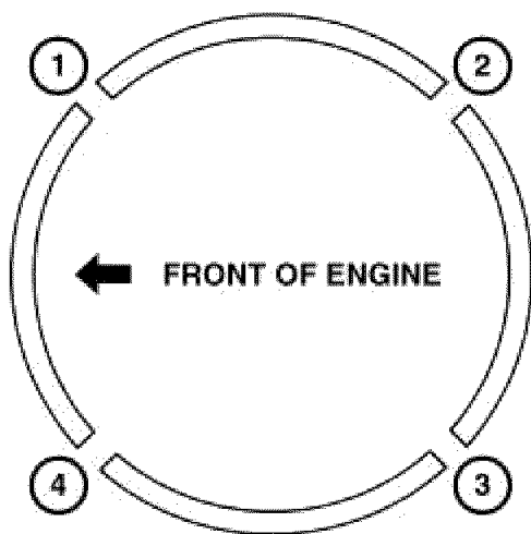
Fig. 208: Piston Ring End Gap Position Courtesy of CHRYSLER LLC
