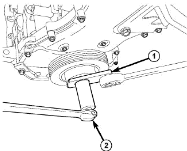
Fig. 197: DAMPER REMOVAL
