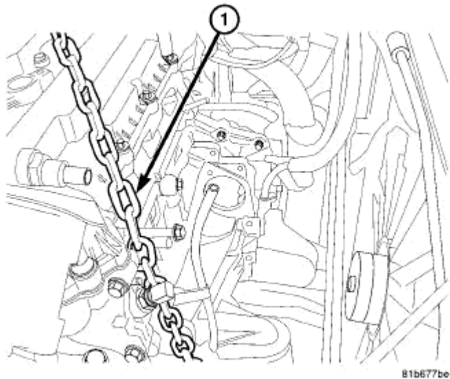
Fig. 220: LIFT CHAIN Courtesy of CHRYSLER LLC
