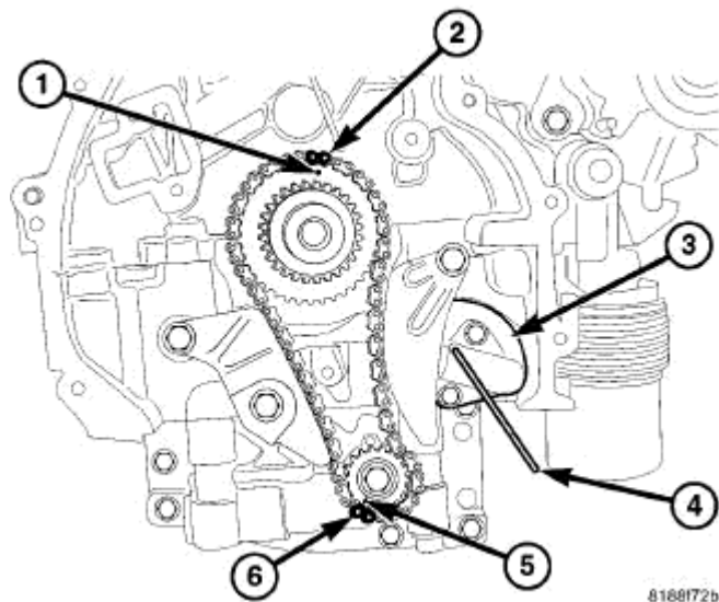
Fig. 302: Balance Shaft Module Tensioner Courtesy of CHRYSLER LLC
