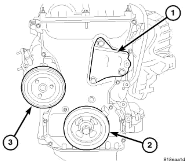
Fig. 193: RIGHT ENGINE MOUNT BRACKET Courtesy of CHRYSLER LLC
