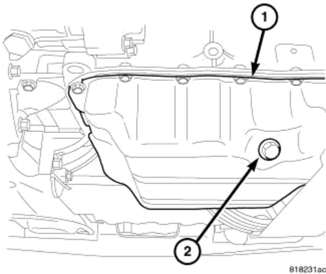
Fig. 294: OIL DRAIN PLUG Courtesy of CHRYSLER LLC
