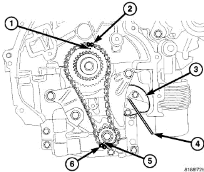
Fig. 354: Balance Shaft Module Tensioner Courtesy of CHRYSLER LLC
