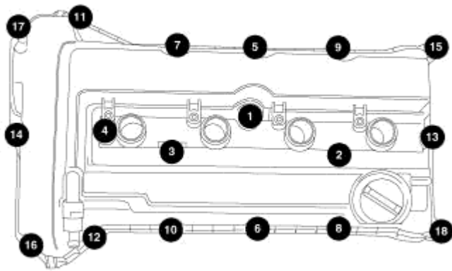
Fig. 156: Cylinder Head Cover Torque Sequence
