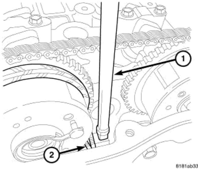
Fig. 131: SEATING WEDGE TOOL Courtesy of CHRYSLER LLC
