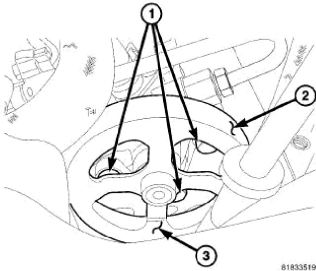
Fig. 64: POWER STEERING PUMP - GAS Courtesy of CHRYSLER LLC
