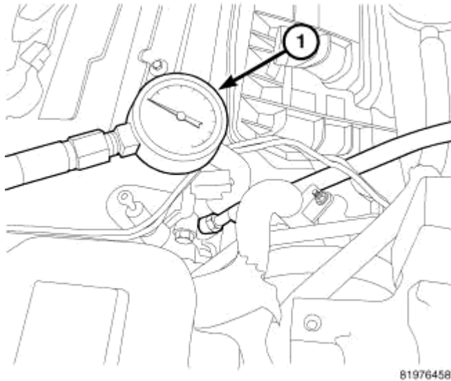
Fig. 259: OIL PSI GAUGE Courtesy of CHRYSLER LLC
