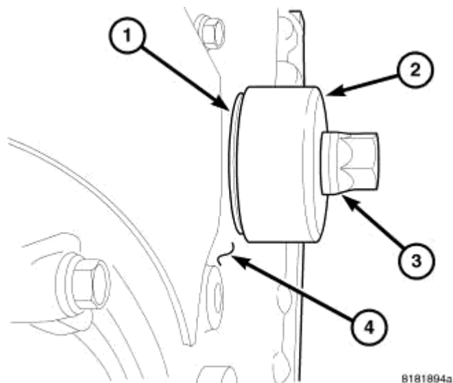
Fig. 224: INSTALLING FRONT SEAL Courtesy of CHRYSLER LLC
