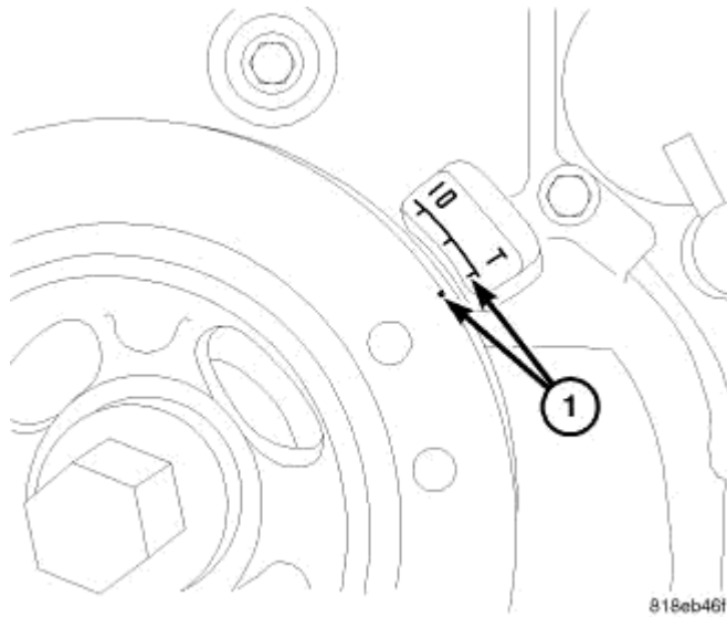
Fig. 365: Top Dead Center Courtesy of CHRYSLER LLC
