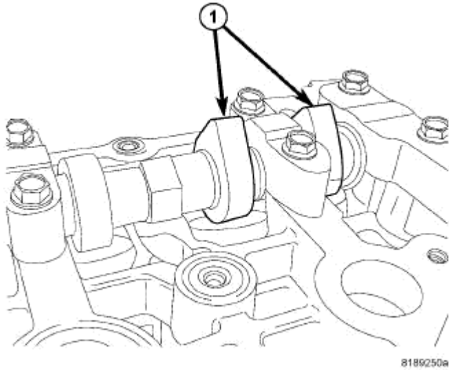
Fig. 116: LOBES VERTICAL Courtesy of CHRYSLER LLC
