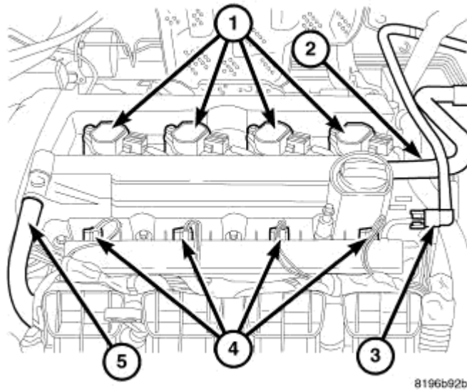
Fig. 151: COIL CONNECTOR
