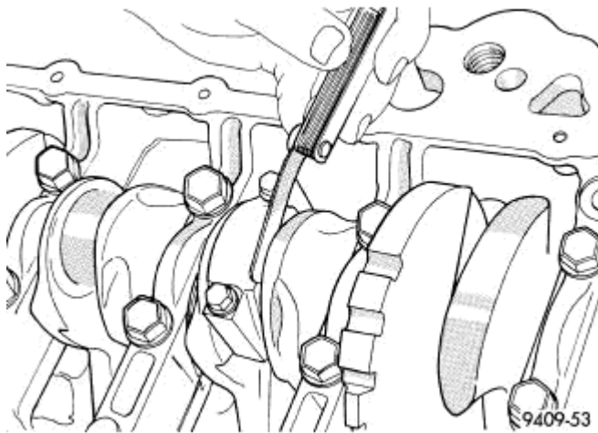
Fig. 171: Connecting Rod Side Clearance Courtesy of CHRYSLER LLC
