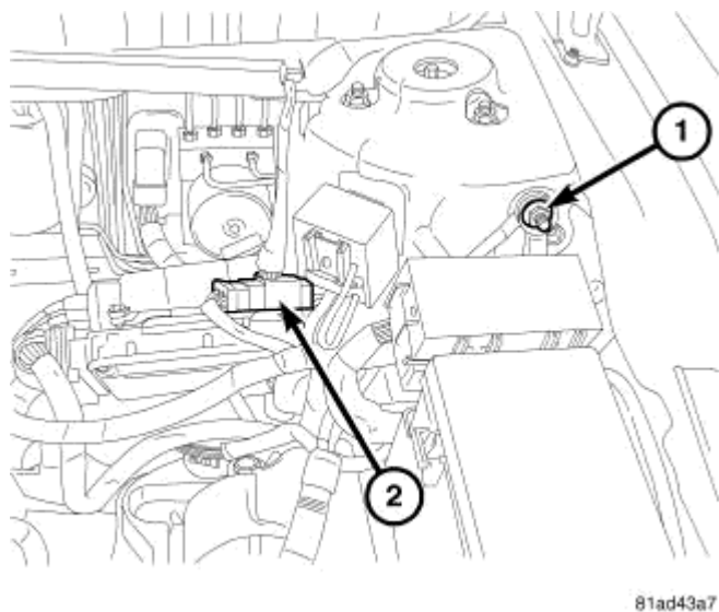
Fig. 332: BATTERY CABLE Courtesy of CHRYSLER LLC
