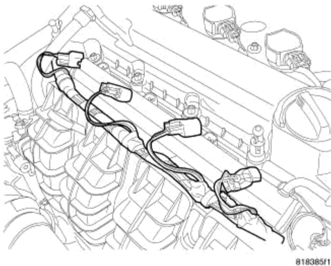
Fig. 78: Electrical Connectors From Fuel Injectors Courtesy of CHRYSLER LLC
