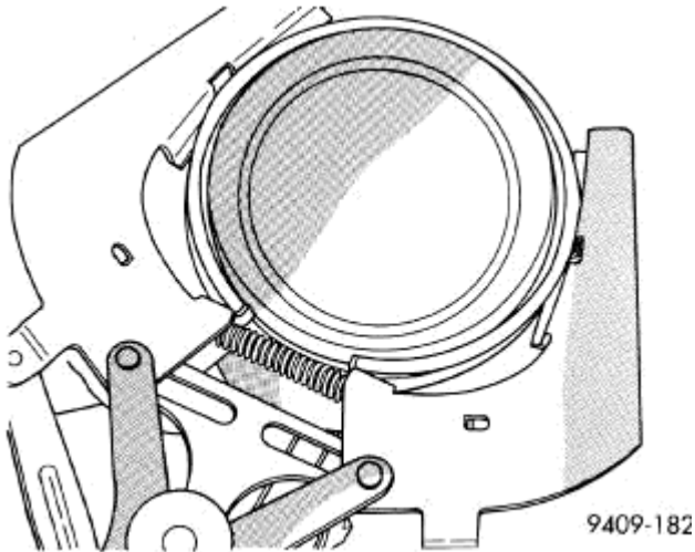
Fig. 206: Piston Rings-Removing and Installing Courtesy of CHRYSLER LLC
