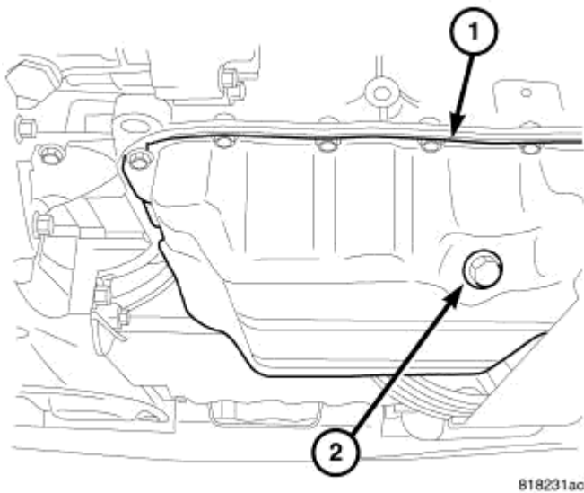
Fig. 289: OIL DRAIN PLUG Courtesy of CHRYSLER LLC
