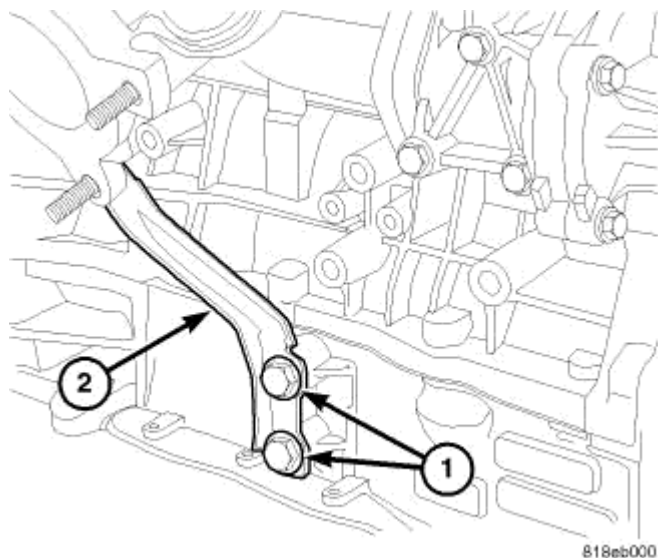
Fig. 326: EXHAUST MANIFOLD SUPPORT BRACKET Courtesy of CHRYSLER LLC
