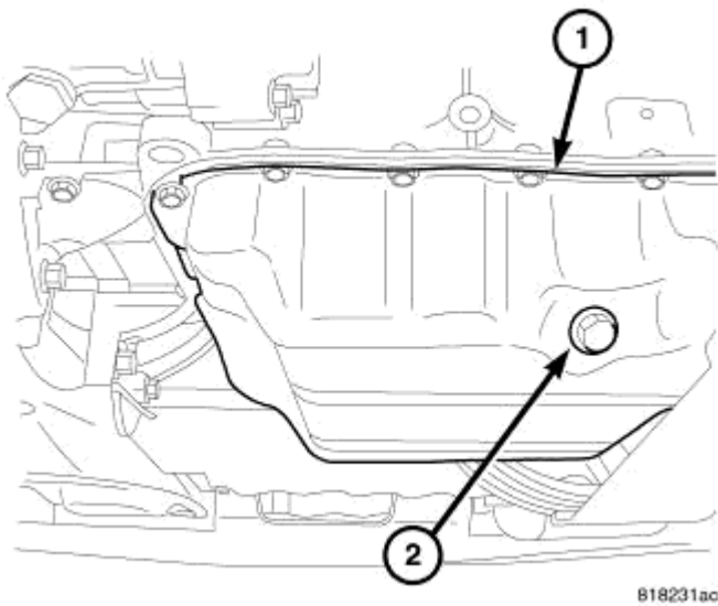
Fig. 285: OIL DRAIN PLUG Courtesy of CHRYSLER LLC
