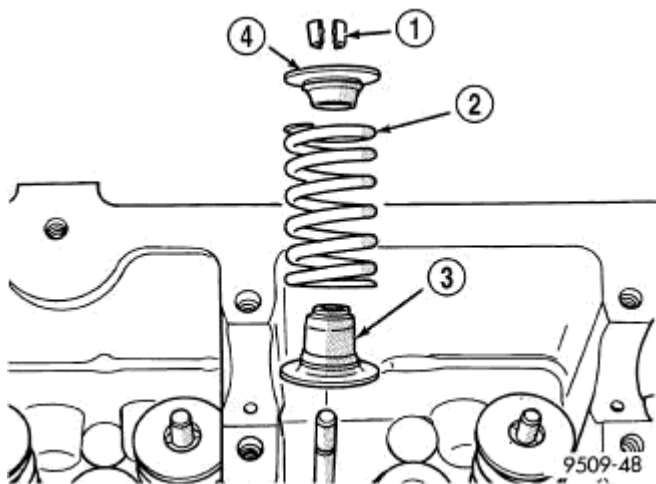
Fig. 163: Valve Spring Assembly Courtesy of CHRYSLER LLC
