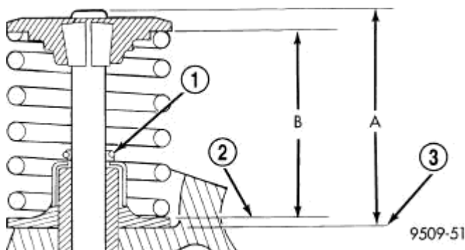
Fig. 165: Spring Installed Height and Valve Tip to Spring Seat Dimensions Courtesy of CHRYSLER LLC
