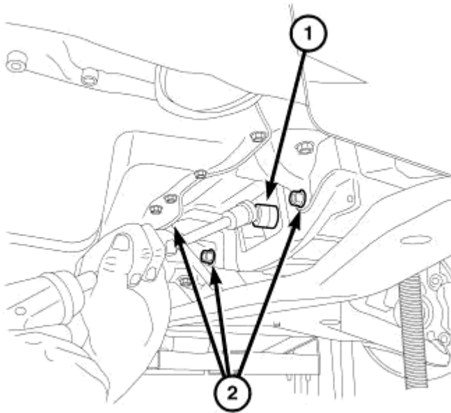
Fig. 20: MODULAR CLUTCH TO FLEX PLATE BOLTS
