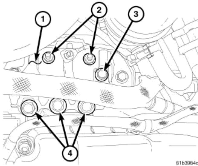
Fig. 63: Right Engine Mount Bracket Retaining Bolts Courtesy of CHRYSLER LLC
