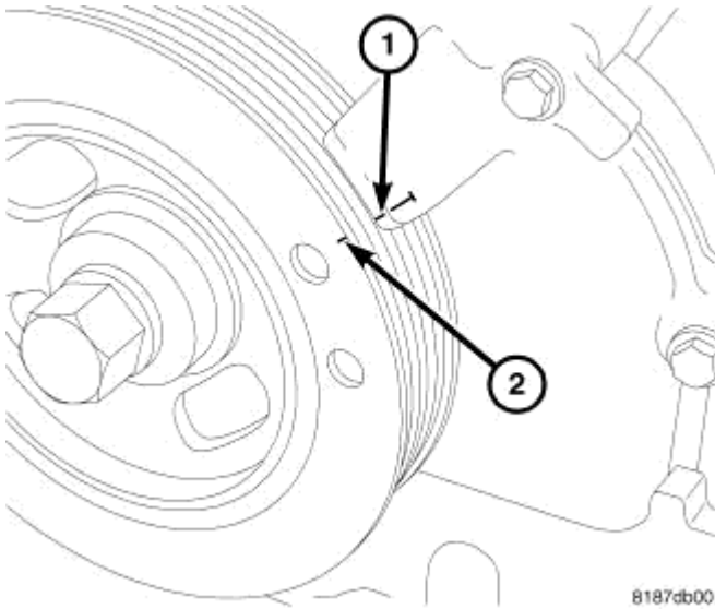
Fig. 343: Top Dead Center Courtesy of CHRYSLER LLC
