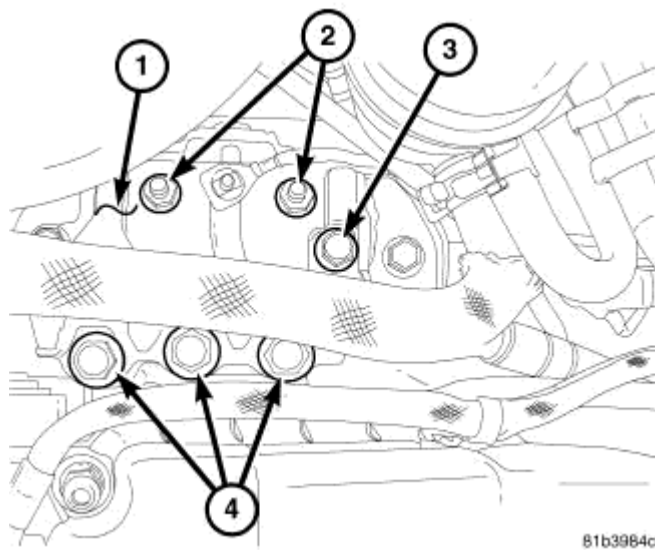
Fig. 72: Right Engine Mount Bracket Retaining Bolts Courtesy of CHRYSLER LLC
