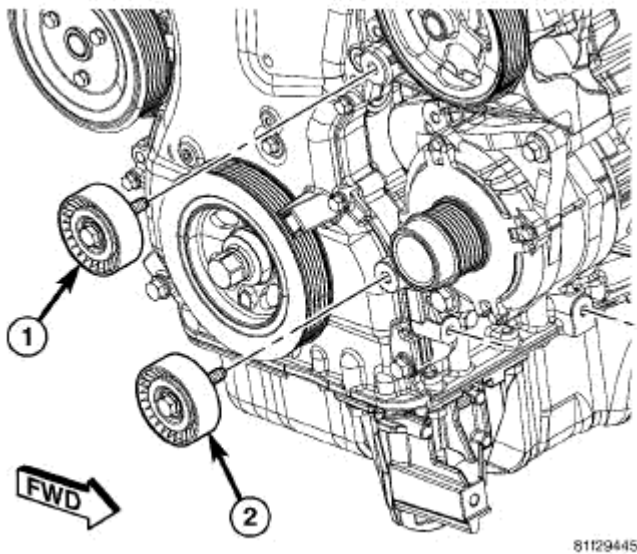
Fig. 68: Accessory Drive Belt Idler Pulley Courtesy of CHRYSLER LLC
