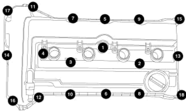
Fig. 364: Cylinder Head Cover Torque Sequence Courtesy of CHRYSLER LLC
