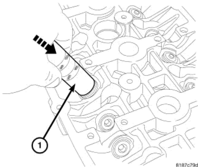
Fig. 160: VALVE REMOVAL
