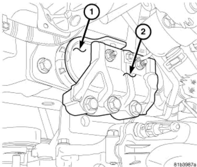
Fig. 240: Engine Mount Bracket Retaining Bolts Courtesy of CHRYSLER LLC
