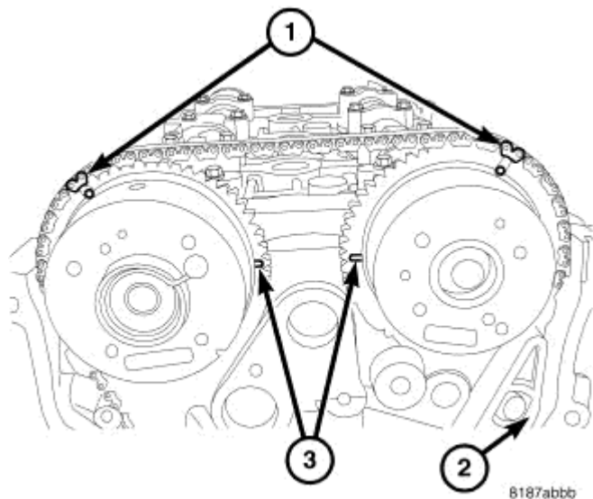
Fig. 127: TIMING CHAIN TIMING MARKS Courtesy of CHRYSLER LLC
