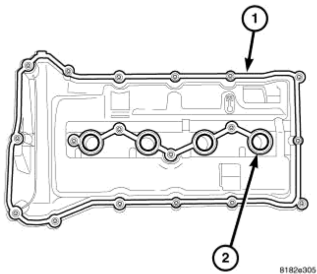
Fig. 153: GASKET LOCATION
