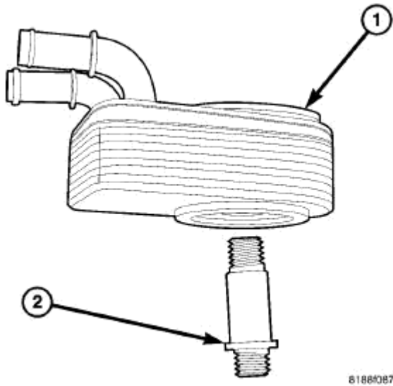
Fig. 278: OIL COOLER MOUNTING Courtesy of CHRYSLER LLC
