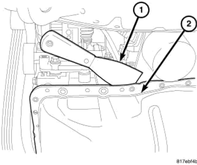
Fig. 179: OIL PAN REMOVAL Courtesy of CHRYSLER LLC
