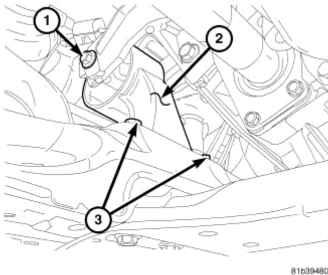
Fig. 248: Rear Mount Retaining Bolts Courtesy of CHRYSLER LLC
