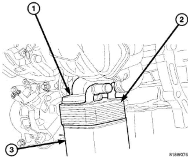
Fig. 277: OIL COOLER
