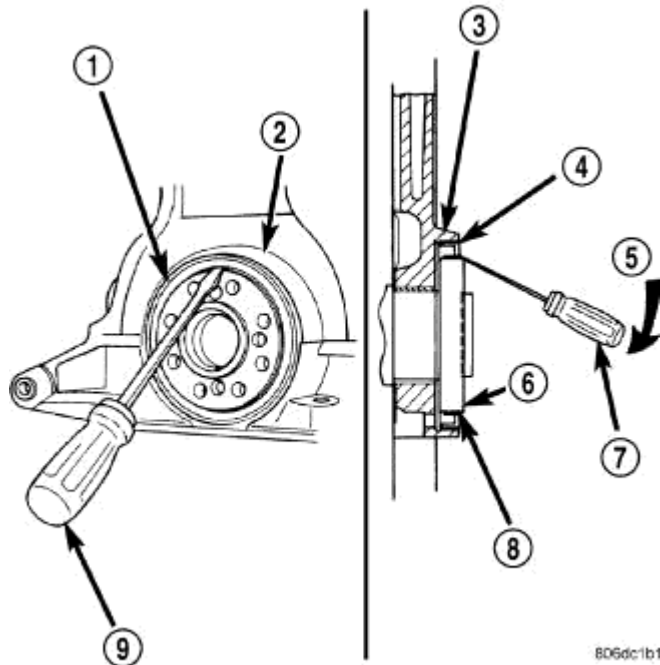
Fig. 228: Rear Crankshaft Oil Seal - Removal
