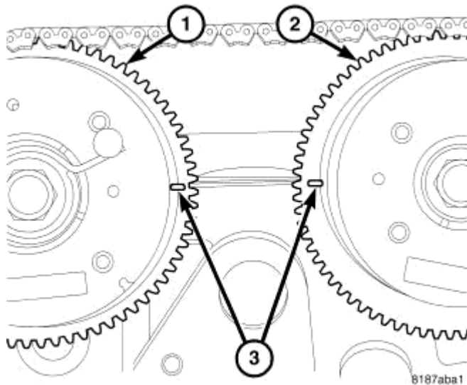
Fig. 146: Camshaft Timing Courtesy of CHRYSLER LLC
