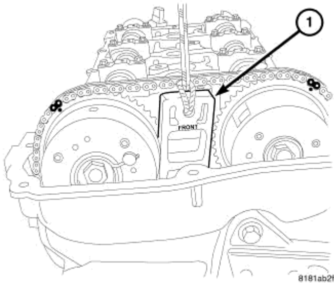
Fig. 144: WEDGE TOOL Courtesy of CHRYSLER LLC
