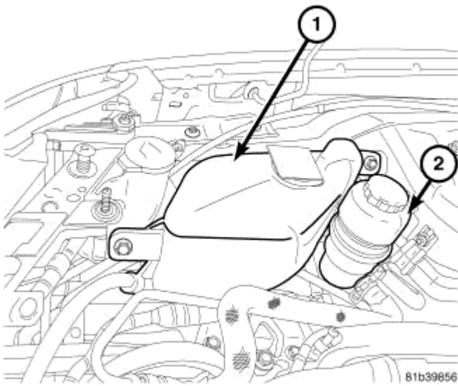
Fig. 237: COOLANT RESERVOIR Courtesy of CHRYSLER LLC
