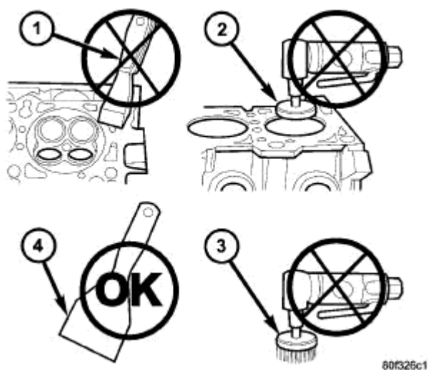
Fig. 3: PROPER TOOL USAGE FOR SURFACE PREPARATION
