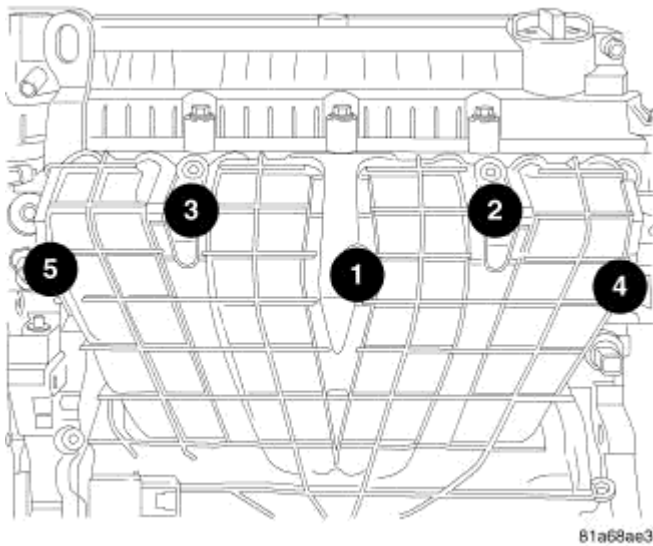
Fig. 107: INTAKE TORQUE SEQUENCE
