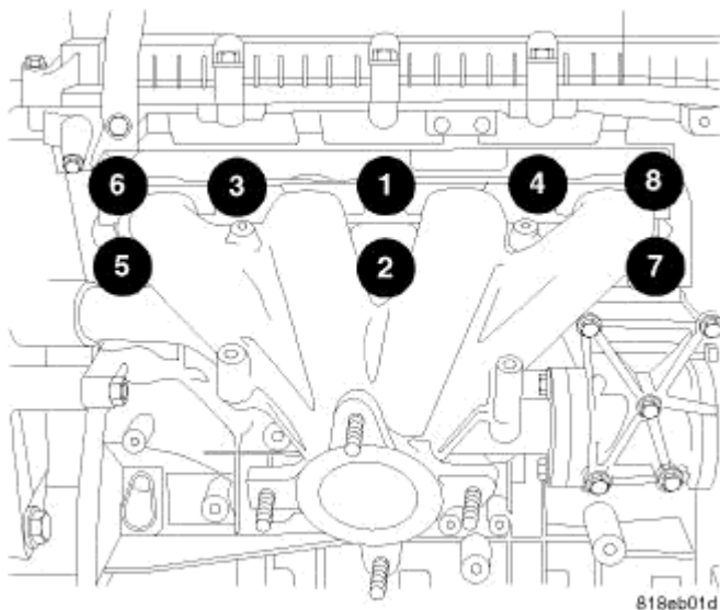
Fig. 324: Exhaust Manifold Retaining Fasteners Torque Sequence Courtesy of CHRYSLER LLC
