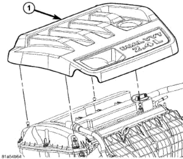
Fig. 125: Engine Cover
