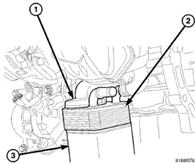
Fig. 280: OIL COOLER Courtesy of CHRYSLER LLC
