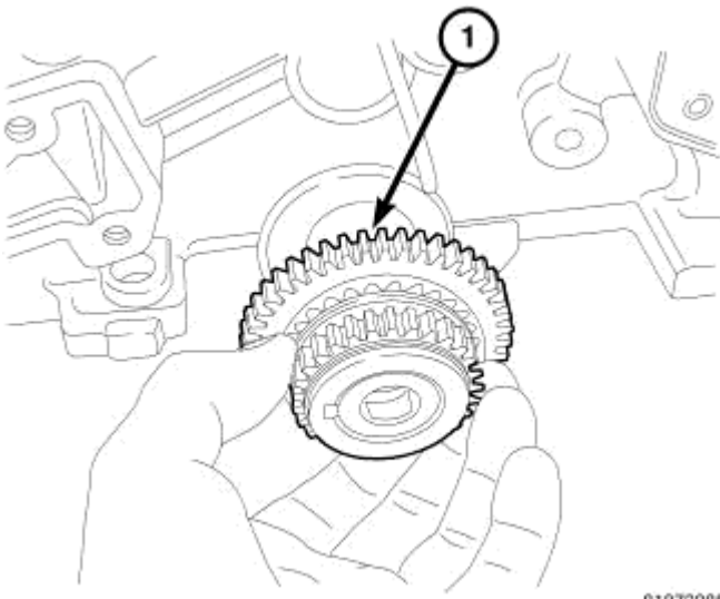
Fig. 351: CRANKSHAFT SPROCKET Courtesy of CHRYSLER LLC
