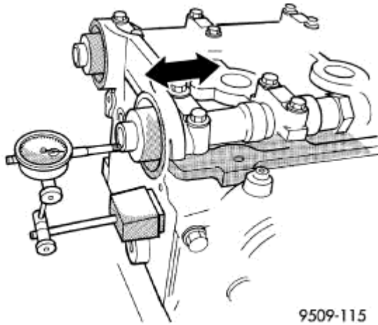
Fig. 124: Camshaft End Play Courtesy of CHRYSLER LLC
