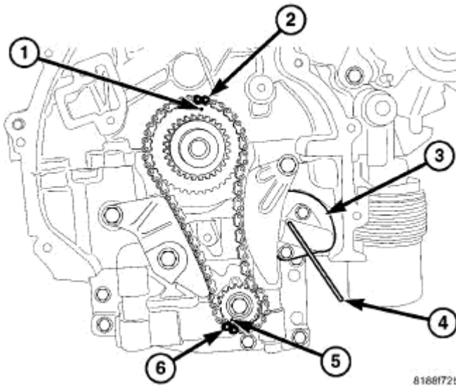
Fig. 352: Balance Shaft Module Tensioner Courtesy of CHRYSLER LLC
