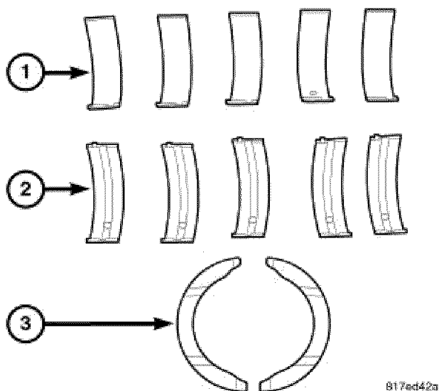
Fig. 188: BEARING IDENTIFICATION
