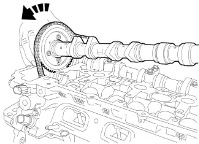
Fig. 134: ROLL CAMSHAFT Courtesy of CHRYSLER LLC
