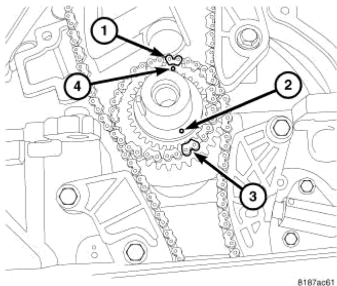
Fig. 347: Crankshaft Timing Marks Courtesy of CHRYSLER LLC
