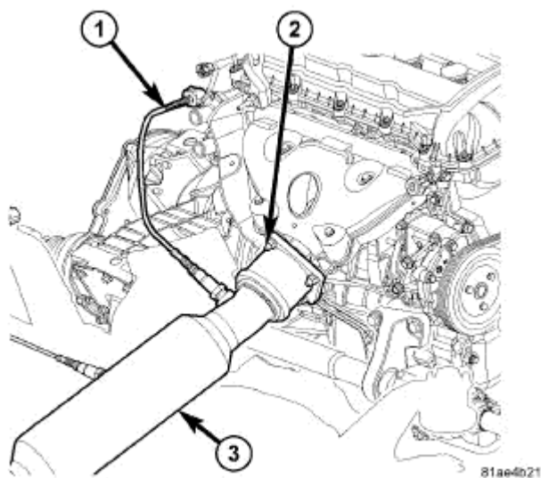
Fig. 71: Catalytic Converter Courtesy of CHRYSLER LLC
