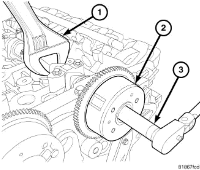
Fig. 113: Camshafts Phaser Removal/Installation Courtesy of CHRYSLER LLC
