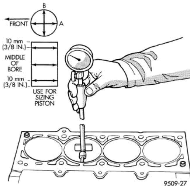
Fig. 168: Checking Cylinder Bore Size Courtesy of CHRYSLER LLC
