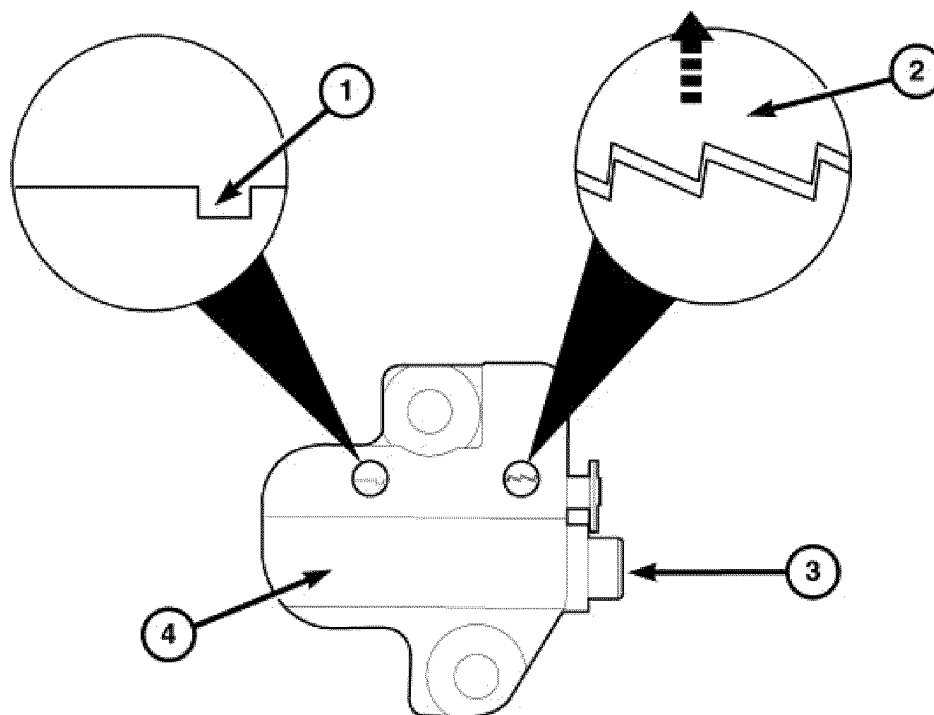
Fig. 129: TENSIONER RESET Courtesy of CHRYSLER LLC
