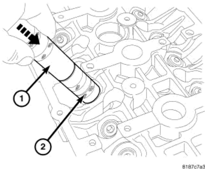
Fig. 162: VALVE INSTALLATION Courtesy of CHRYSLER LLC
