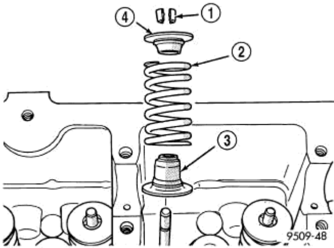
Fig. 161: Valve Spring Assembly Courtesy of CHRYSLER LLC
