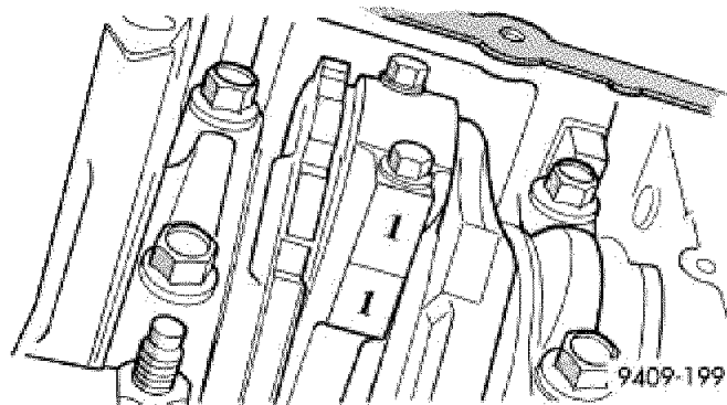
Fig. 182: Identify Connecting Rod to Cylinder-Typical Courtesy of CHRYSLER LLC
