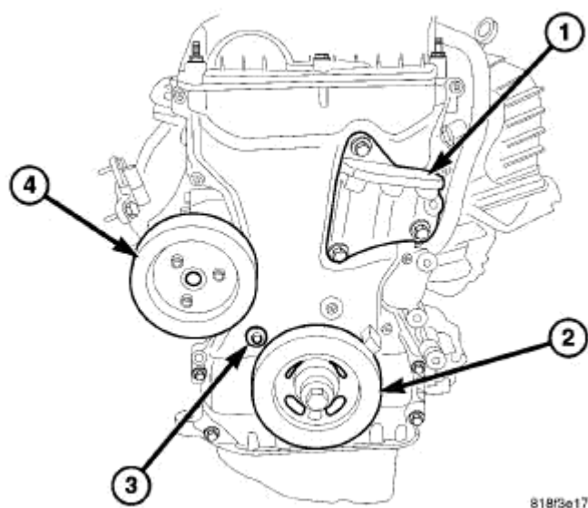
Fig. 74: Right Side Engine Mount Bracket Bolt Courtesy of CHRYSLER LLC
