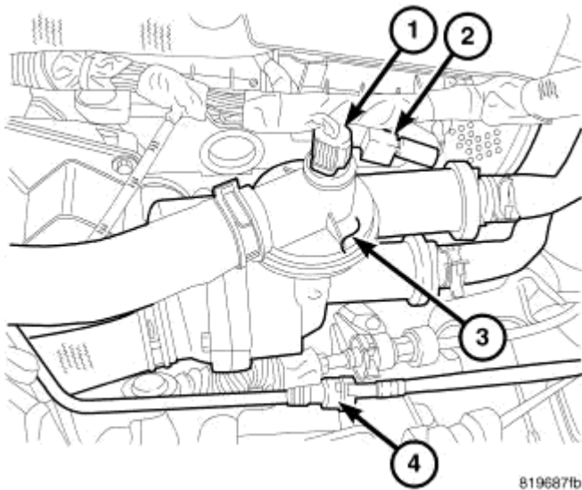
Fig. 80: COOLANT ADAPTER Courtesy of CHRYSLER LLC
