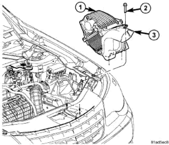
Fig. 43: Air Cleaner Housing Courtesy of CHRYSLER LLC
