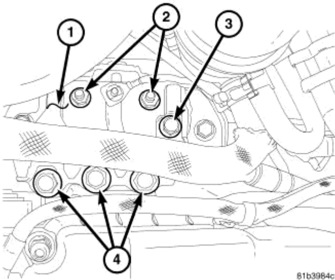
Fig. 23: Right Engine Mount Bracket Retaining Bolts Courtesy of CHRYSLER LLC
