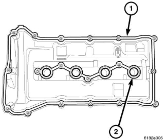
Fig. 147: GASKET LOCATION
