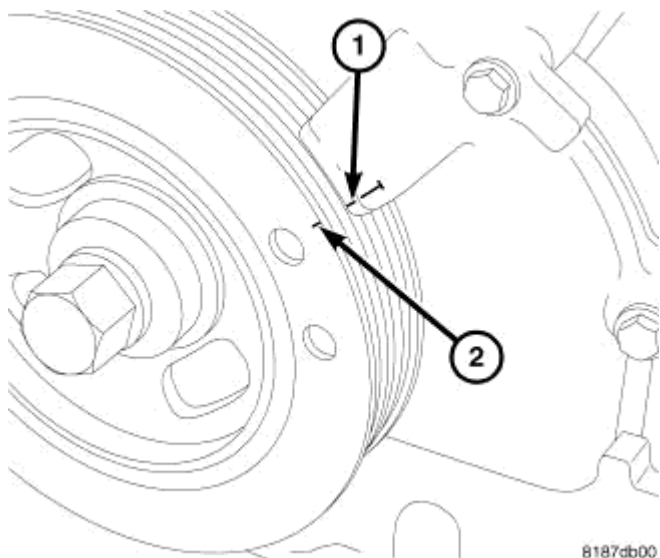
Fig. 299: Top Dead Center Courtesy of CHRYSLER LLC
