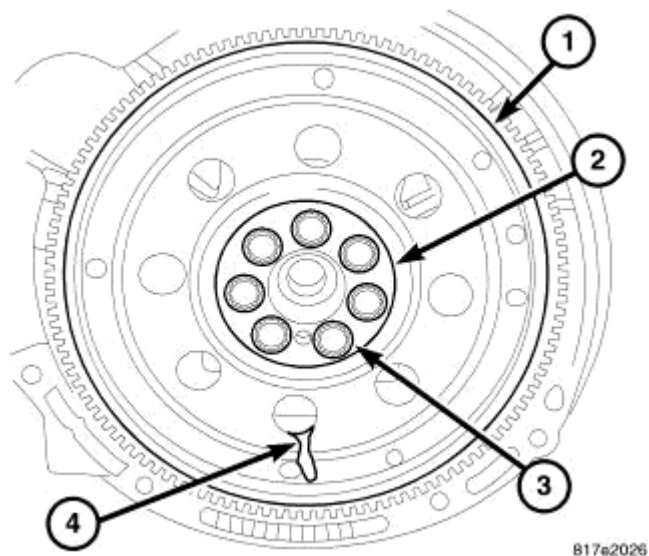
Fig. 175: FLEX PLATE Courtesy of CHRYSLER LLC
