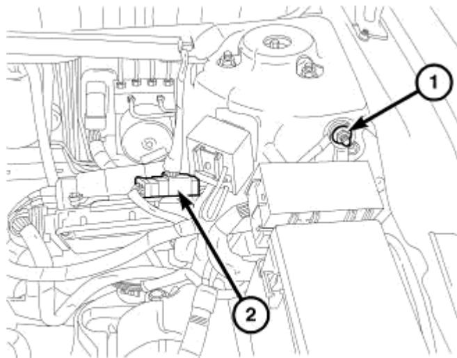
Fig. 340: BATTERY CABLE Courtesy of CHRYSLER LLC
