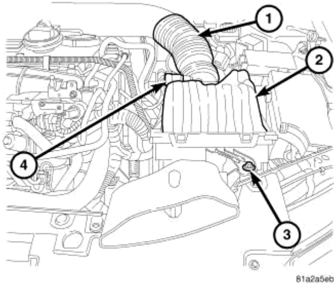
Fig. 61: Air Cleaner Housing Courtesy of CHRYSLER LLC
