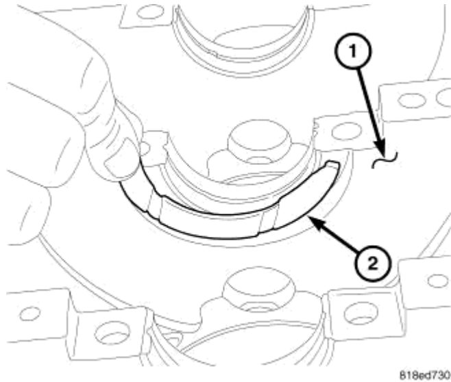
Fig. 187: INSTALLING THRUST BEARING
