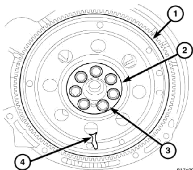
Fig. 227: FLEX PLATE
