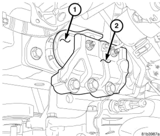
Fig. 239: Engine Mount Bracket Retaining Bolts Courtesy of CHRYSLER LLC
