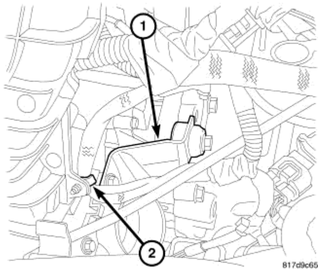
Fig. 81: Throttle Body Support Bracket Courtesy of CHRYSLER LLC
