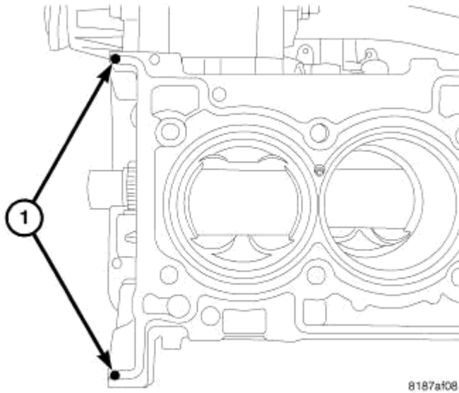
Fig. 91: Two Dots Of Mopar® Engine Sealant RTV On Cylinder Head Gasket Courtesy of CHRYSLER LLC
