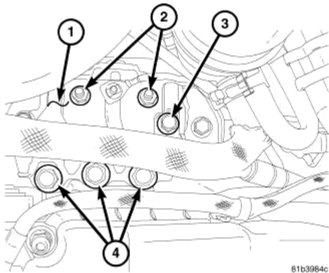
Fig. 370: Right Engine Mount Bracket Retaining Bolts Courtesy of CHRYSLER LLC
