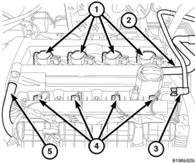
Fig. 108: COIL CONNECTOR
