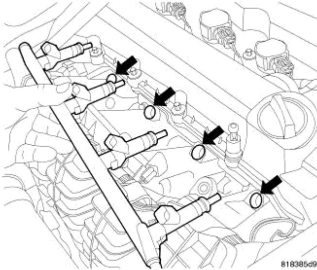
Fig. 79: RAIL REMOVAL/INSTALL Courtesy of CHRYSLER LLC
