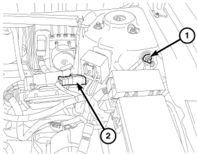
Fig. 328: BATTERY CABLE Courtesy of CHRYSLER LLC
