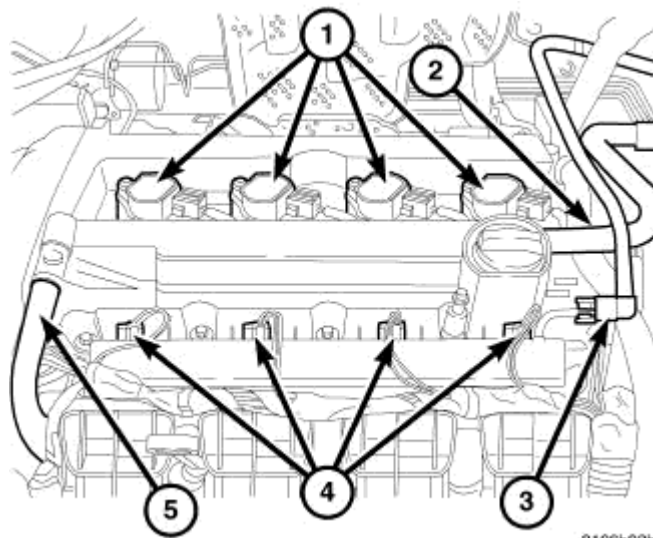
Fig. 157: Coil Connector
