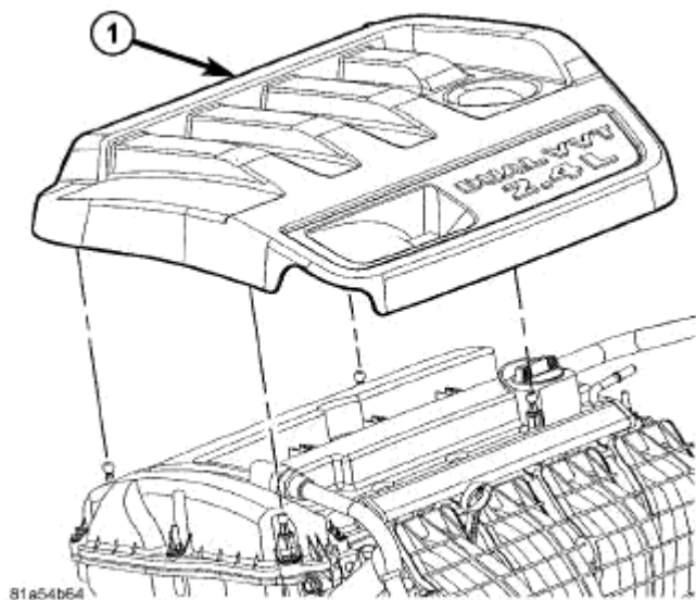
Fig. 360: Engine Cover
