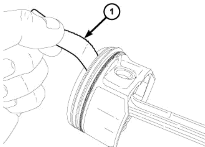
Fig. 205: Checking Piston Ring To Groove Side Clearance Courtesy of CHRYSLER LLC
