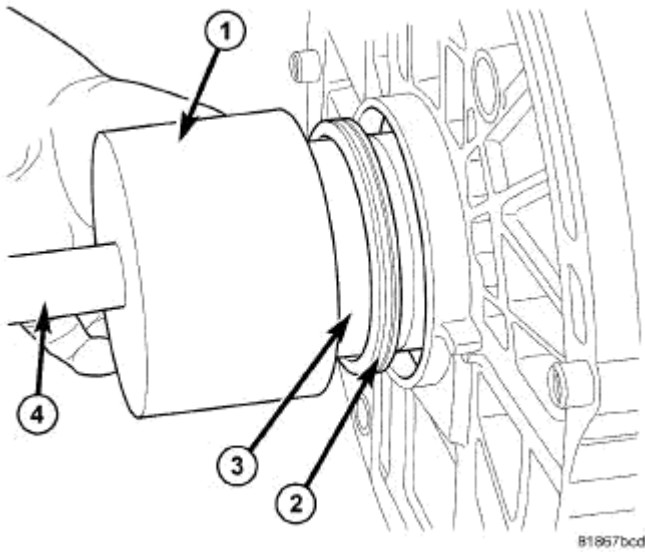
Fig. 229: REAR MAIN INSTALLATION Courtesy of CHRYSLER LLC
