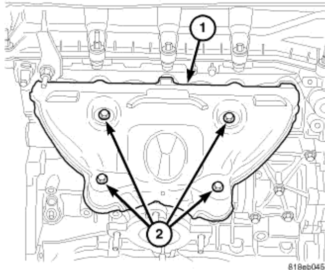
Fig. 325: EXHAUST MANIFOLD HEAT SHIELD Courtesy of CHRYSLER LLC
