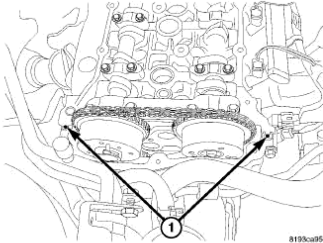
Fig. 155: Cylinder Head/Front Cover T-Joint Courtesy of CHRYSLER LLC
