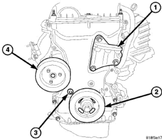
Fig. 69: Right Side Engine Mount Bracket Bolt Courtesy of CHRYSLER LLC
