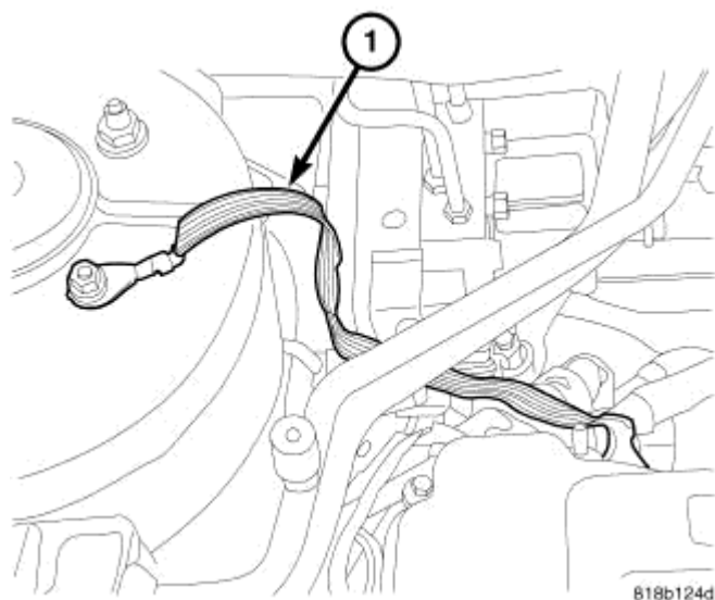
Fig. 29: GROUND STRAP Courtesy of CHRYSLER LLC
