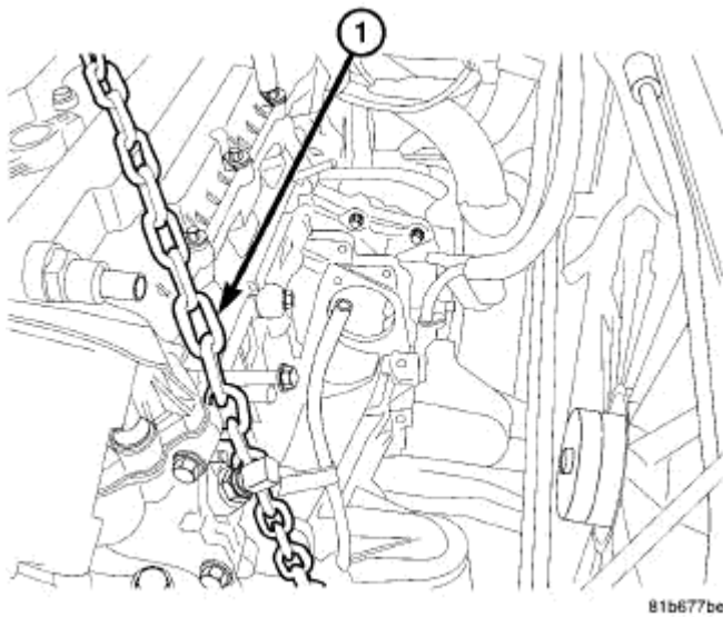
Fig. 26: LIFT CHAIN
