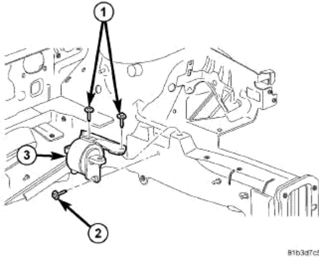
Fig. 233: Frame Rail Fastener Courtesy of CHRYSLER LLC
