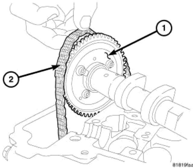
Fig. 135: CHAIN REMOVAL Courtesy of CHRYSLER LLC
