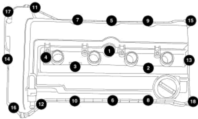
Fig. 65: Cylinder Head Cover Torque Sequence Courtesy of CHRYSLER LLC
