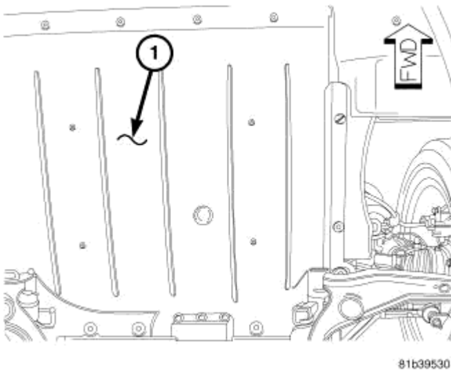
Fig. 243: LOWER SILENCER Courtesy of CHRYSLER LLC
