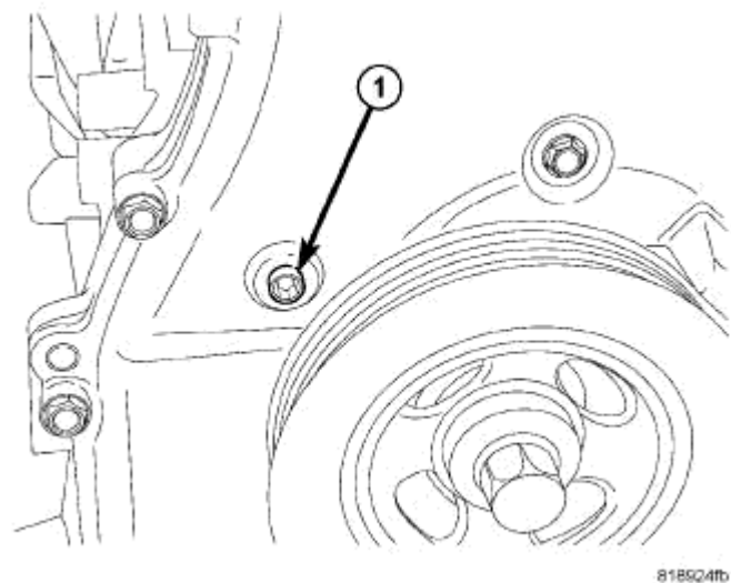
Fig. 128: TENSIONER ACCESS PLUG Courtesy of CHRYSLER LLC
