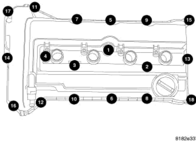
Fig. 148: Cylinder Head Cover Torque Sequence
