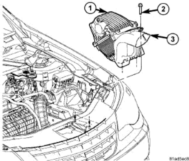
Fig. 59: Air Cleaner Housing Courtesy of CHRYSLER LLC
