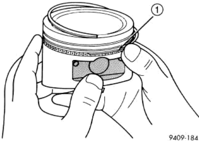
Fig. 207: Installing Side Rail Courtesy of CHRYSLER LLC
