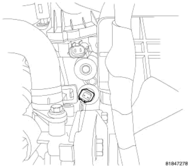
Fig. 267: OIL PRESSURE SENSOR Courtesy of CHRYSLER LLC
