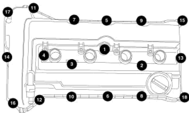
Fig. 152: Cylinder Head Cover Torque Sequence
