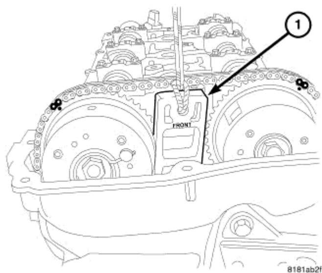
Fig. 130: WEDGE TOOL Courtesy of CHRYSLER LLC
