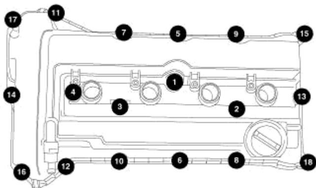
Fig. 122: Cylinder Head Cover Torque Sequence Courtesy of CHRYSLER LLC
