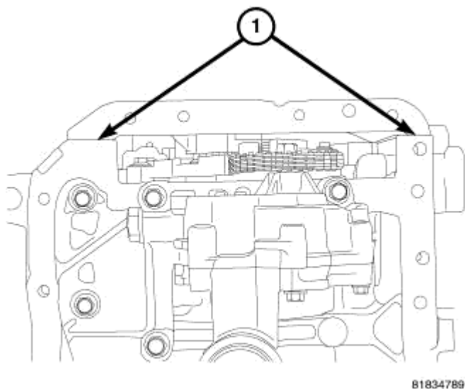
Fig. 292: SEALER LOCATION Courtesy of CHRYSLER LLC
