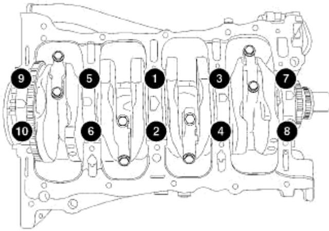
Fig. 183: MAIN BEARING CAP TORQUE SEQUENCE Courtesy of CHRYSLER LLC
