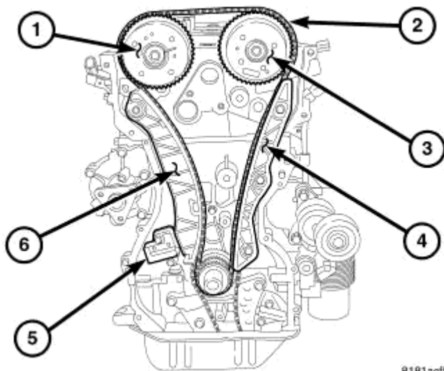
Fig. 103: TIMING DRIVE
