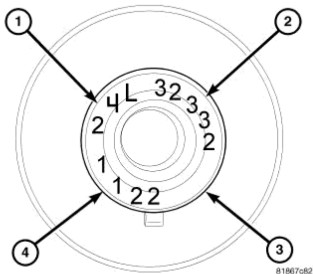
Fig. 169: BEARING SELECTION Courtesy of CHRYSLER LLC
