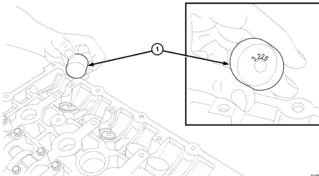
Fig. 121: TAPPET IDENTIFICATION
