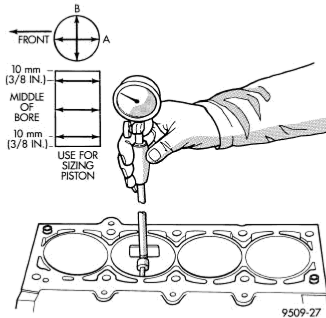
Fig. 210: Checking Cylinder Bore Size Courtesy of CHRYSLER LLC
