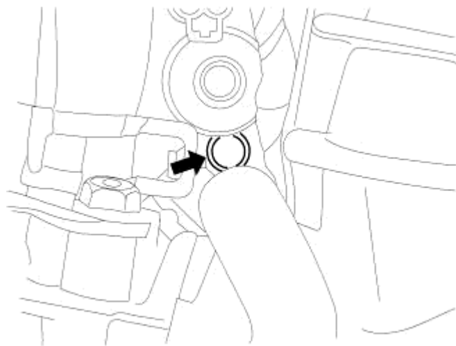
Fig. 273: SOLENOID MOUNTING BOLT Courtesy of CHRYSLER LLC
