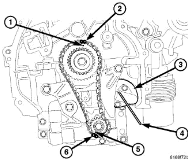
Fig. 307: Balance Shaft Module Tensioner Courtesy of CHRYSLER LLC
