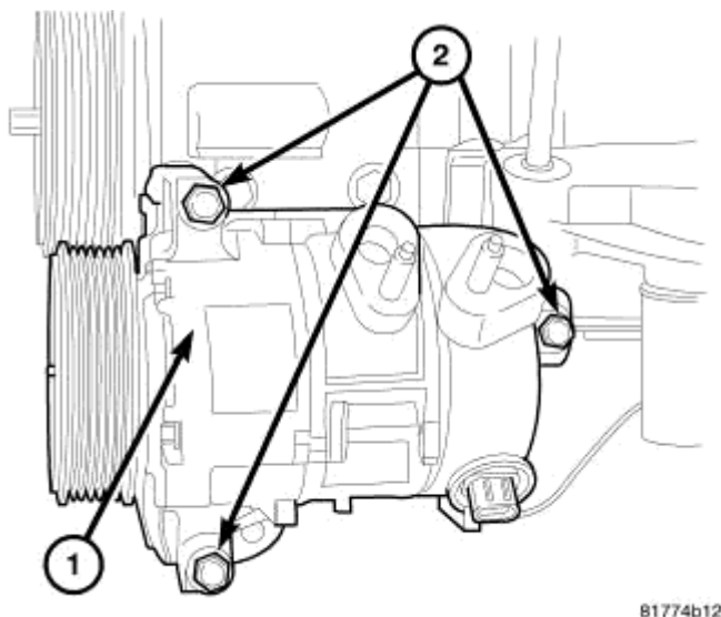
Fig. 310: A/C Compressor Removal/Installation Courtesy of CHRYSLER LLC
