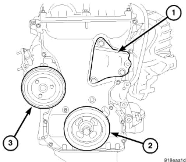
Fig. 178: RIGHT ENGINE MOUNT BRACKET Courtesy of CHRYSLER LLC
