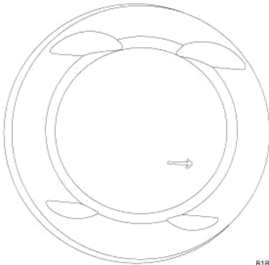
Fig. 217: PISTON INSTALLATION Courtesy of CHRYSLER LLC
