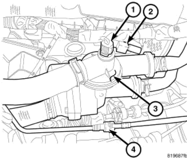
Fig. 83: COOLANT ADAPTER Courtesy of CHRYSLER LLC
