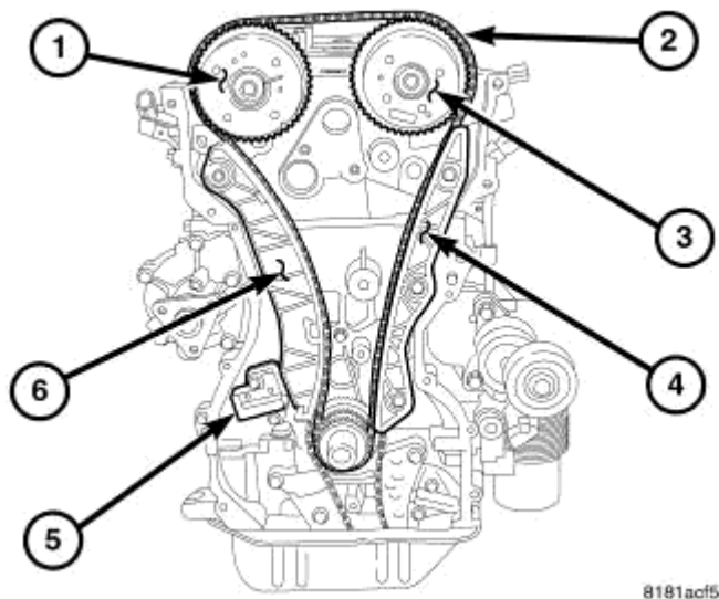
Fig. 342: TIMING DRIVE
