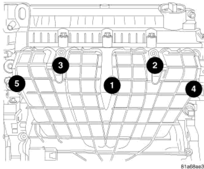
Fig. 336: Intake Manifold Retaining Bolts Torque Sequence
