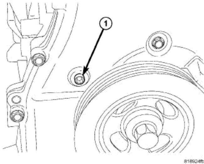
Fig. 145: TENSIONER ACCESS PLUG Courtesy of CHRYSLER LLC
