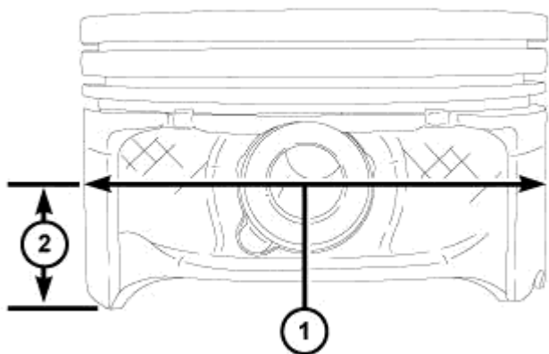
Fig. 209: Measuring Pistons & Cylinder Bores
