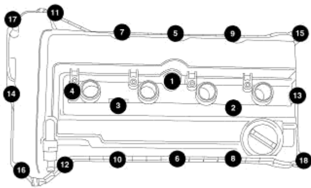
Fig. 104: Cylinder Head Cover Torque Sequence
