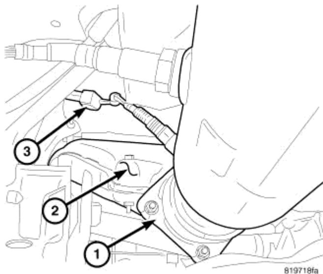
Fig. 321: Catalytic Converter At Exhaust Manifold Courtesy of CHRYSLER LLC
