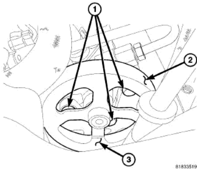
Fig. 363: POWER STEERING PUMP - GAS Courtesy of CHRYSLER LLC
