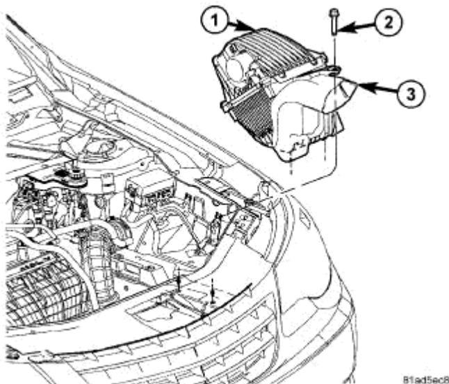
Fig. 339: Air Cleaner Housing Courtesy of CHRYSLER LLC
