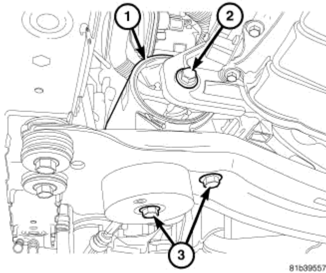
Fig. 244: FRONT MOUNT Courtesy of CHRYSLER LLC
