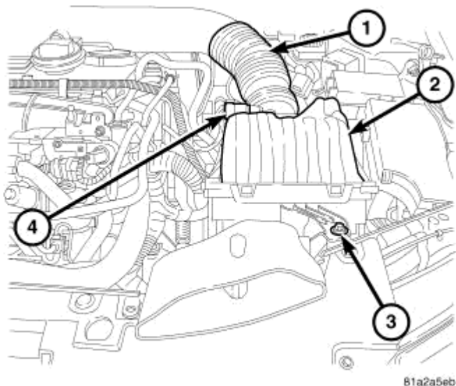
Fig. 391: Air Cleaner Housing
