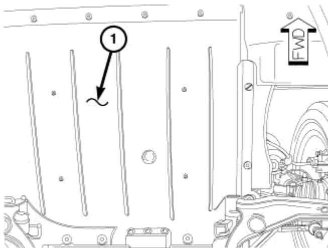
Fig. 254: LOWER SILENCER Courtesy of CHRYSLER LLC
