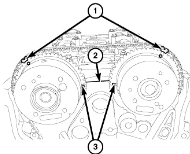
Fig. 357: Timing Chain Timing Marks
