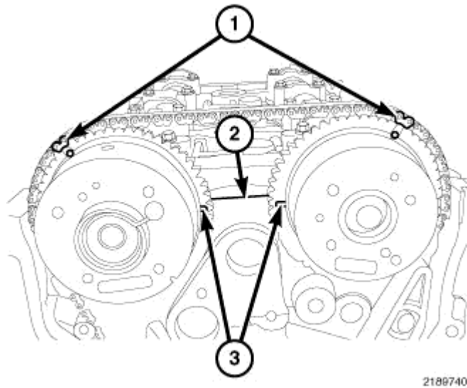
Fig. 138: Timing Chain Timing Marks Courtesy of CHRYSLER LLC
