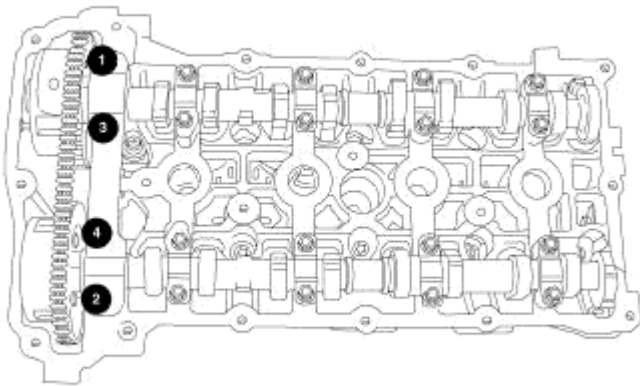
Fig. 132: Front Camshaft Cap Removal Sequence Courtesy of CHRYSLER LLC
