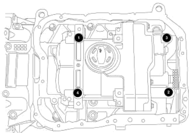
Fig. 306: Balance Shaft Module Torque Sequence Courtesy of CHRYSLER LLC
