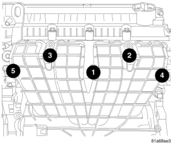
Fig. 82: Intake Manifold Retaining Bolts Torque Sequence Courtesy of CHRYSLER LLC
