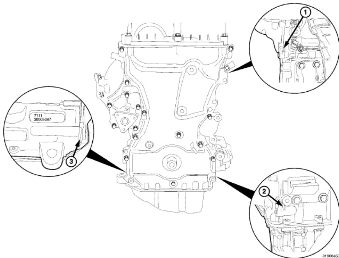
Fig. 75: TIMING CHAIN COVER PRY POINTS Courtesy of CHRYSLER LLC
