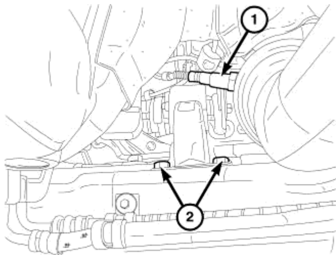
Fig. 249: Rear Mount Retaining Bolts & Oxygen Sensor Courtesy of CHRYSLER LLC
