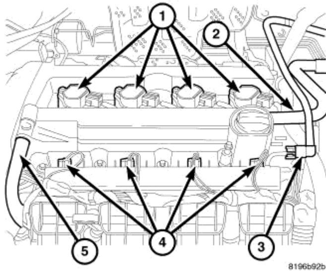
Fig. 38: COIL CONNECTOR Courtesy of CHRYSLER LLC
