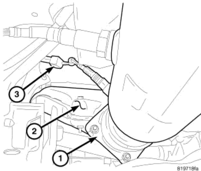
Fig. 31: Exhaust Pipe Bolts Courtesy of CHRYSLER LLC
