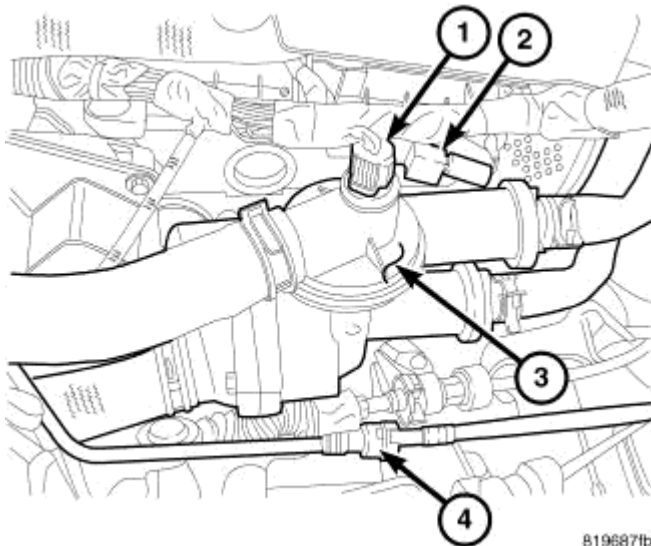
Fig. 97: COOLANT ADAPTER Courtesy of CHRYSLER LLC
