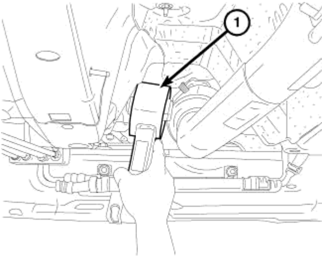
Fig. 251: Removing/Installing Rear Mount Towards Rear Of Vehicle Courtesy of CHRYSLER LLC
