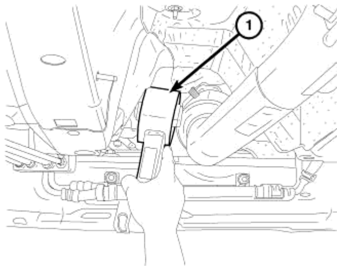
Fig. 250: Removing/Installing Rear Mount Towards Rear Of Vehicle Courtesy of CHRYSLER LLC
