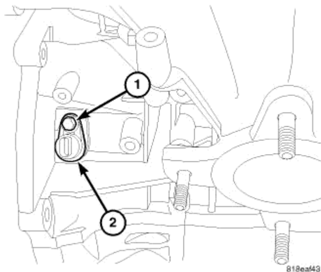
Fig. 30: CRANKSHAFT POSITION SENSOR Courtesy of CHRYSLER LLC
