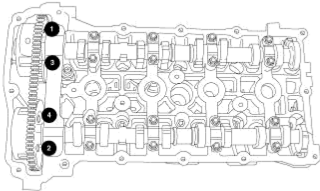
Fig. 85: Front Camshaft Cap Removal Sequence Courtesy of CHRYSLER LLC
