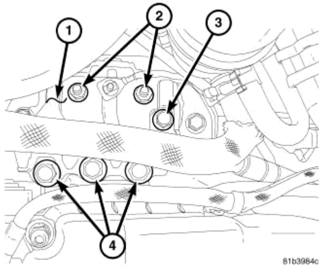
Fig. 27: Right Engine Mount Bracket Retaining Bolts Courtesy of CHRYSLER LLC
