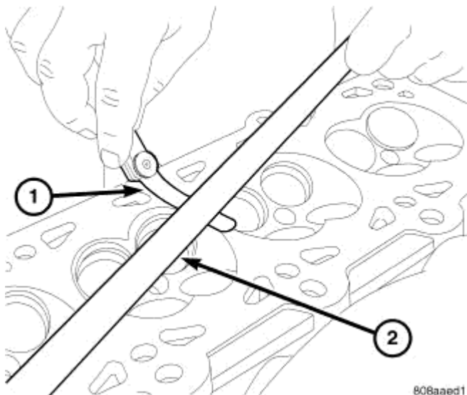
Fig. 87: Checking Cylinder Head Flatness
