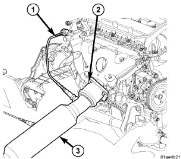
Fig. 105: Catalytic Converter Courtesy of CHRYSLER LLC
