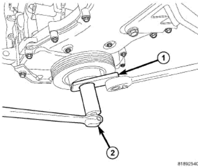
Fig. 221: Damper Removal Courtesy of CHRYSLER LLC
