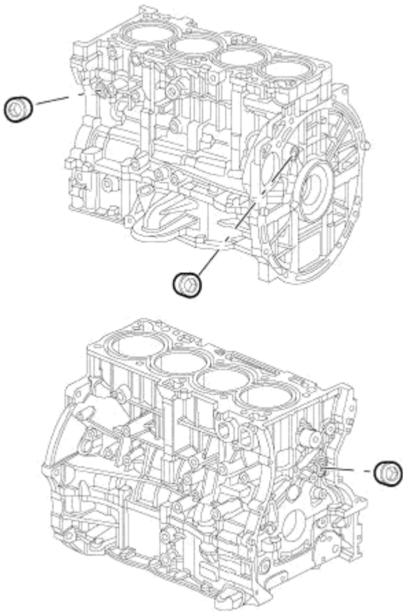
Fig. 295: Engine Block Tapered Plugs Courtesy of CHRYSLER LLC
