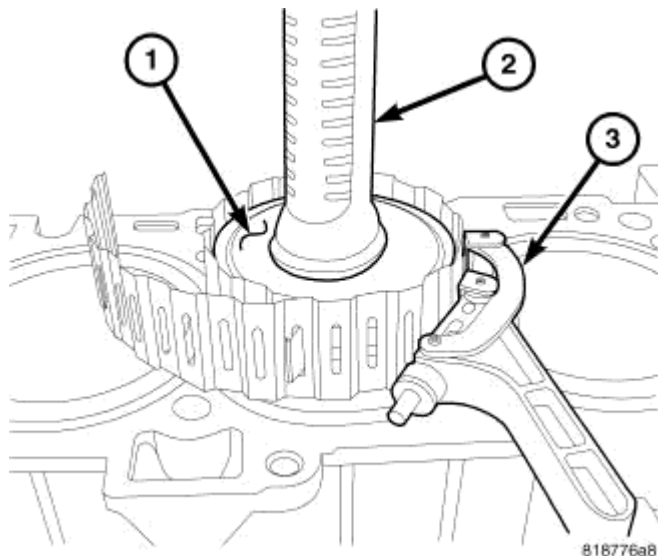
Fig. 218: RING COMPRESSOR
