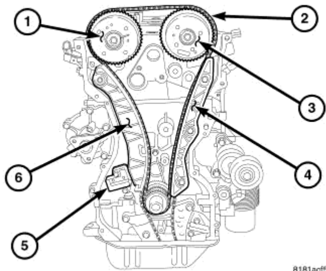
Fig. 76: TIMING DRIVE Courtesy of CHRYSLER LLC
