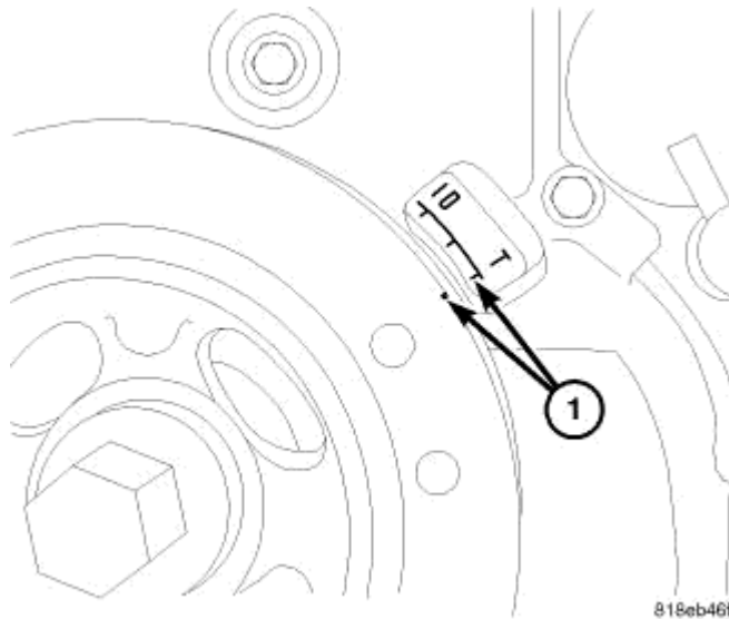
Fig. 66: Top Dead Center Courtesy of CHRYSLER LLC
