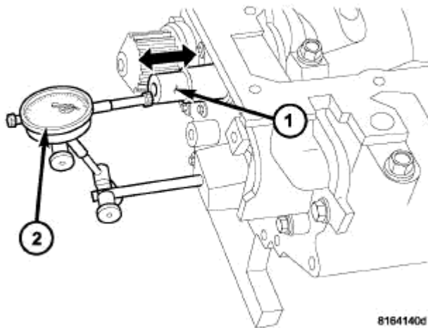
Fig. 174: Checking Crankshaft End Play - Dial Indicator
