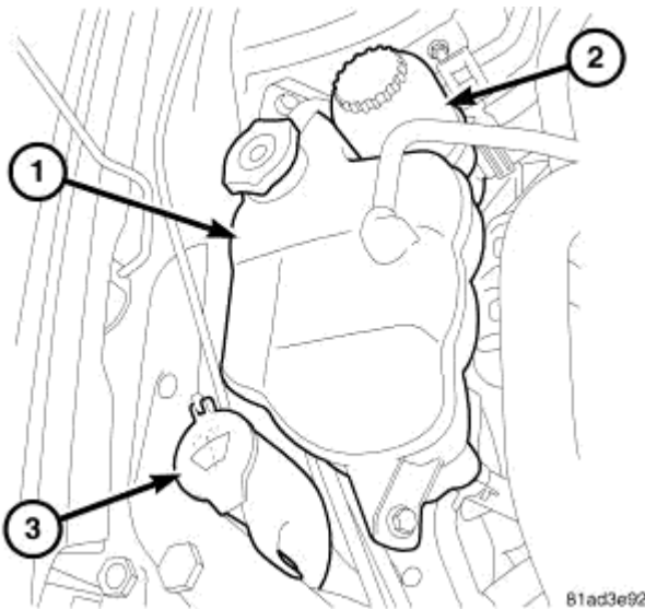
Fig. 110: Coolant Reservoir
