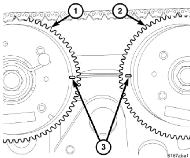
Fig. 344: Camshaft Timing Courtesy of CHRYSLER LLC
