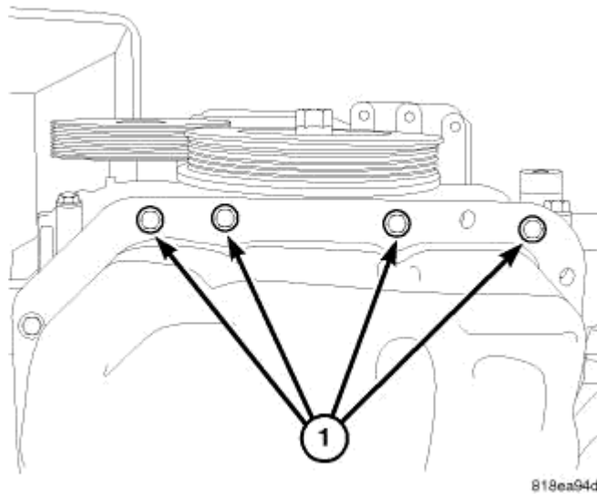
Fig. 70: TIMING CHAIN COVER LOWER BOLTS Courtesy of CHRYSLER LLC
