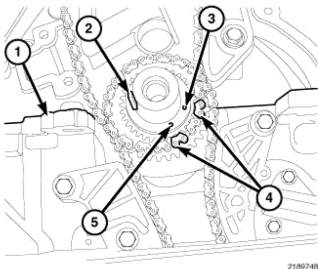
Fig. 356: Crankshaft Timing Marks
