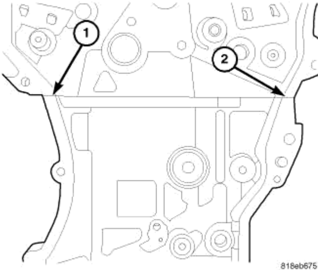
Fig. 375: FRONT COVER UPPER T-JOINT Courtesy of CHRYSLER LLC
