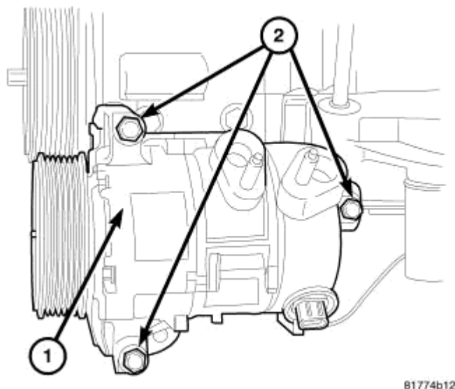
Fig. 313: A/C Compressor Removal/Installation Courtesy of CHRYSLER LLC
