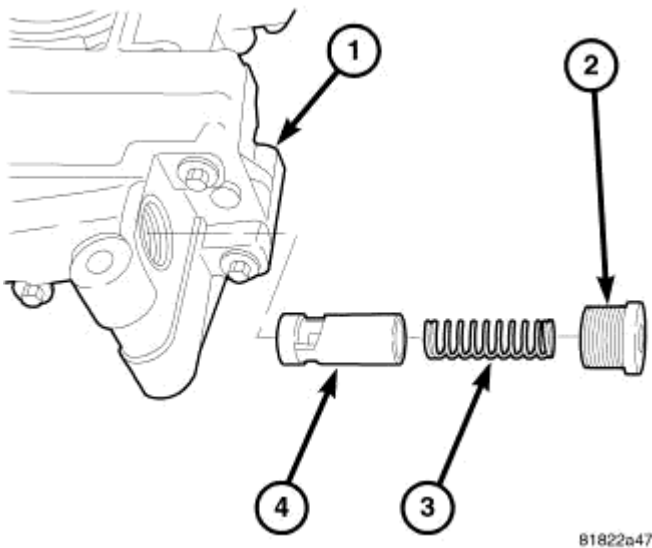
Fig. 316: OIL PRESSURE RELIEF VALVE Courtesy of CHRYSLER LLC
