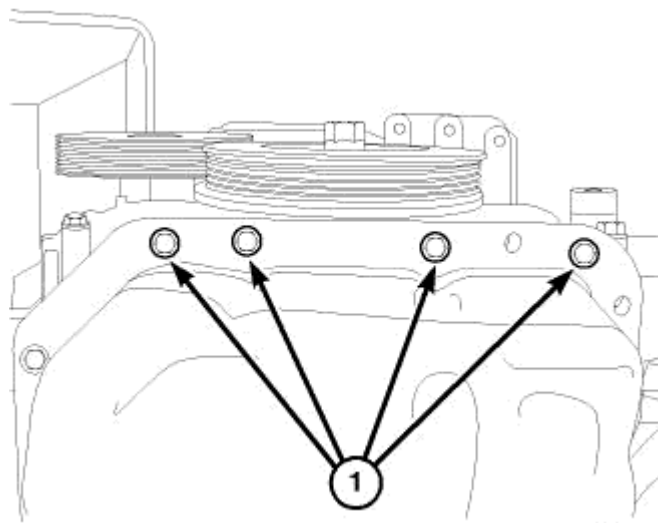
Fig. 383: TIMING CHAIN COVER LOWER BOLTS Courtesy of CHRYSLER LLC
