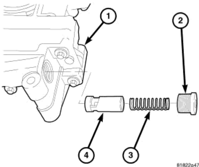
Fig. 314: OIL PRESSURE RELIEF VALVE
