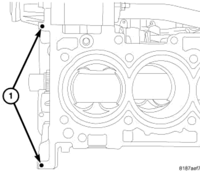
Fig. 90: Two Dots Of Mopar® Engine Sealant RTV On Cylinder Block Courtesy of CHRYSLER LLC
