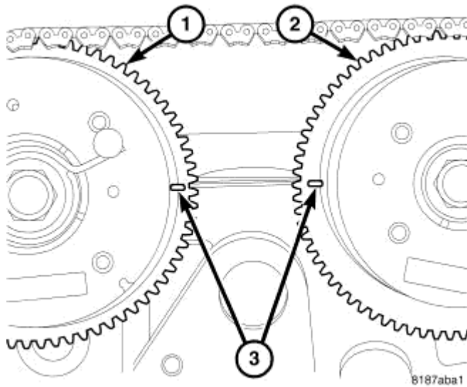
Fig. 100: Camshaft Timing Courtesy of CHRYSLER LLC
