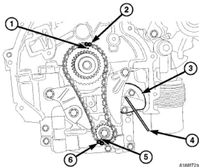
Fig. 300: Balance Shaft Module Tensioner Courtesy of CHRYSLER LLC
