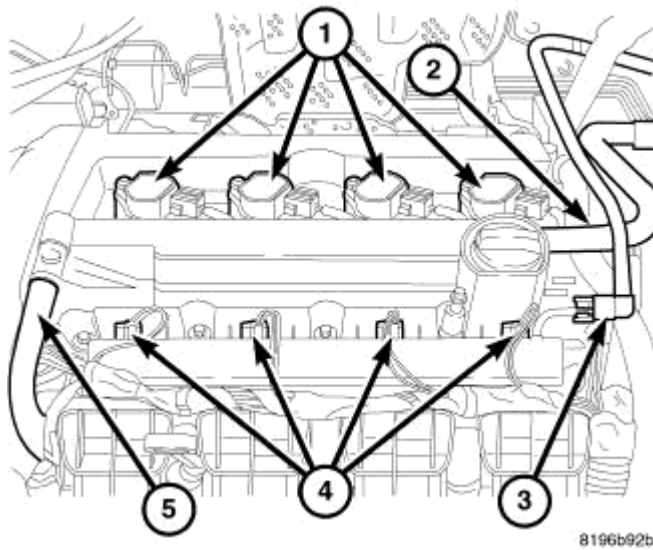
Fig. 338: COIL CONNECTOR Courtesy of CHRYSLER LLC
