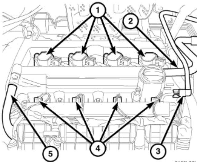
Fig. 15: Coil Connector Courtesy of CHRYSLER LLC
