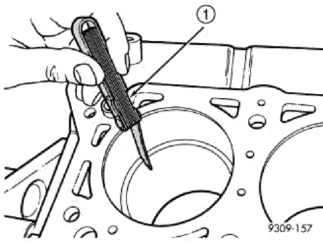
Fig. 204: Check Gap on Piston Rings
