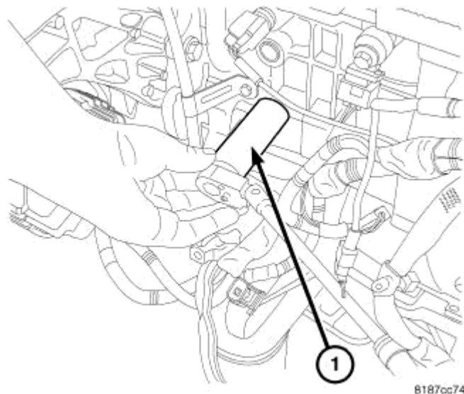
Fig. 311: OIL SENDER Courtesy of CHRYSLER LLC
