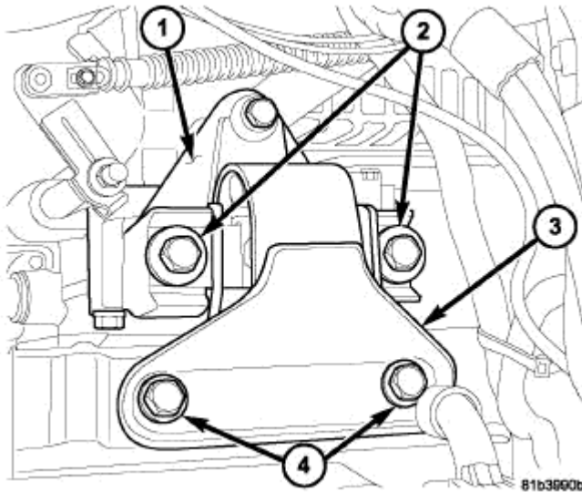
Fig. 232: LEFT MOUNT Courtesy of CHRYSLER LLC
