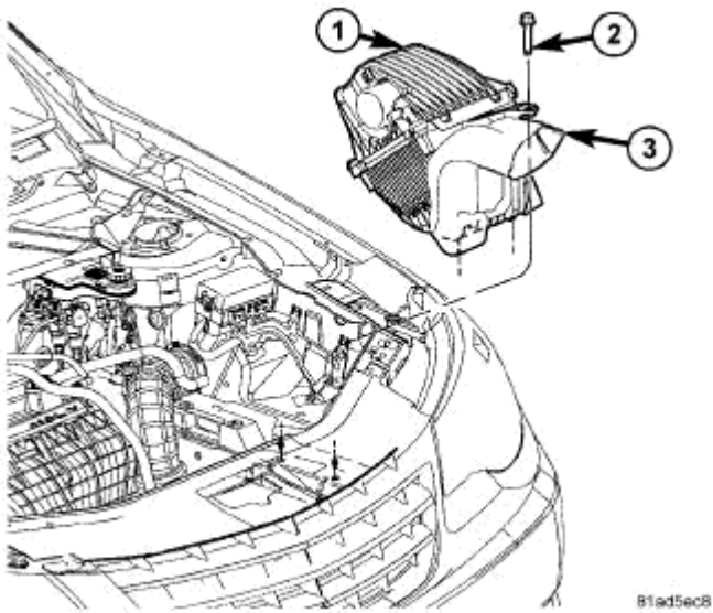
Fig. 231: Air Cleaner Assembly Courtesy of CHRYSLER LLC
