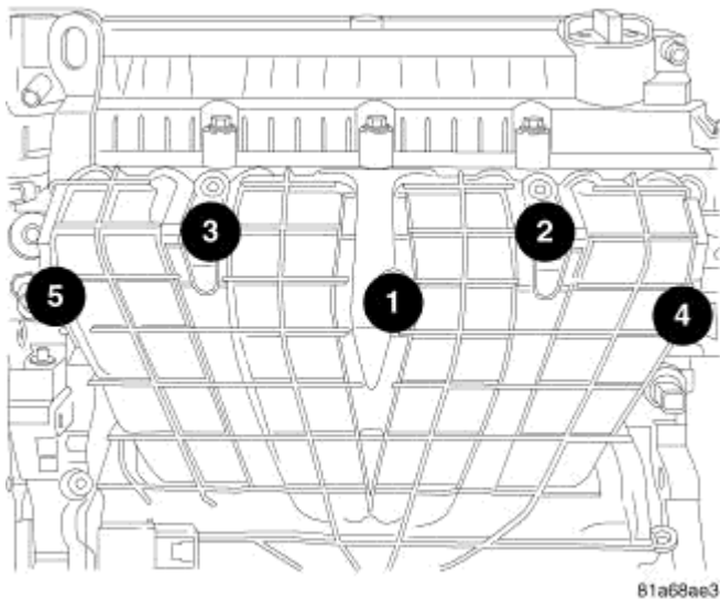
Fig. 337: Intake Manifold Retaining Bolts Torque Sequence Courtesy of CHRYSLER LLC
