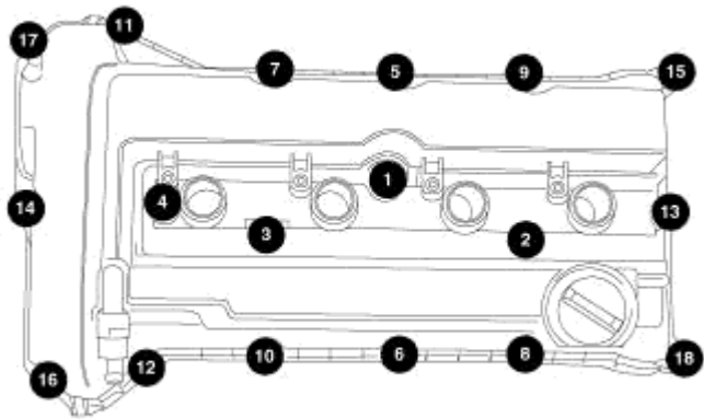
Fig. 387: Cylinder Head Cover Torque Sequence Courtesy of CHRYSLER LLC
