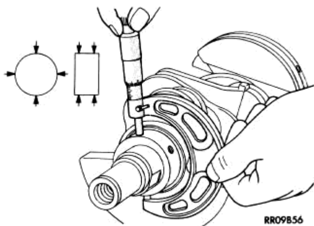
Fig. 184: Crankshaft Journal Measurements - Typical Courtesy of CHRYSLER LLC
