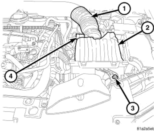
Fig. 111: Air Cleaner Housing Courtesy of CHRYSLER LLC
