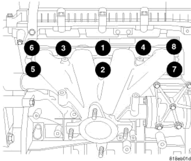
Fig. 323: Exhaust Manifold Retaining Fasteners Torque Sequence Courtesy of CHRYSLER LLC
