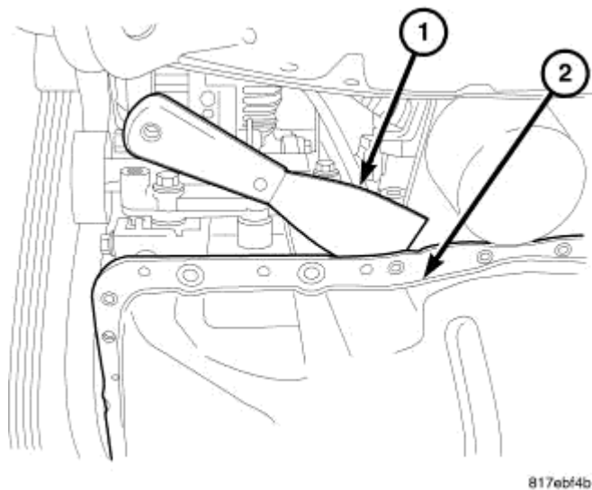
Fig. 291: OIL PAN REMOVAL Courtesy of CHRYSLER LLC
