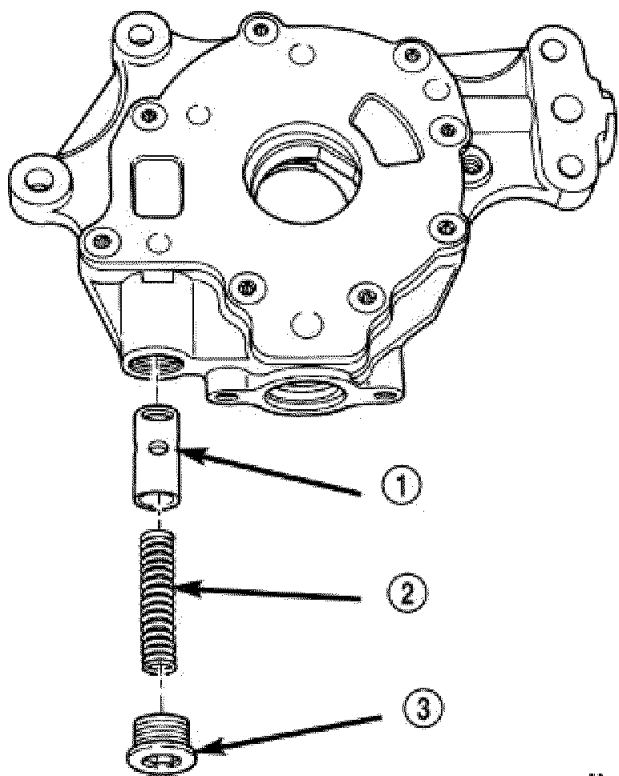
Fig. 285: Oil Pressure Relief Valve Courtesy of CHRYSLER LLC
