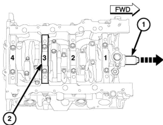
Fig. 187: Moving Crankshaft Forward So Crankshaft Face Is Tight Against Thrust Bearing Courtesy of CHRYSLER LLC
