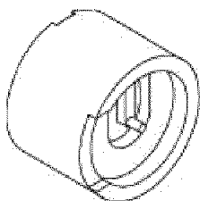
Fig. 69: Timing Chain Tensioner Resetting Gauge 8186 Courtesy of CHRYSLER LLC
