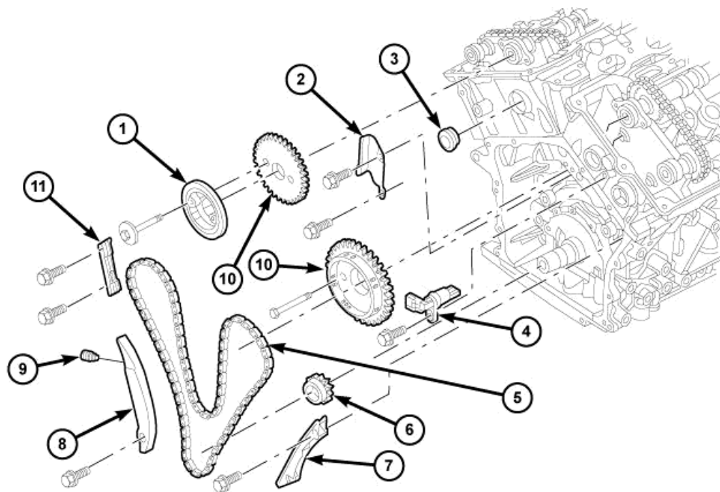
Fig. 331: Identifying Timing Drive System Components Courtesy of CHRYSLER LLC
