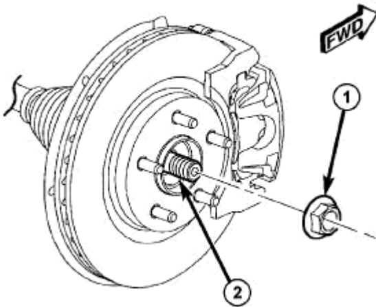
Fig. 17: Axle Shafts Hub Nut
