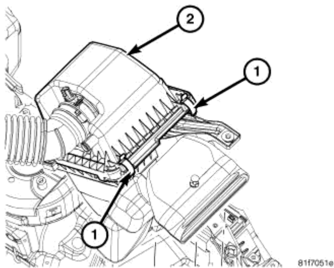
Fig. 86: Air Filter Housing Clips Courtesv of CHRYSLER LLC
