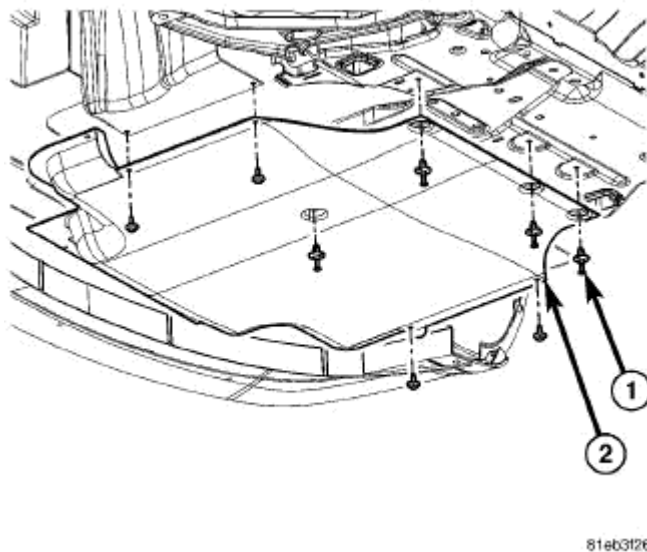
Fig. 242: Belly Pan Courtesy of CHRYSLER LLC
