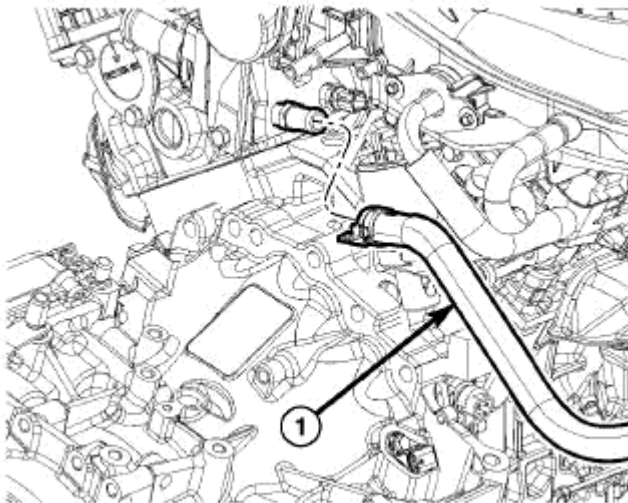
Fig. 35: Heater Hose From Engine Coolant Outlet Courtesy of CHRYSLER LLC
