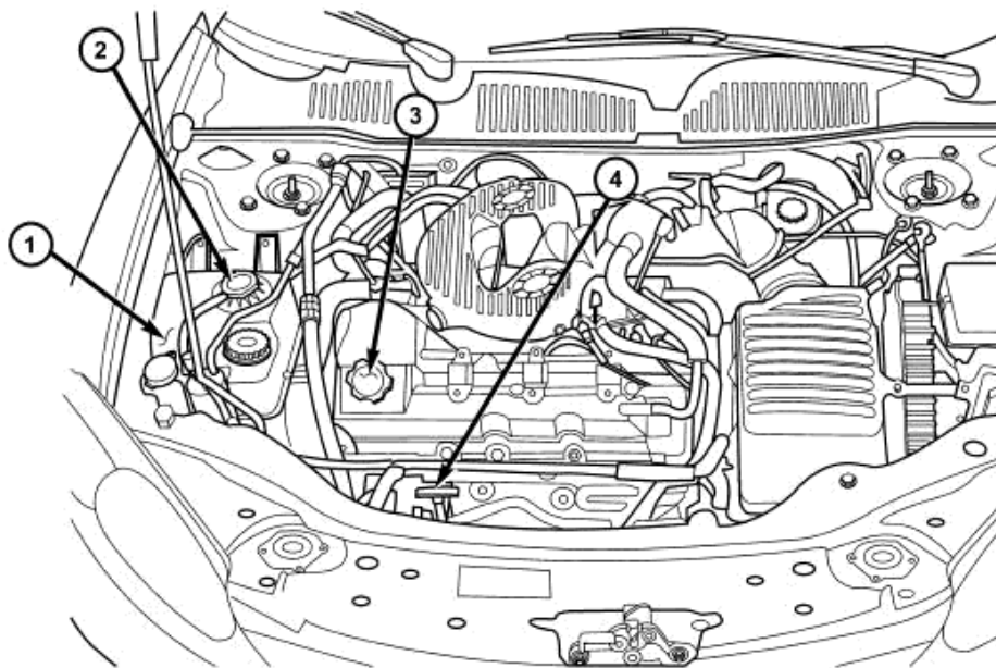
Fig. 258: Identifying Oil Dipstick, Fill Cap, Coolant Pressure Cap & Coolant Pressure Container Courtesy of CHRYSLER LLC
