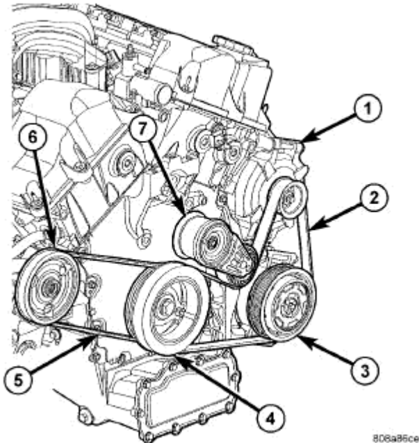
Fig. 345: Accessory Drive Belt System - 2.7L Courtesy of CHRYSLER LLC
