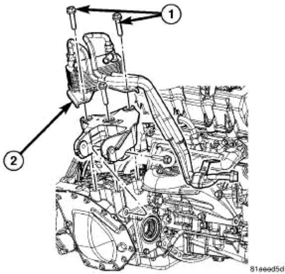
Fig. 253: Oil Cooler Fasteners Courtesy of CHRYSLER LLC
