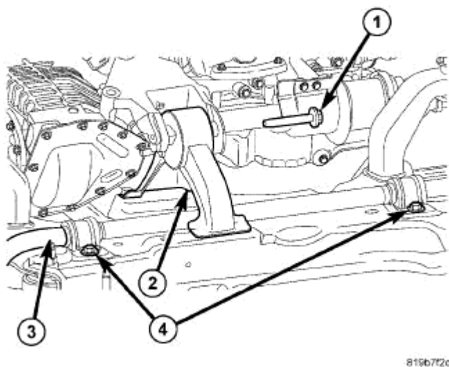
Fig. 238: Rear Isolator On Suspension Crossmember
