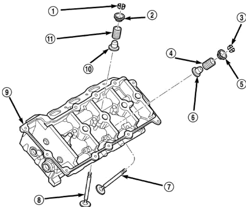
Fig. 158: Cylinder Head, Valves & Springs Courtesy of CHRYSLER LLC
