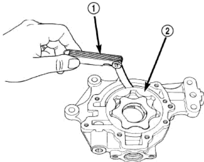
Fig. 281: MEASURING OUTER ROTOR CLEARANCE IN HOUSING Courtesy of CHRYSLER LLC
