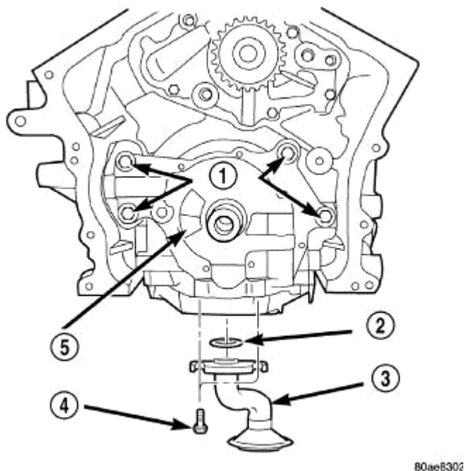
Fig. 284: Oil Pump & Pick-up Tube Courtesy of CHRYSLER LLC
