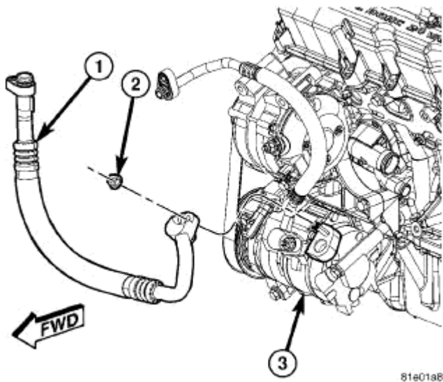
Fig. 14: A/C Compressor To Bracket Courtesy of CHRYSLER LLC
