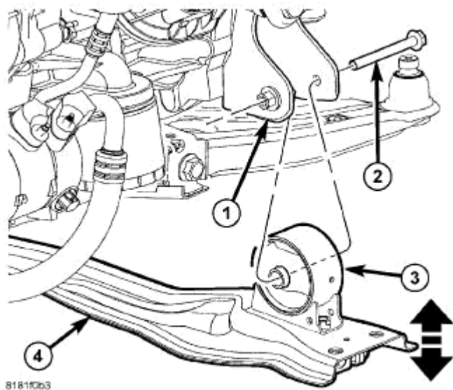
Fig. 173: Front Engine Mount Through Bolt Courtesy of CHRYSLER LLC
