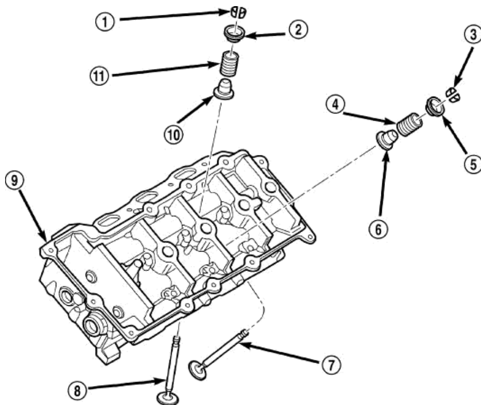
Fig. 162: Cylinder Head, Valves & Springs Courtesy of CHRYSLER LLC
