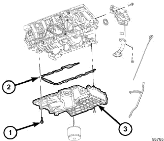
Fig. 267: Oil Pan Attaching Fasteners Courtesy of CHRYSLER LLC
