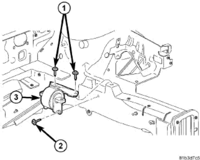
Fig. 231: Mount Isolator Bolts Courtesy of CHRYSLER LLC
