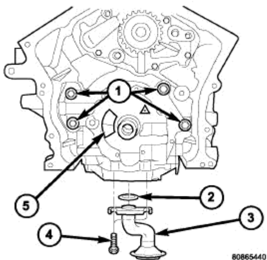
Fig. 194: Oil Pump & Pick-up Tube Courtesy of CHRYSLER LLC
