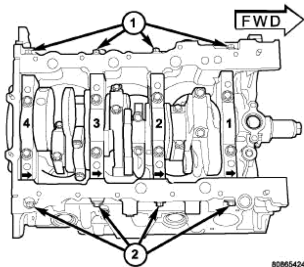
Fig. 182: Main Bearing Cap Identification Courtesy of CHRYSLER LLC
