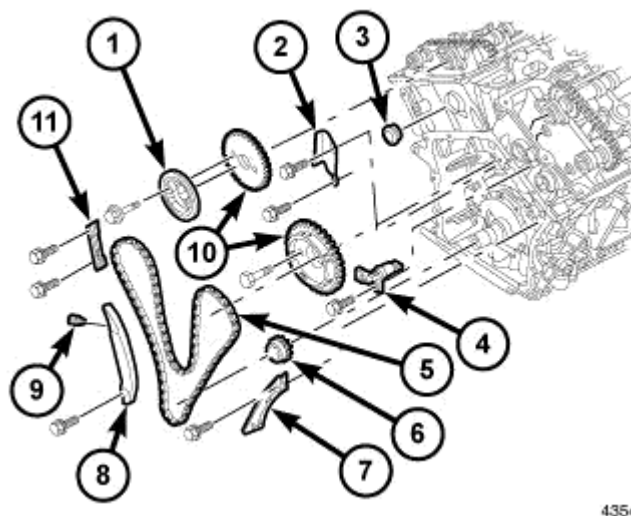
Fig. 342: TIMING DRIVE SYSTEM - PRIMARY Courtesy of CHRYSLER LLC
