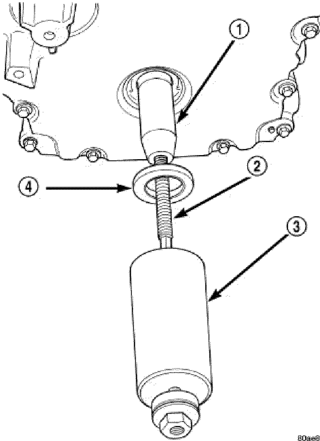
Fig. 213: Crankshaft Front Oil Seal - Installation Courtesy of CHRYSLER LLC
