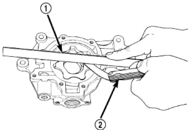
Fig. 283: MEASURING CLEARANCE OVER ROTORS Courtesy of CHRYSLER LLC
