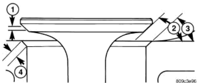
Fig. 152: Valve Face & Seat Courtesy of CHRYSLER LLC
