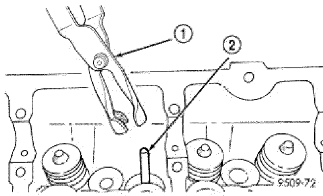
Fig. 143: Valve Stem Seal-Removal/Installation Courtesy of CHRYSLER LLC
