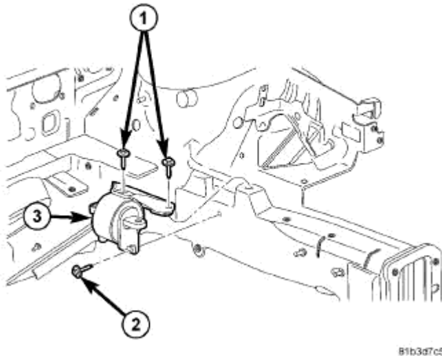
Fig. 230: Mount Isolator Bolts Courtesy of CHRYSLER LLC
