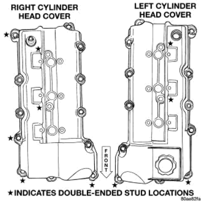
Fig. 95: Cylinder Head Covers Courtesy of CHRYSLER LLC
