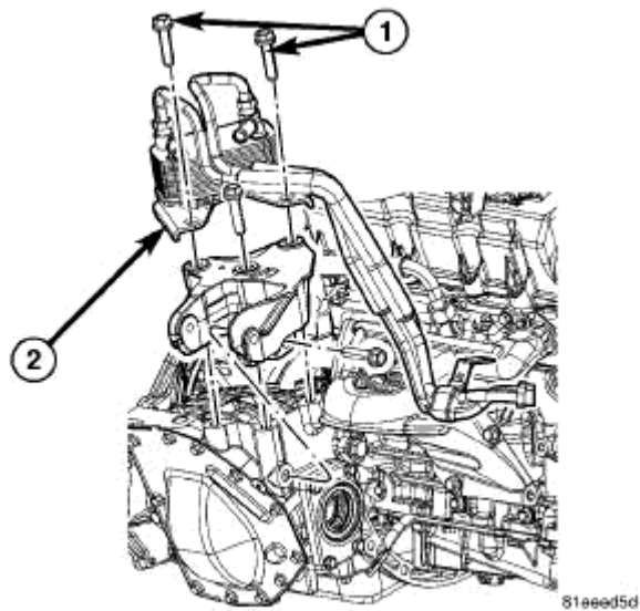
Fig. 250: Oil Cooler Fasteners Courtesy of CHRYSLER LLC
