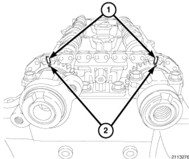
Fig. 116: Identifying Marked Links & Timing Dot On Camshaft Sprockets Courtesy of CHRYSLER LLC
