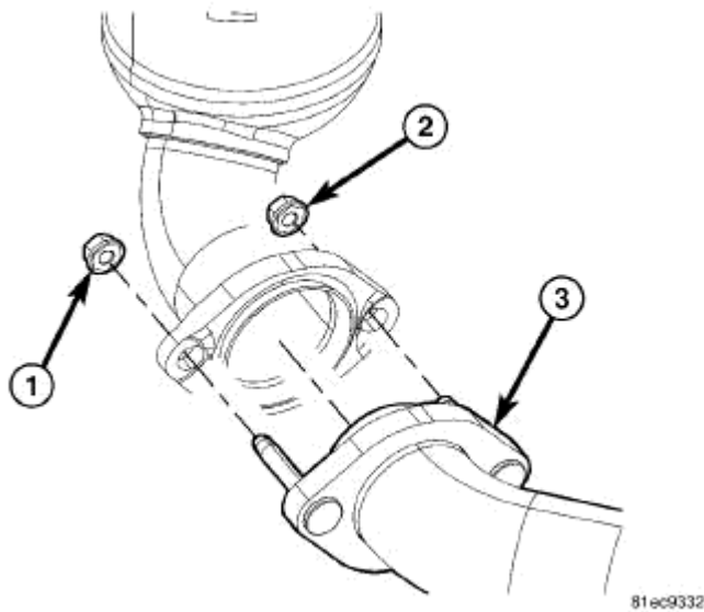
Fig. 301: Front Maniverter-To-Cross Under Fasteners Courtesy of CHRYSLER LLC
