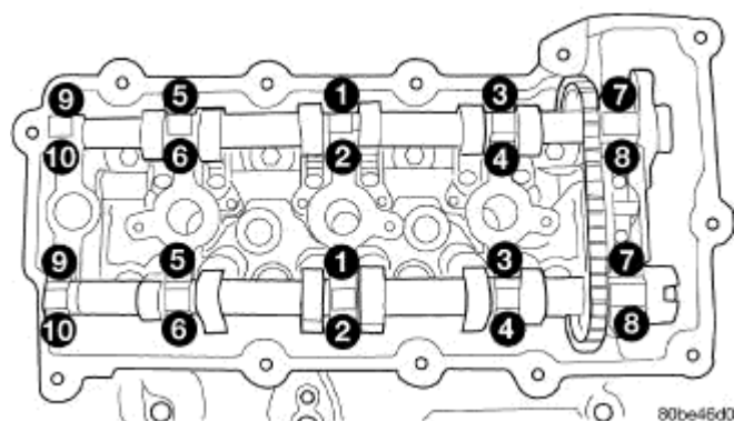
Fig. 117: Camshaft Bearing Cap Tightening Sequence Courtesy of CHRYSLER LLC
