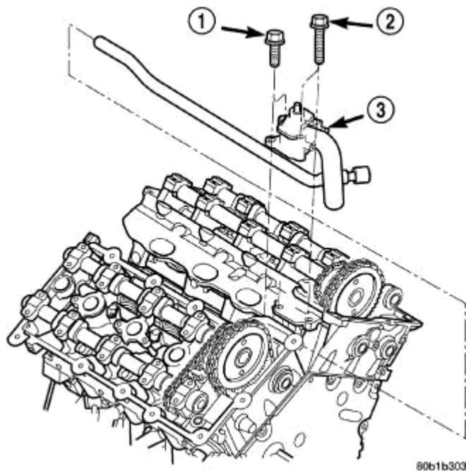
Fig. 104: WATER OUTLET CONNECTOR Courtesy of CHRYSLER LLC
