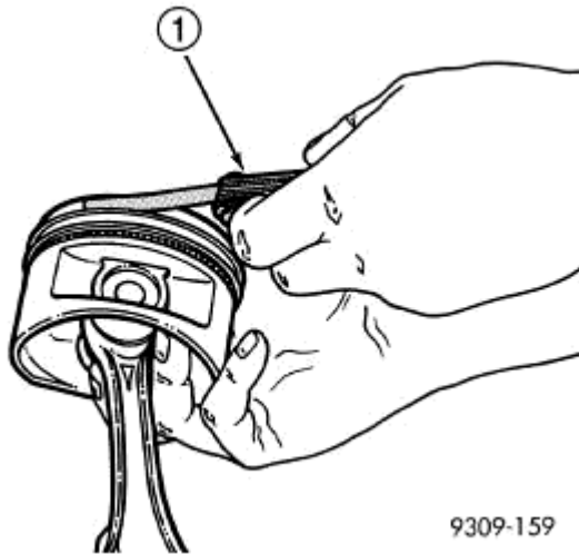
Fig. 201: Measuring Piston Ring Side Clearance Courtesy of CHRYSLER LLC
