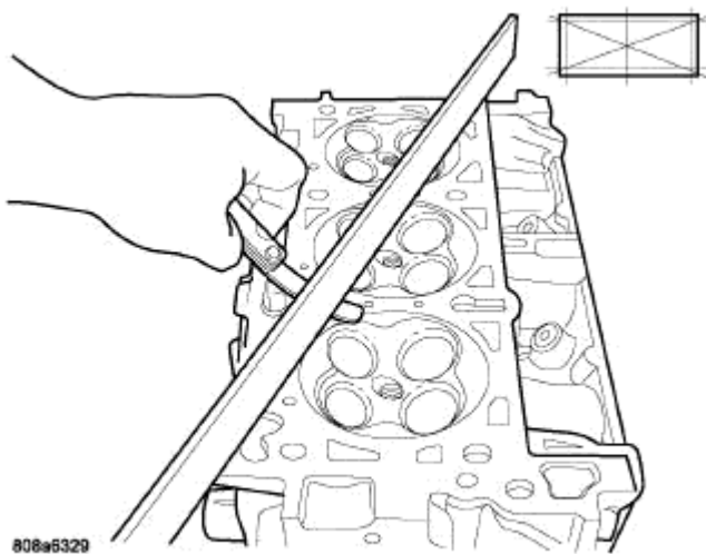
Fig. 100: Checking Cylinder Head Flatness-Typical Courtesy of CHRYSLER LLC
