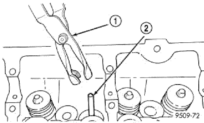
Fig. 146: Valve Stem Seal-Removal/Installation
