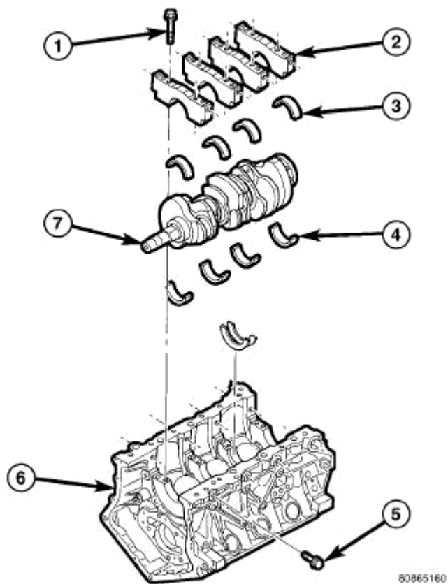
Fig. 186: Cylinder Block & Crankshaft Courtesy of CHRYSLER LLC
