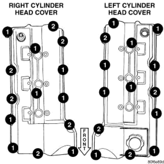
Fig. 131: Cylinder Head Cover Fasteners Courtesy of CHRYSLER LLC
