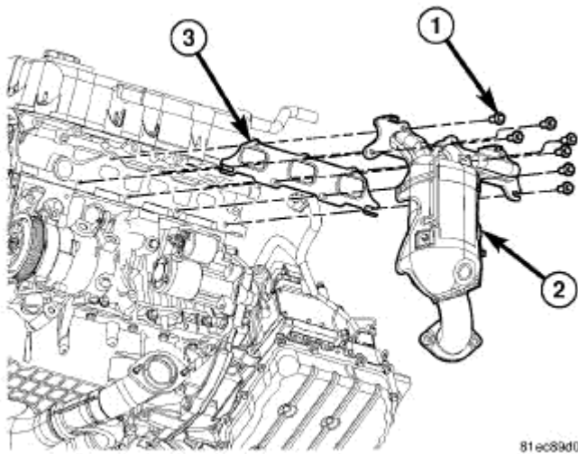
Fig. 300: Front Exhaust Maniverter Attaching Bolts Courtesy of CHRYSLER LLC
