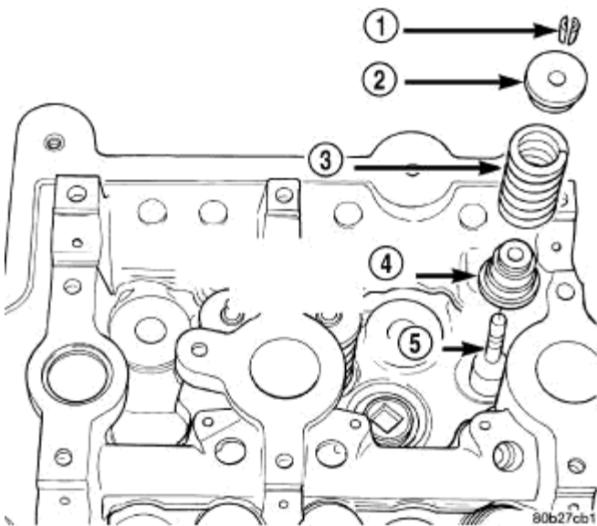
Fig. 156: Valve Seal & Spring Courtesy of CHRYSLER LLC
