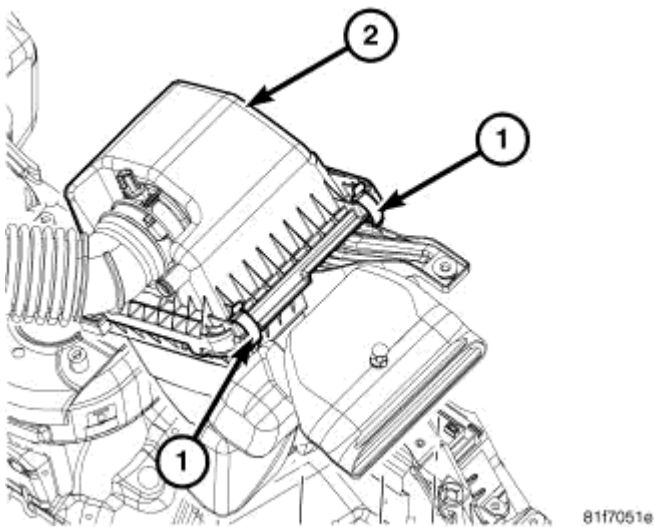
Fig. 85: Air Filter Housing Clips Courtesy of CHRYSLER LLC
