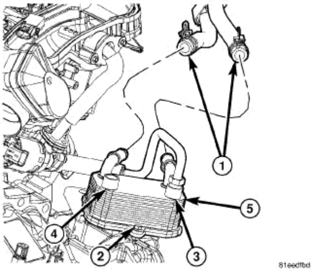
Fig. 251: Heater Hoses From Oil Cooler Courtesy of CHRYSLER LLC
