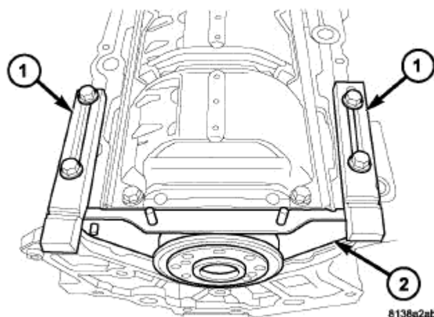
Fig. 220: REAR MAIN - SPECIAL TOOL 8225 Courtesy of CHRYSLER LLC
