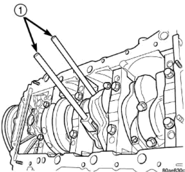
Fig. 209: Connecting Rod Guides Courtesy of CHRYSLER LLC
