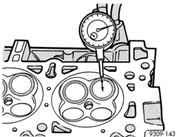
Fig. 160: Measuring Valve Guide Wear - Typical Courtesy of CHRYSLER LLC
