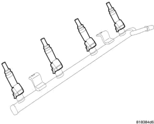
Fig. 322: Fuel Injector Location - Typical Courtesy of CHRYSLER LLC
