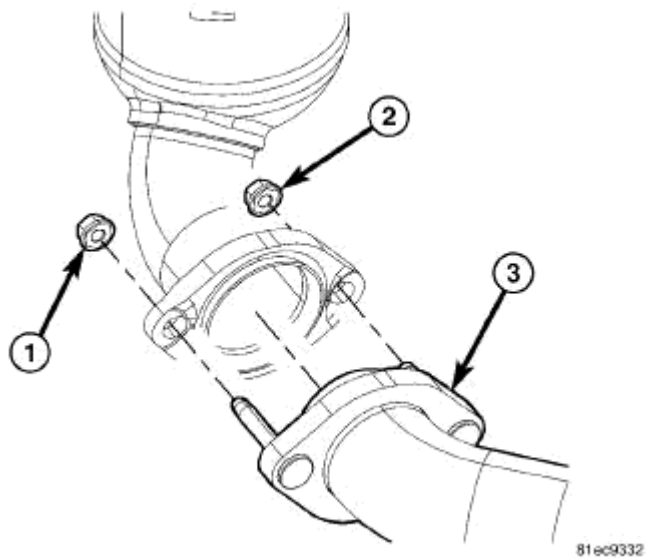
Fig. 290: Front Maniverter-To-Cross Under Fasteners Courtesy of CHRYSLER LLC
