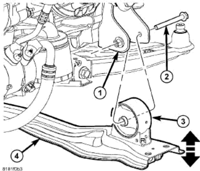
Fig. 18: Front Engine Mount Through Bolt Courtesy of CHRYSLER LLC
