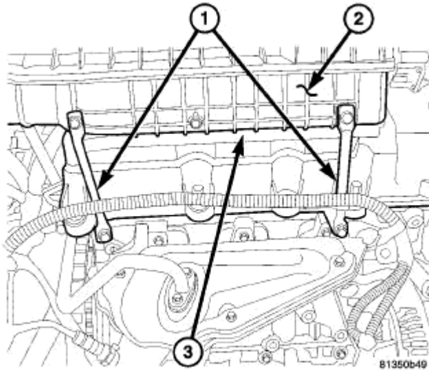
Fig. 320: Intake Brackets Courtesy of CHRYSLER LLC
