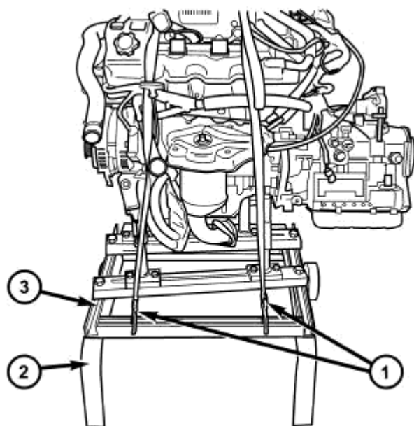
Fig. 31: ENGINE REMOVAL CRADLE Courtesy of CHRYSLER LLC
