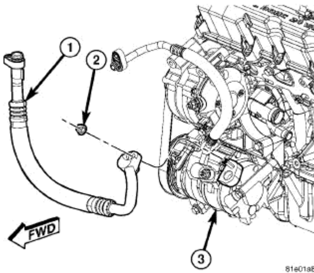
Fig. 43: A/C Compressor To Bracket
