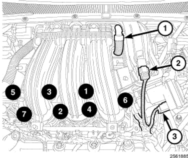
Fig. 321: Locating Manifold Bolts, Manifold Absolute Pressure Sensor & Electronic Throttle Control Electrical Connectors Courtesy of CHRYSLER LLC
