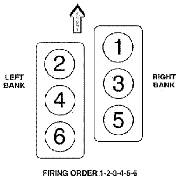
Fig. 2: Cylinder Numbering & Firing Order Courtesy of CHRYSLER LLC
