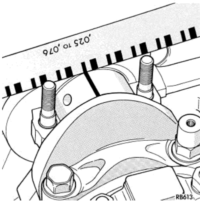
Fig. 166: Checking Connecting Rod Bearing Clearance-Typical
