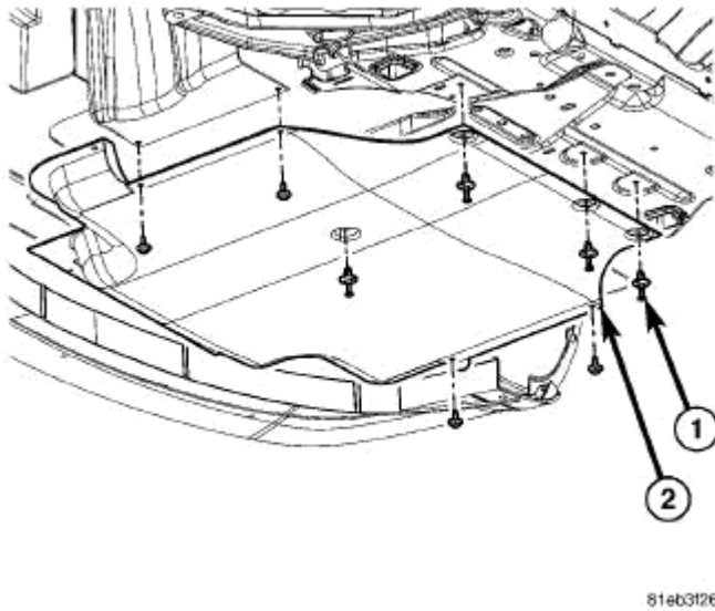
Fig. 7: Belly Pan
