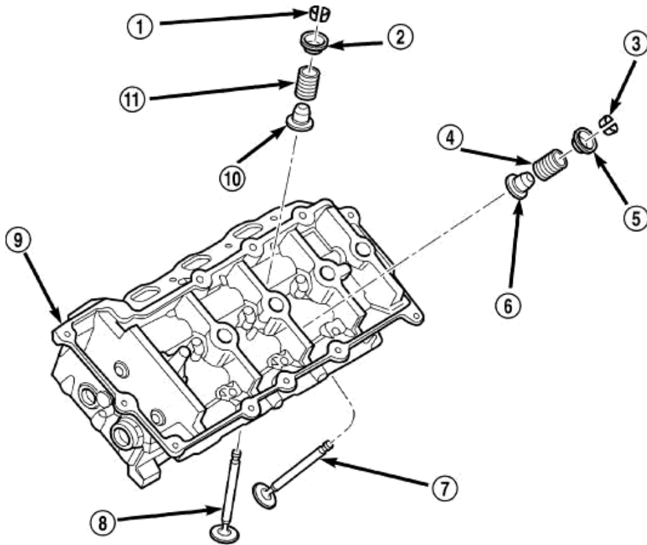
Fig. 91: Cylinder Head, Valves & Springs Courtesy of CHRYSLER LLC
