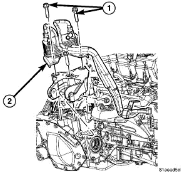
Fig. 254: Oil Cooler Fasteners Courtesy of CHRYSLER LLC
