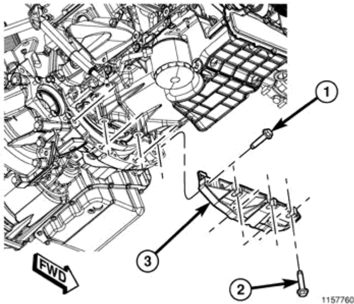
Fig. 263: Structural Collar Courtesy of CHRYSLER LLC
