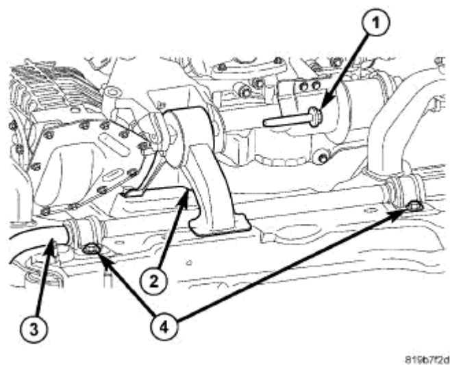
Fig. 240: Rear Isolator On Suspension Crossmember Courtesy of CHRYSLER LLC
