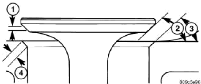
Fig. 153: Valve Face & Seat Courtesy of CHRYSLER LLC
