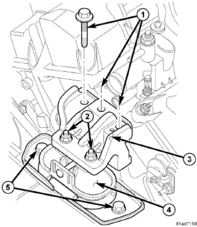
Fig. 245: Right Engine Mount Courtesy of CHRYSLER LLC
