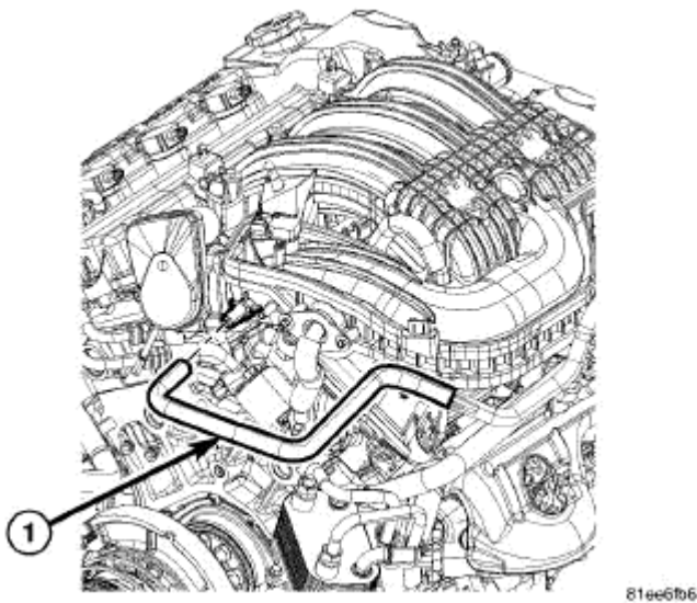
Fig. 32: Brake Booster Vacuum Hose Courtesy of CHRYSLER LLC
