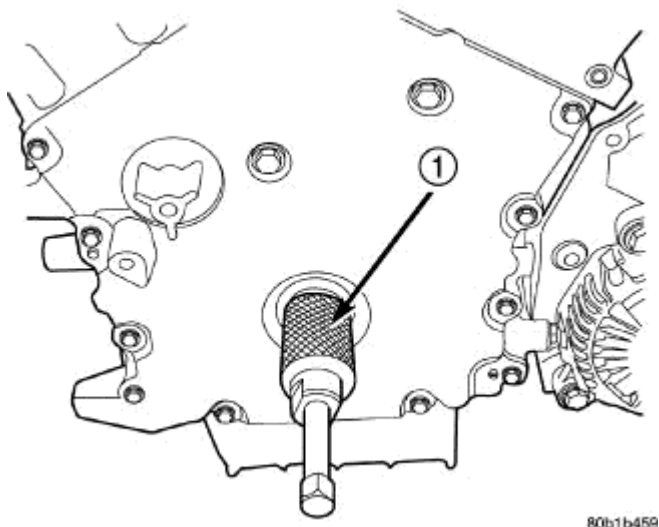
Fig. 212: Crankshaft Front Oil Seal - Removal Courtesy of CHRYSLER LLC
