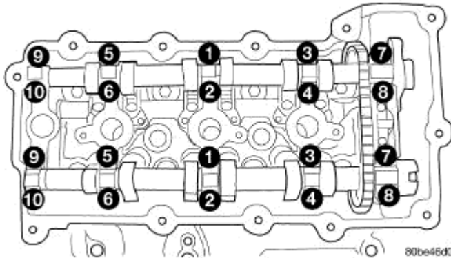
Fig. 97: Camshaft Bearing Cap Tightening Sequence Courtesy of CHRYSLER LLC
