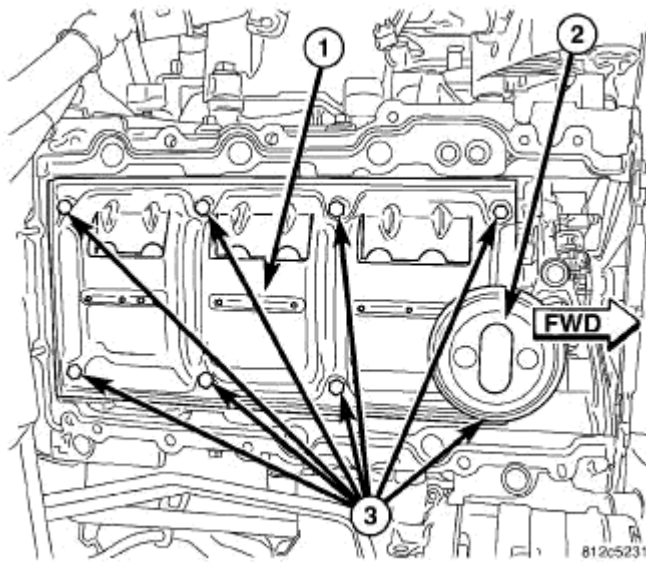
Fig. 192: Windage Tray Courtesy of CHRYSLER LLC
