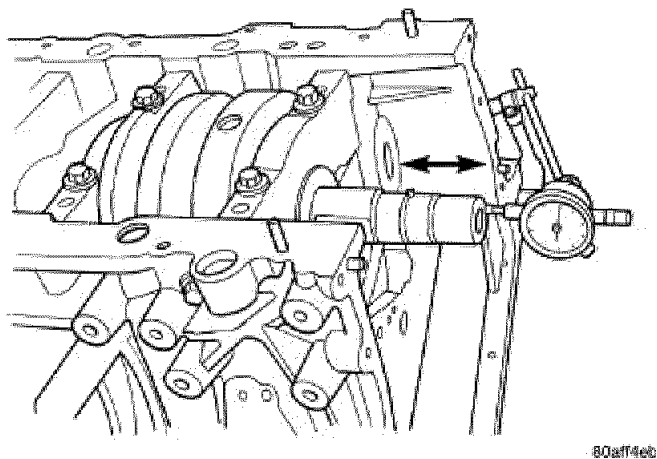
Fig. 178: CHECKING CRANKSHAFT END PLAY Courtesy of CHRYSLER LLC
