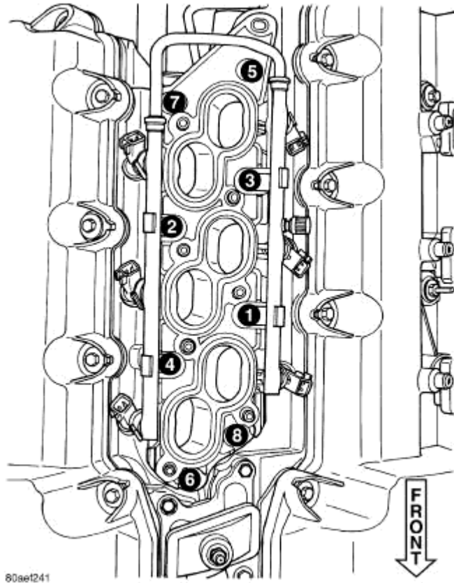
Fig. 94: Lower Intake Manifold Tightening Sequence Courtesy of CHRYSLER LLC
