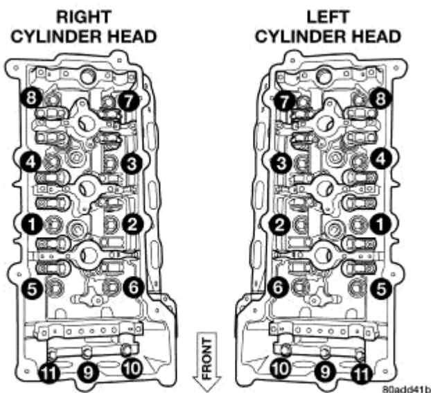
Fig. 102: Cylinder Head Tightening Sequence Courtesy of CHRYSLER LLC
