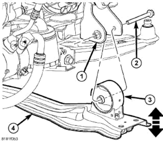
Fig. 262: Front Engine Mount Through Bolt Courtesy of CHRYSLER LLC
