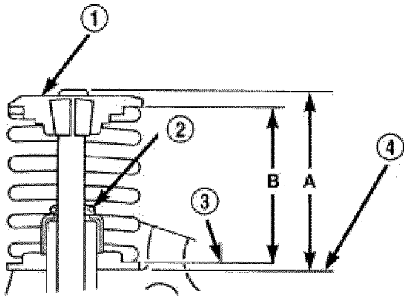
Fig. 155: Valve Tip Height & Valve Spring Installed Height Courtesy of CHRYSLER LLC
