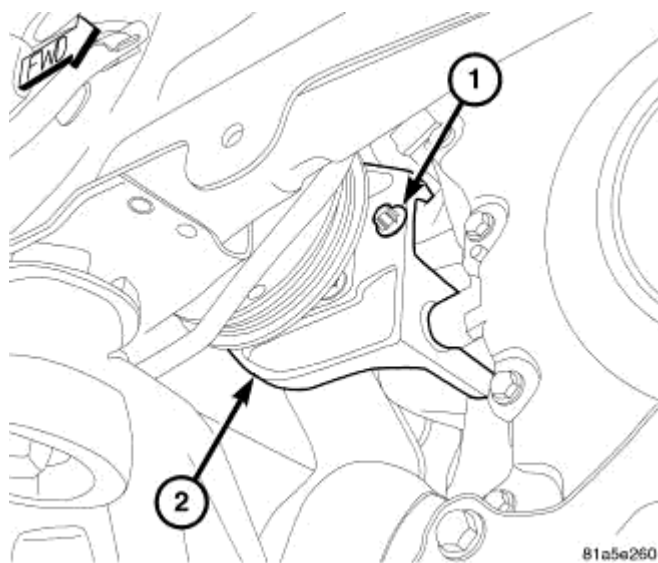
Fig. 344: FRONT PUMP MOUNTING BRACKET BOLTS - 2.7L
