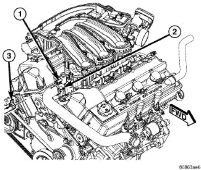
Fig. 96: Coolant Outlet Connector - 2.7L Courtesy of CHRYSLER LLC
