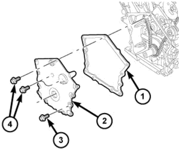
Fig. 352: TIMING CHAIN COVER
