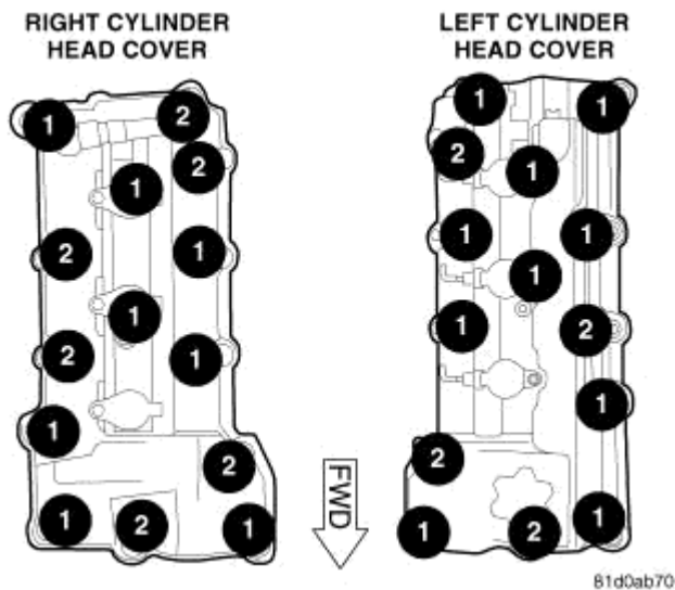
Fig. 123: Cylinder Head Cover Fasteners Courtesy of CHRYSLER LLC
