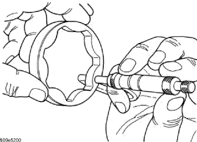
Fig. 279: MEASURING OUTER ROTOR THICKNESS Courtesy of CHRYSLER LLC
