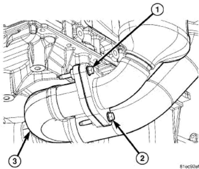
Fig. 312: Exhaust Cross-Under Pipe Courtesy of CHRYSLER LLC
