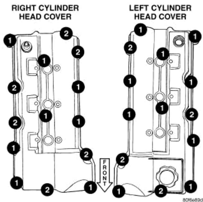
Fig. 195: Cylinder Head Cover Fasteners Courtesy of CHRYSLER LLC
