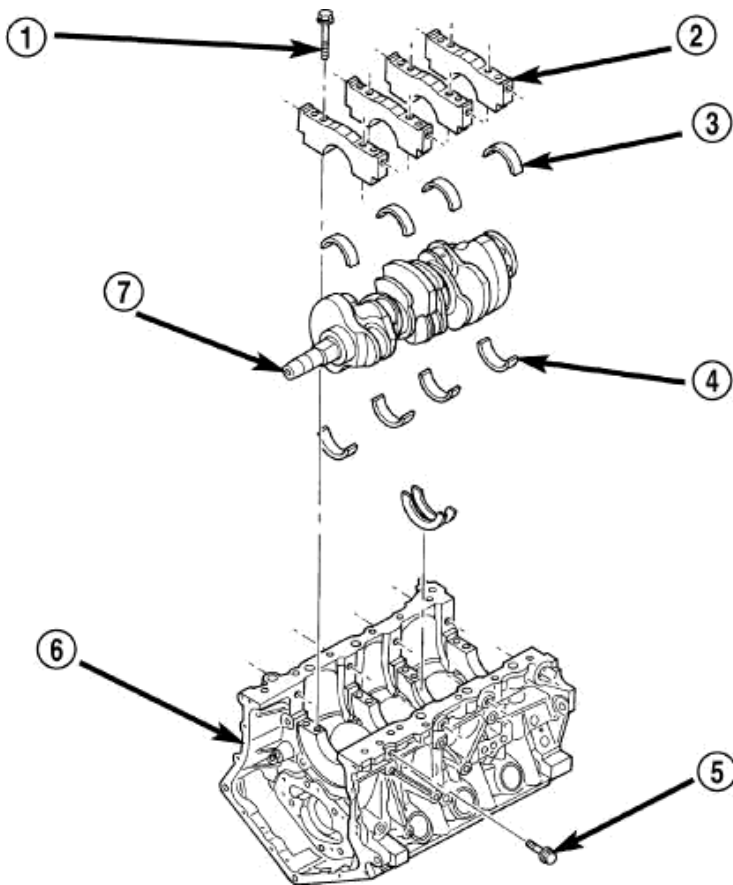
Fig. 163: Engine Block & Crankshaft Courtesy of CHRYSLER LLC
