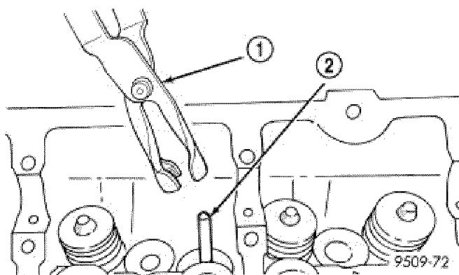
Fig. 140: Valve Stem Seal-Removal/Installation Courtesy of CHRYSLER LLC
