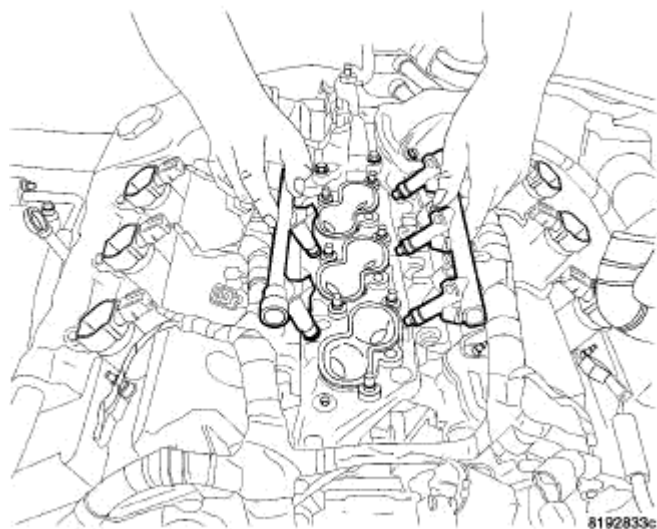
Fig. 323: FUEL RAIL REMOVE/INSTALL Courtesy of CHRYSLER LLC
