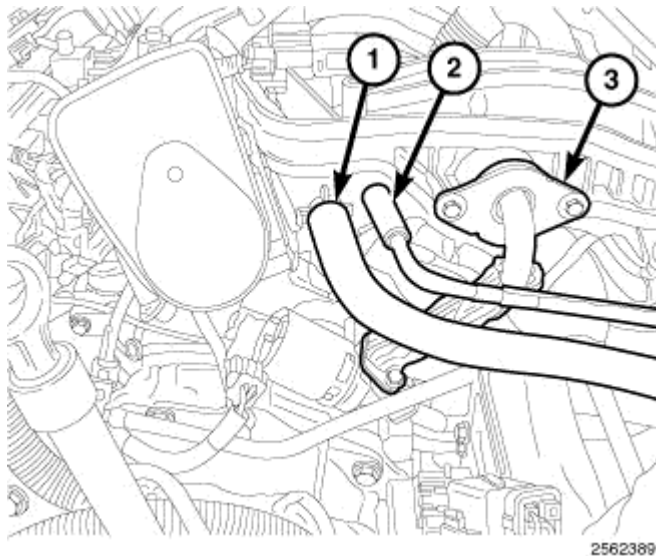
Fig. 319: Locating Upper Exhaust Gas Recirculation Tube, Brake Booster Hose & Vapor Purge Hose Courtesv of CHRYSLER LLC
