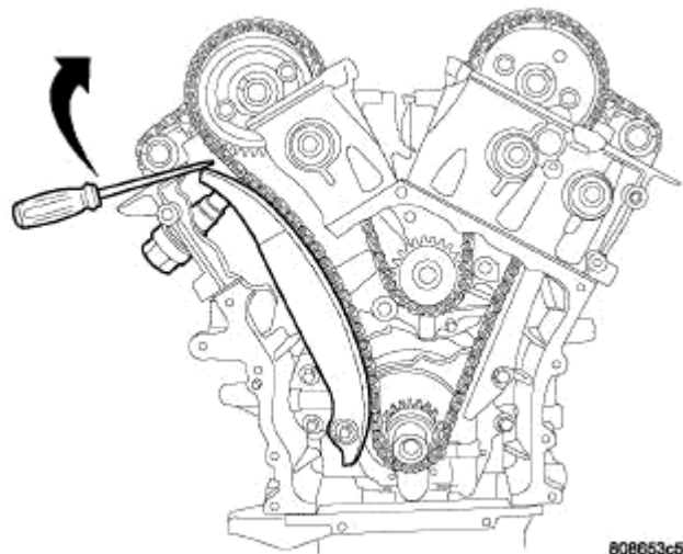
Fig. 343: TIMING CHAIN TENSIONER ACTIVATING Courtesy of CHRYSLER LLC
