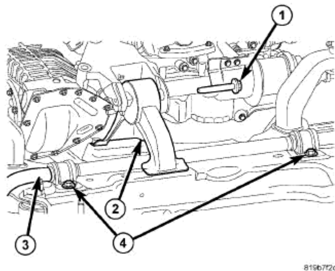
Fig. 237: Rear Engine Mount & Transaxle Bracket Courtesy of CHRYSLER LLC
