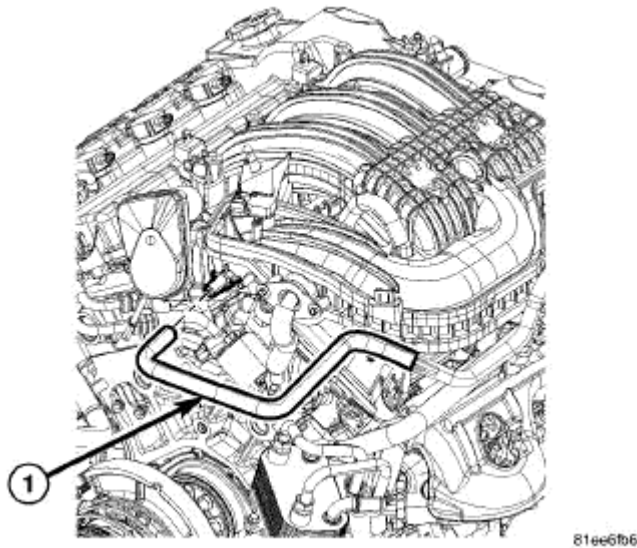
Fig. 30: Brake Booster Vacuum Hose Courtesy of CHRYSLER LLC
