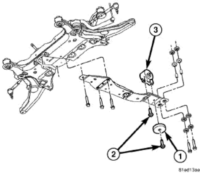
Fig. 225: Front Mount Vertical Bolts Courtesy of CHRYSLER LLC
