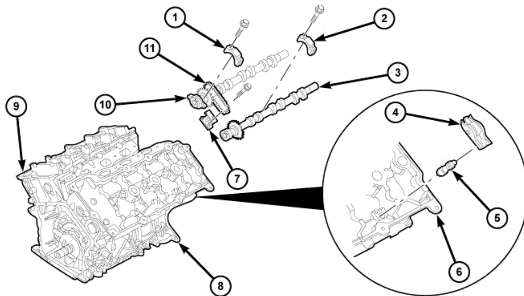
Fig. 332: Camshaft & Valvetrain Components Courtesy of CHRYSLER LLC
