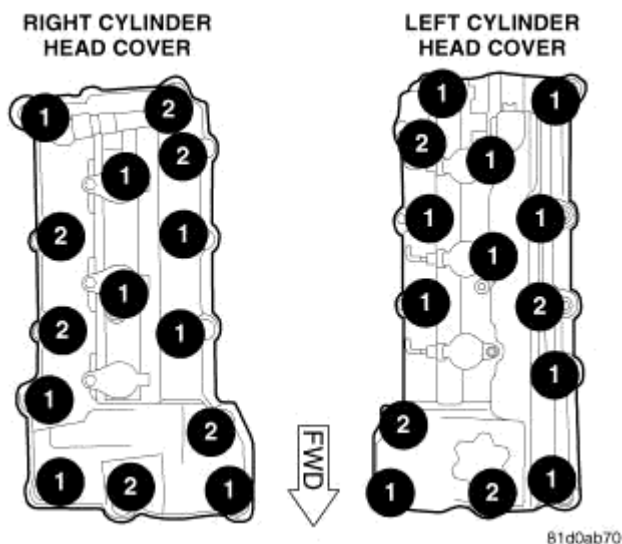
Fig. 127: Cylinder Head Cover Fasteners Courtesy of CHRYSLER LLC
