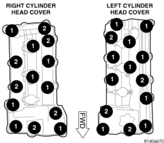
Fig. 346: Cylinder Head Cover Fasteners
