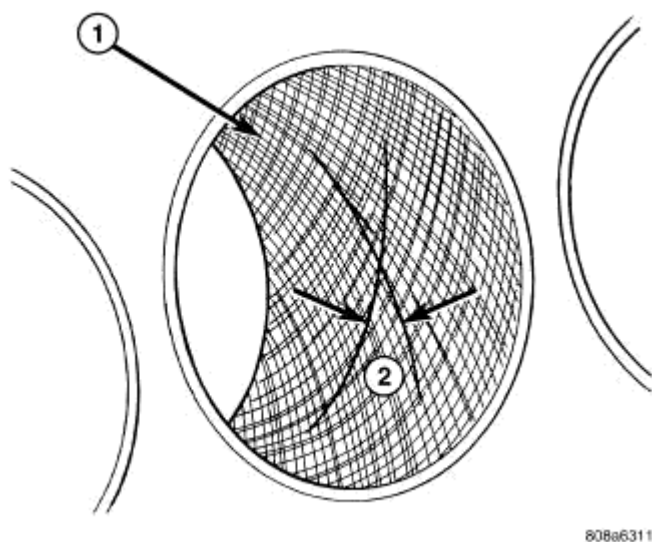
Fig. 164: Cylinder Bore Cross-Hatch Pattern Courtesy of CHRYSLER LLC
