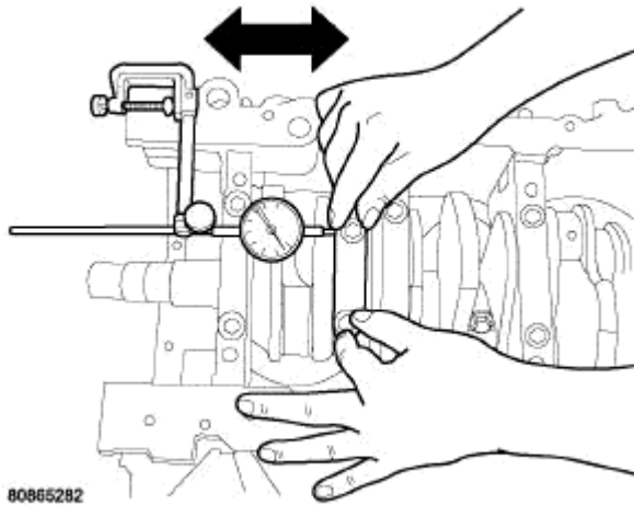
Fig. 191: Measuring Connecting Rod Side Clearance Courtesy of CHRYSLER LLC
