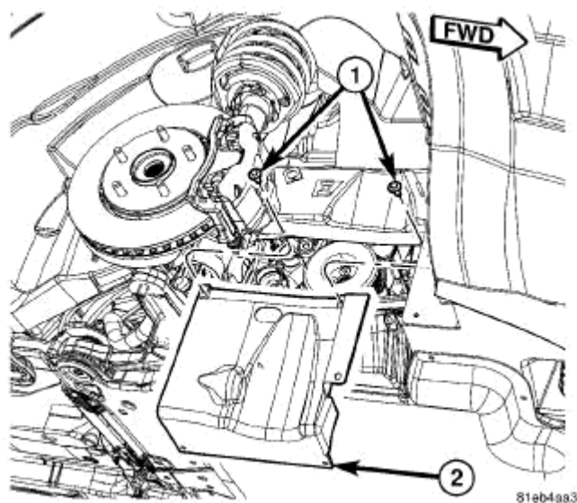
Fig. 52: Right Lower Splash Shield Courtesy of CHRYSLER LLC
