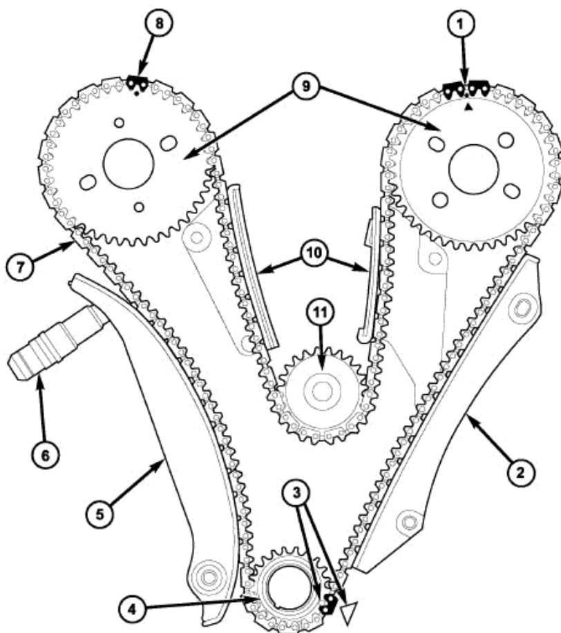
Fig. 338: TIMING CHAIN ALIGNMENT MARKS - PRIMARY Courtesy of CHRYSLER LLC
