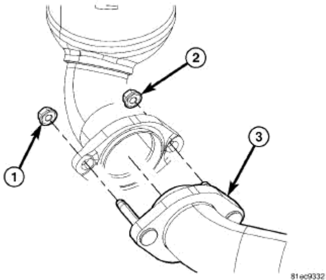
Fig. 291: Front Maniverter-To-Cross Under Fasteners Courtesy of CHRYSLER LLC
