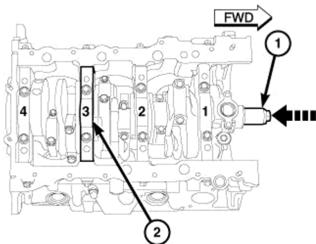
Fig. 189: Moving Crankshaft Rearward So Crankshaft Face Is Tight Against Thrust Bearing Courtesy of CHRYSLER LLC
