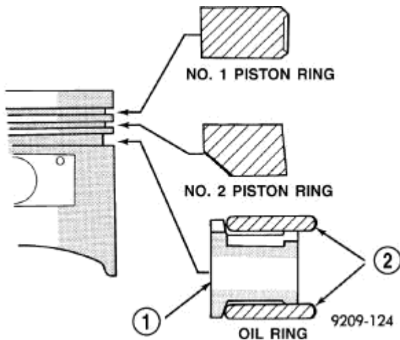
Fig. 202: PISTON RING - INSTALLATION Courtesy of CHRYSLER LLC
