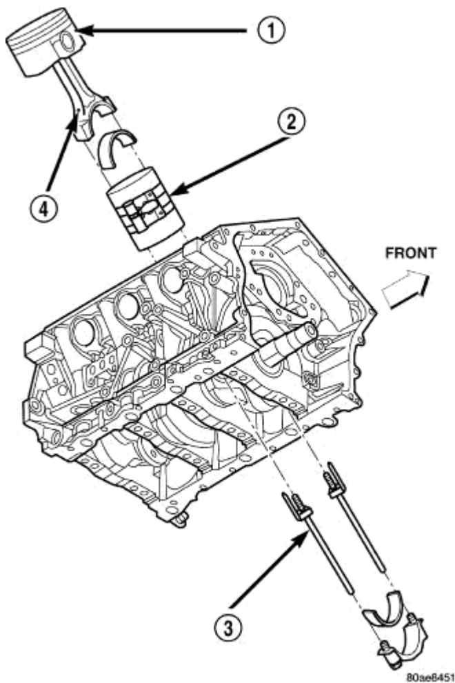
Fig. 206: Piston & Connecting Rod Courtesy of CHRYSLER LLC
