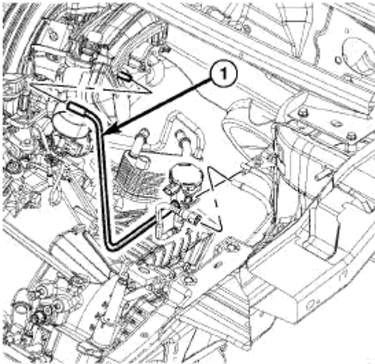
Fig. 29: Vapor Purge Vacuum Hose Courtesy of CHRYSLER LLC
