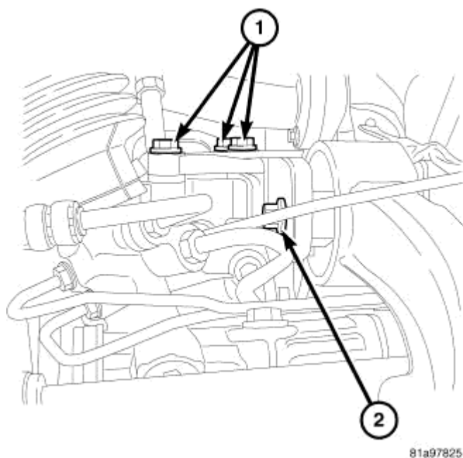
Fig. 235: Identifying Rear Mount Bracket-To-Transaxle Case Bolts Courtesy of CHRYSLER LLC
