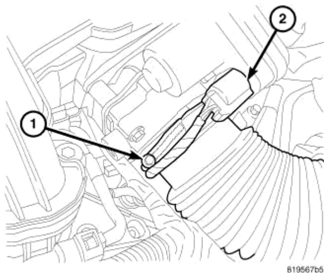
Fig. 24: Electronic Throttle Control Harness Connector Courtesy of CHRYSLER LLC
