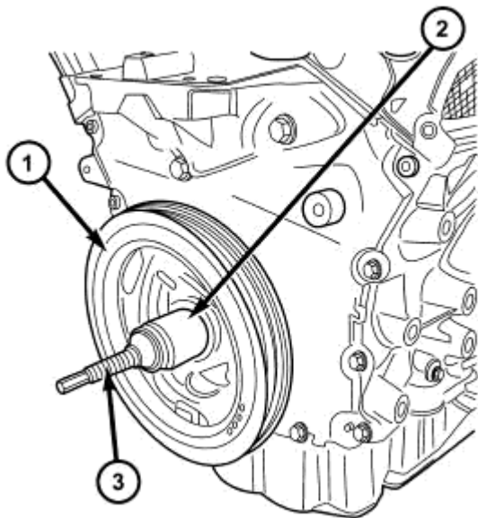
Fig. 197: Vibration Damper - Installation Courtesy of CHRYSLER LLC
