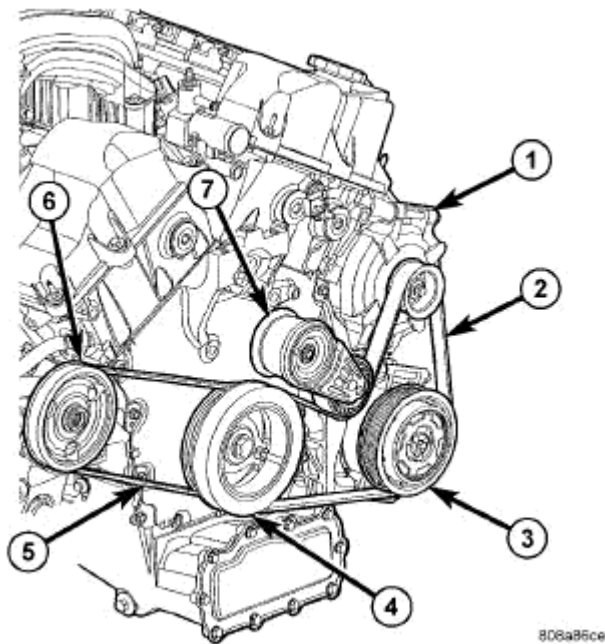
Fig. 107: Accessory Drive Belt System - 2.7L Courtesy of CHRYSLER LLC
