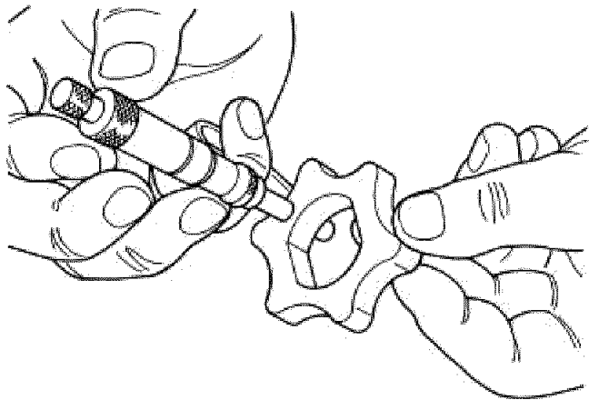
Fig. 280: MEASURING INNER ROTOR THICKNESS Courtesy of CHRYSLER LLC
