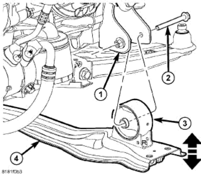
Fig. 226: Front Engine Mount Through Bolt Courtesy of CHRYSLER LLC
