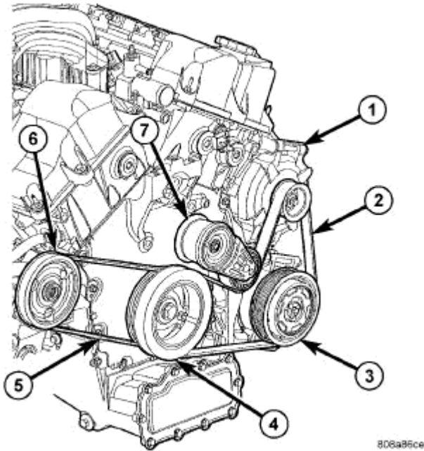
Fig. 44: Accessory Drive Belt System - 2.7L Courtesy of CHRYSLER LLC
