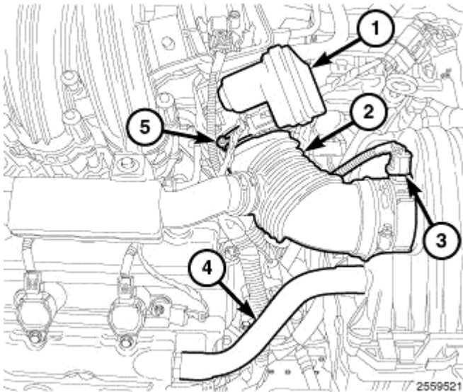
Fig. 318: Identifying Air Makeup Hose, Throttle Body & Air Inlet Hose Courtesy of CHRYSLER LLC
