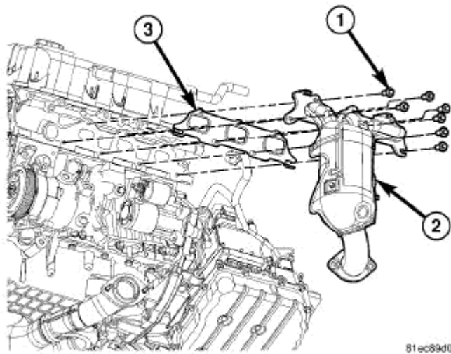
Fig. 299: Front Exhaust Maniverter Attaching Bolts Courtesy of CHRYSLER LLC
