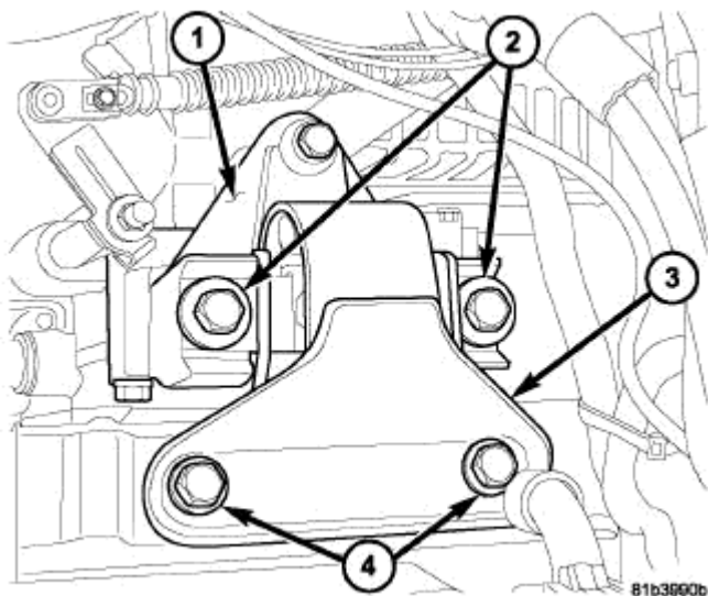
Fig. 232: Identifying Left Engine Mount Courtesy of CHRYSLER LLC
