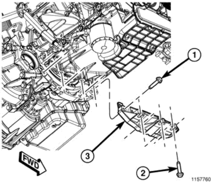
Fig. 175: Structural Collar Courtesy of CHRYSLER LLC
