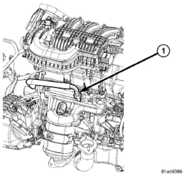
Fig. 314: Exhaust Gas Recirculation Tube Courtesy of CHRYSLER LLC
