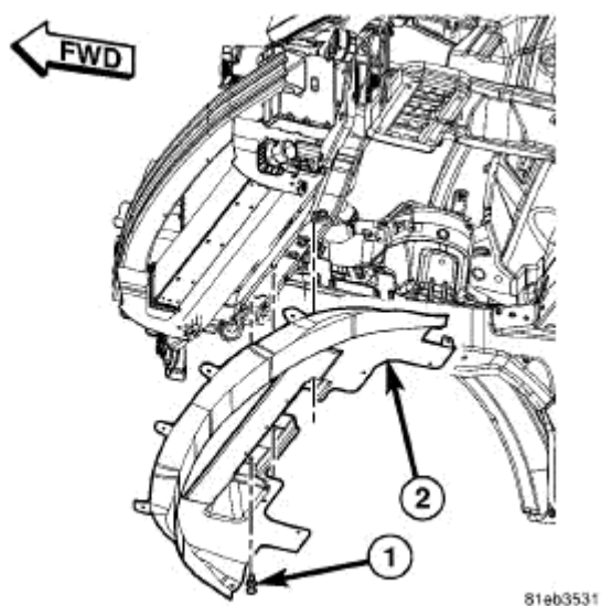
Fig. 10: Lower Fascia Closeout Panel Courtesy of CHRYSLER LLC
