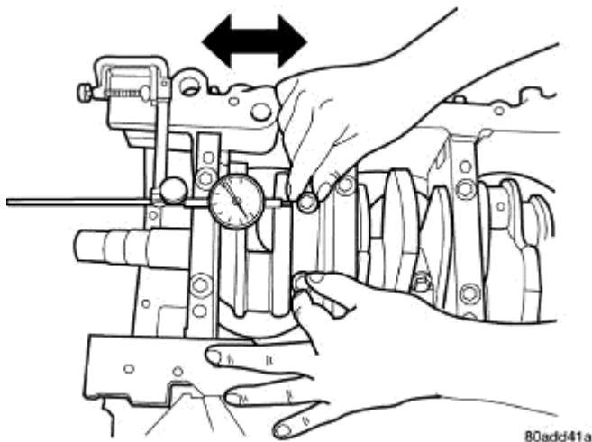
Fig. 168: Connecting Rod Side Clearance Measuring Courtesy of CHRYSLER LLC
