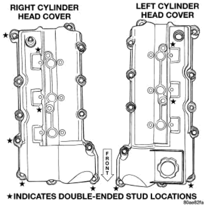
Fig. 105: Cylinder Head Covers Courtesy of CHRYSLER LLC
