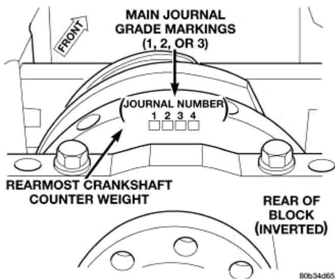
Fig. 170: Crankshaft Main Journal Grade Marking Location Courtesy of CHRYSLER LLC
