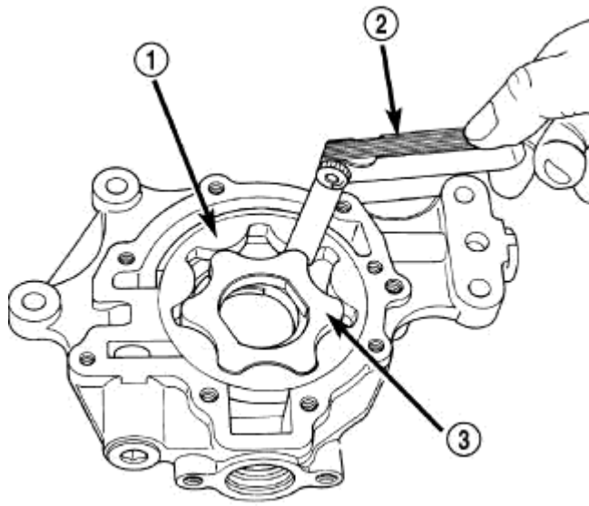
Fig. 282: MEASURING CLEARANCE BETWEEN ROTORS Courtesy of CHRYSLER LLC
