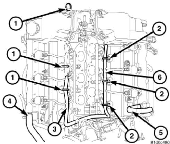
Fig. 124: Engine Harness Retaining Clips Courtesy of CHRYSLER LLC
