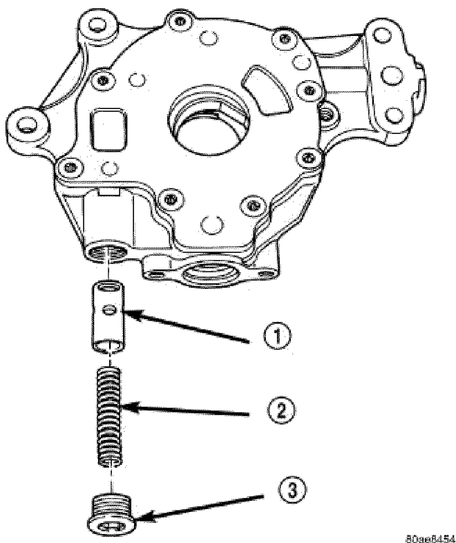
Fig. 276: Oil Pressure Relief Valve Courtesy of CHRYSLER LLC
