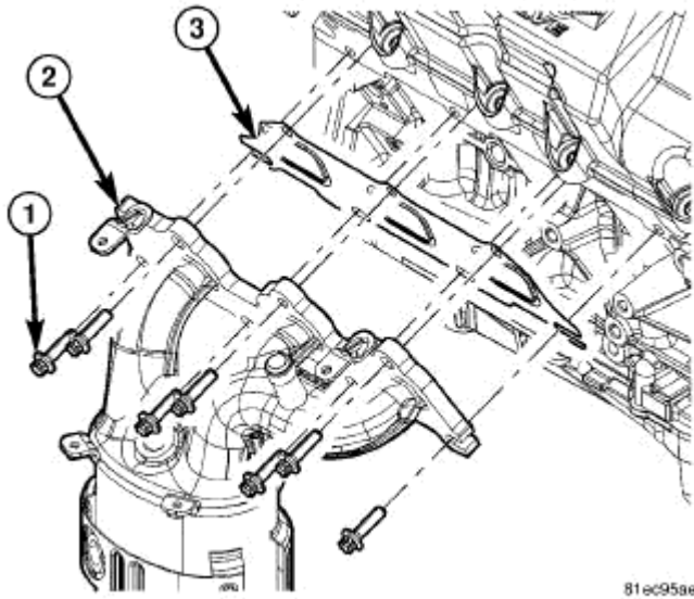
Fig. 311: Rear Maniverter Fasteners Courtesy of CHRYSLER LLC
