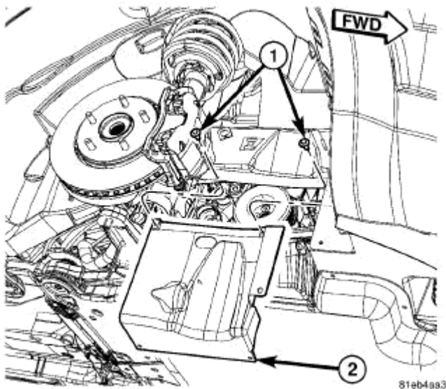
Fig. 261: Right Lower Splash Shield
