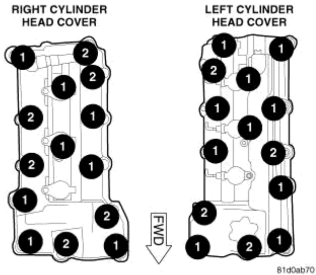
Fig. 119: Cylinder Head Cover Fasteners Courtesy of CHRYSLER LLC
