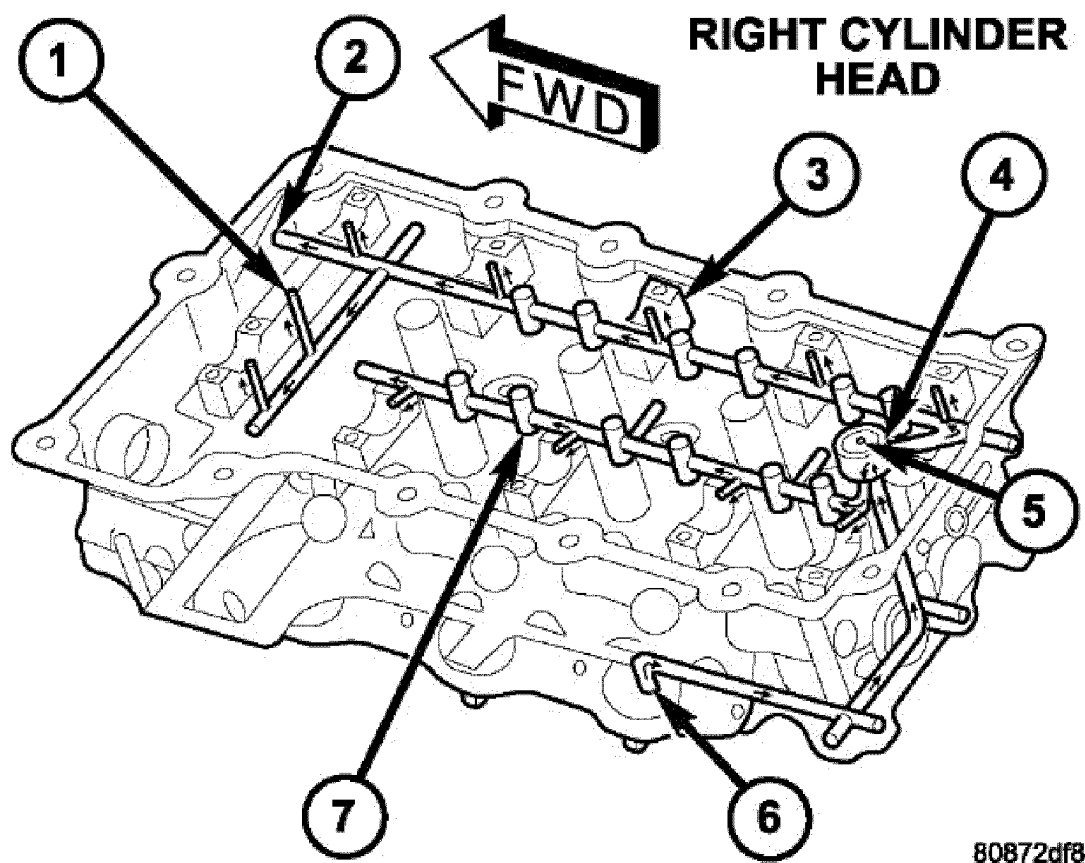
Fig. 249: Cylinder Head Oil Lubrication System - Right Side Courtesy of CHRYSLER LLC
