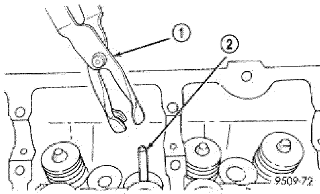
Fig. 139: Valve Stem Seal-Removal/Installation
