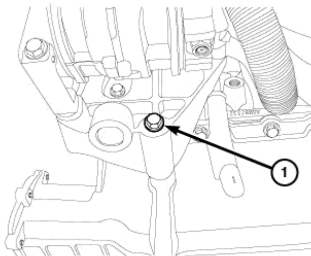
Fig. 268: A/C Compressor Mounting Bracket Lower Bolt Courtesy of CHRYSLER LLC
