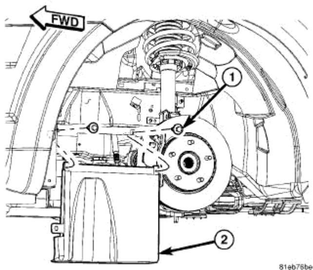
Fig. 8: Left Lower Splash Shield Courtesy of CHRYSLER LLC
