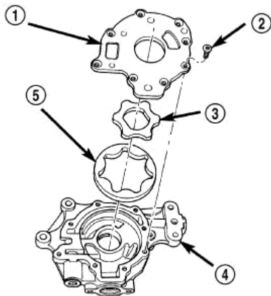
Fig. 277: Oil Pump
