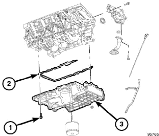
Fig. 266: Oil Pan Attaching Fasteners Courtesy of CHRYSLER LLC
