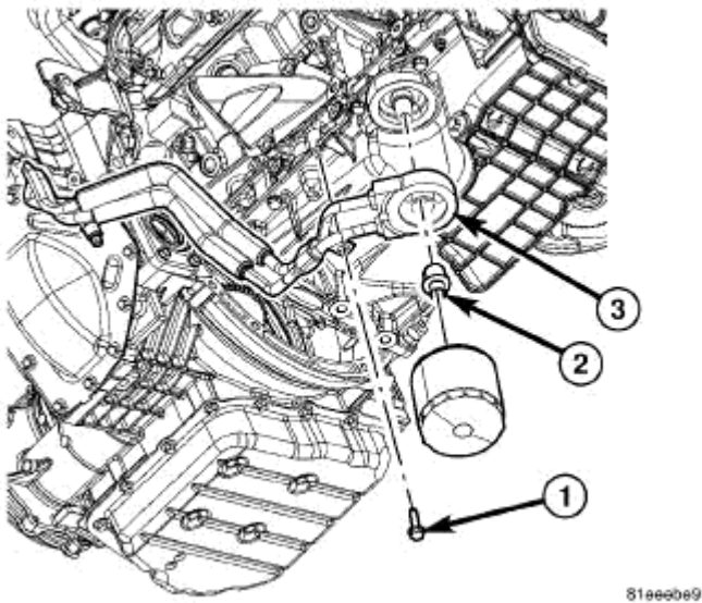
Fig. 252: Cooler Line Retaining Bracket Fastener Courtesy of CHRYSLER LLC
