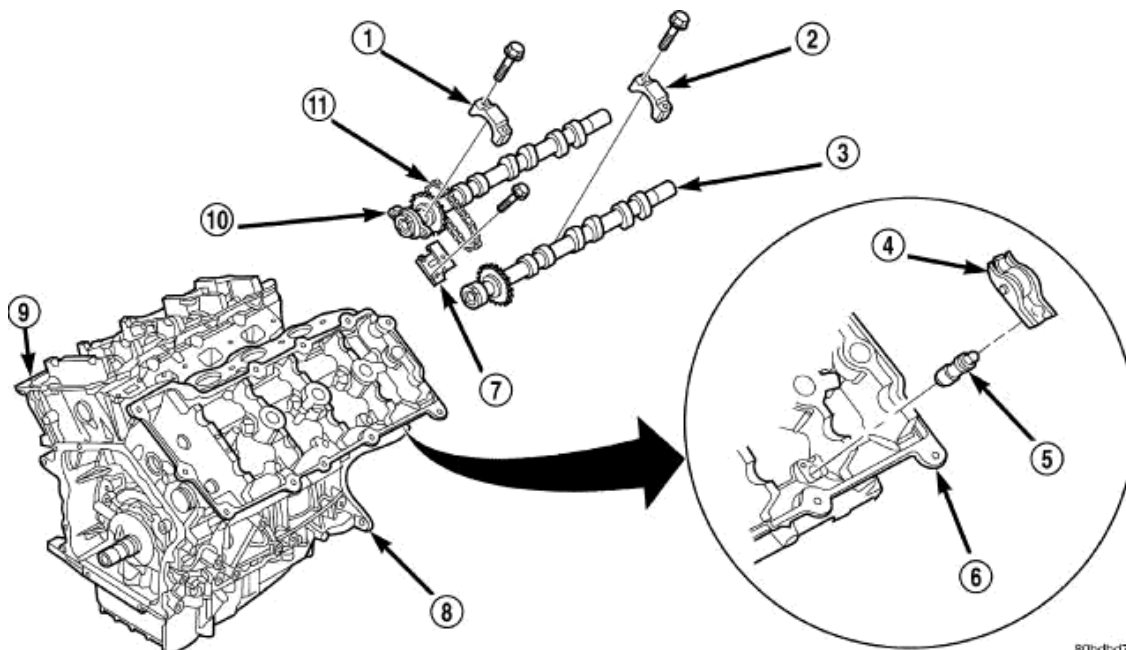
Fig. 108: Camshaft & Valvetrain Components Courtesy of CHRYSLER LLC
