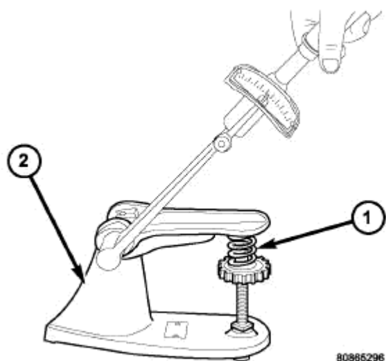
Fig. 145: TESTING VALVE SPRING
