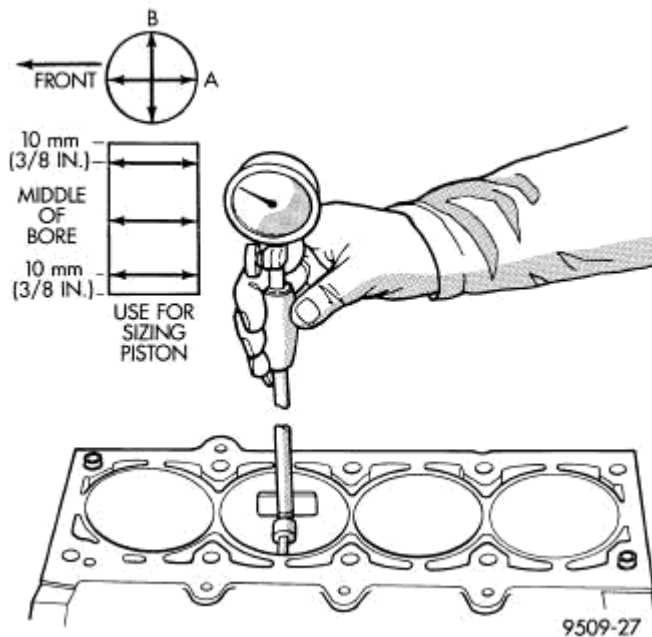
Fig. 165: Checking Cylinder Bore Size Courtesy of CHRYSLER LLC
