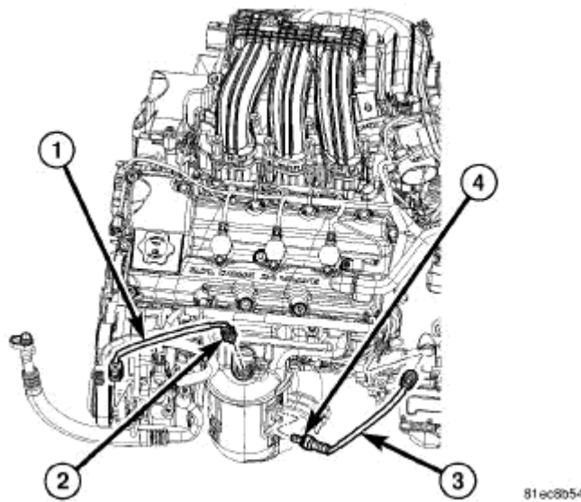
Fig. 303: Oxygen Sensors Courtesy of CHRYSLER LLC
