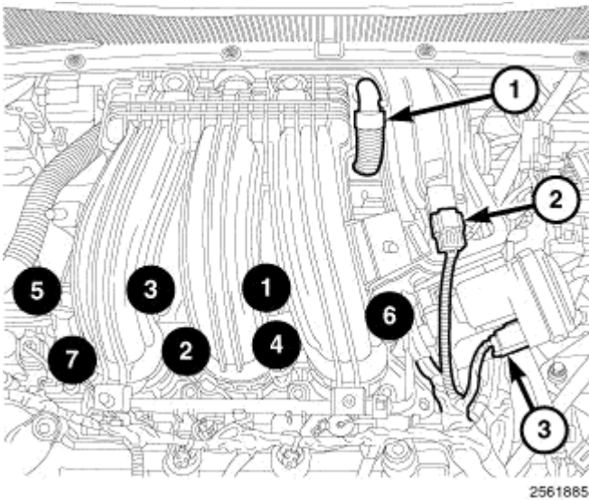
Fig. 325: Locating Manifold Bolts, Manifold Absolute Pressure Sensor & Electronic Throttle Control Electrical Connectors
