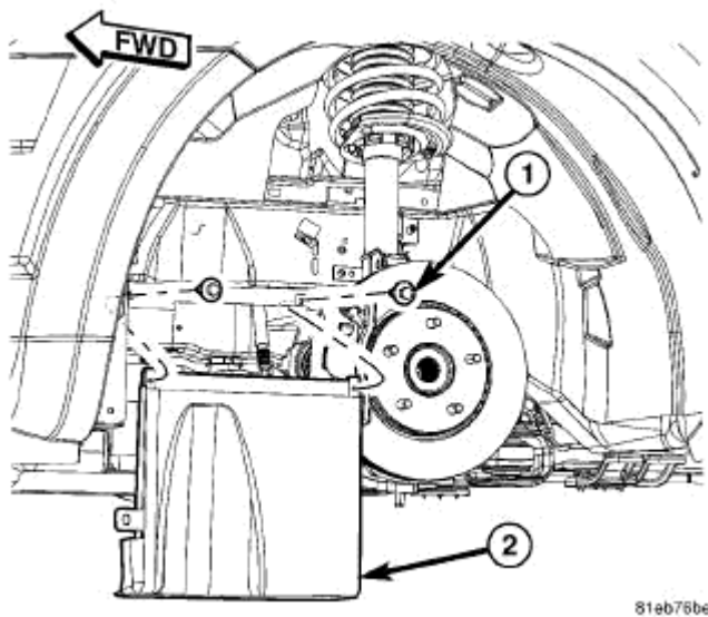
Fig. 51: Left Lower Splash Shield Courtesy of CHRYSLER LLC
