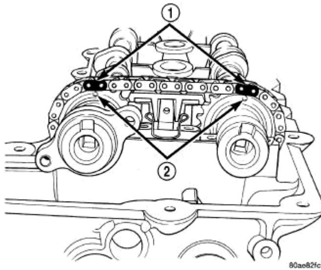
Fig. 115: Camshaft Chain Timing Courtesy of CHRYSLER LLC
