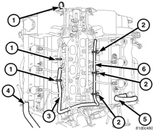
Fig. 120: Engine Harness Retaining Clips Courtesy of CHRYSLER LLC
