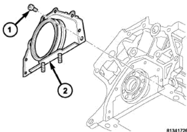
Fig. 217: Oil Seal Retainer Courtesy of CHRYSLER LLC
