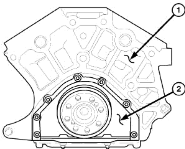
Fig. 216: REAR MAIN SEAL-INSTALLED Courtesy of CHRYSLER LLC
