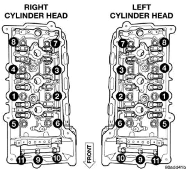
Fig. 99: Cylinder Head Tightening Sequence
