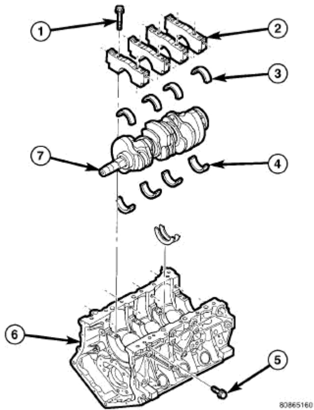
Fig. 183: Cylinder Block & Crankshaft Courtesy of CHRYSLER LLC
