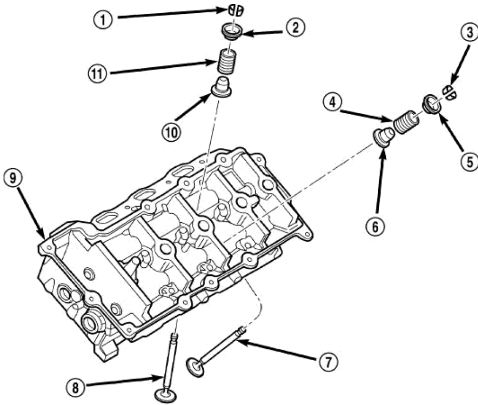
Fig. 144: Cylinder Head, Valves & Springs Courtesy of CHRYSLER LLC
