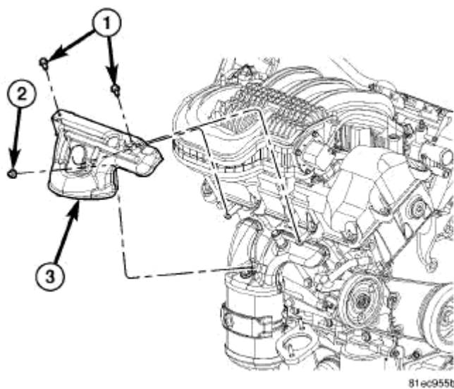
Fig. 308: Rear Manifold Heat Shield Courtesy of CHRYSLER LLC
