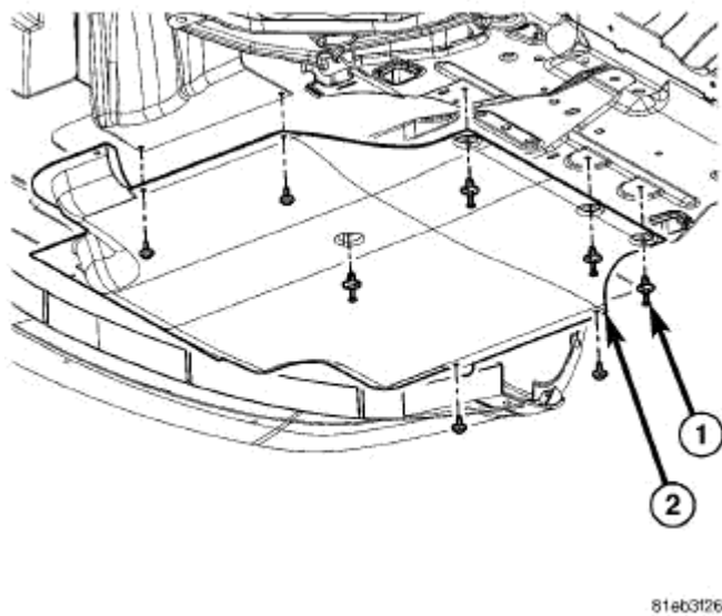
Fig. 233: Belly Pan Courtesy of CHRYSLER LLC
