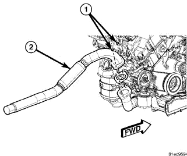
Fig. 293: Exhaust Extension Pipe Courtesy of CHRYSLER LLC
