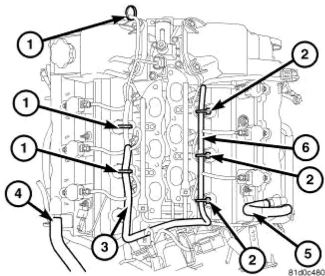
Fig. 130: Engine Harness Retaining Clips Courtesy of CHRYSLER LLC
