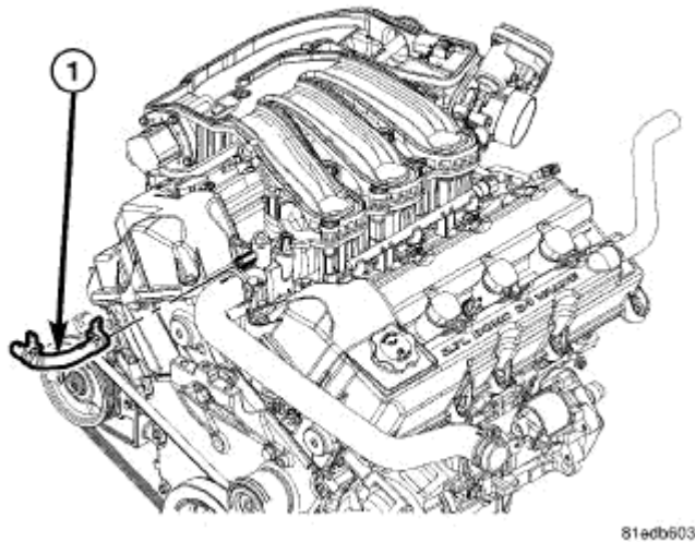
Fig. 37: Coolant Pressure Bottle Coolant Hose Courtesy of CHRYSLER LLC
