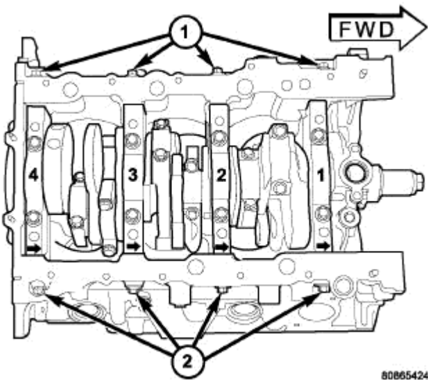
Fig. 193: Main Bearing Cap Identification Courtesy of CHRYSLER LLC
