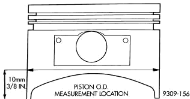
Fig. 207: Piston Measurements Courtesy of CHRYSLER LLC
