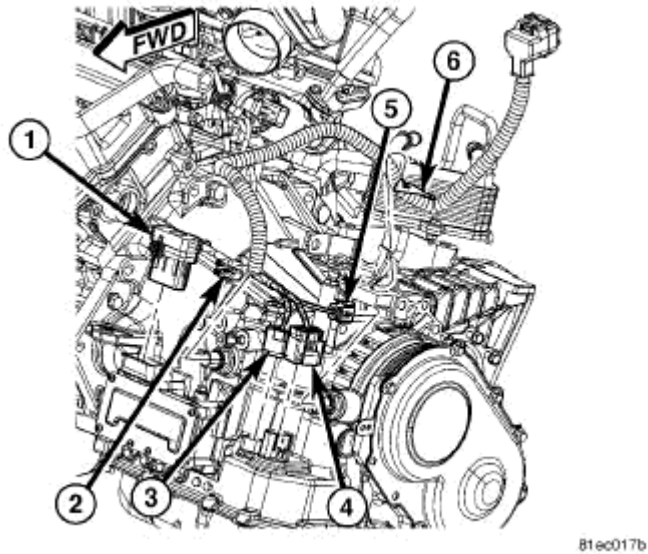
Fig. 49: Transmission Control Module Harness Connector Courtesy of CHRYSLER LLC
