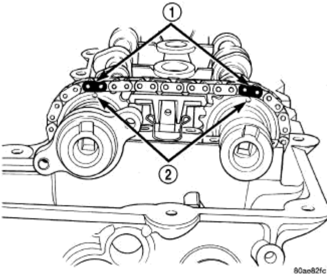
Fig. 112: Camshaft Chain Timing Courtesy of CHRYSLER LLC
