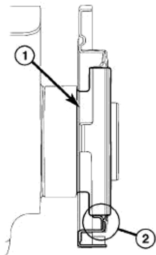
Fig. 218: REAR SEAL INSTALLED Courtesy of CHRYSLER LLC
