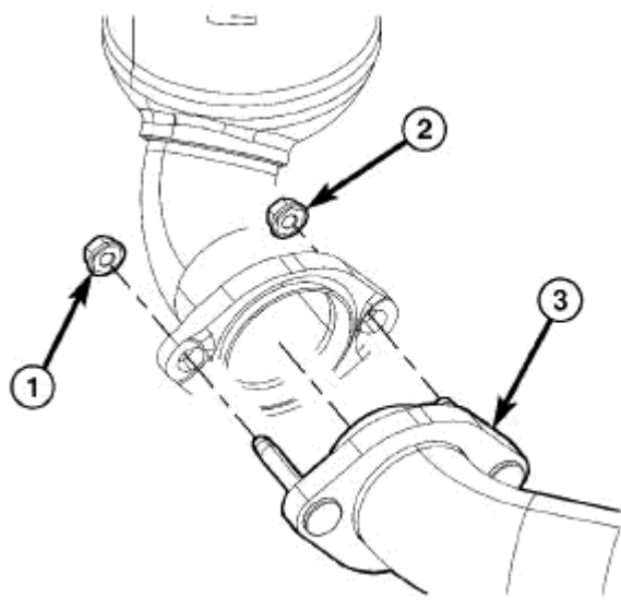
Fig. 298: Front Maniverter-To-Cross Under Fasteners
