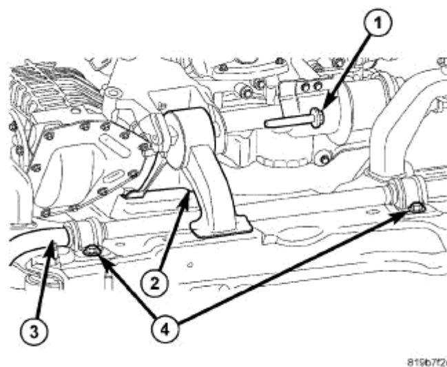
Fig. 39: Rear Engine Mount & Transaxle Bracket
