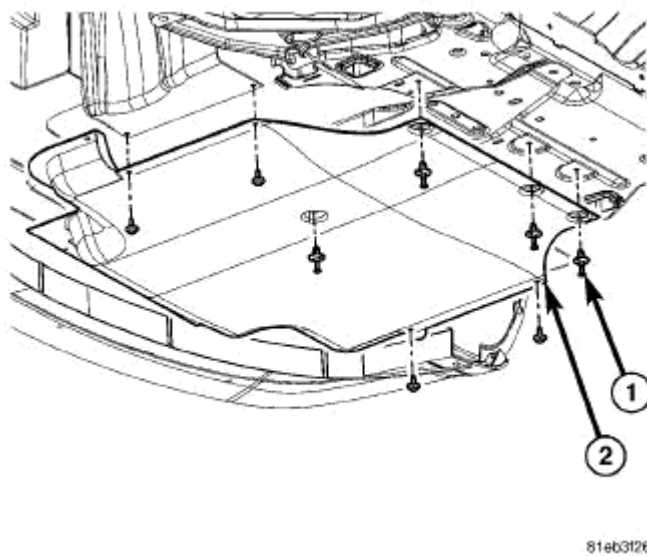
Fig. 177: Belly Pan Courtesy of CHRYSLER LLC
