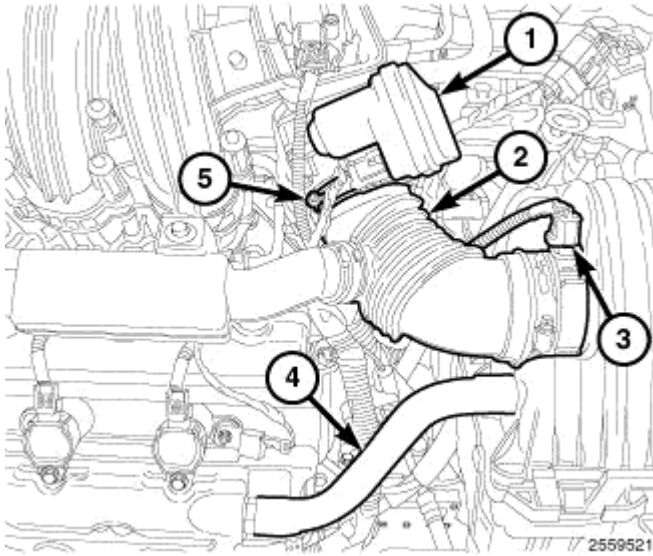
Fig. 328: Identifying Air Makeup Hose, Throttle Body & Air Inlet Hose Courtesy of CHRYSLER LLC
