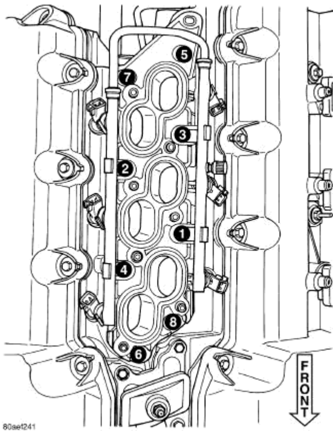
Fig. 329: Lower Intake Manifold Tightening Sequence Courtesy of CHRYSLER LLC
