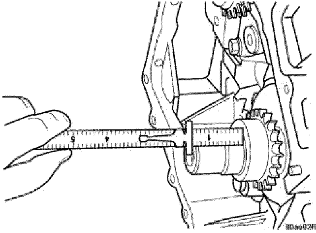
Fig. 348: Crankshaft Sprocket Depth Measurement Courtesy of CHRYSLER LLC
