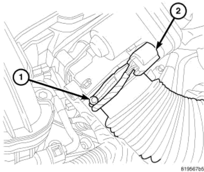
Fig. 148: Air Cleaner Housing & Inlet Hose Courtesy of CHRYSLER LLC
