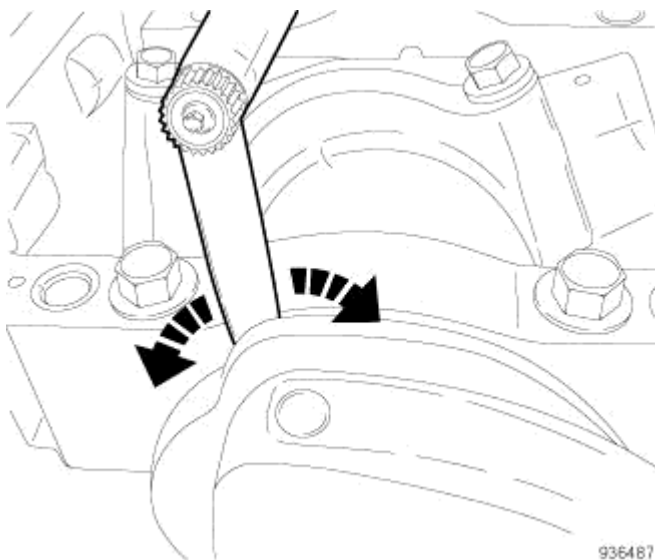
Fig. 188: Sliding Feeler Gauge Side-To-Side Across Bearing Cap Courtesy of CHRYSLER LLC
