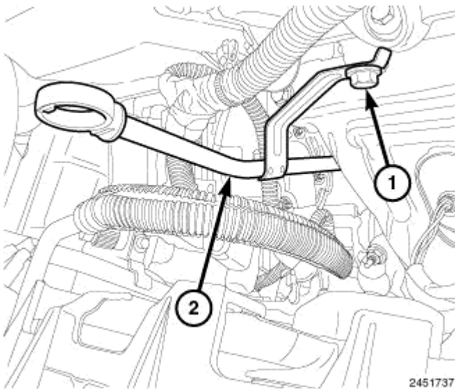
Fig. 259: Identifying Oil Dipstick Tube & Bolt Courtesy of CHRYSLER LLC
