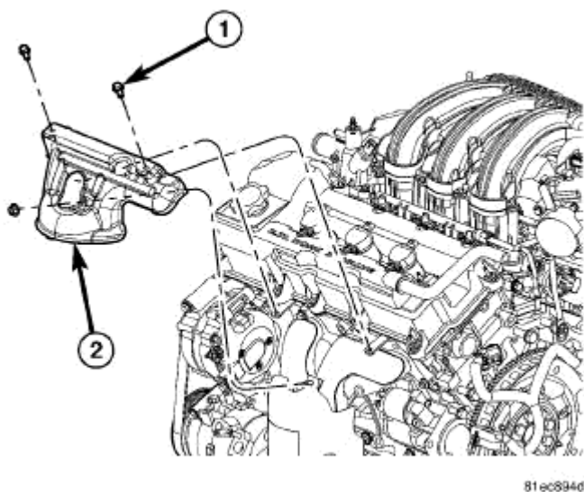
Fig. 296: Upper Manifold Heat Shield Courtesy of CHRYSLER LLC
