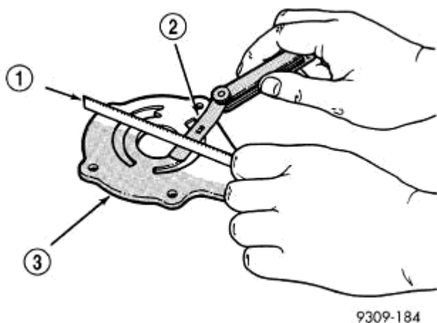
Fig. 278: CHECKING OIL PUMP COVER FLATNESS - TYPICAL Courtesy of CHRYSLER LLC
