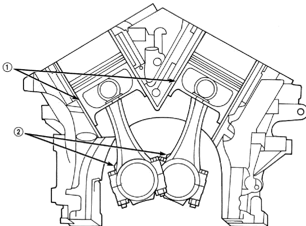
Fig. 211: Piston & Connecting Rod Positioning (Front View of Engine) Courtesy of CHRYSLER LLC
