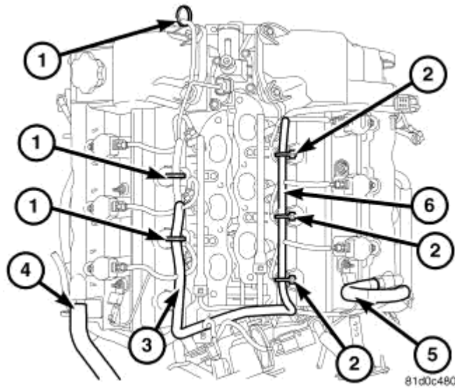
Fig. 125: Engine Harness Retaining Clips Courtesy of CHRYSLER LLC
