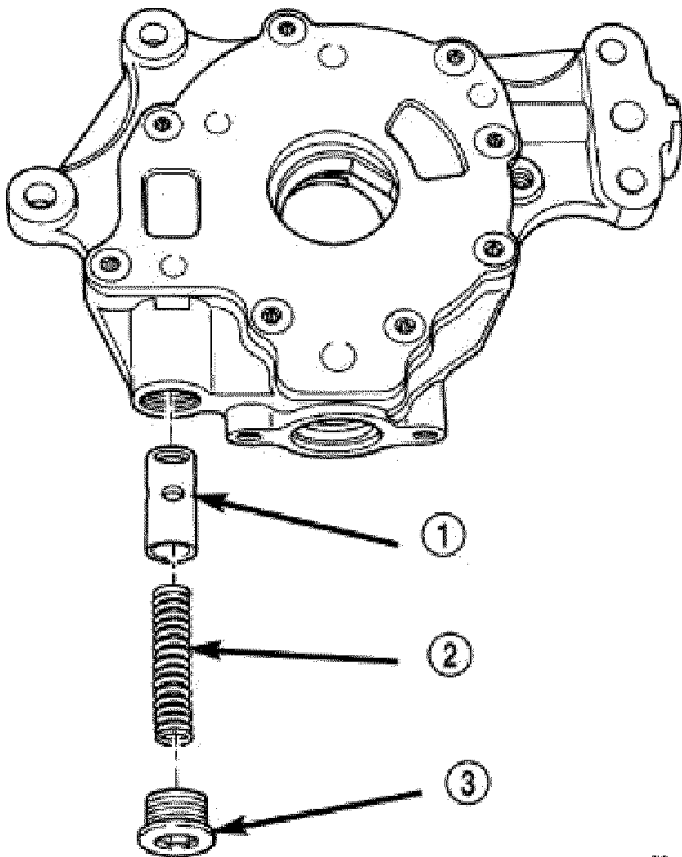
Fig. 286: Oil Pressure Relief Valve Courtesy of CHRYSLER LLC
