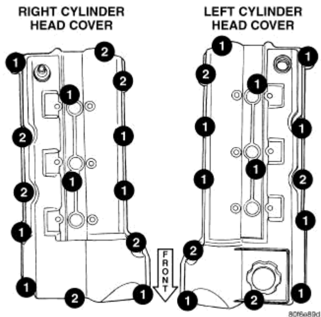
Fig. 142: Cylinder Head Cover Fasteners Courtesy of CHRYSLER LLC
