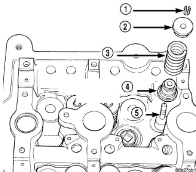
Fig. 157: Valve Seal & Spring Courtesy of CHRYSLER LLC
