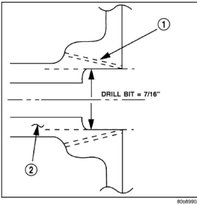
Fig. 317: MANIFOLD PORT (NIPPLE) REPAIR Courtesy of CHRYSLER LLC
