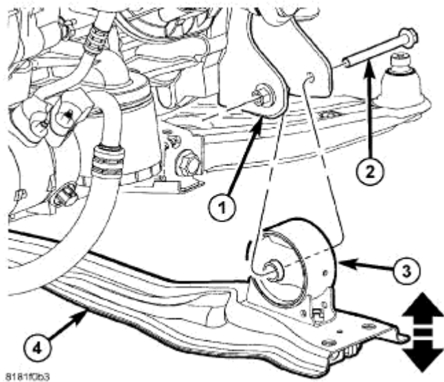
Fig. 241: Front Engine Mount Through Bolt Courtesy of CHRYSLER LLC
