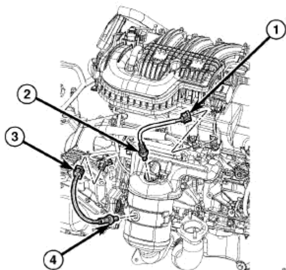
Fig. 306: Oxygen Sensors
