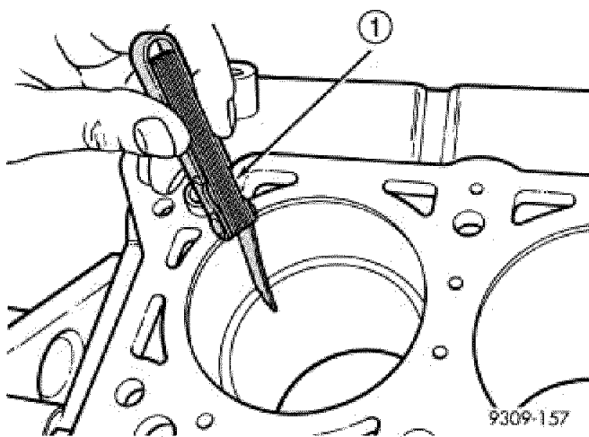
Fig. 200: CHECK GAP ON PISTON RINGS
