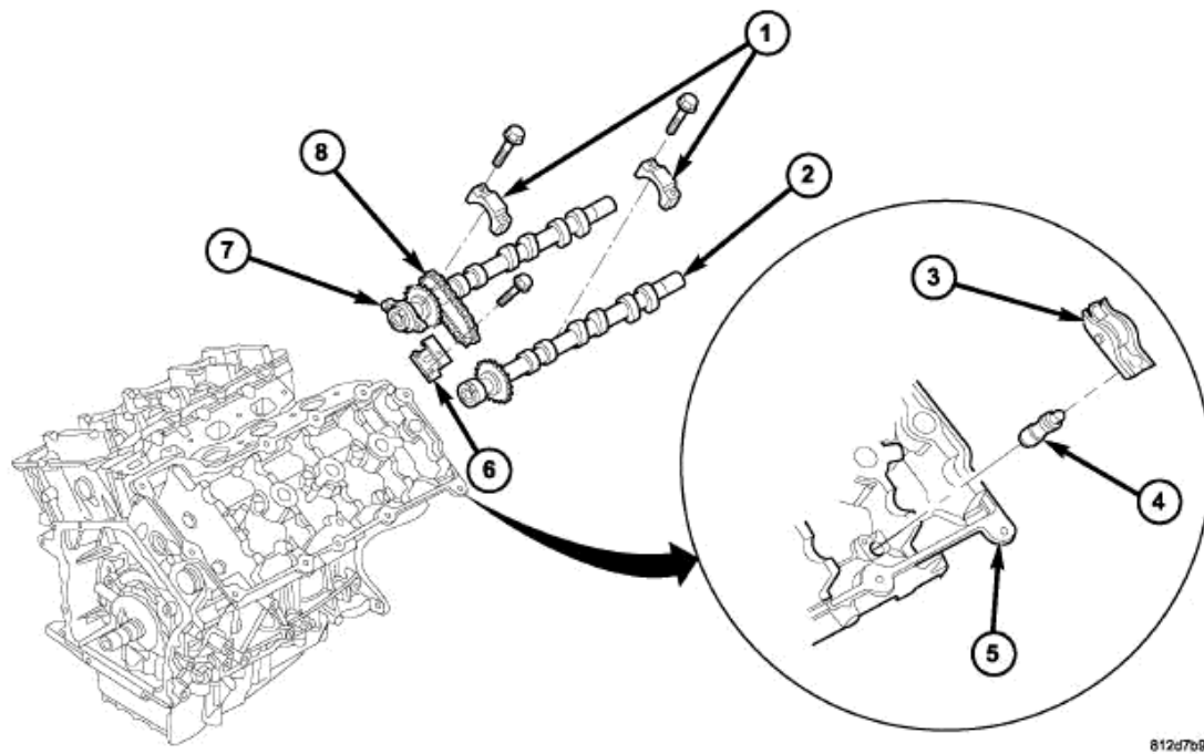
Fig. 110: Camshaft & Valvetrain Components Courtesy of CHRYSLER LLC
