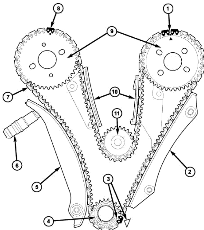
Fig. 339: TIMING CHAIN ALIGNMENT MARKS - PRIMARY Courtesy of CHRYSLER LLC
