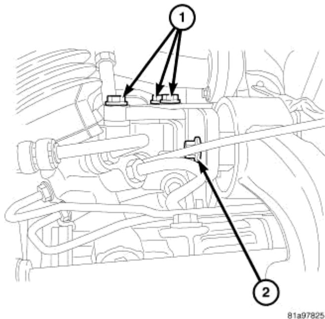
Fig. 239: Identifying Rear Mount Bracket-To-Transaxle Case Bolts Courtesy of CHRYSLER LLC
