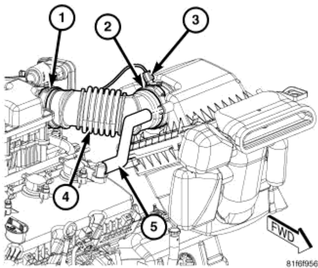
Fig. 87: Inlet Air Temperature Sensor Electrical Connector Courtesy of CHRYSLER LLC
