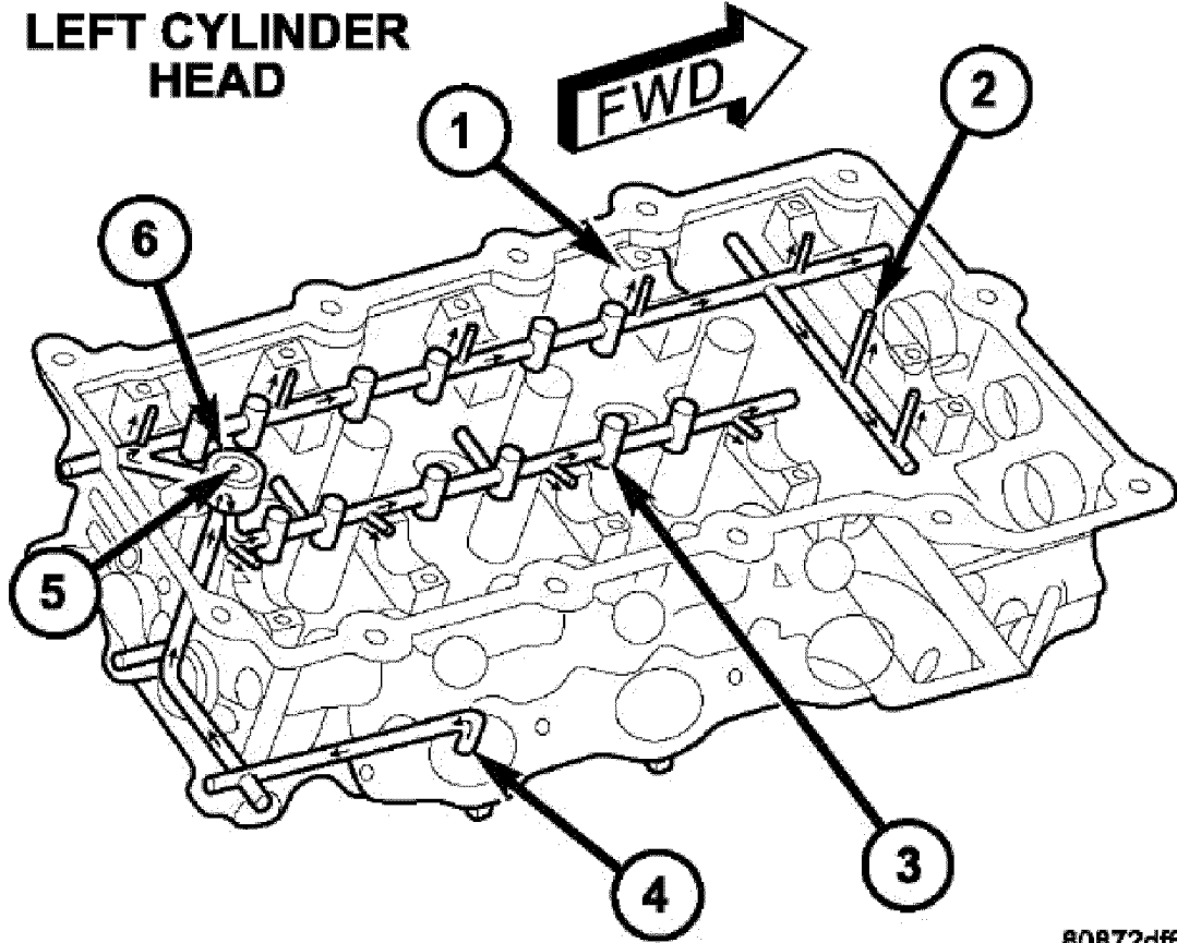
Fig. 248: Cylinder Head Oil Lubrication System - Left Side Courtesy of CHRYSLER LLC
