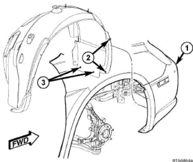
Fig. 354: Removing/Installing Front Splash Shields Courtesy of CHRYSLER LLC
