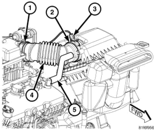
Fig. 90: Inlet Air Temperature Sensor Electrical Connector Courtesy of CHRYSLER LLC
