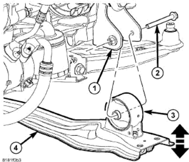
Fig. 236: Front Engine Mount Through Bolt Courtesy of CHRYSLER LLC
