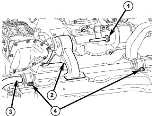
Fig. 23: Rear Engine Mount & Transaxle Bracket
