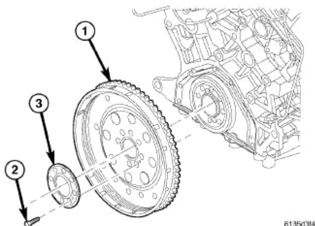
Fig. 221: Flex Plate
