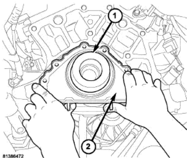
Fig. 219: REAR MAIN INSTALLATION
