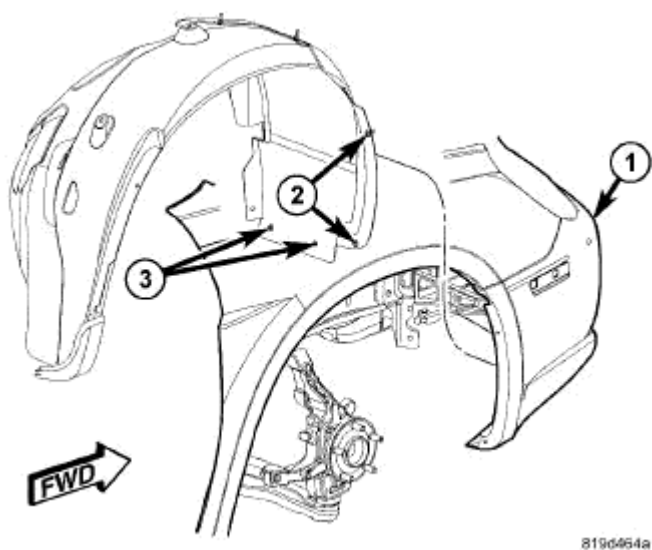
Fig. 349: FRONT SPLASH SHIELDS
