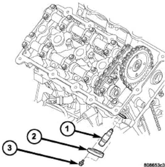
Fig. 341: PRIMARY TIMING CHAIN TENSIONER Courtesy of CHRYSLER LLC
