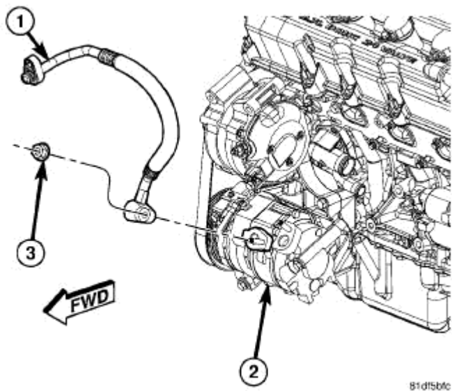
Fig. 13: A/C Discharge Line At Compressor Courtesy of CHRYSLER LLC
