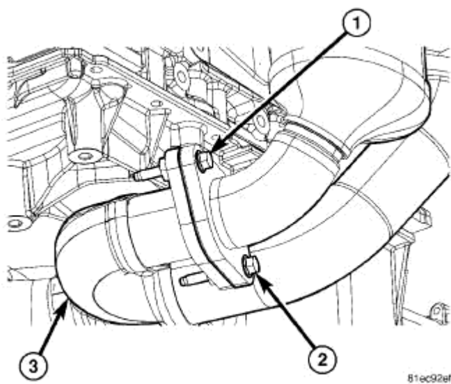
Fig. 309: Exhaust Cross-Under Pipe Courtesy of CHRYSLER LLC
