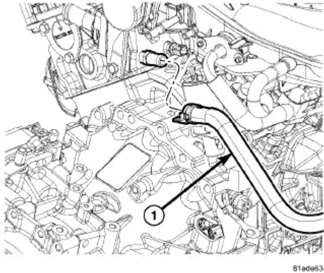
Fig. 26: Heater Hose From Engine Coolant Outlet Courtesy of CHRYSLER LLC
