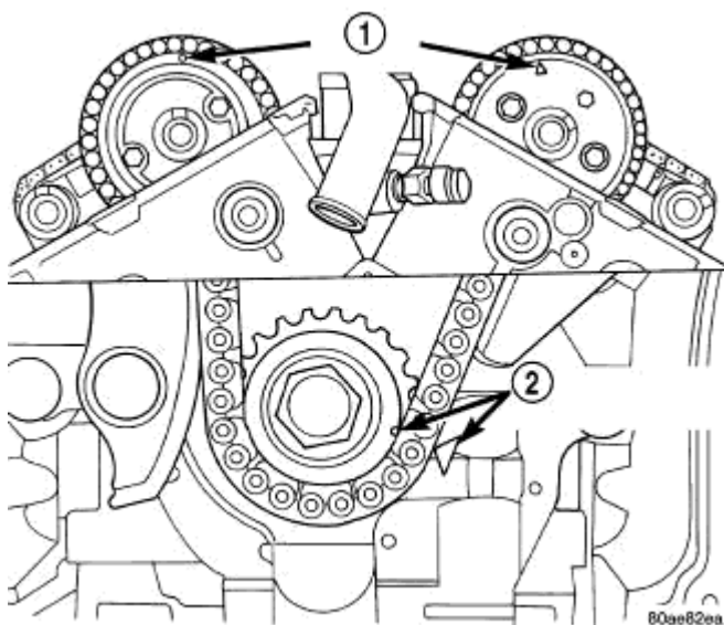
Fig. 334: TIMING MARK ALIGNMENT Courtesy of CHRYSLER LLC
