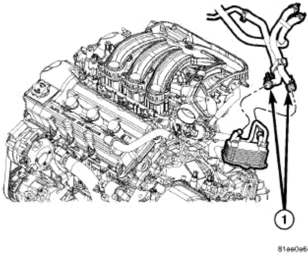
Fig. 27: Oil Cooler Lines Courtesy of CHRYSLER LLC
