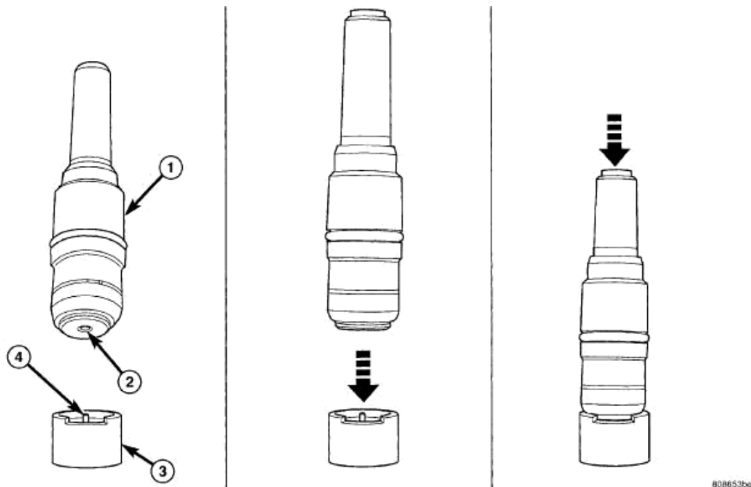
Fig. 340: TIMING CHAIN TENSIONER - OIL PURGING Courtesy of CHRYSLER LLC
