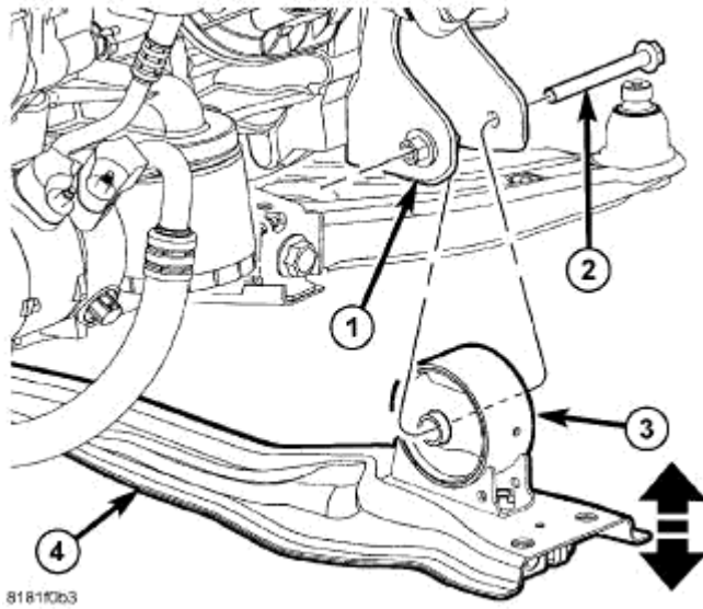
Fig. 271: Front Engine Mount Through Bolt Courtesy of CHRYSLER LLC
