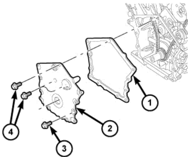
Fig. 351: TIMING CHAIN COVER
