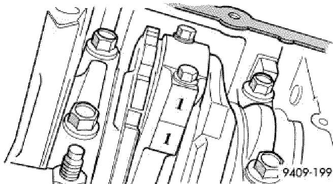
Fig. 208: Identify Connecting Rod to Cylinder Courtesy of CHRYSLER LLC
