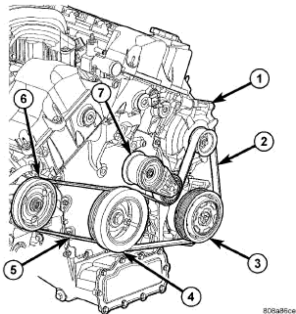
Fig. 93: Accessory Drive Belt System - 2.7L Courtesy of CHRYSLER LLC
