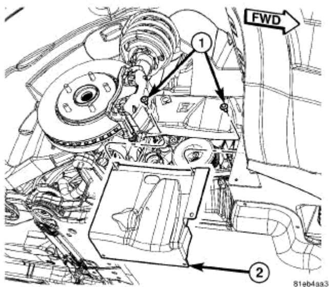
Fig. 9: Right Lower Splash Shield Courtesy of CHRYSLER LLC
