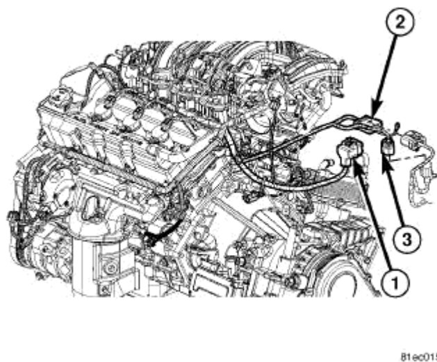
Fig. 48: Engine Electrical Harnesses Connectors Courtesy of CHRYSLER LLC
