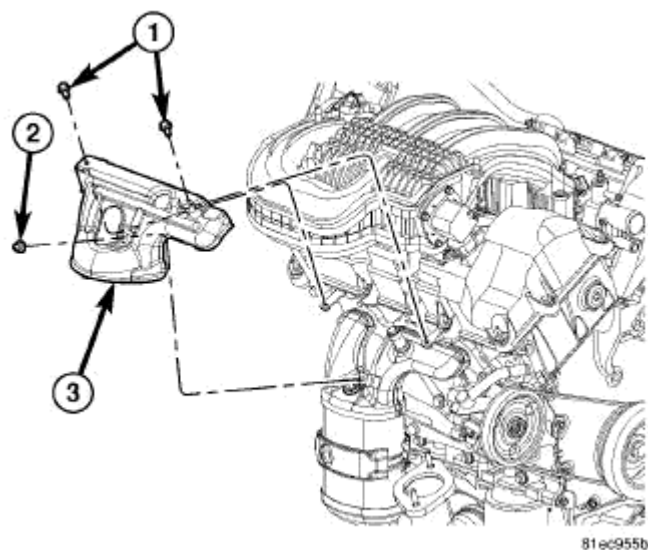
Fig. 313: Rear Manifold Heat Shield Courtesy of CHRYSLER LLC
