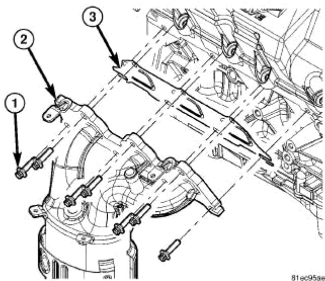
Fig. 310: Rear Maniverter Fasteners Courtesy of CHRYSLER LLC
