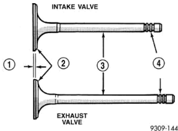
Fig. 159: Intake & Exhaust Valves Courtesy of CHRYSLER LLC
