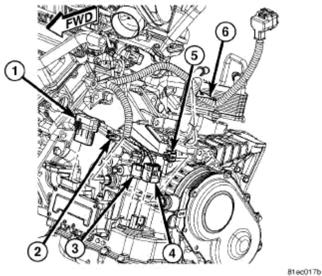
Fig. 12: Transmission Control Module Harness Connector Courtesy of CHRYSLER LLC
