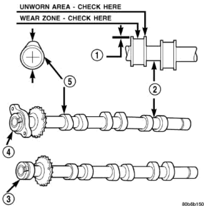
Fig. 111: Camshaft Inspection Courtesy of CHRYSLER LLC
