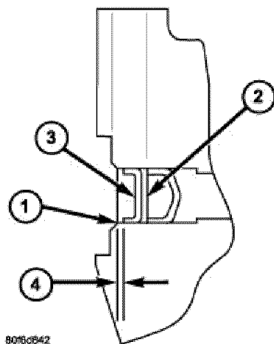
Fig. 92: Oil Gallery Cup Plug Courtesy of CHRYSLER LLC
