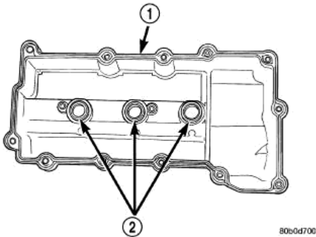
Fig. 122: Cylinder Head Cover Gasket & Spark Plug Seals Courtesy of CHRYSLER LLC
