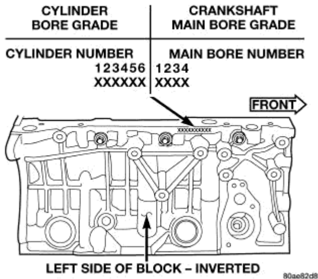
Fig. 169: Cylinder Block Main Bore Grade Marking Courtesy of CHRYSLER LLC
