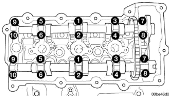
Fig. 103: Camshaft Bearing Cap Tightening Sequence Courtesy of CHRYSLER LLC
