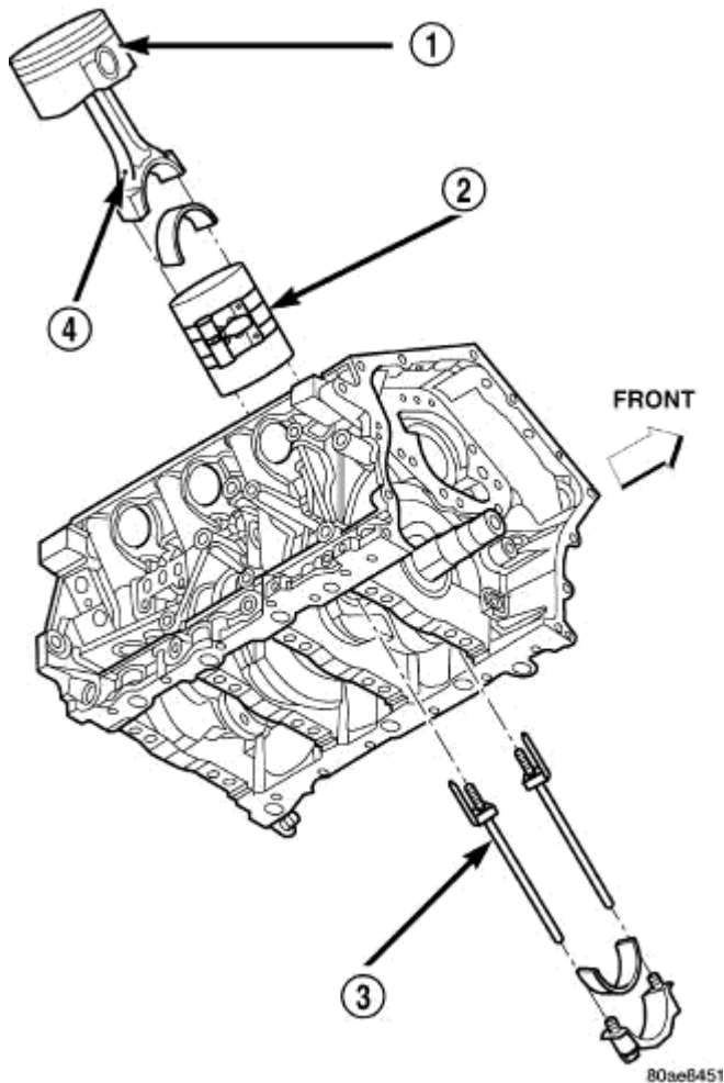
Fig. 210: Piston & Connecting Rod Courtesy of CHRYSLER LLC
