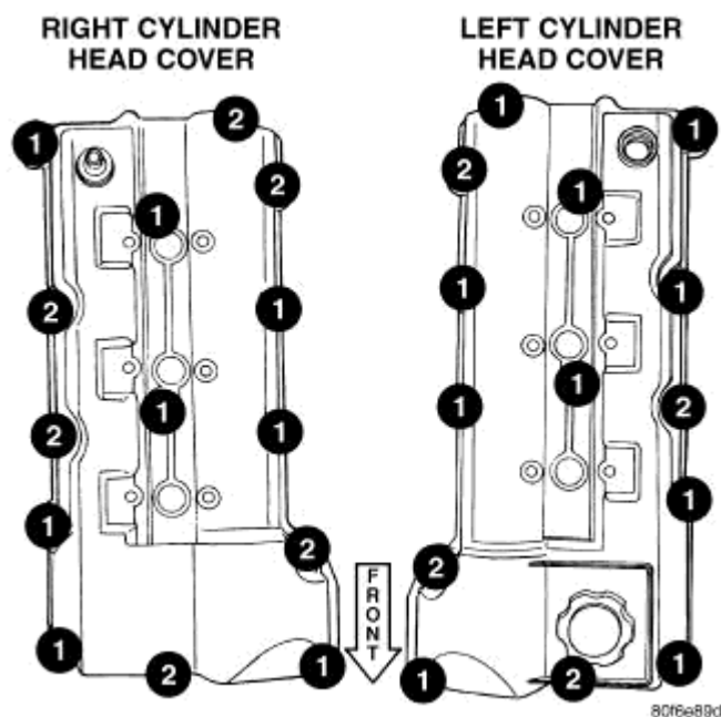
Fig. 147: Cylinder Head Cover Fasteners Courtesy of CHRYSLER LLC
