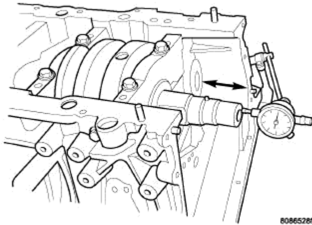
Fig. 190: CHECKING CRANKSHAFT END PLAY Courtesy of CHRYSLER LLC
