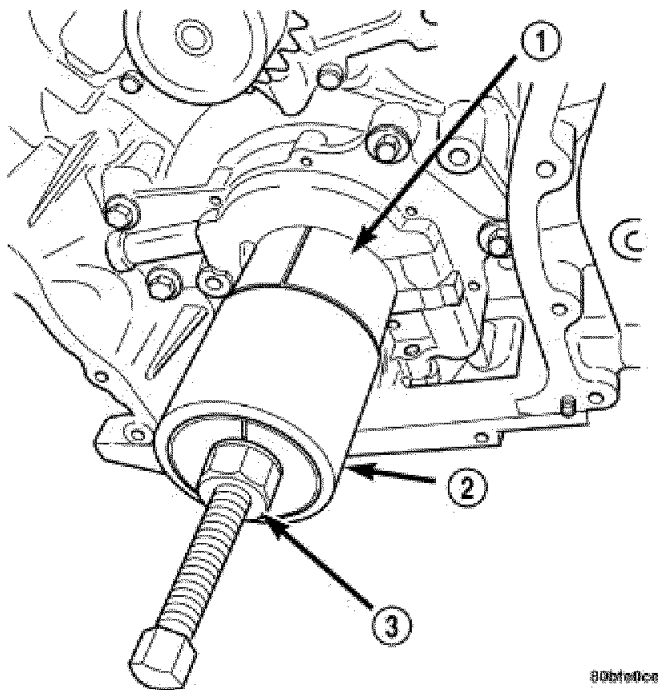
Fig. 337: Crankshaft Sprocket - Removal Courtesy of CHRYSLER LLC
