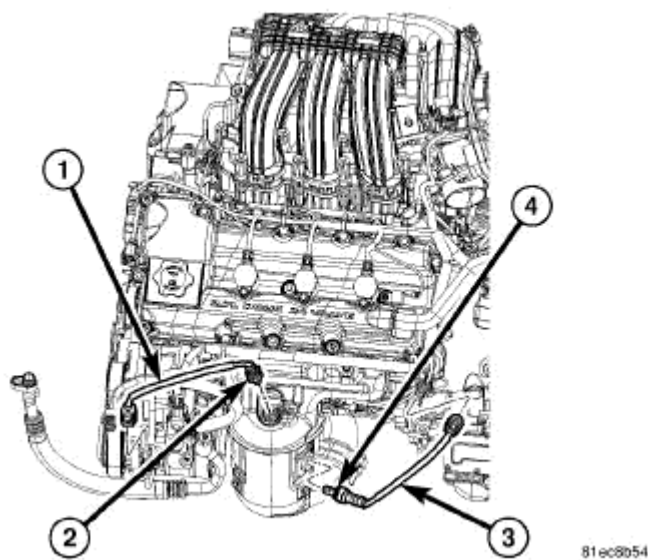
Fig. 295: Oxygen Sensors Courtesy of CHRYSLER LLC
