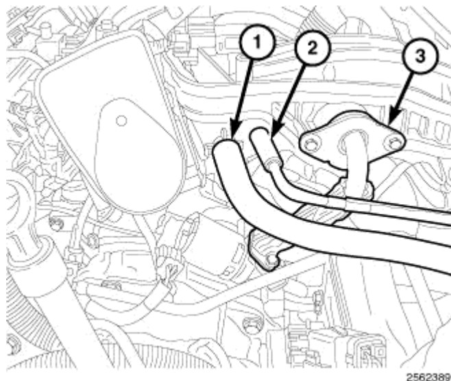
Fig. 326: Locating Upper Exhaust Gas Recirculation Tube, Brake Booster Hose & Vapor Purge Hose
