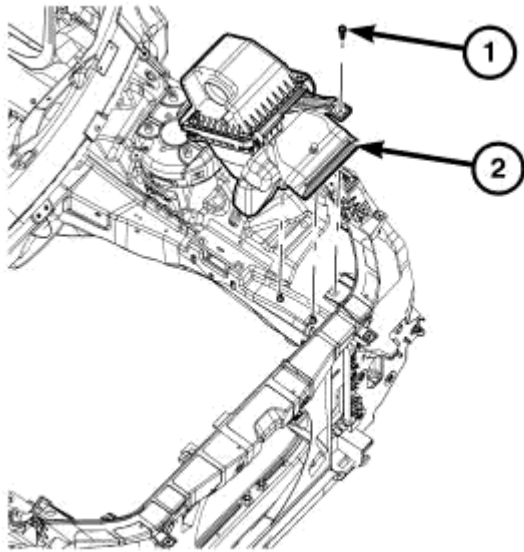
Fig. 88: Retainer From Bracket Courtesy of CHRYSLER LLC
