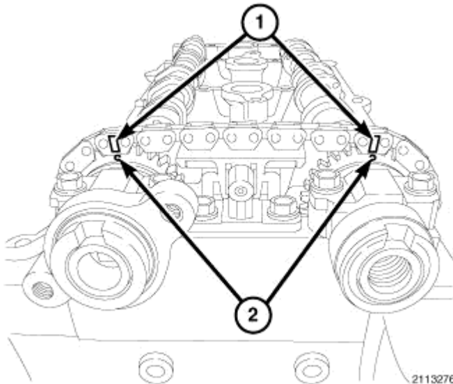
Fig. 113: Identifying Marked Links & Timing Dot On Camshaft Sprockets Courtesy of CHRYSLER LLC
