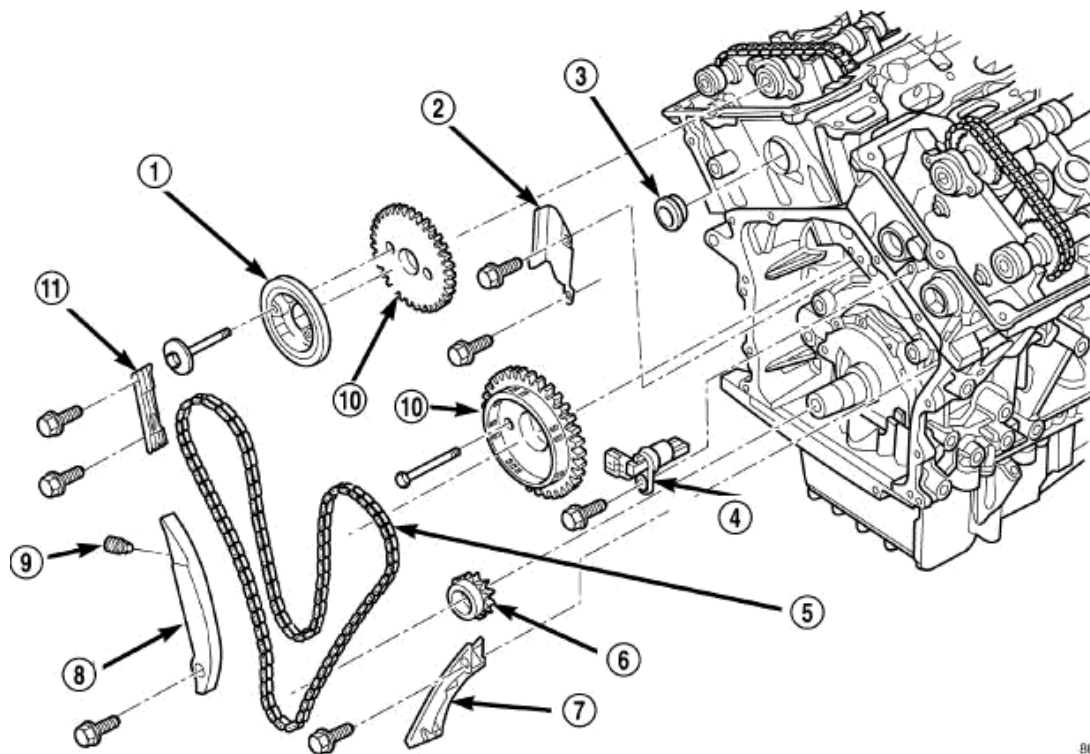
Fig. 336: TIMING DRIVE SYSTEM - PRIMARY Courtesy of CHRYSLER LLC
