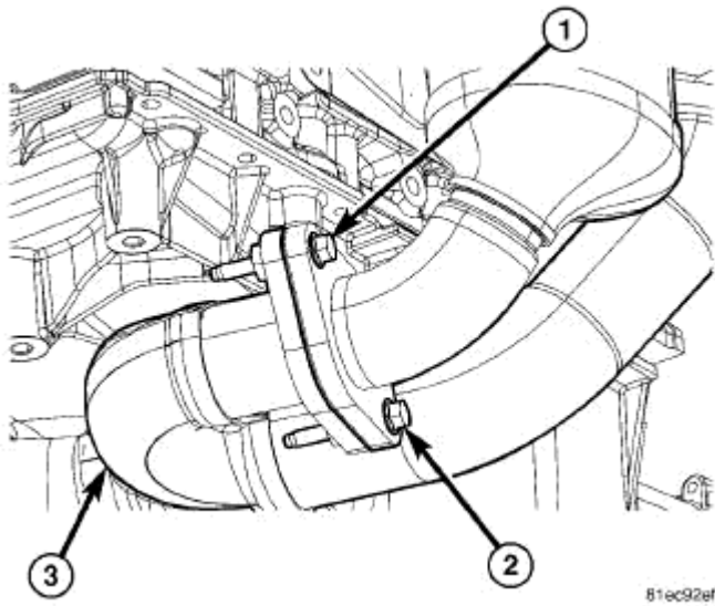
Fig. 269: Exhaust Cross-Under Pipe Courtesy of CHRYSLER LLC
