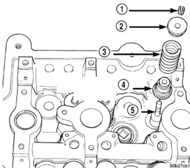
Fig. 150: Valve Seal & Spring Courtesy of CHRYSLER LLC
