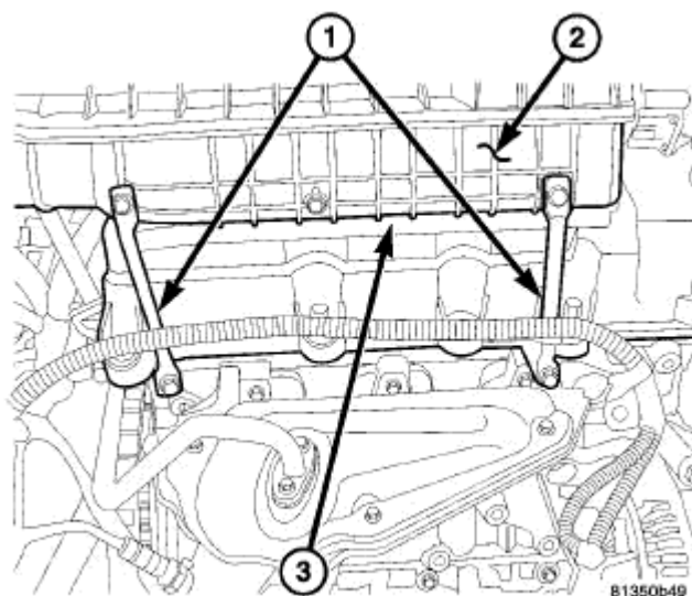
Fig. 327: Intake Brackets
