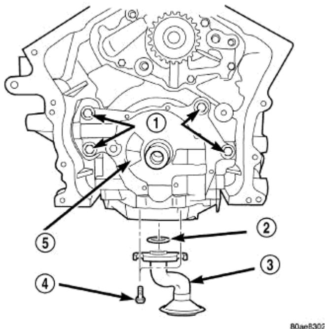
Fig. 275: Oil Pump & Pick-up Tube Courtesy of CHRYSLER LLC
