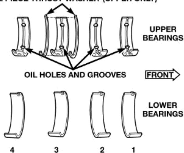
Fig. 184: Main Bearing Identification Courtesy of CHRYSLER LLC
