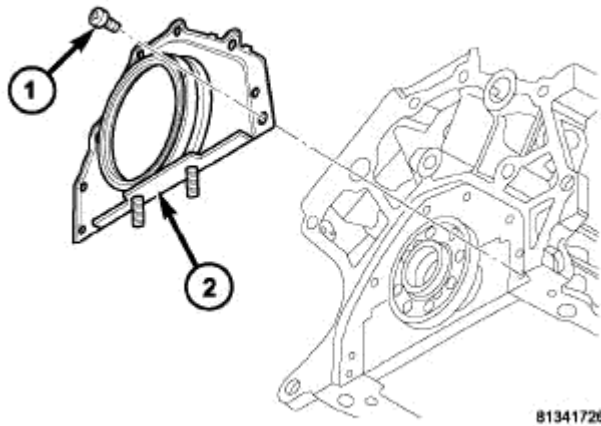
Fig. 180: Oil Seal Retainer
