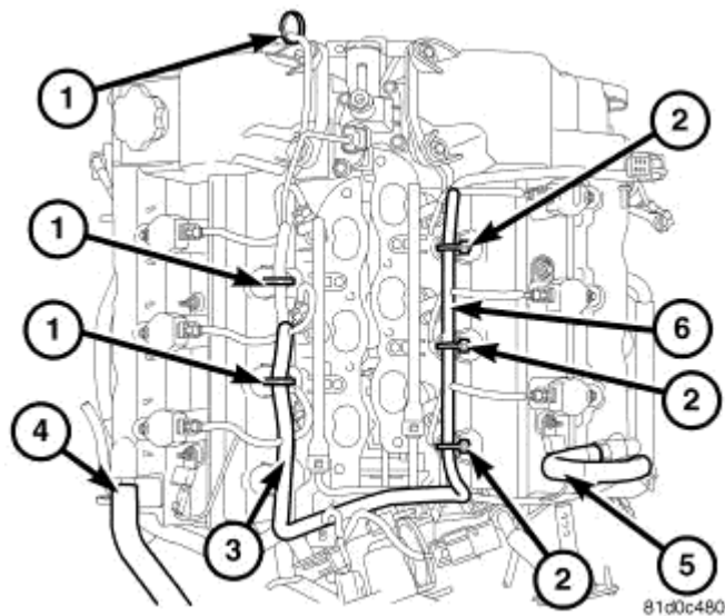
Fig. 118: Engine Harness Retaining Clips Courtesy of CHRYSLER LLC
