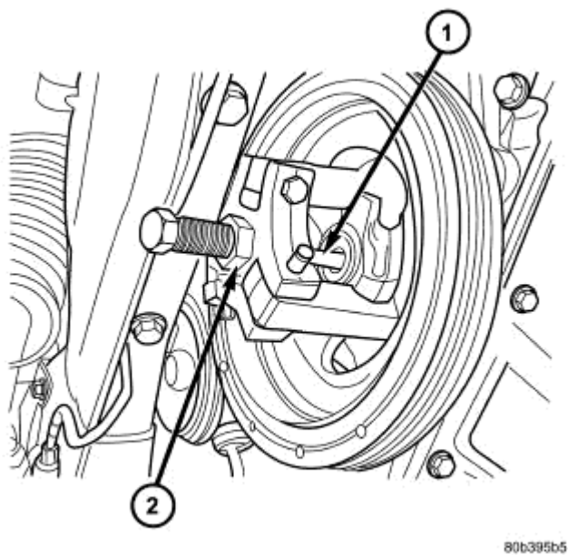
Fig. 196: Vibration Damper - Removal Courtesy of CHRYSLER LLC
