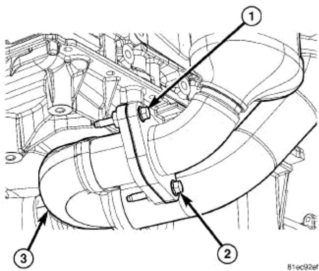
Fig. 264: Exhaust Cross-Under Pipe Courtesy of CHRYSLER LLC
