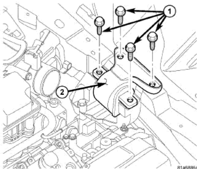
Fig. 229: Left Mount Vertical Bolts
