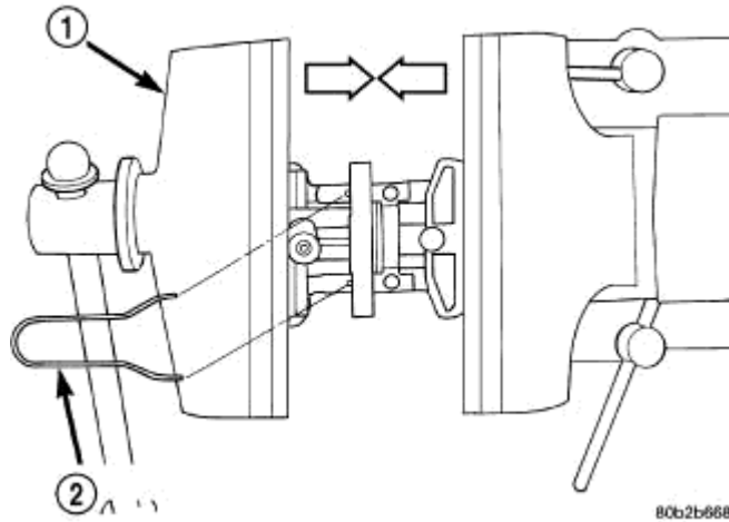
Fig. 114: Locking Camshaft (Secondary) Chain Tensioner Courtesy of CHRYSLER LLC
