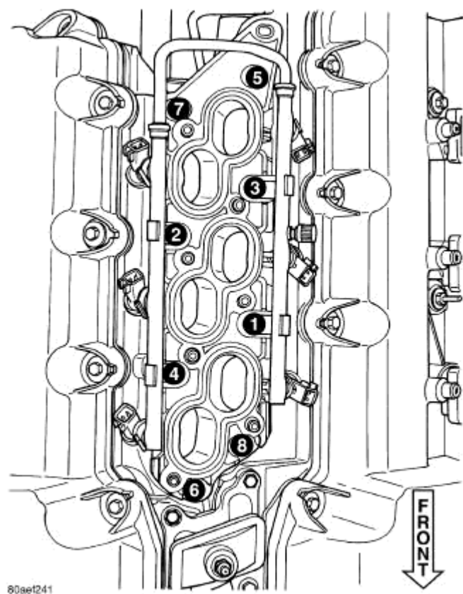
Fig. 106: Lower Intake Manifold Tightening Sequence Courtesy of CHRYSLER LLC
