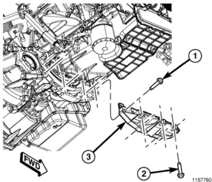
Fig. 174: Structural Collar Courtesy of CHRYSLER LLC
