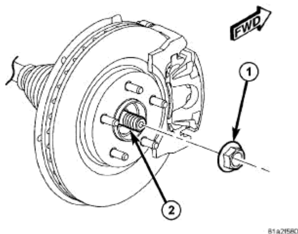
Fig. 47: Axle Shafts Hub Nut Courtesy of CHRYSLER LLC
