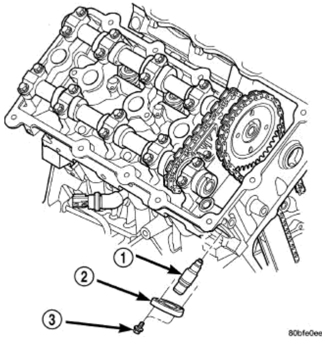
Fig. 335: PRIMARY TIMING CHAIN TENSIONER Courtesy of CHRYSLER LLC
