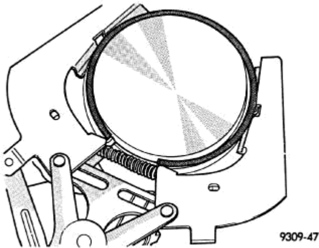
Fig. 204: Upper and Intermediate Rings - Installation Courtesy of CHRYSLER LLC
