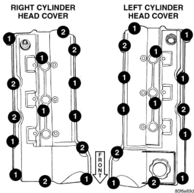
Fig. 132: Cylinder Head Cover Fasteners Courtesy of CHRYSLER LLC
