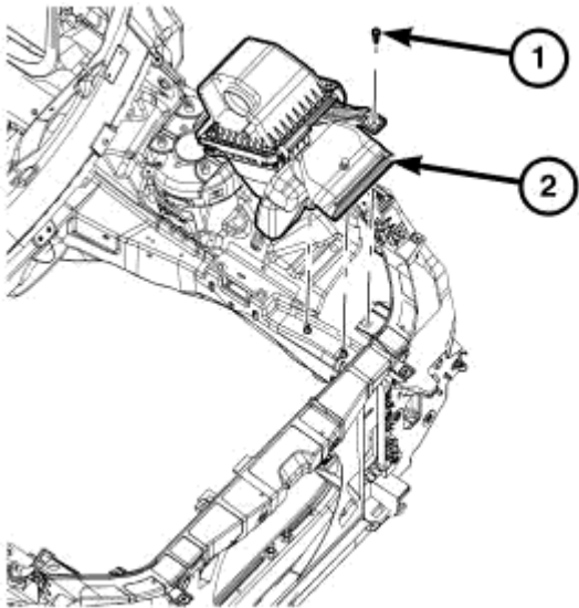
Fig. 89: Retainer From Bracket Courtesy of CHRYSLER LLC
