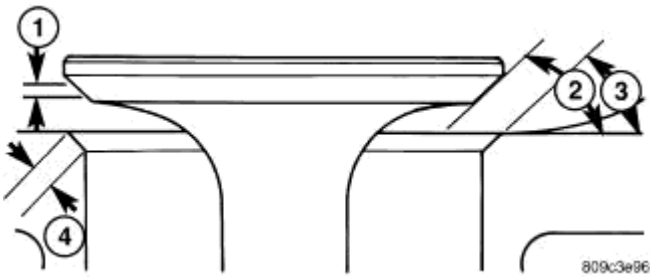
Fig. 154: Valve Face & Seat Courtesy of CHRYSLER LLC
