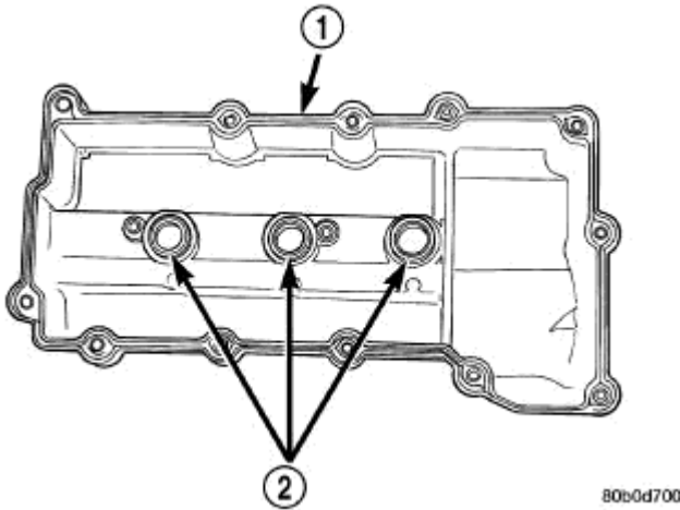
Fig. 121: Cylinder Head Cover Gasket & Spark Plug Seals
