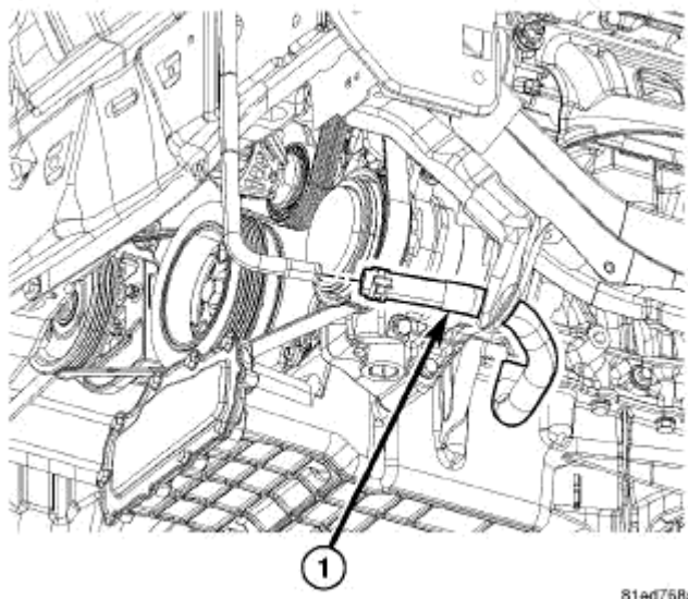
Fig. 20: Heater Return Hose Courtesy of CHRYSLER LLC
