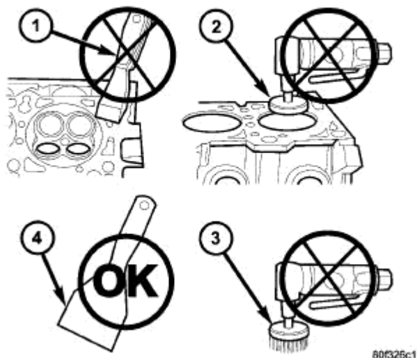
Fig. 4: PROPER TOOL USAGE FOR SURFACE PREPARATION
