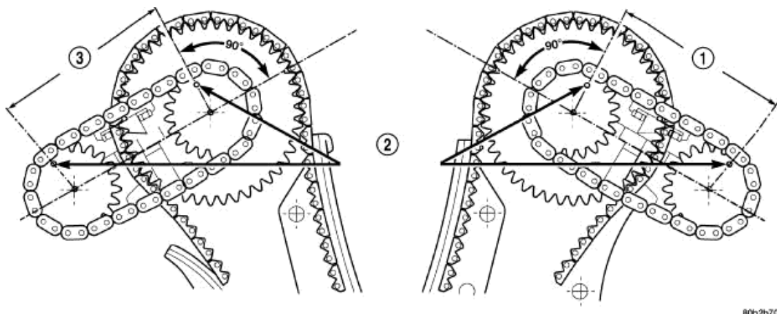
Fig. 333: ENGINE TIMING Courtesy of CHRYSLER LLC
