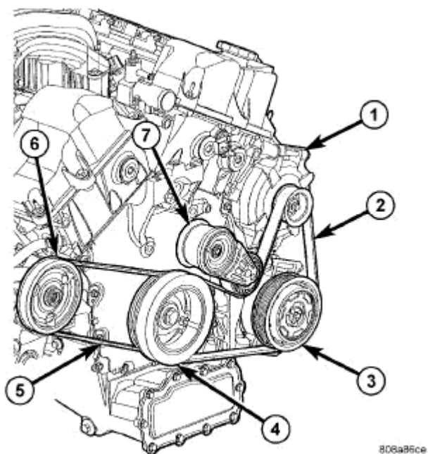
Fig. 350: Accessory Drive Belt System - 2.7L
