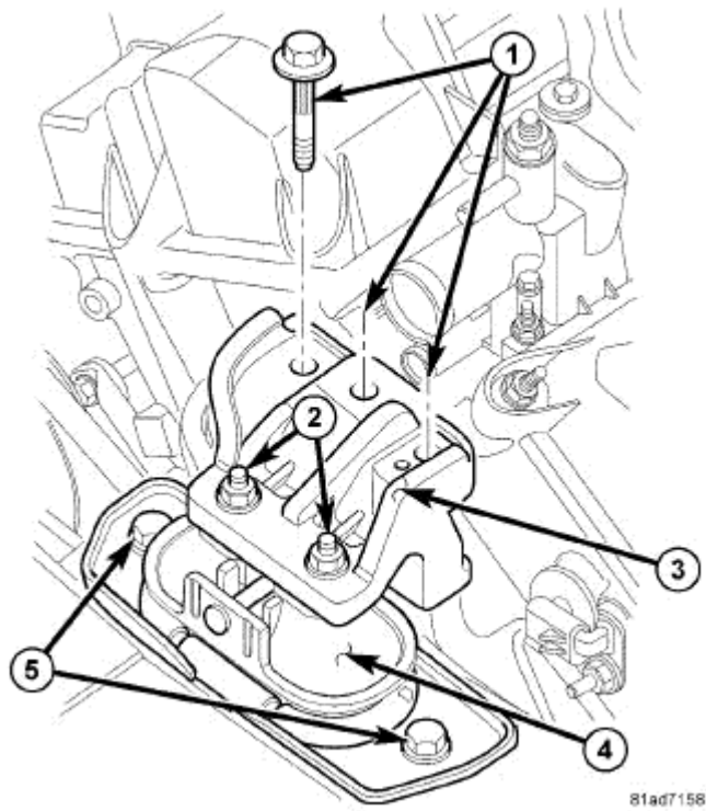
Fig. 244: Right Engine Mount Courtesy of CHRYSLER LLC
