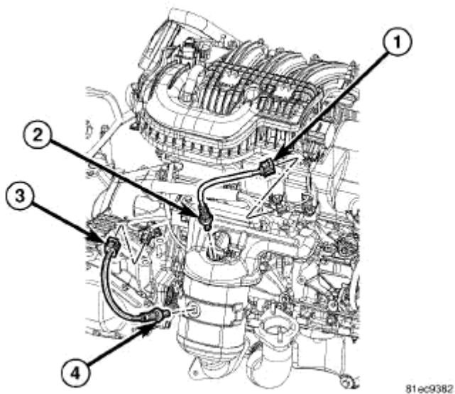
Fig. 315: Oxygen Sensors Courtesy of CHRYSLER LLC
