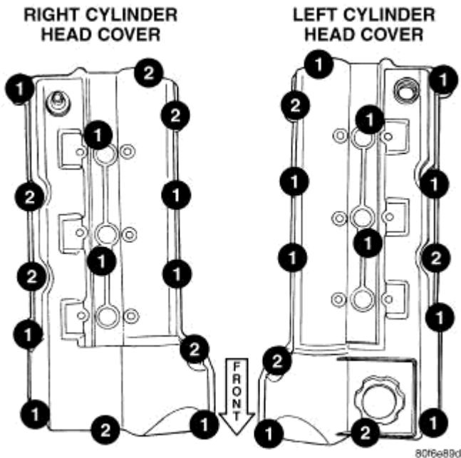
Fig. 134: Cylinder Head Cover Fasteners
