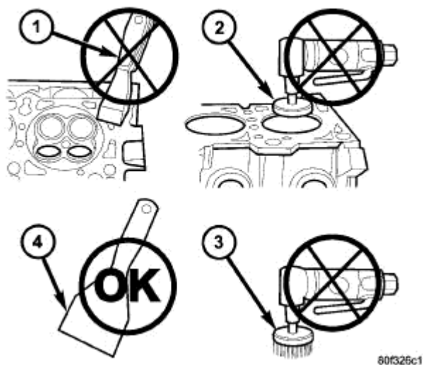
Fig. 5: PROPER TOOL USAGE FOR SURFACE PREPARATION
