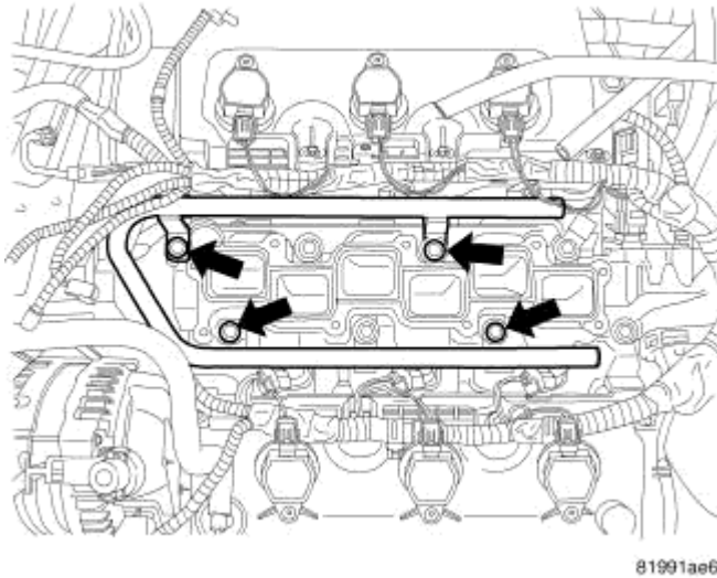
Fig. 182: Fuel Rail Bolts Courtesy of CHRYSLER LLC
