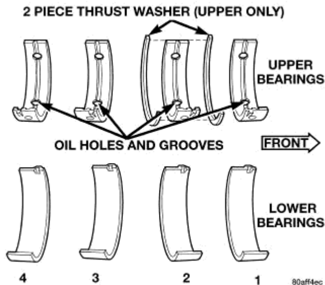
Fig. 279: Main Bearing Identification
