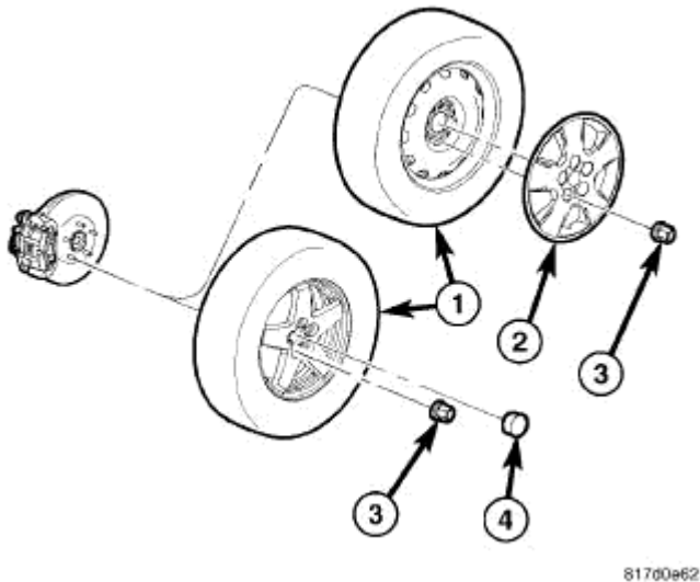
Fig. 399: TIRE & WHEEL MOUNTING
