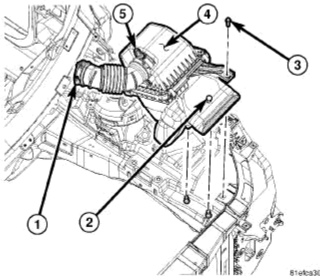
Fig. 322: HOUSING - AIR CLEANER Courtesy of CHRYSLER LLC
