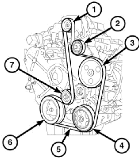
Fig. 73: 3.5L ENGINE ACCESSORY DRIVE BELT INSTALLATION Courtesy of CHRYSLER LLC
