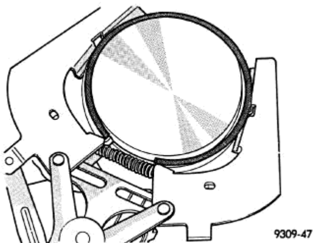
Fig. 301: Removing/Installing Upper And Intermediate Rings Courtesy of CHRYSLER LLC
