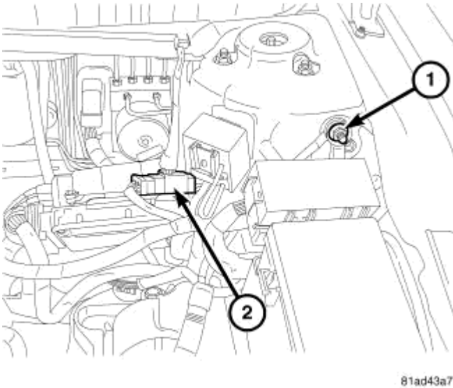
Fig. 425: BATTERY CABLE Courtesy of CHRYSLER LLC
