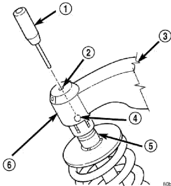
Fig. 207: Purging Air From Lash Adjuster Courtesy of CHRYSLER LLC
