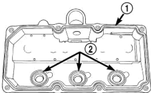
Fig. 196: Cvylinder Head Cover Gasket & Spark Plug Tube Seals
