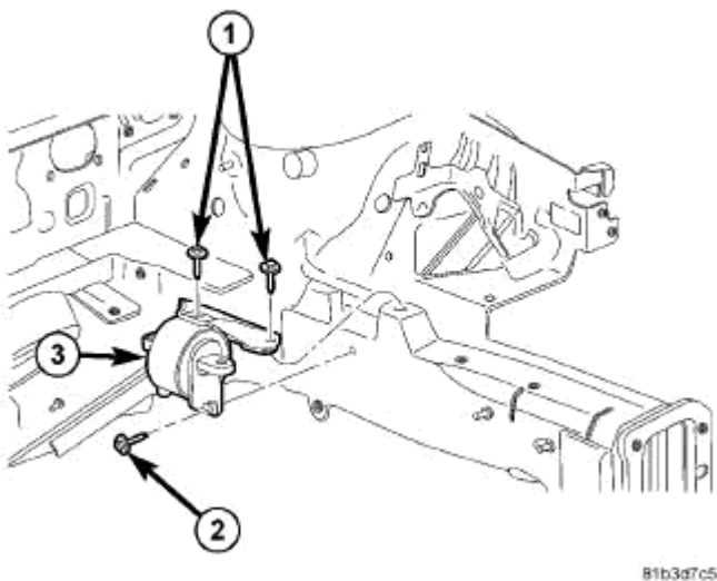
Fig. 319: LEFT ISOLATOR INSTALLATION Courtesy of CHRYSLER LLC
