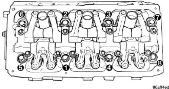
Fig. 154: Cylinder Head Bolt Tightening Sequence Courtesy of CHRYSLER LLC
