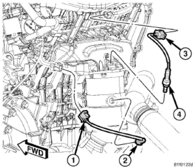
Fig. 401: Right Manifold Downstream/Upstream Oxygen Sensors Courtesy of CHRYSLER LLC
