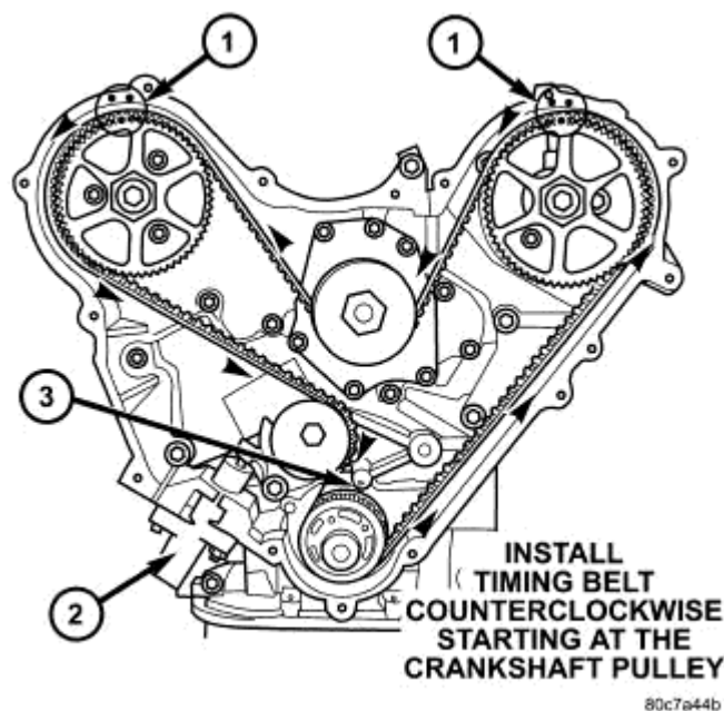
Fig. 450: TIMING BELT INSTALLATION
