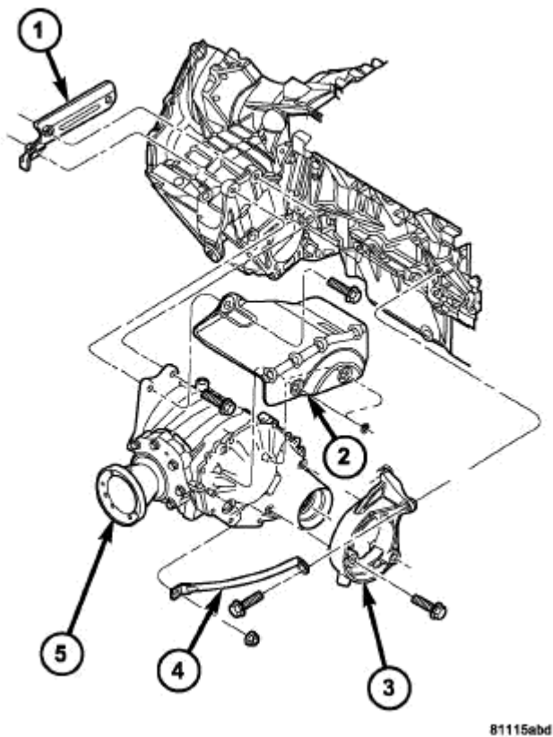
Fig. 25: Power Transfer Unit Mounting Courtesy of CHRYSLER LLC
