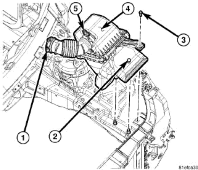
Fig. 110: HOUSING - AIR CLEANER Courtesy of CHRYSLER LLC
