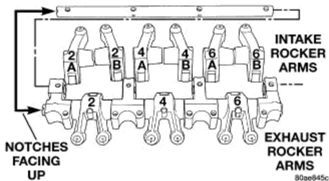
Fig. 213: Rocker Arms & Shafts Courtesy of CHRYSLER LLC
