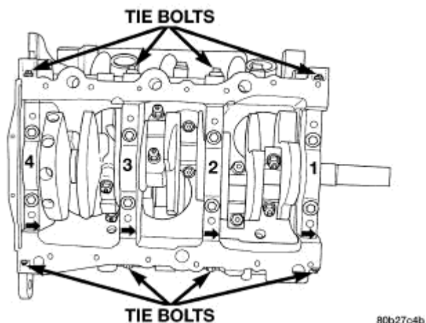
Fig. 270: Main Bearing Cap Identification Courtesy of CHRYSLER LLC
