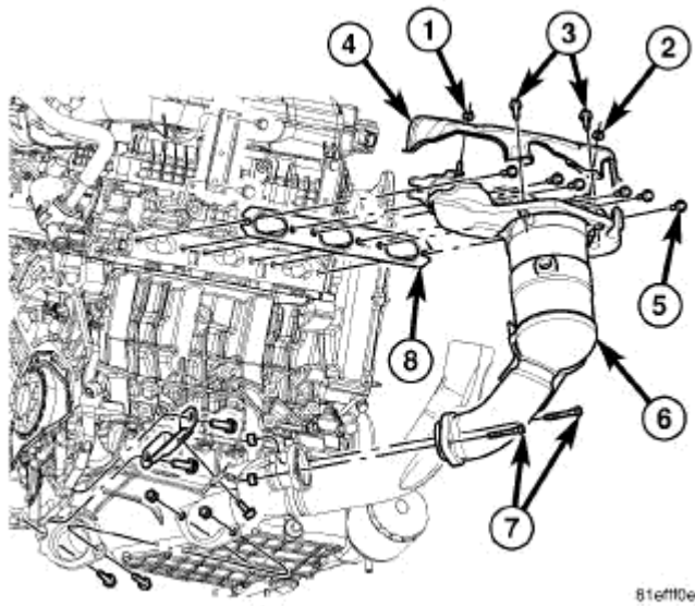
Fig. 412: Maniverter Retaining Bolts Courtesy of CHRYSLER LLC
