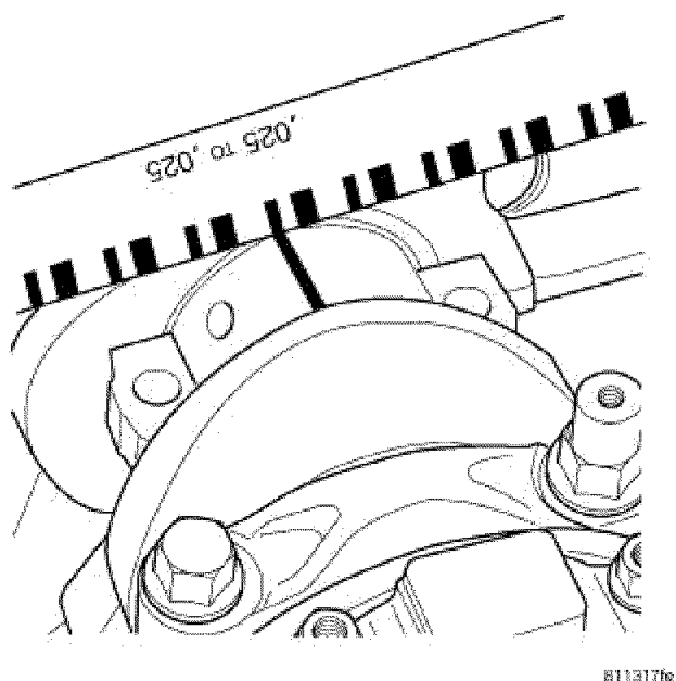
Fig. 261: CONNECTING ROD BEARING CLEARANCE
