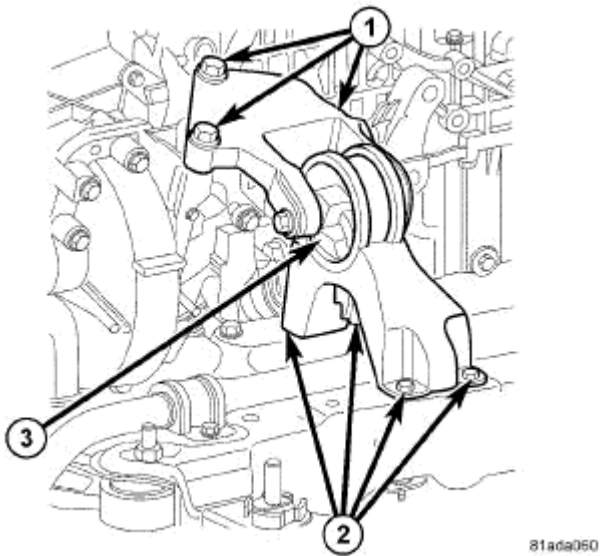
Fig. 327: REAR MOUNT
