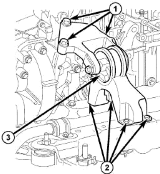
Fig. 332: REAR MOUNT
