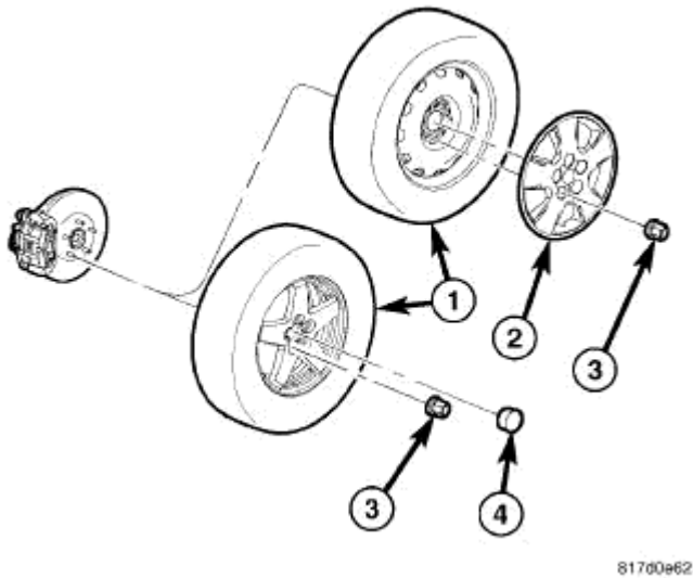
Fig. 394: TIRE & WHEEL MOUNTING Courtesy of CHRYSLER LLC
