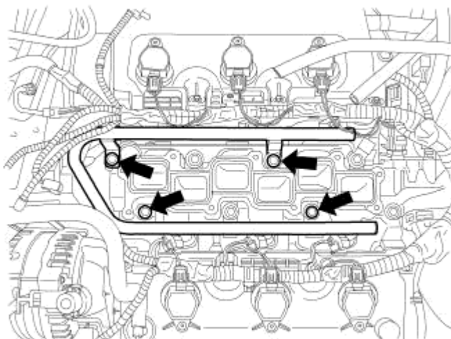
Fig. 138: Fuel Rail Bolts Courtesy of CHRYSLER LLC
