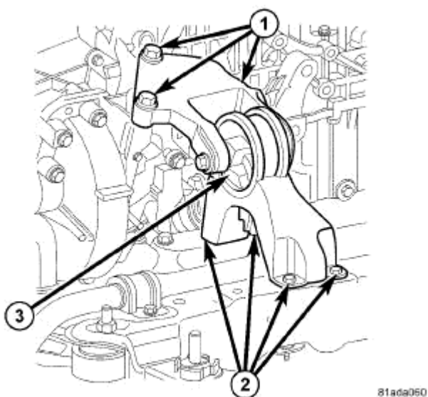
Fig. 334: REAR MOUNT
