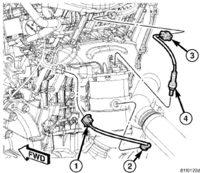
Fig. 414: Right Manifold Downstream/Upstream Oxygen Sensors Courtesy of CHRYSLER LLC
