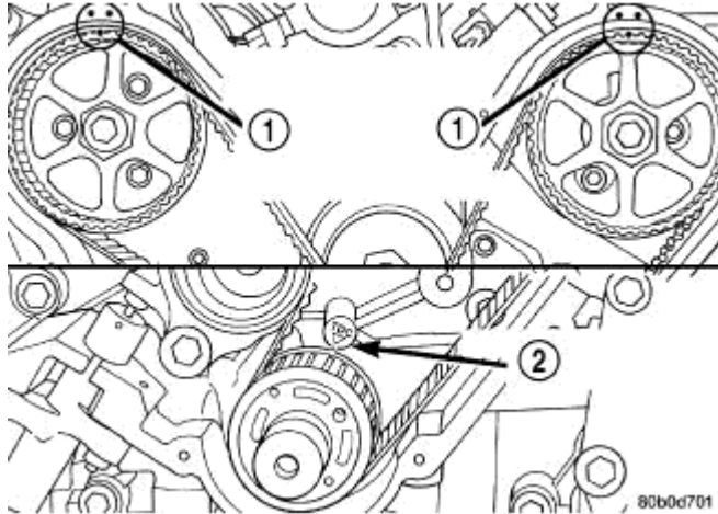
Fig. 159: CAMSHAFT SPROCKET TIMING MARKS Courtesy of CHRYSLER LLC
