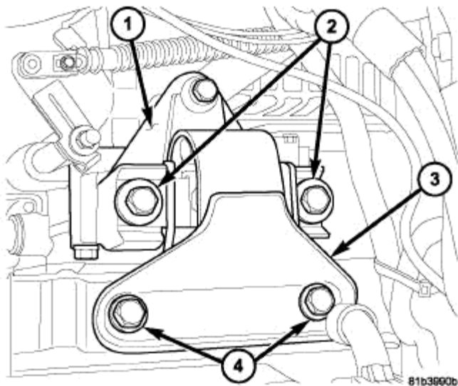
Fig. 320: LEFT MOUNT Courtesy of CHRYSLER LLC
