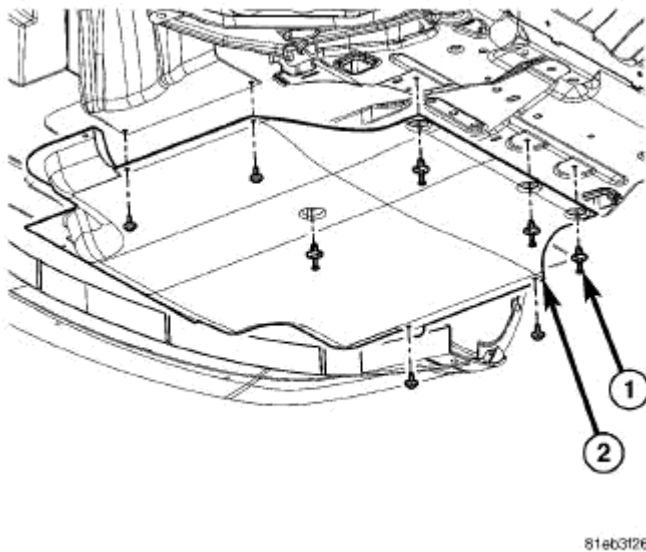
Fig. 316: Belly Pan Fasteners Courtesy of CHRYSLER LLC
