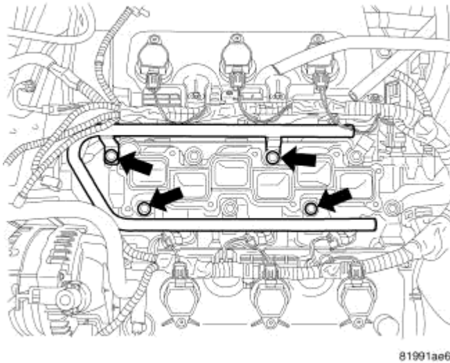
Fig. 429: Fuel Rail Bolts Courtesy of CHRYSLER LLC
