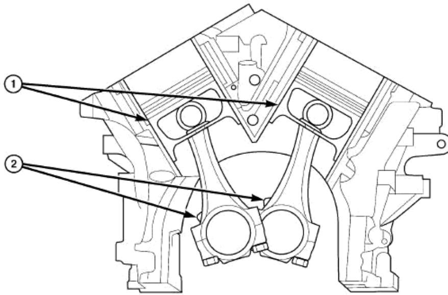
Fig. 311: PISTON & CONNECTING ROD POSITIONING Courtesy of CHRYSLER LLC
