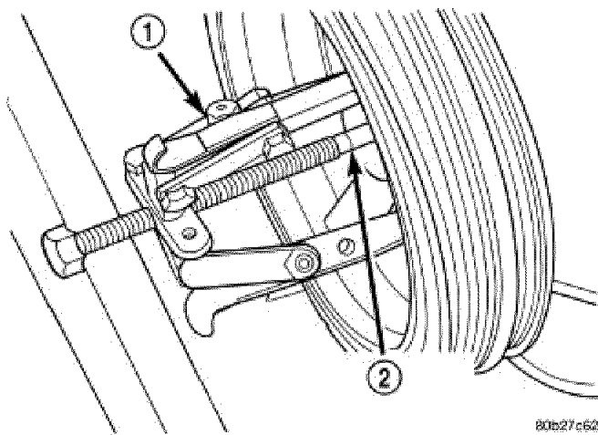
Fig. 289: Crankshaft Damper-Removal Courtesy of CHRYSLER LLC
