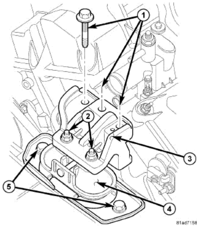
Fig. 324: Right Side Engine Mount Bolts Courtesy of CHRYSLER LLC
