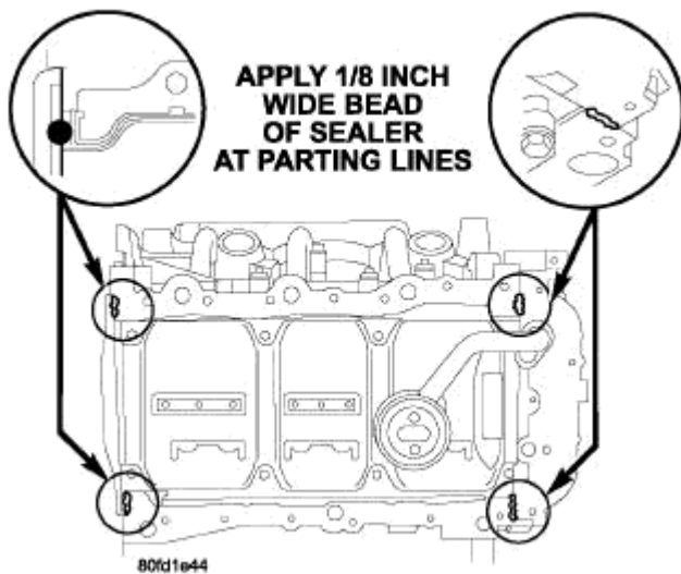
Fig. 356: OIL PAN SEALING - TYPICAL Courtesy of CHRYSLER LLC
