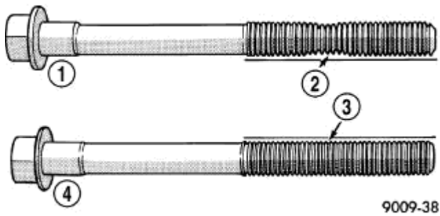
Fig. 307: Check for Stretched Bolts Courtesy of CHRYSLER LLC
