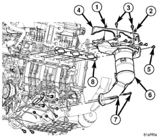
Fig. 402: Manifold Retaining Bolts Courtesy of CHRYSLER LLC
