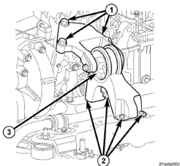
Fig. 330: REAR MOUNT
