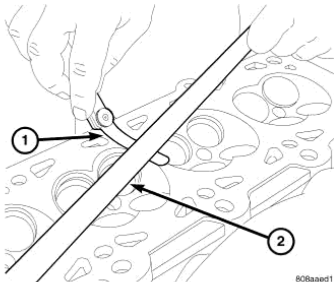
Fig. 150: Checking Cylinder Head Flatness
