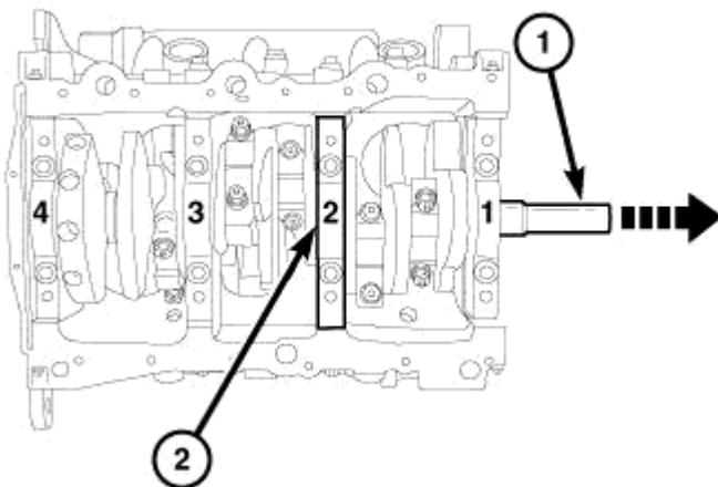
Fig. 282: Moving Crankshaft Forward To Limit Of Travel Courtesy of CHRYSLER LLC
