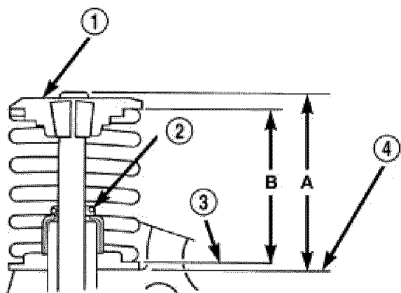
Fig. 258: Checking Valve Tip Height & Valve Spring Installed Height Courtesy of CHRYSLER LLC
