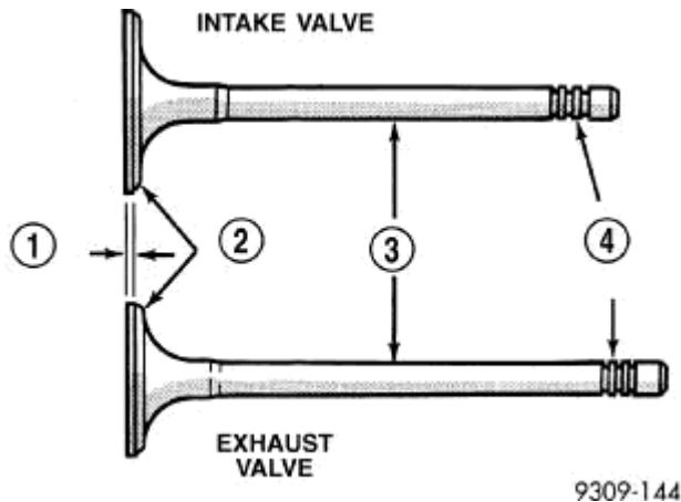
Fig. 256: Intake & Exhaust Valves Courtesy of CHRYSLER LLC
