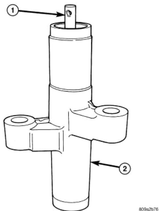
Fig. 467: TIMING BELT TENSIONER
