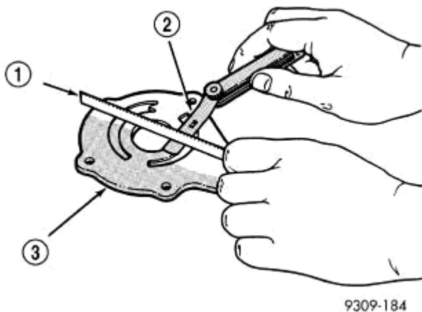
Fig. 365: Checking Oil Pump Cover Flatness
