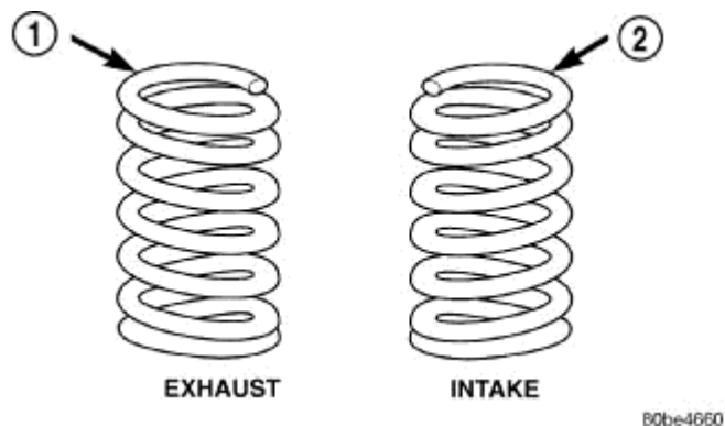
Fig. 255: Valve Spring Identification
