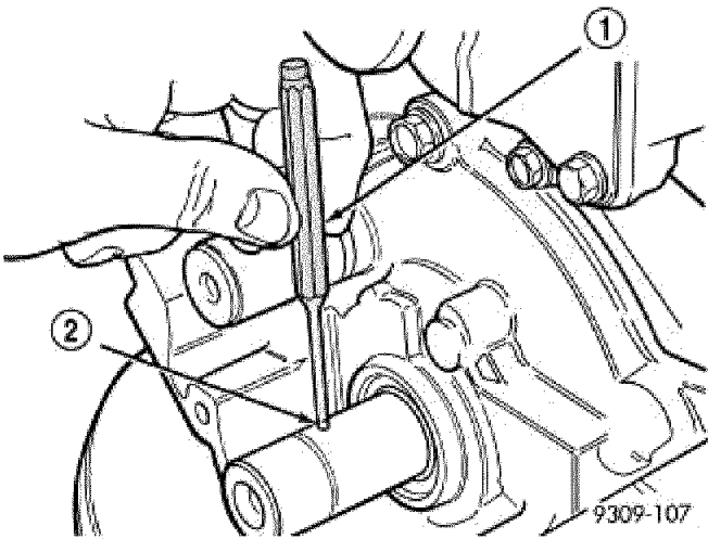
Fig. 312: Crankshaft Sprocket Dowel Pin-Removal/Installation Courtesy of CHRYSLER LLC
