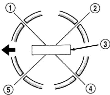
Fig. 308: PISTON RING END GAP POSITION Courtesy of CHRYSLER LLC
