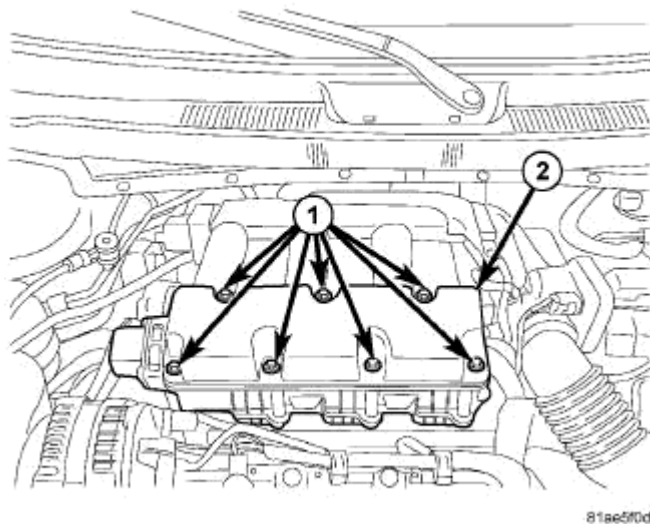
Fig. 183: Upper Intake Manifold Courtesy of CHRYSLER LLC
