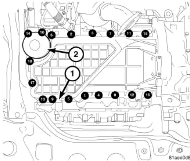
Fig. 357: OIL PAN
