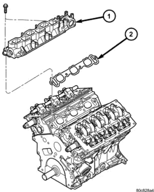
Fig. 120: Lower Intake Manifold Courtesy of CHRYSLER LLC
