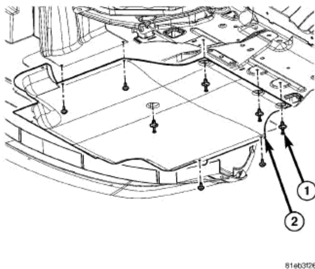
Fig. 340: Belly Pan Fasteners
