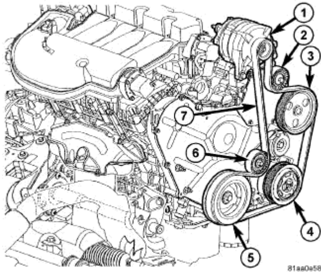
Fig. 228: Identifying Accessory Drive Belt & Pulleys
