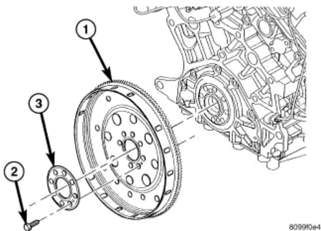
Fig. 292: FLEX PLATE
