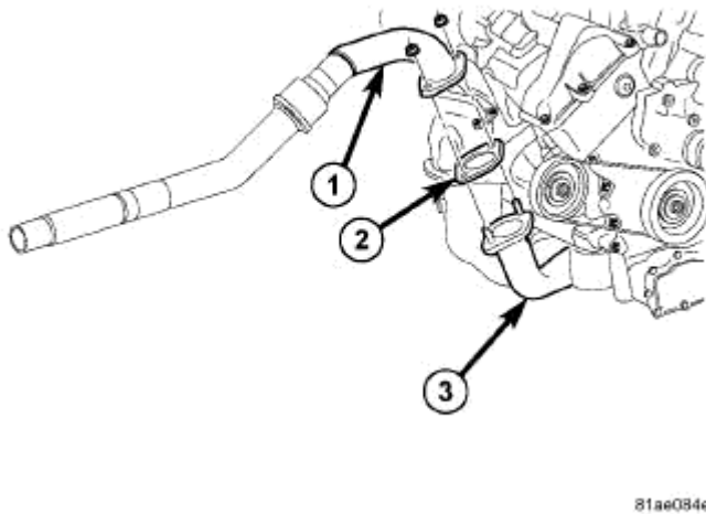
Fig. 72: Exhaust Extension Pipe & Gasket Courtesy of CHRYSLER LLC
