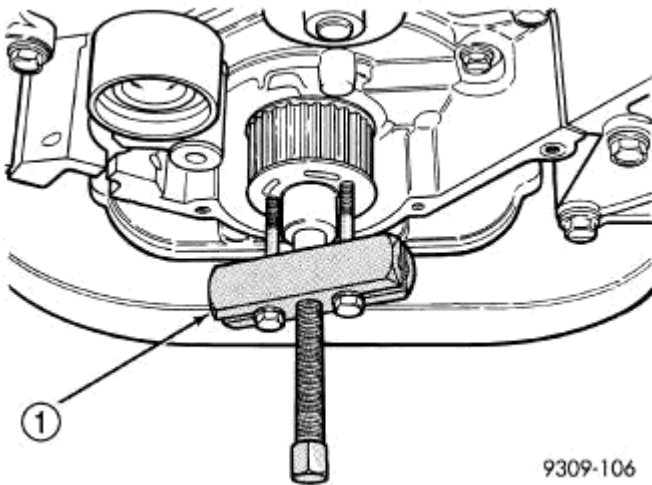
Fig. 445: Crankshaft Sprocket - Removal Courtesy of CHRYSLER LLC
