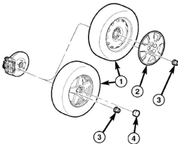
Fig. 409: TIRE & WHEEL MOUNTING Courtesy of CHRYSLER LLC
