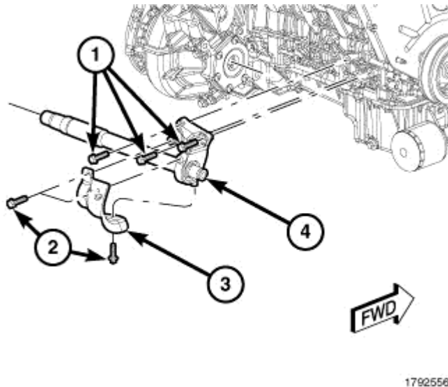
Fig. 413: Right Half Shaft & Intermediate Shaft Courtesy of CHRYSLER LLC
