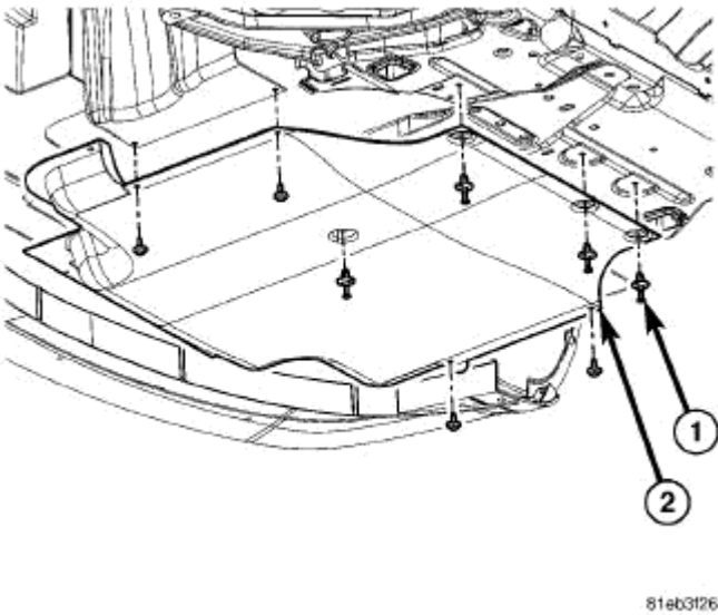
Fig. 393: Belly Pan Fasteners Courtesy of CHRYSLER LLC
