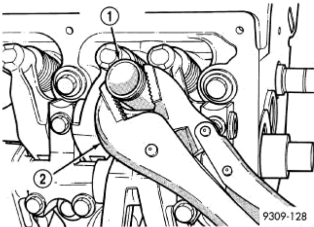
Fig. 249: Servicing Spark Plug Tubes Courtesy of CHRYSLER LLC
