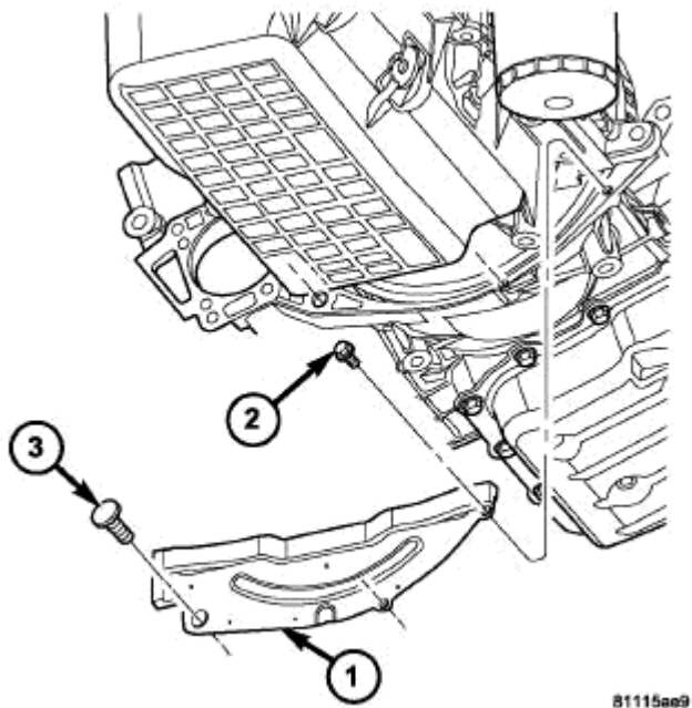
Fig. 7: Torque Converter Dust Shield Courtesy of CHRYSLER LLC
