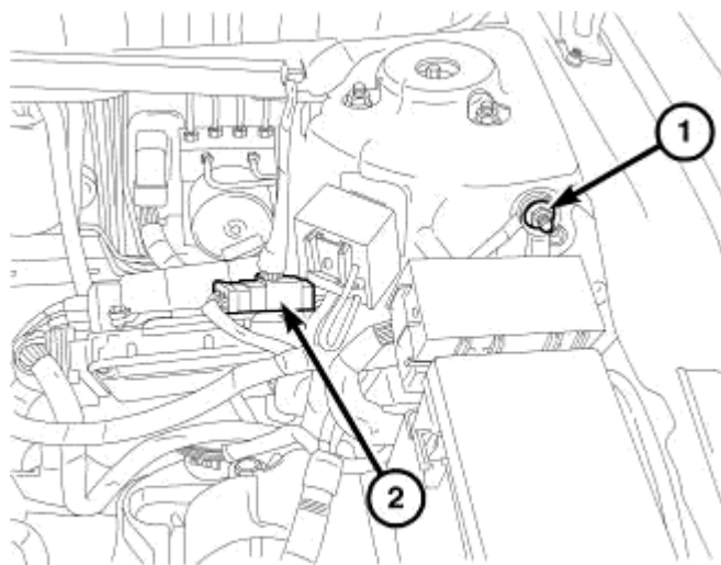
Fig. 418: BATTERY CABLE Courtesy of CHRYSLER LLC
