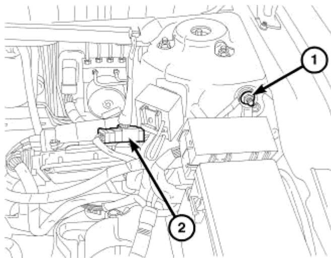
Fig. 12: BATTERY CABLE Courtesy of CHRYSLER LLC
