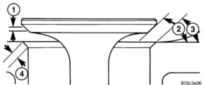
Fig. 252: Valve Face & Seat Courtesy of CHRYSLER LLC
