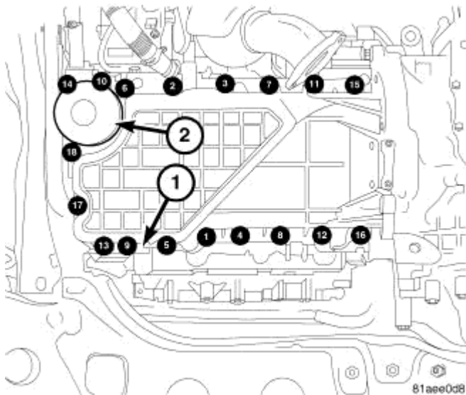
Fig. 355: OIL PAN
