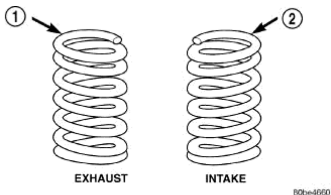
Fig. 243: Valve Spring Identification
