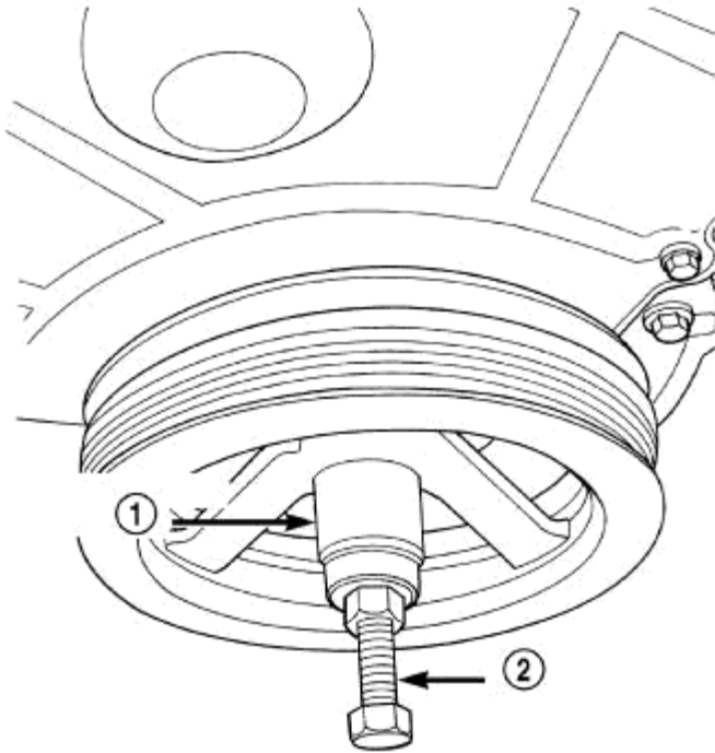
Fig. 290: Crankshaft Damper-Installation
