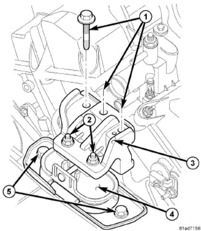
Fig. 325: Right Side Engine Mount Bolts Courtesy of CHRYSLER LLC
