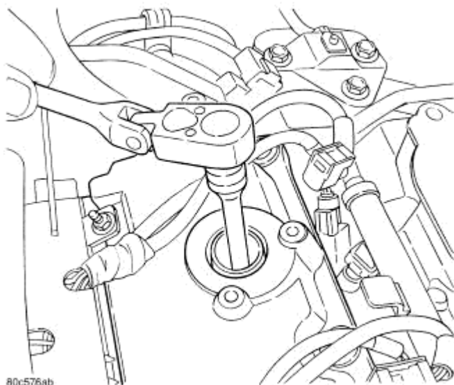
Fig. 10: SPARK PLUG REMOVAL/INSTALLATION Courtesy of CHRYSLER LLC
