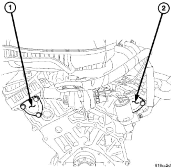
Fig. 194: CAMSHAFT THRUST PLATES
