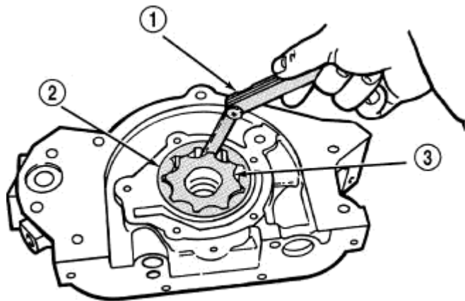
Fig. 369: Measuring Clearance Between Rotors Courtesy of CHRYSLER LLC
