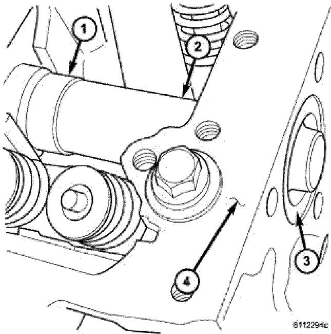
Fig. 156: CAMSHAFT INSTALLATION - LEFT Courtesy of CHRYSLER LLC
