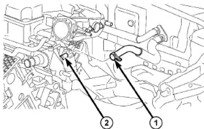
Fig. 58: Heater Core Supply Hose Courtesy of CHRYSLER LLC
