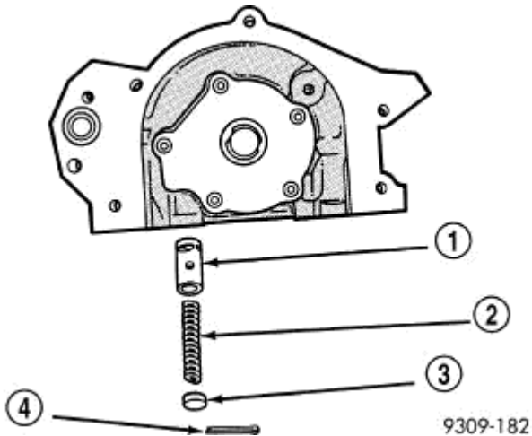
Fig. 377: Oil Pressure Relief Valve
