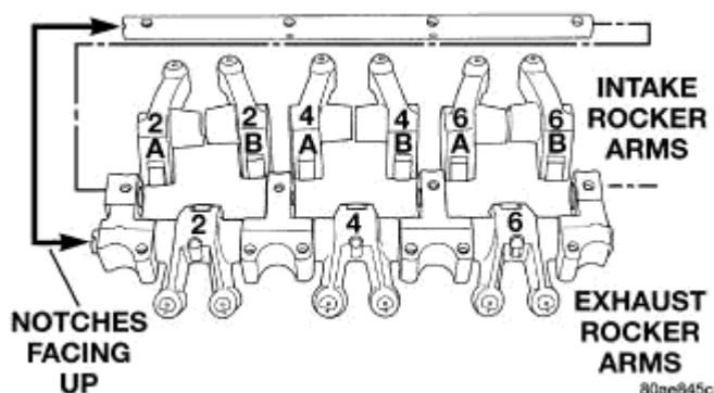
Fig. 204: Rocker Arms & Shafts Courtesy of CHRYSLER LLC
