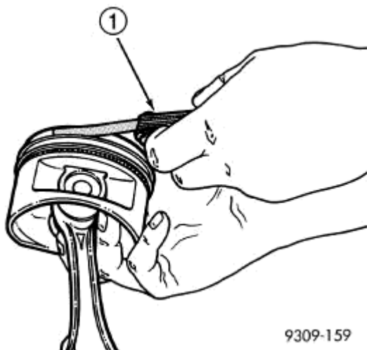
Fig. 300: MEASURING PISTON RING SIDE CLEARANCE Courtesy of CHRYSLER LLC
