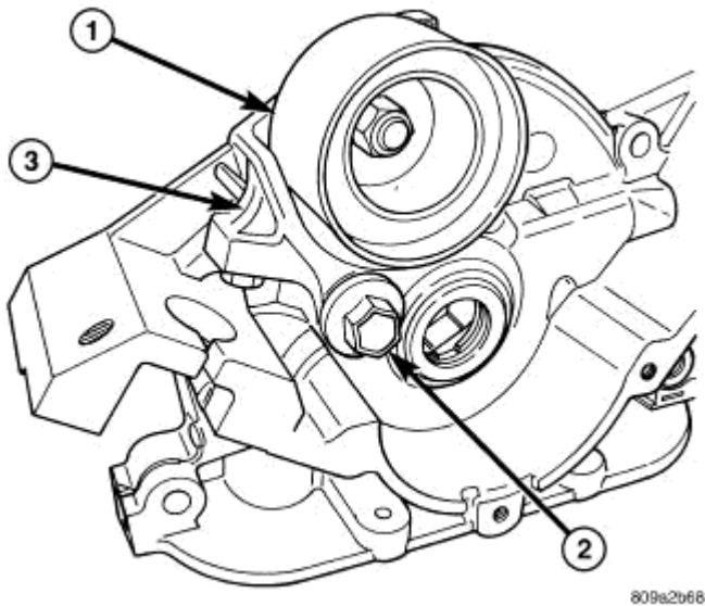
Fig. 466: TENSIONER PULLEY
