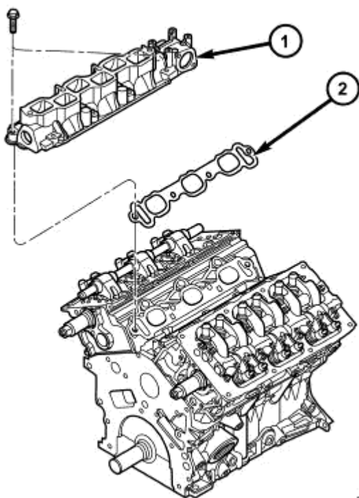
Fig. 139: Lower Intake Manifold Courtesy of CHRYSLER LLC
