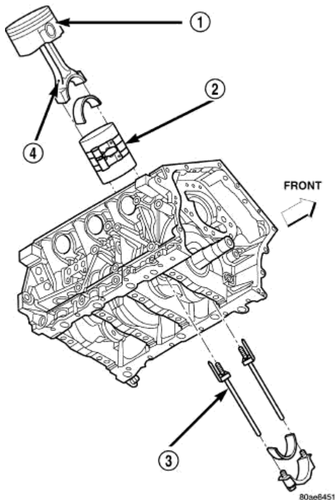
Fig. 309: Piston & Connecting Rod
