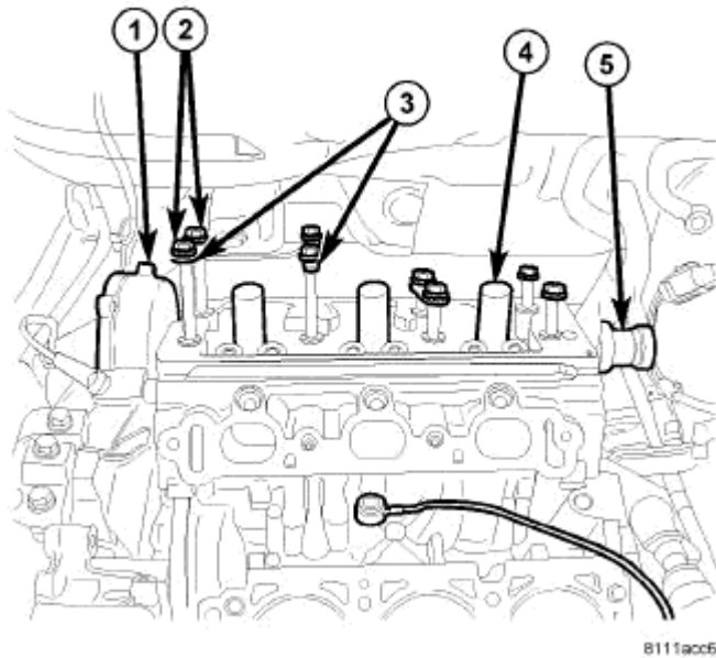
Fig. 131: RIGHT CYLINDER HEAD
