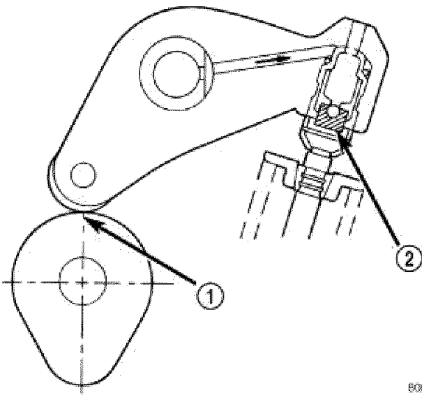
Fig. 205: Rocker Arm Positioned On Base Circle Of Camshaft Courtesy of CHRYSLER LLC
