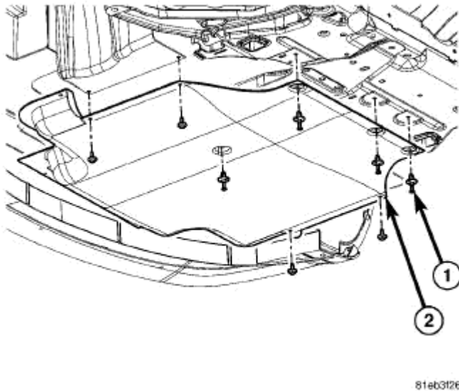
Fig. 321: Belly Pan Fasteners Courtesy of CHRYSLER LLC
