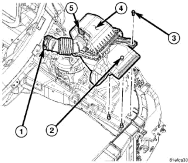
Fig. 315: HOUSING - AIR CLEANER Courtesy of CHRYSLER LLC
