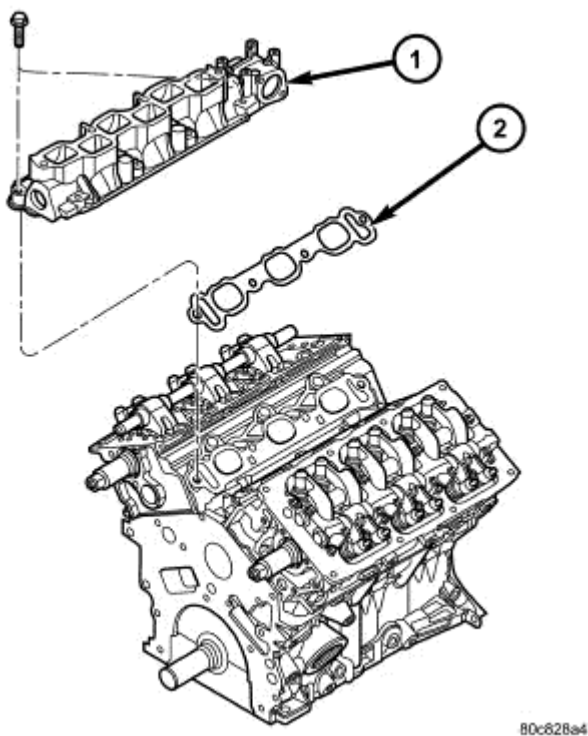
Fig. 164: Lower Intake Manifold Courtesy of CHRYSLER LLC
