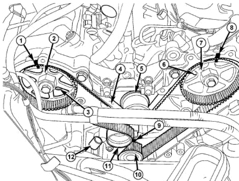
Fig. 440: TIMING GEAR MARKS Courtesy of CHRYSLER LLC
