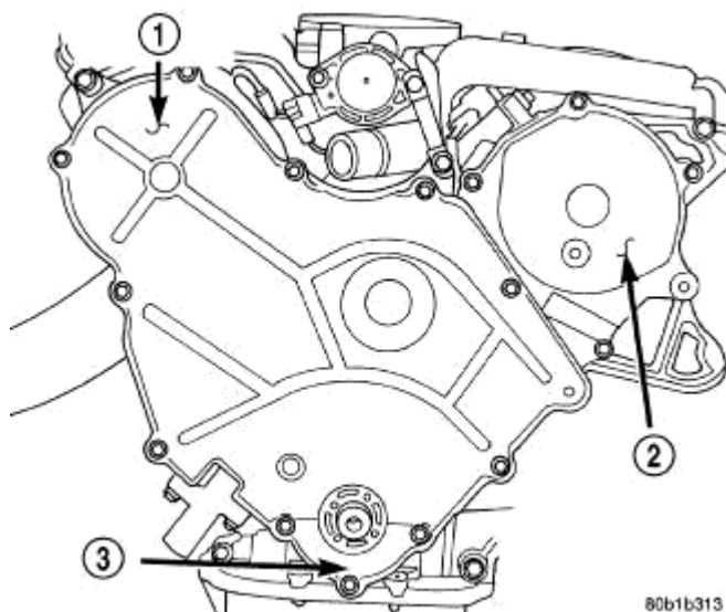
Fig. 124: TIMING BELT COVERS Courtesy of CHRYSLER LLC
