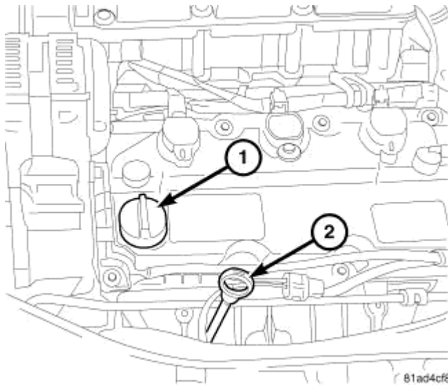
Fig. 349: ENGINE OIL FILLER CAP & DIPSTICK Courtesy of CHRYSLER LLC
