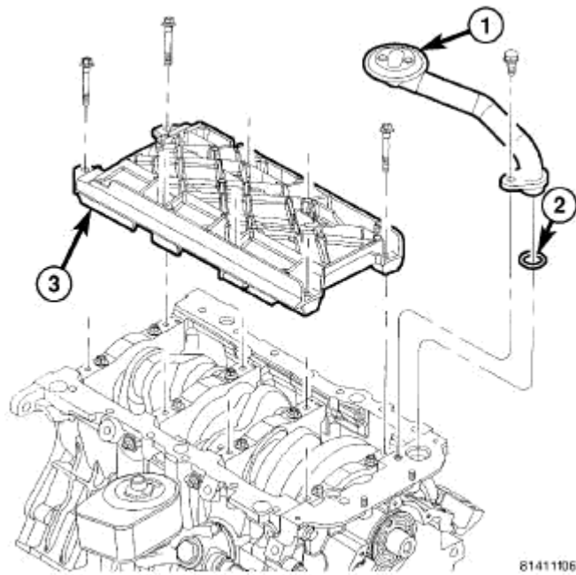
Fig. 286: OIL PICK UP TUBE & WINDAGE TRAY
