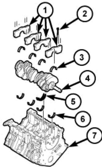
Fig. 281: Main Bearings Assembly Courtesy of CHRYSLER LLC
