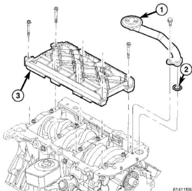
Fig. 275: OIL PICK UP TUBE & WINDAGE TRAY
