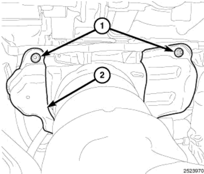
Fig. 411: Lower Maniverter Heatshield Courtesy of CHRYSLER LLC
