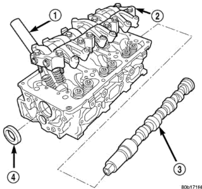
Fig. 126: Cylinder Head, Camshaft & Rocker Arms
