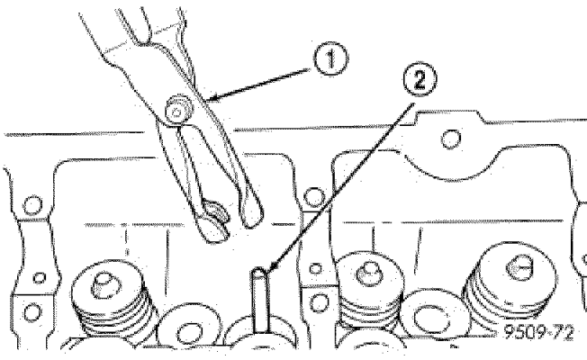
Fig. 241: Valve Stem Seal - Removal Courtesy of CHRYSLER LLC
