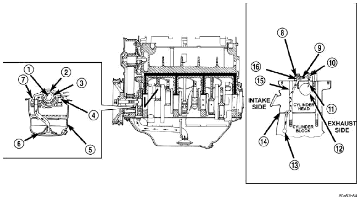
Fig. 342: Oil Lubrication System Courtesy of CHRYSLER LLC
