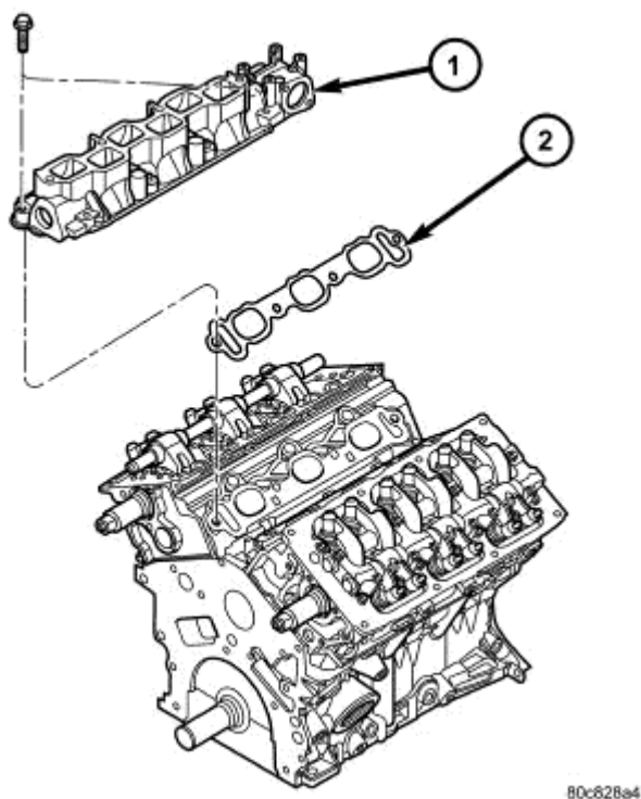
Fig. 431: Lower Intake Manifold Courtesy of CHRYSLER LLC
