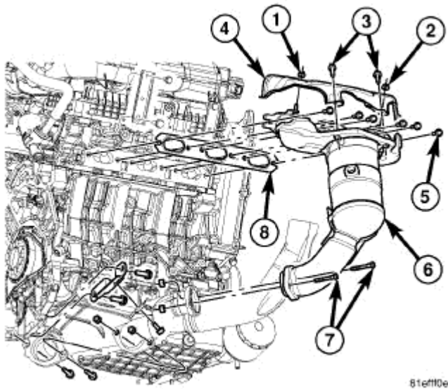
Fig. 404: Maniverter Retaining Bolts Courtesy of CHRYSLER LLC
