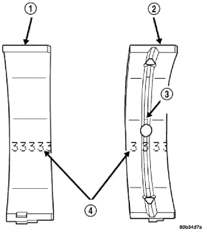
Fig. 268: Main Bearing Grade Marks Courtesy of CHRYSLER LLC
