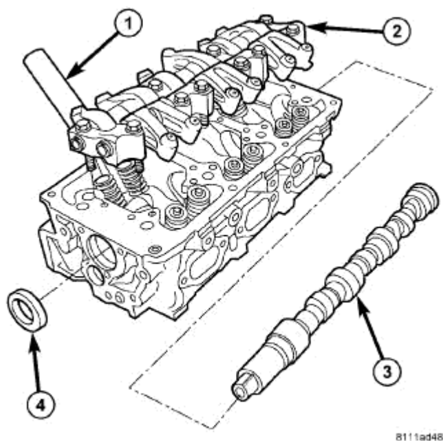
Fig. 250: CAMSHAFT, ROCKER ARM ASSEMBLY & CYLINDER HEAD
