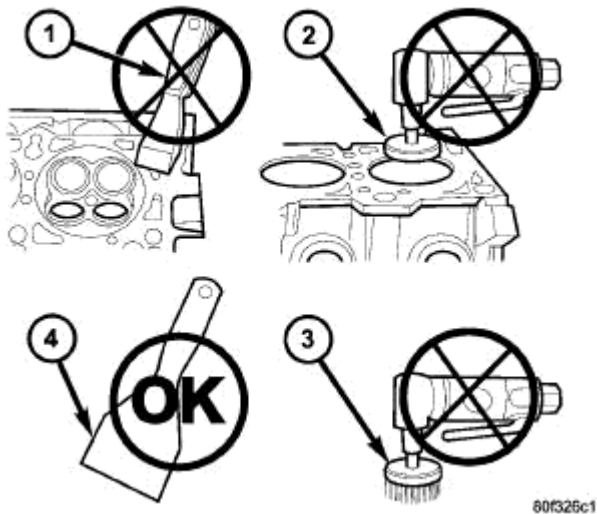
Fig. 9: PROPER TOOL USAGE FOR SURFACE PREPARATION
