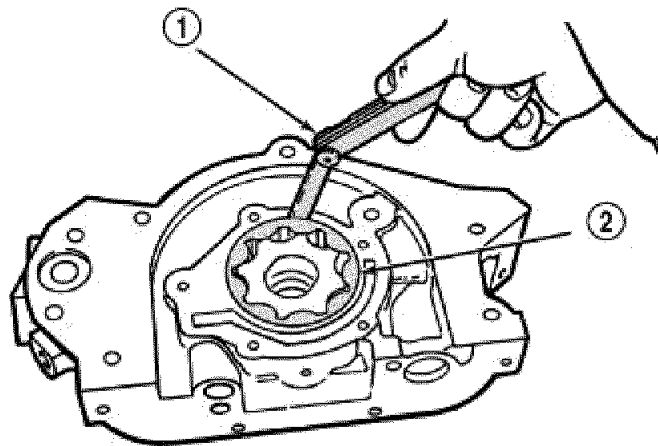
Fig. 368: Measuring Outer Rotor Clearance in Housing Courtesy of CHRYSLER LLC
