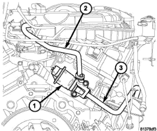
Fig. 125: Exhaust Gas Recirculation System
