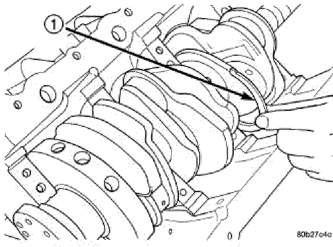
Fig. 280: Thrust Washer Installation Courtesy of CHRYSLER LLC
