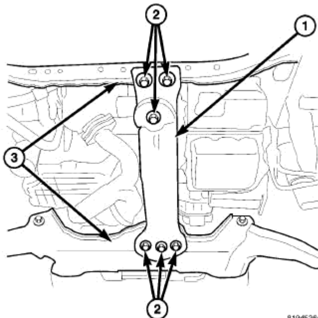
Fig. 361: FORE-AFT Crossmember
