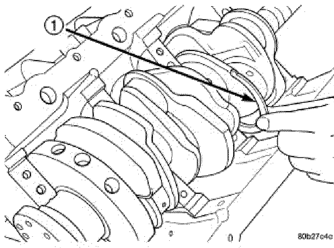
Fig. 273: Thrust Washer Installation Courtesy of CHRYSLER LLC
