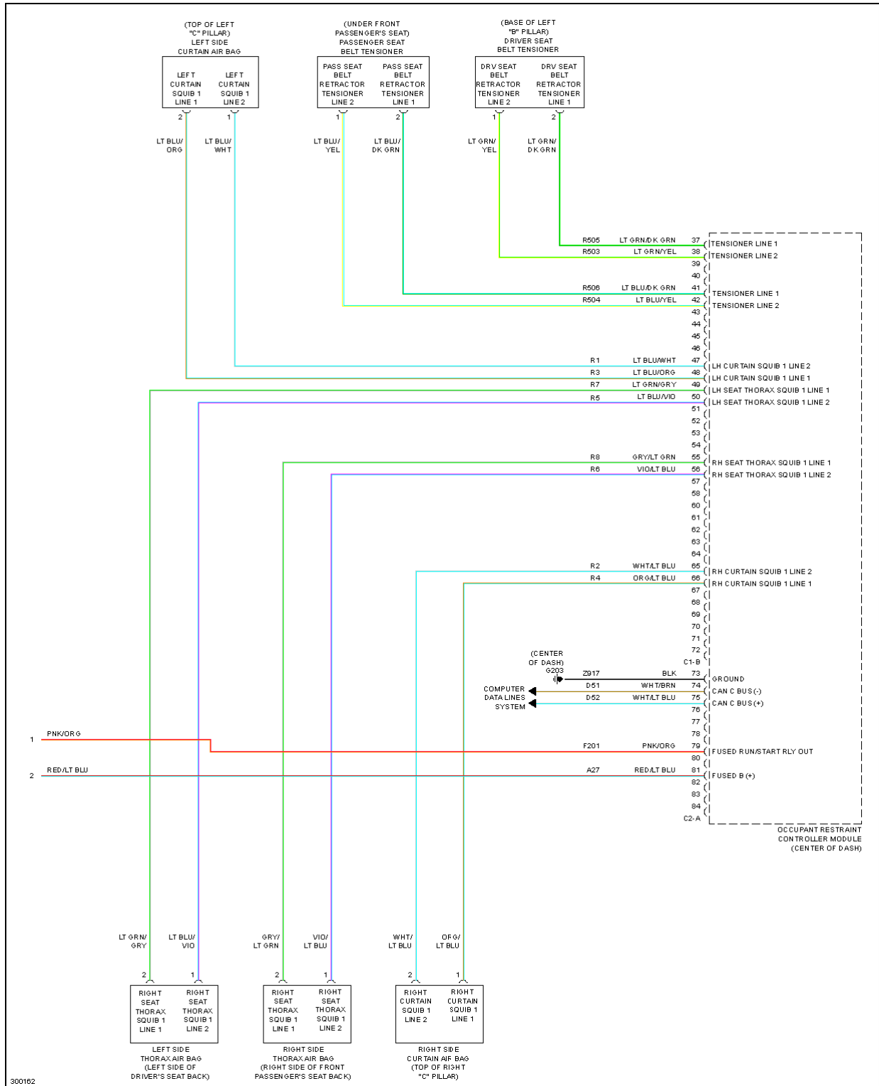
Fig. 68: Supplemental Restraints Circuit (3 of 3)
