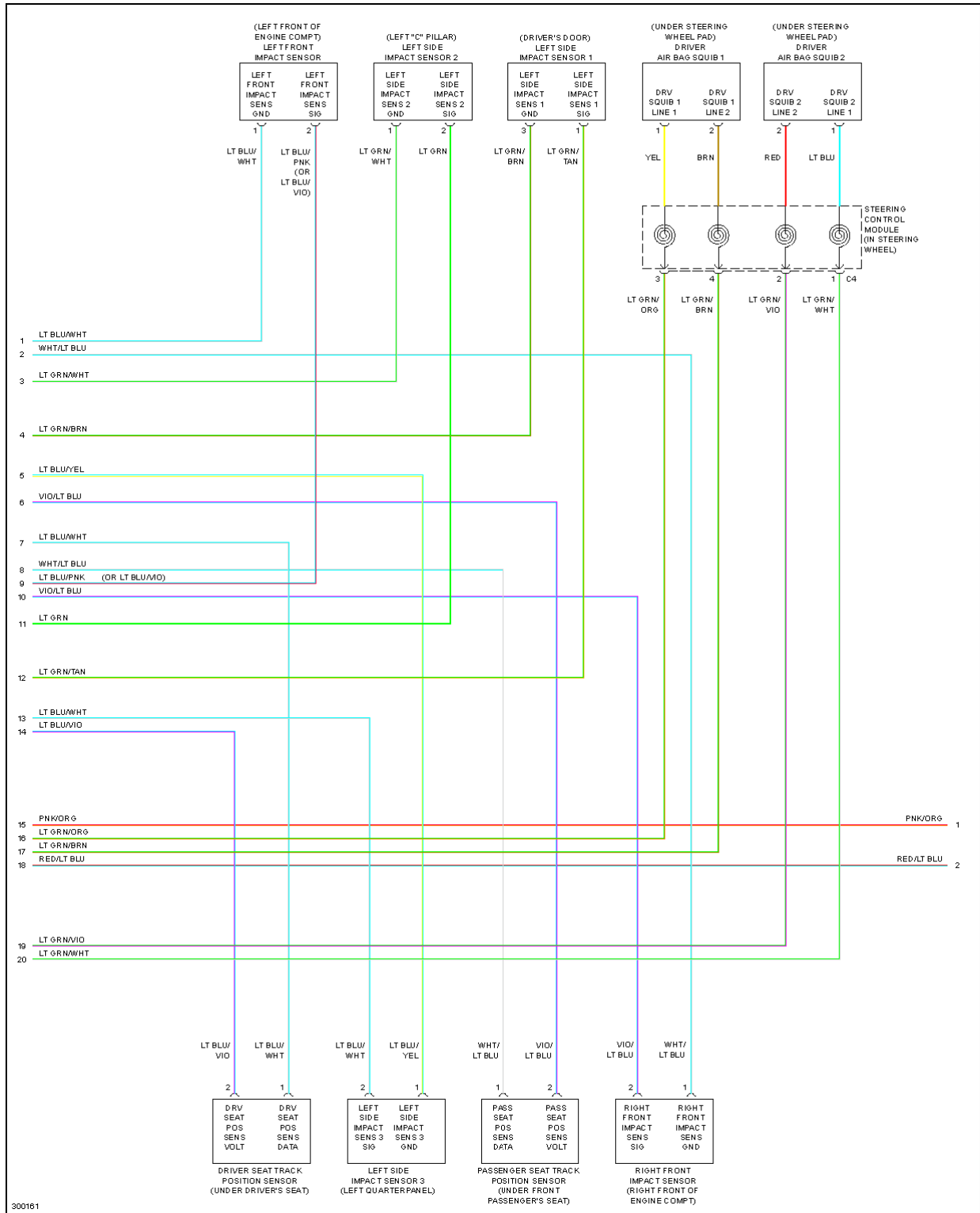
Fig. 67: Supplemental Restraints Circuit (2 of 3)
