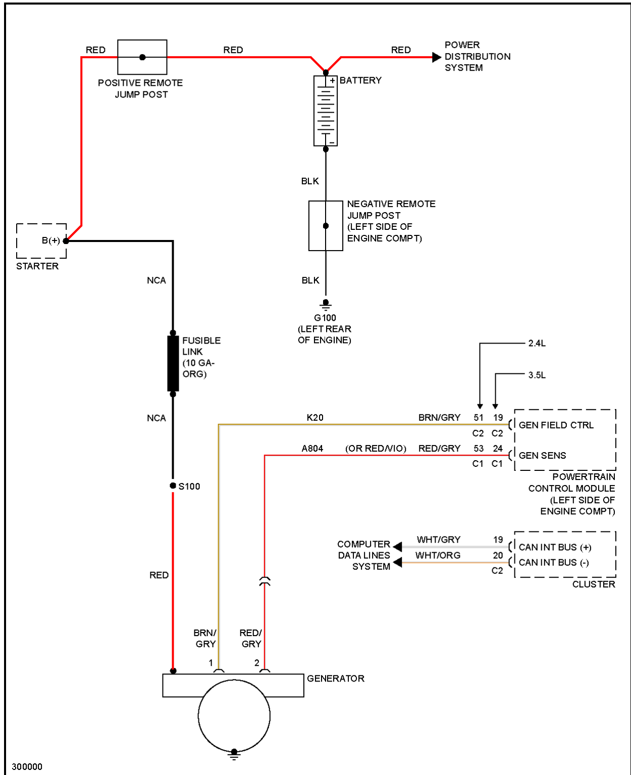
Fig. 64: Charging Circuit
