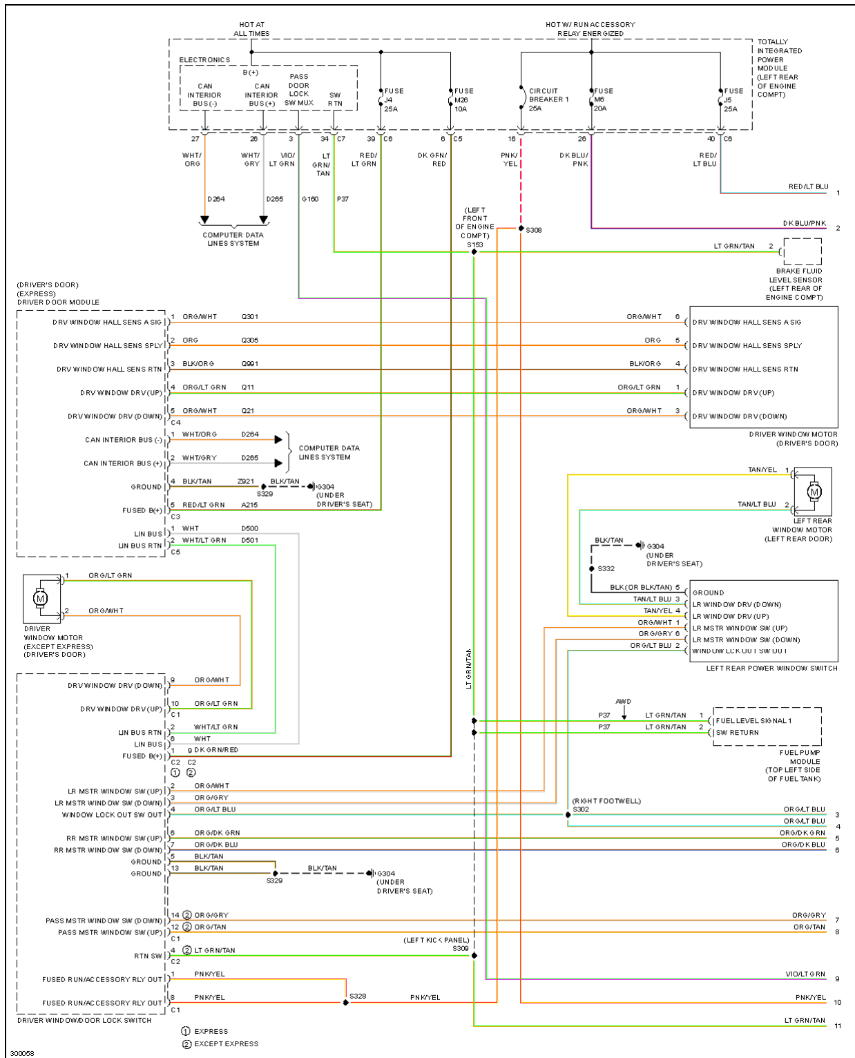
Fig. 55: Power Windows Circuit (1 of 2)
