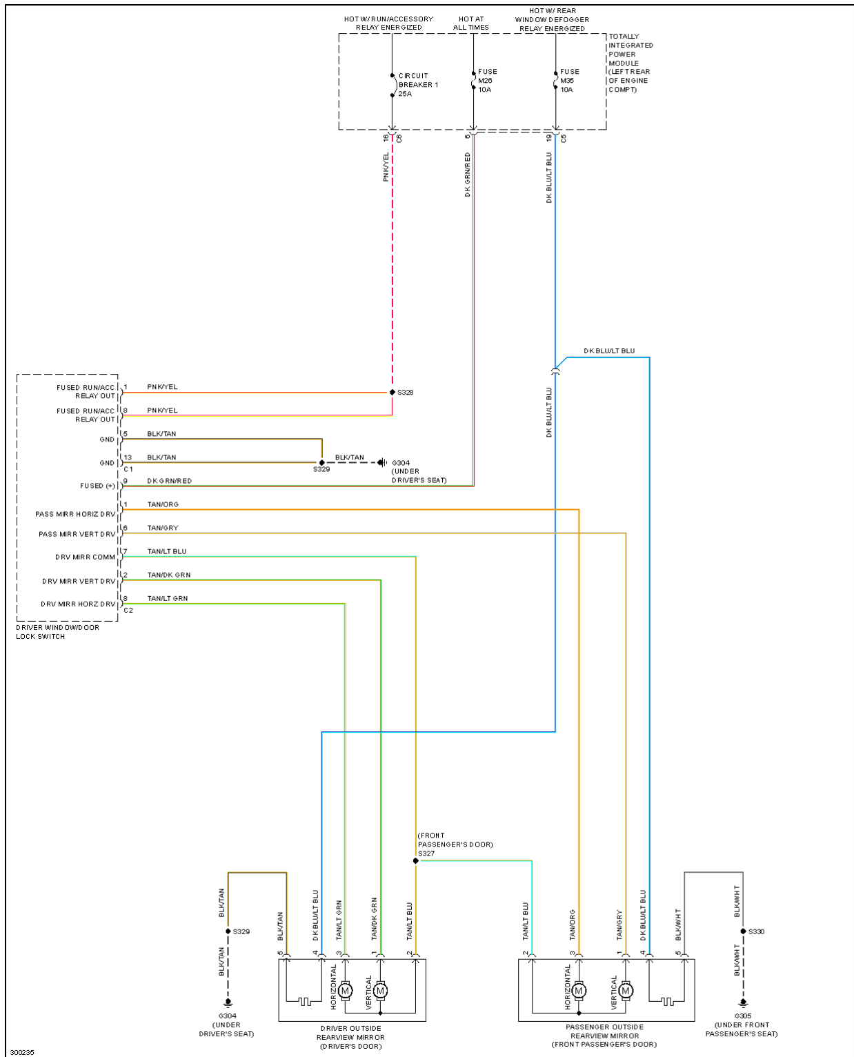
Fig. 51: Power Mirrors Circuit, W/O Express Up/Down Windows
