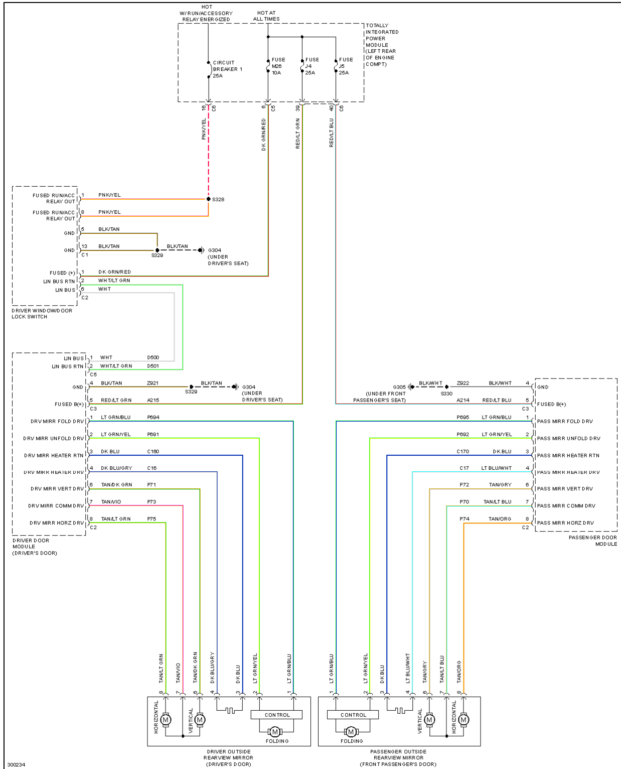
Fig. 50: Power Mirrors Circuit, W/ Express Up/Down Windows
