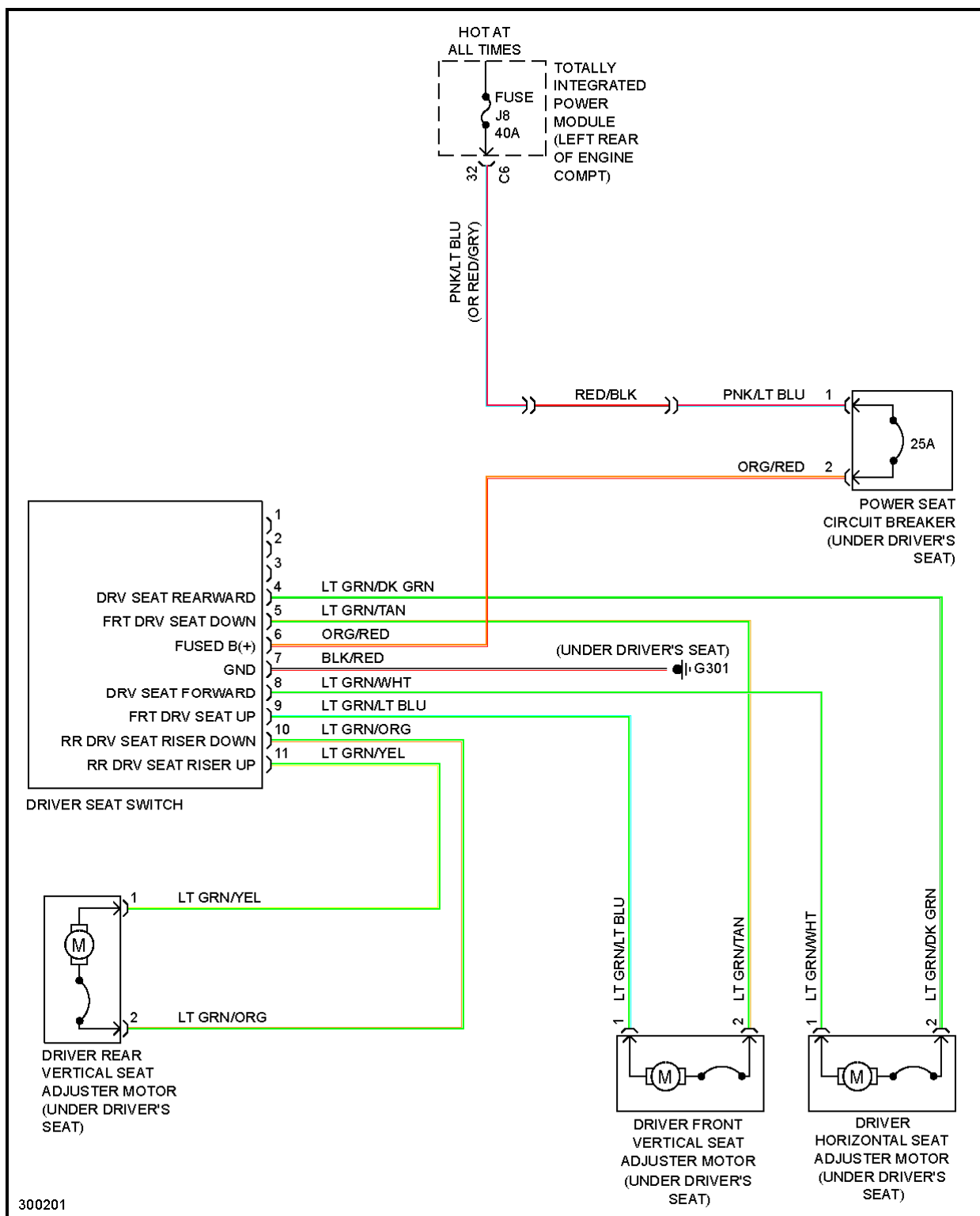
Fig. 53: Power Seat Circuit
