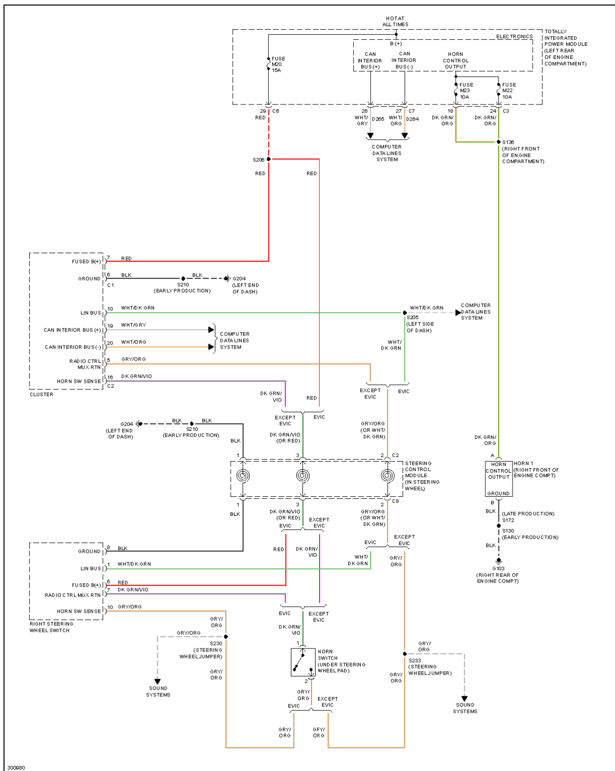
Fig. 33: Horn Circuit
