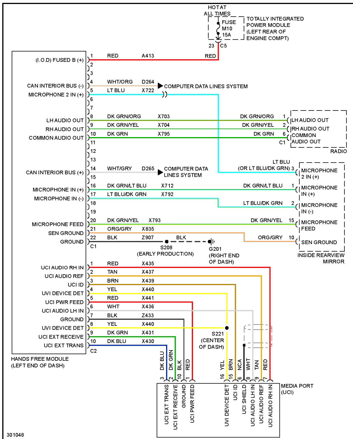
Fig. 57: Hands Free Module Circuit
