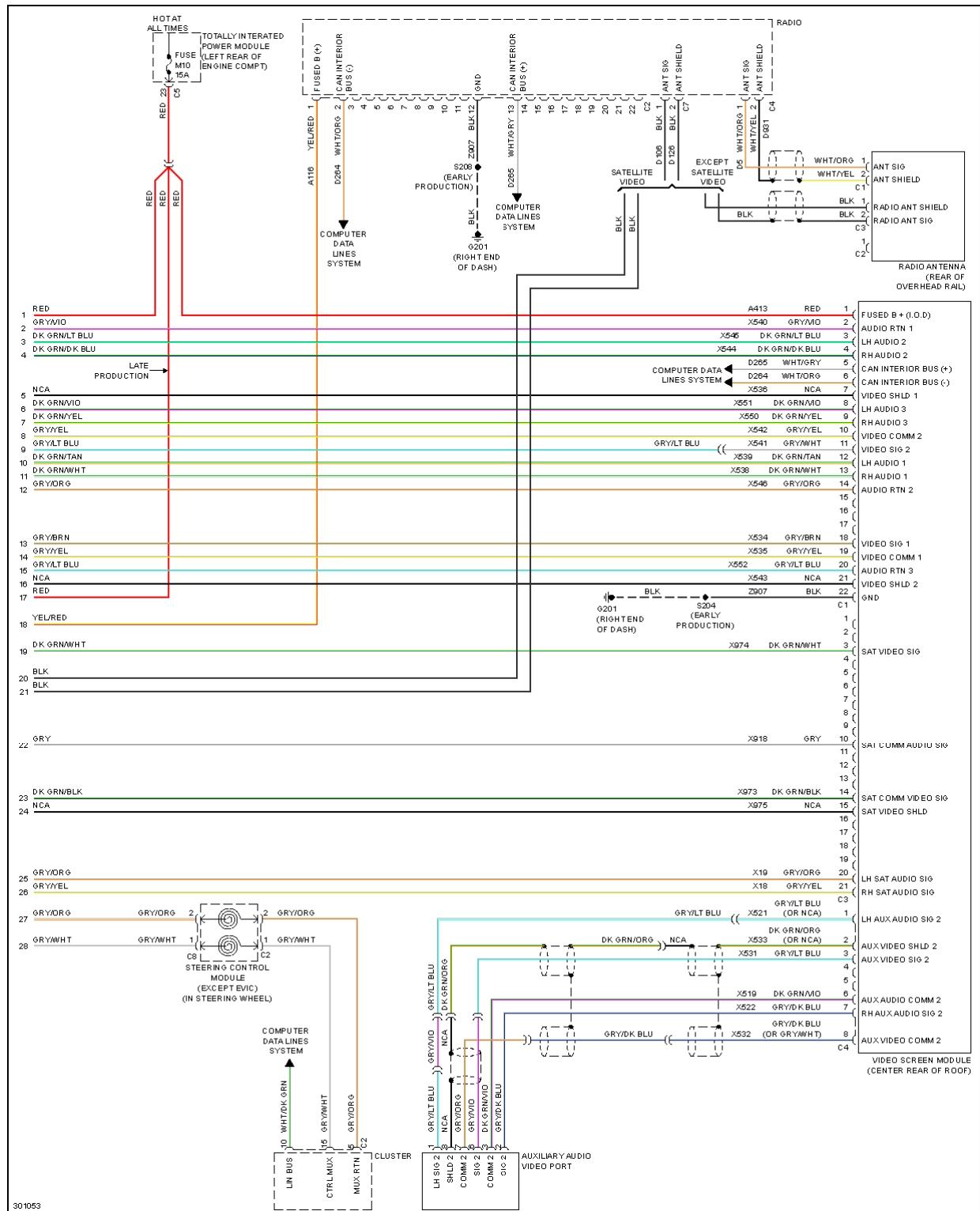
Fig. 42: Navigation Circuit, Premium (4 of 4)
