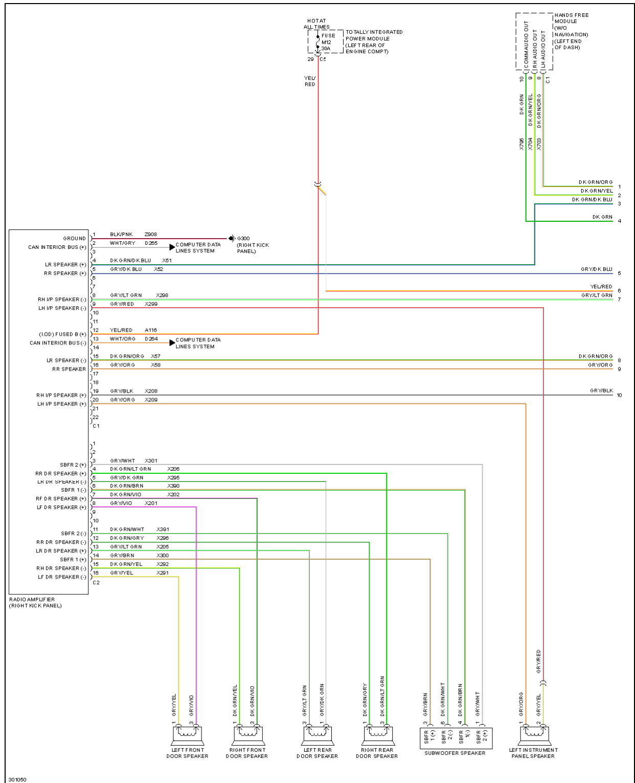
Fig. 39: Navigation Circuit, Premium (1 of 4)
