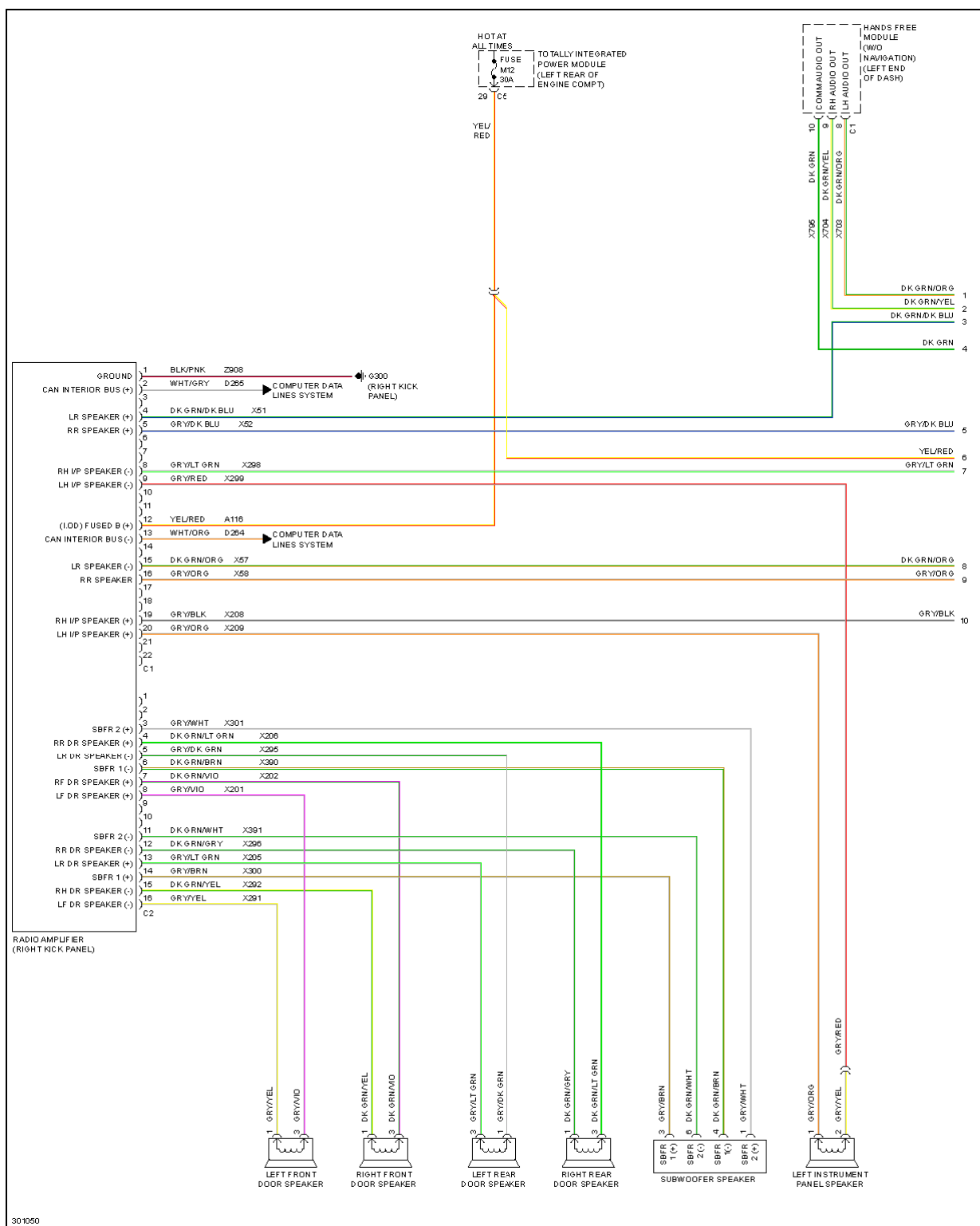
Fig. 59: Radio Circuit, Premium (1 of 4)
