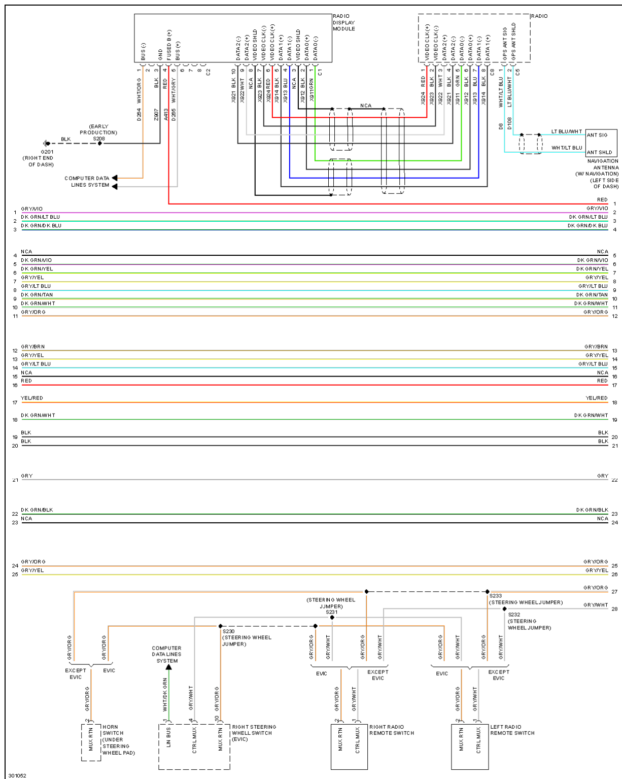
Fig. 61: Radio Circuit, Premium (3 of 4)
