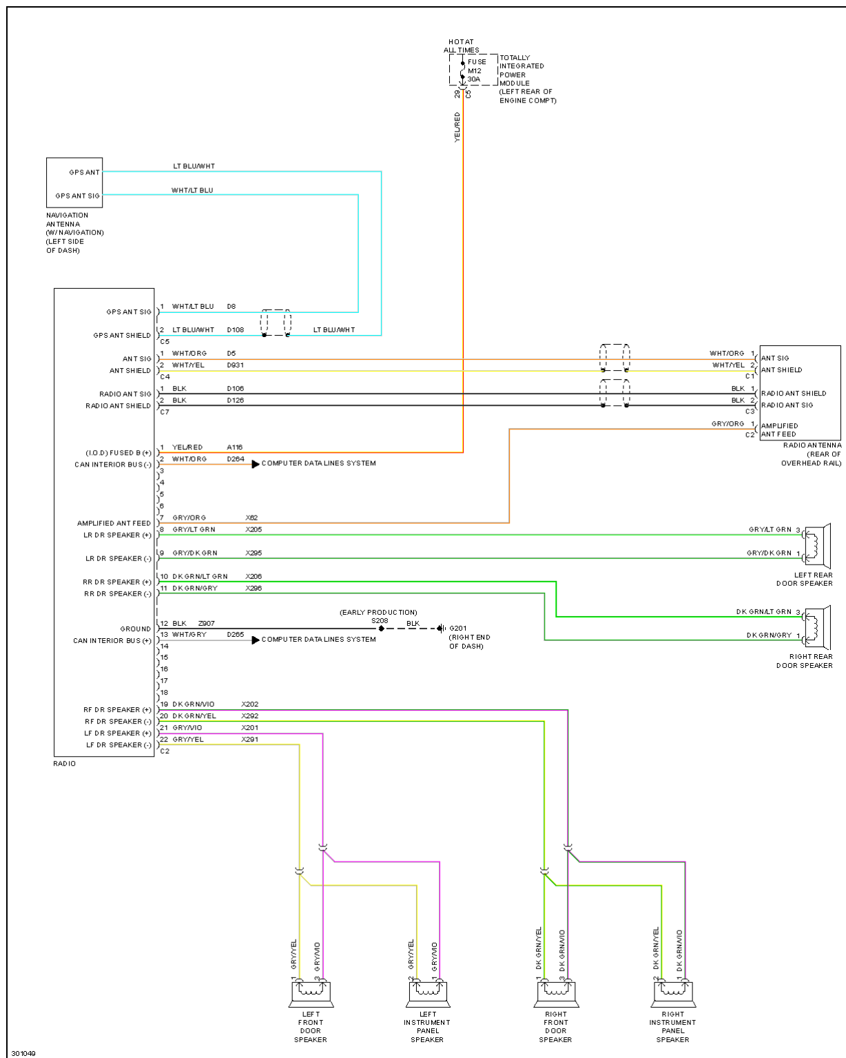
Fig. 58: Radio Circuit, Base
