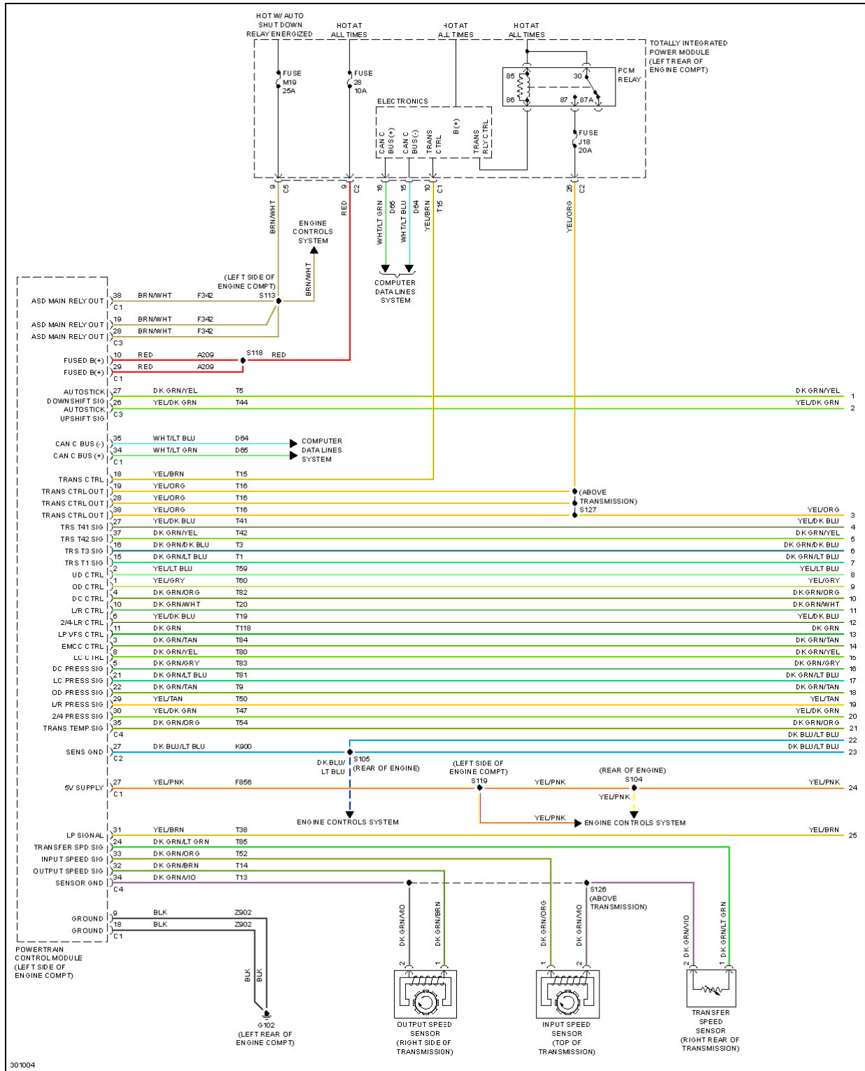
Fig. 71: 3.5L, A/T Circuit (1 of 2)
