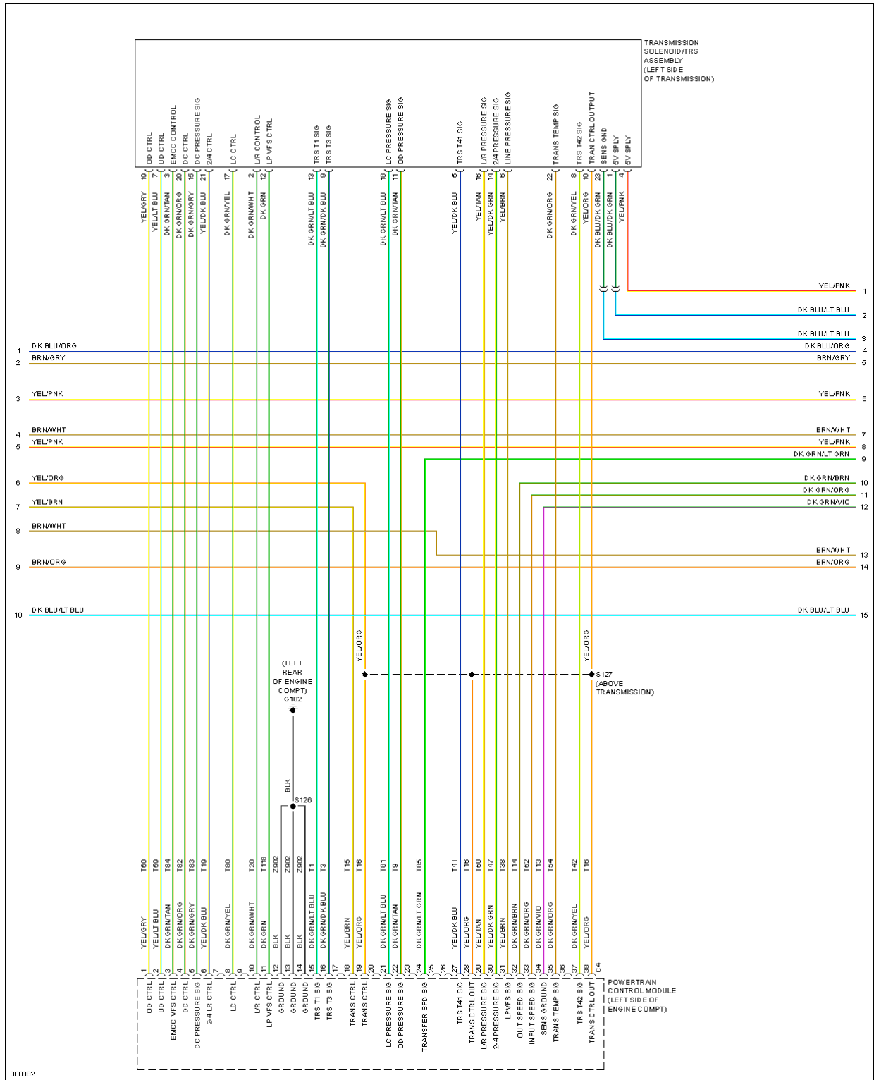
Fig. 22: 3.5L, Engine Performance Circuit (3 of 5)
