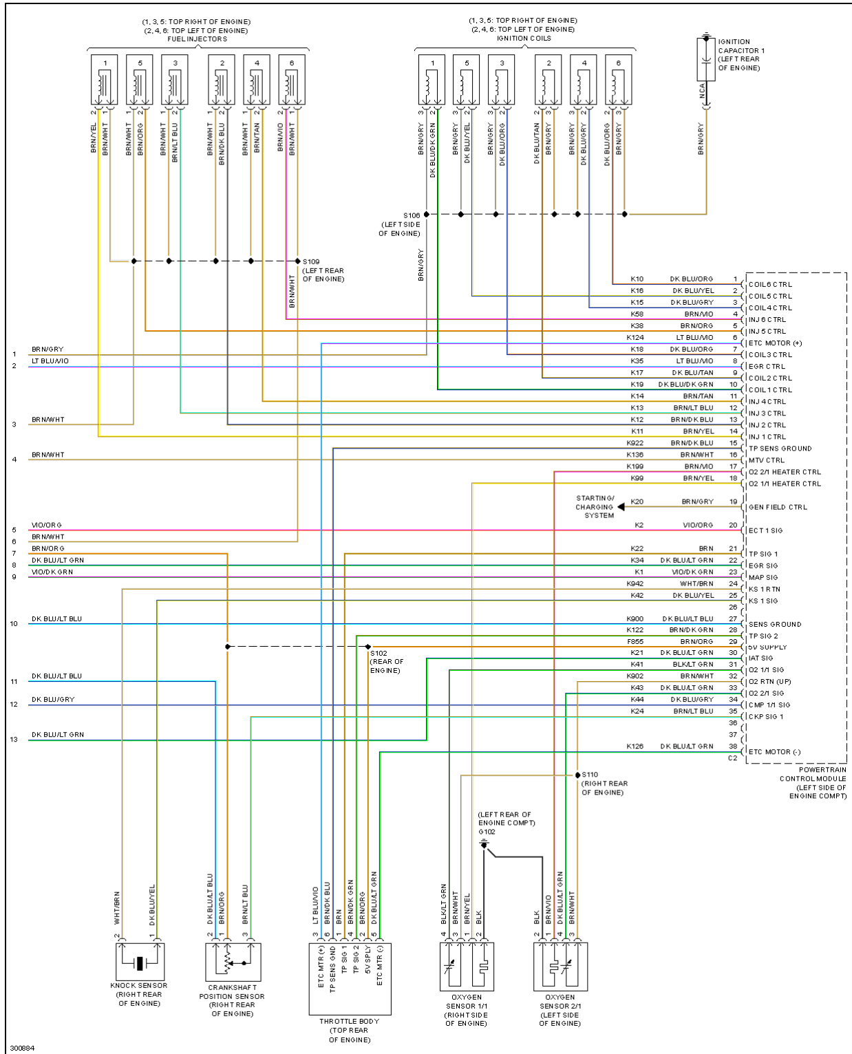
Fig. 24: 3.5L, Engine Performance Circuit (5 of 5)
