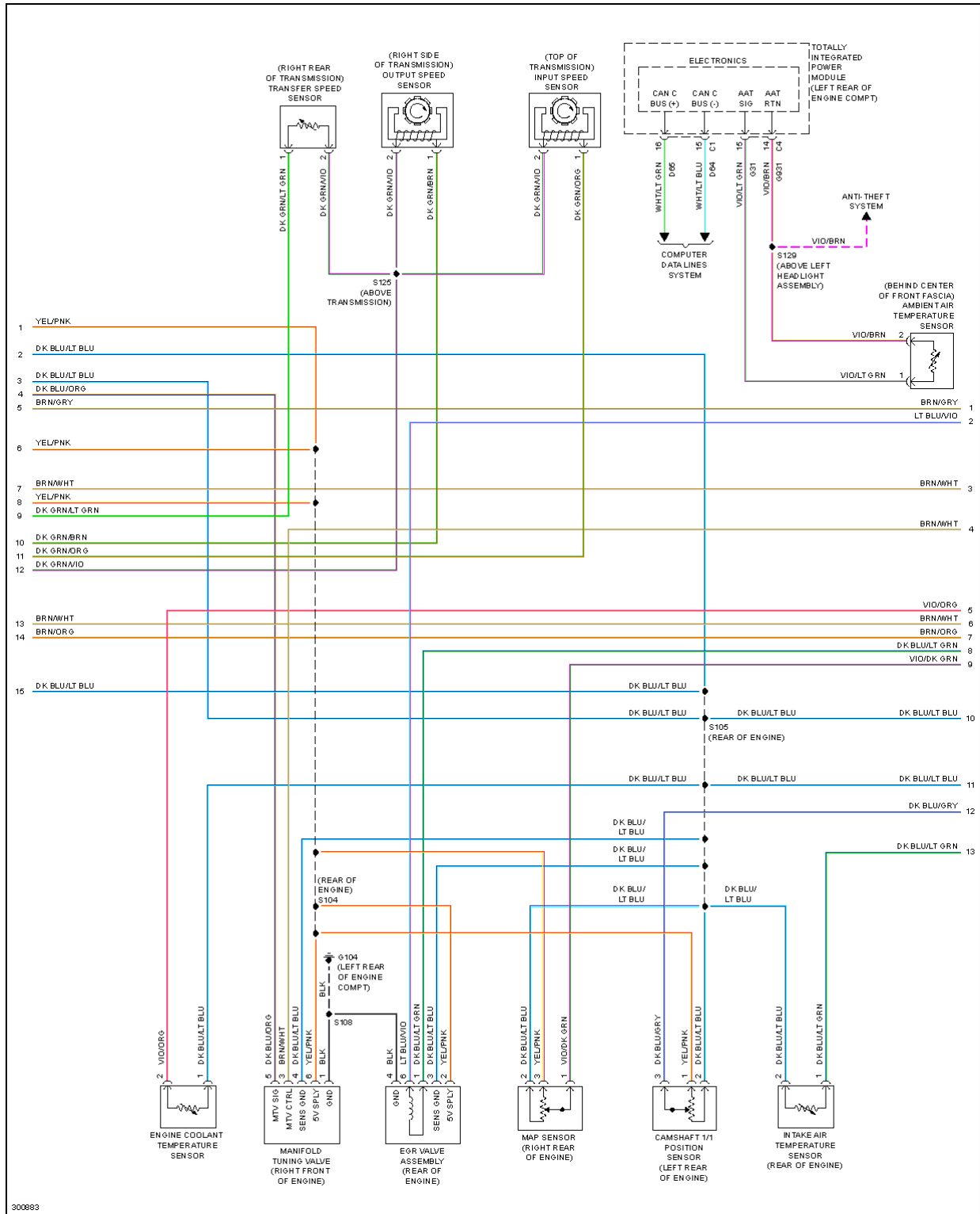
Fig. 23: 3.5L, Engine Performance Circuit (4 of 5)
