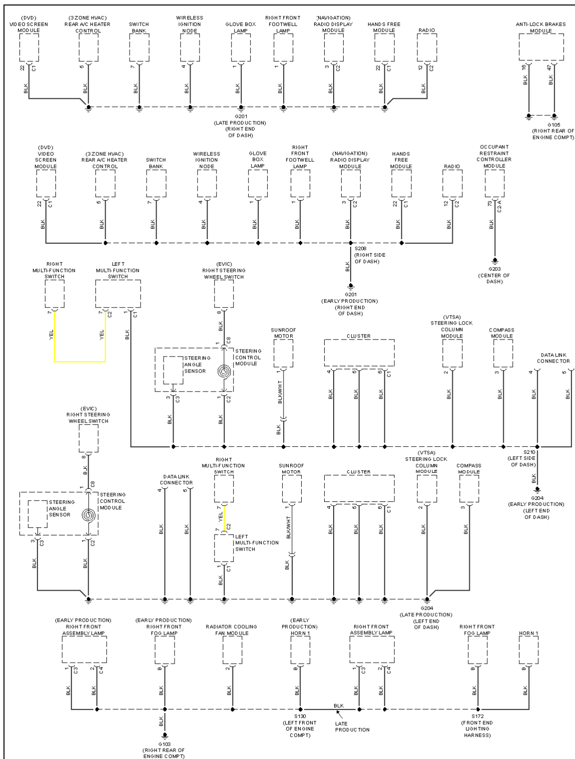
Fig. 29: Ground Distribution Circuit (2 of 4)
