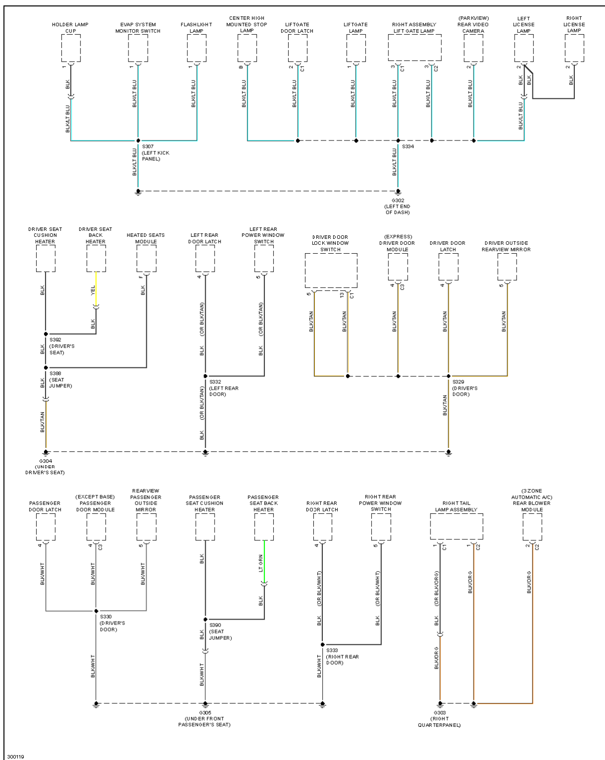
Fig. 30: Ground Distribution Circuit (3 of 4)
