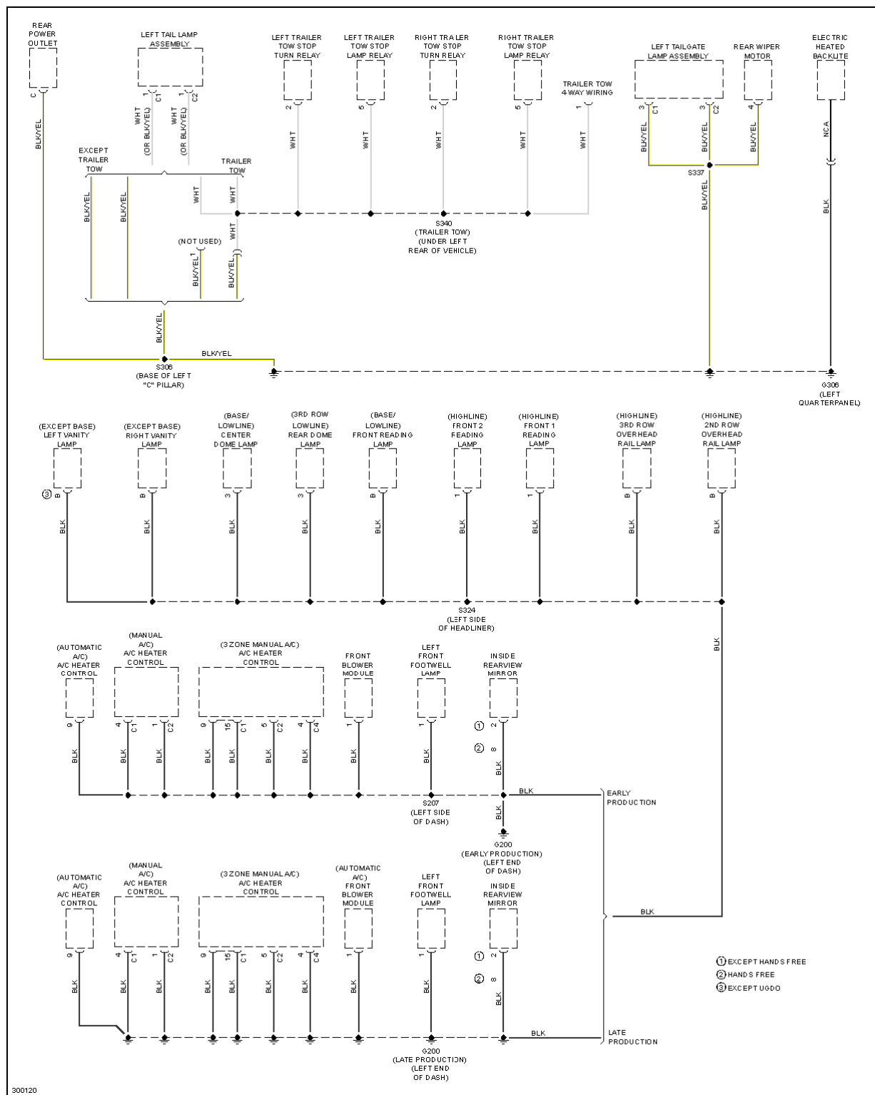
Fig. 31: Ground Distribution Circuit (4 of 4)
