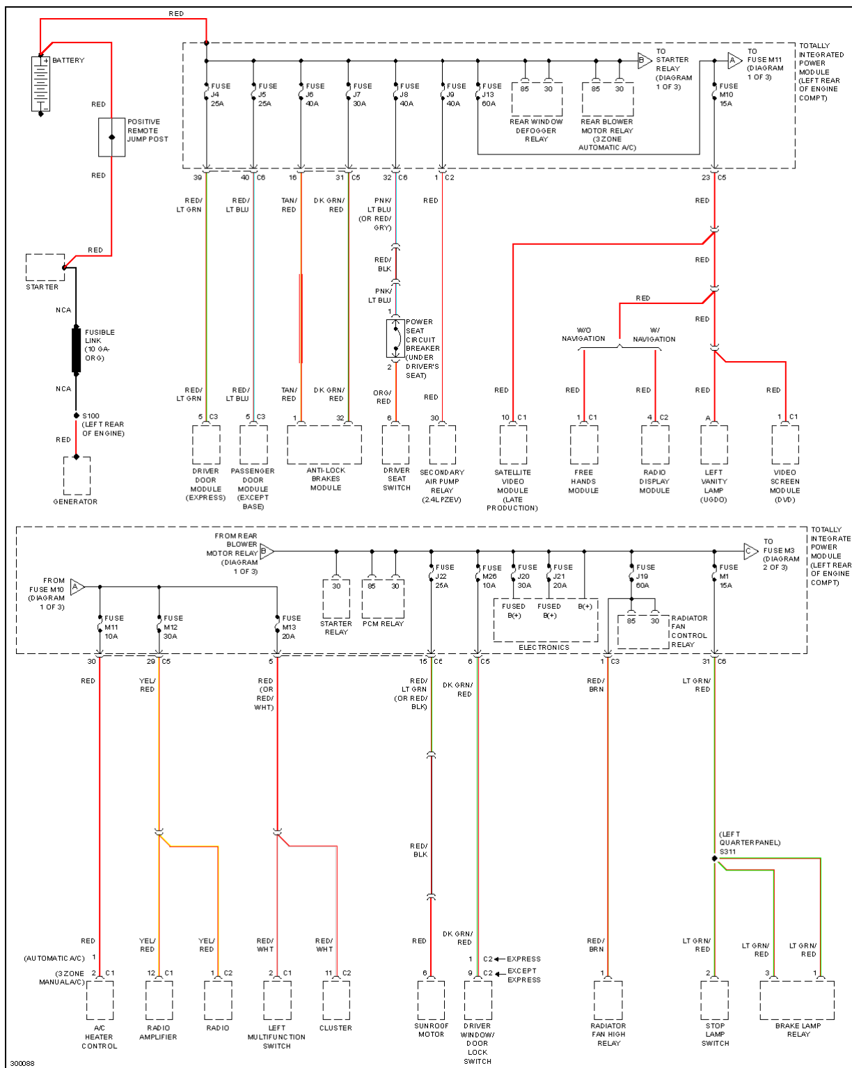
Fig. 44: Power Distribution Circuit (1 of 3)
