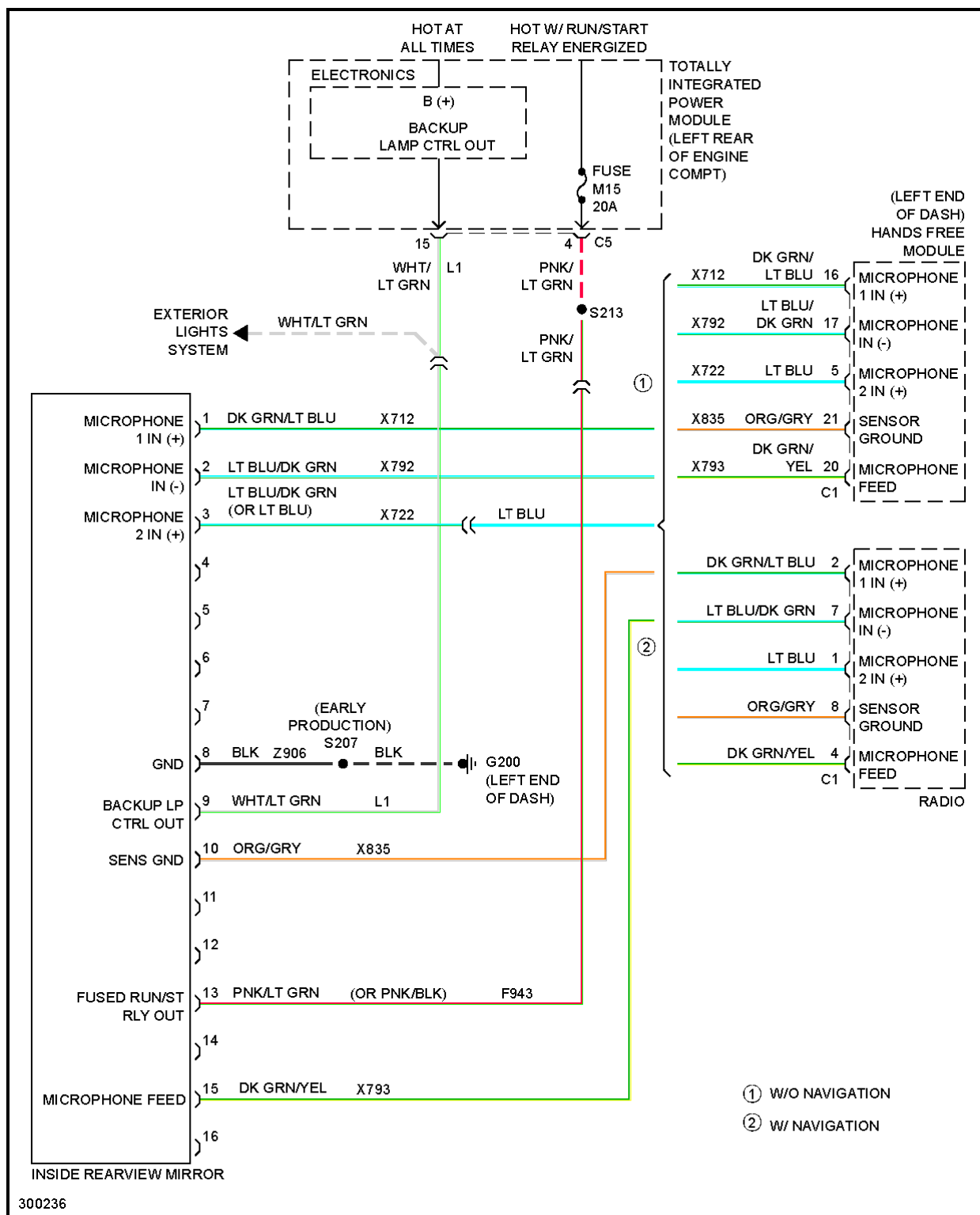
Fig. 49: Automatic Day/Night Mirror Circuit, W/O Hands Free
