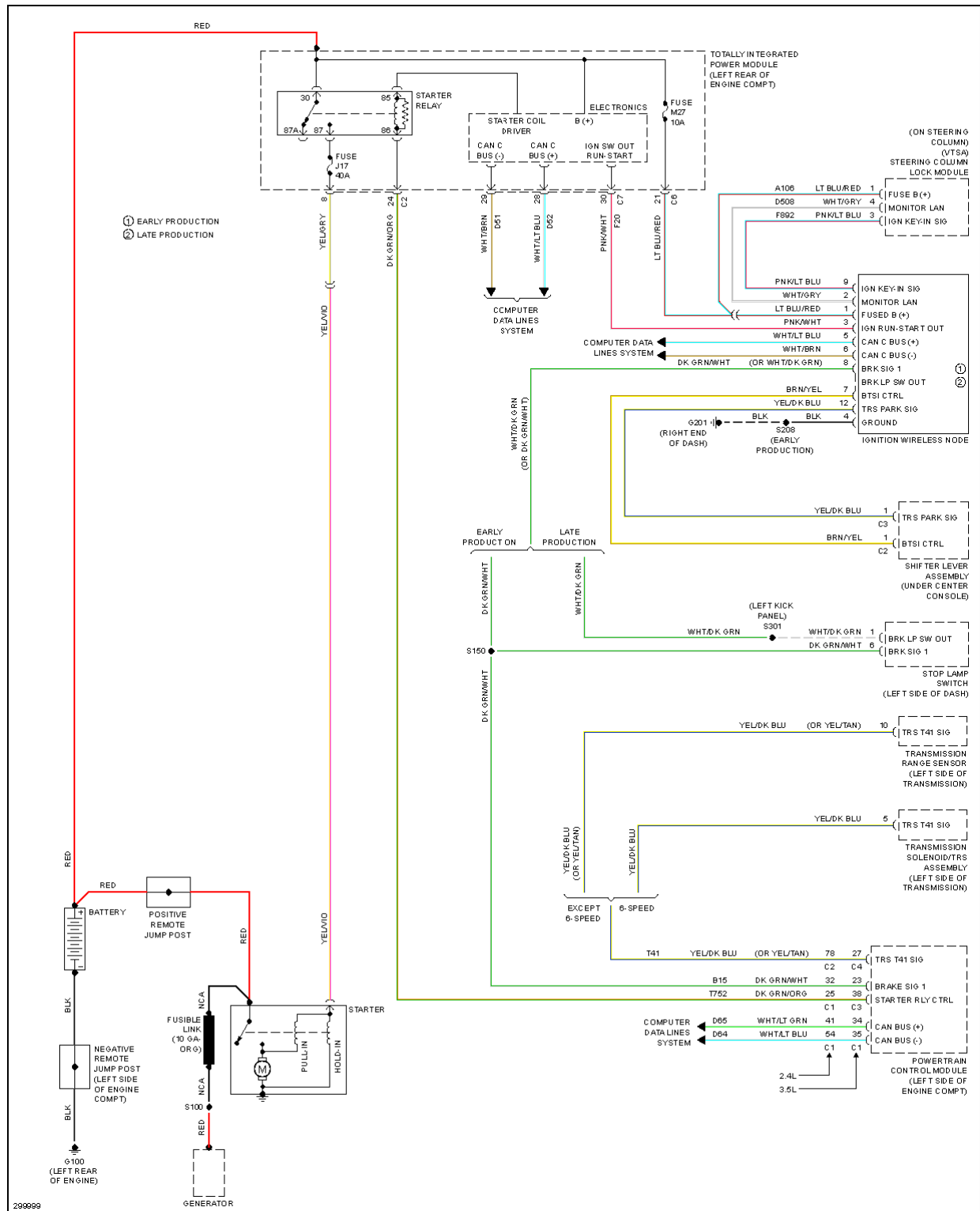
Fig. 65: Starting Circuit
