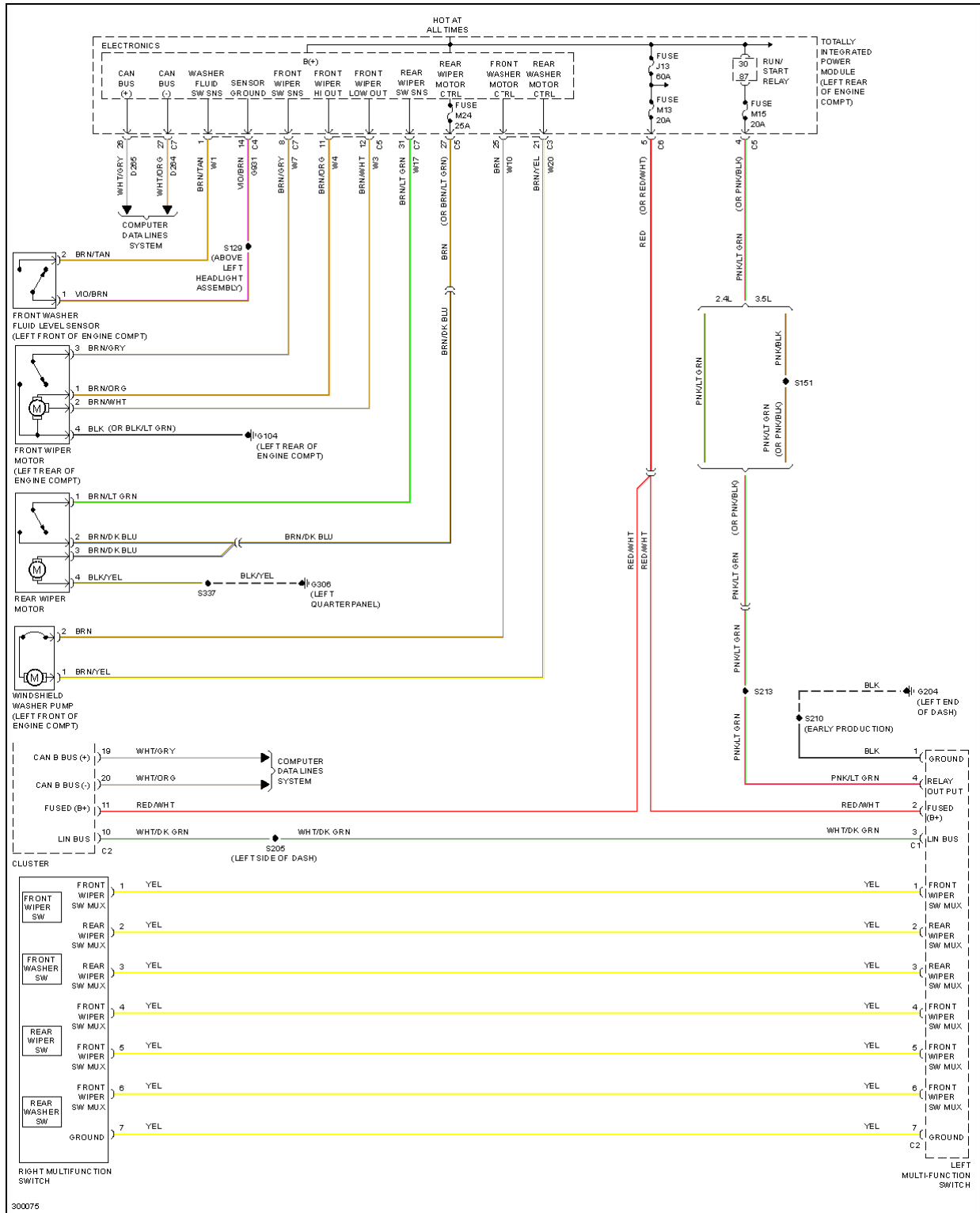
Fig. 74: Wiper/Washer Circuit
