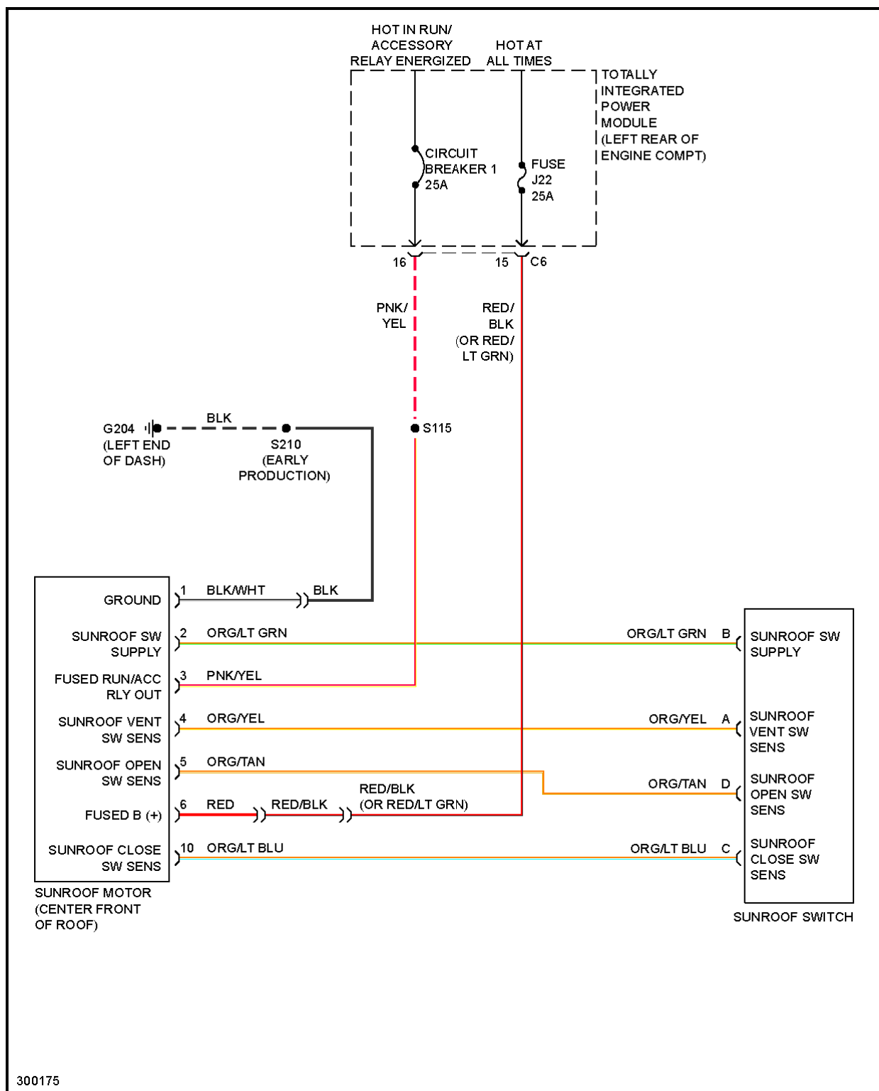
Fig. 54: Power Top/Sunroof Circuit
