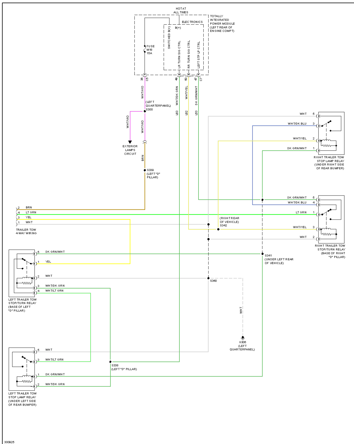
Fig. 27: Trailer Tow Circuit
