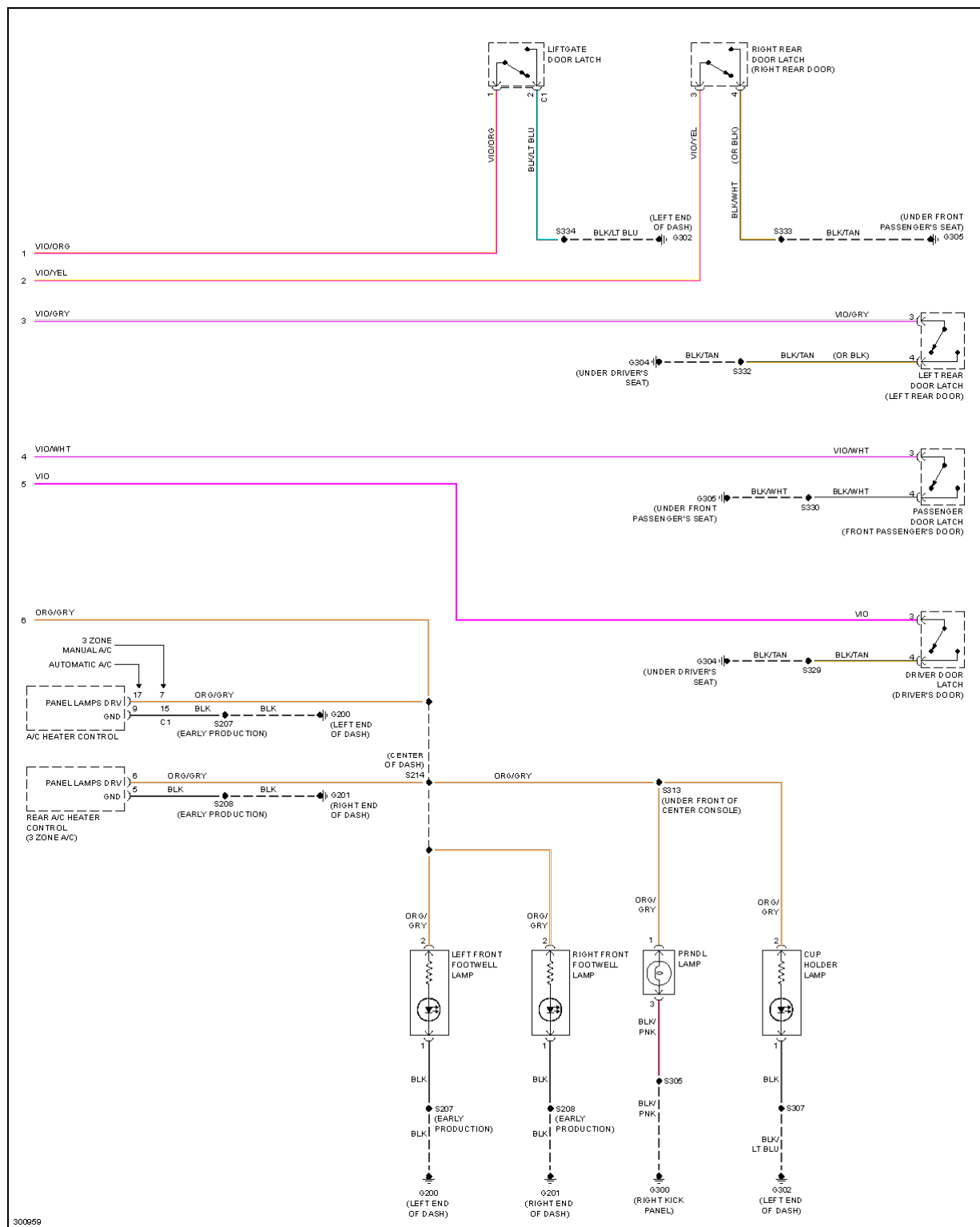
Fig. 36: Interior Lights Circuit (2 of 2)
