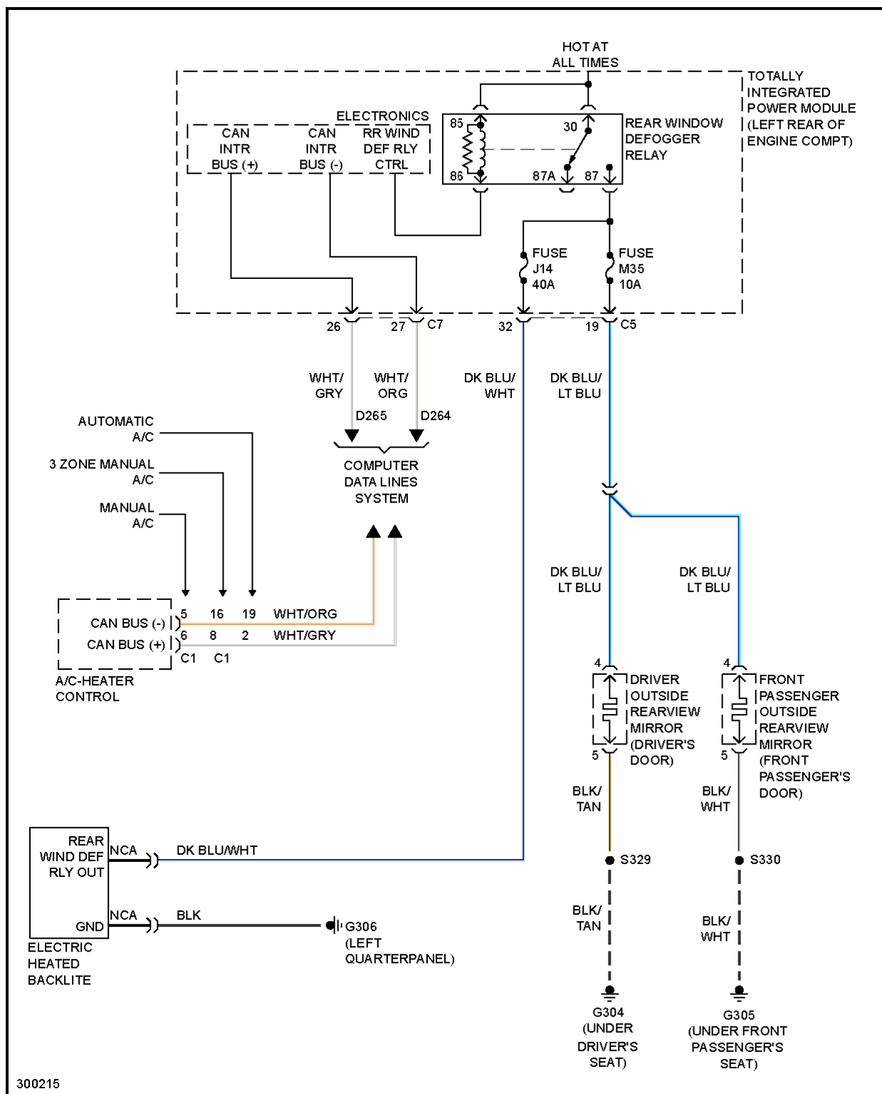
Fig. 15: Defoggers Circuit, W/O Express Up/Down Windows
