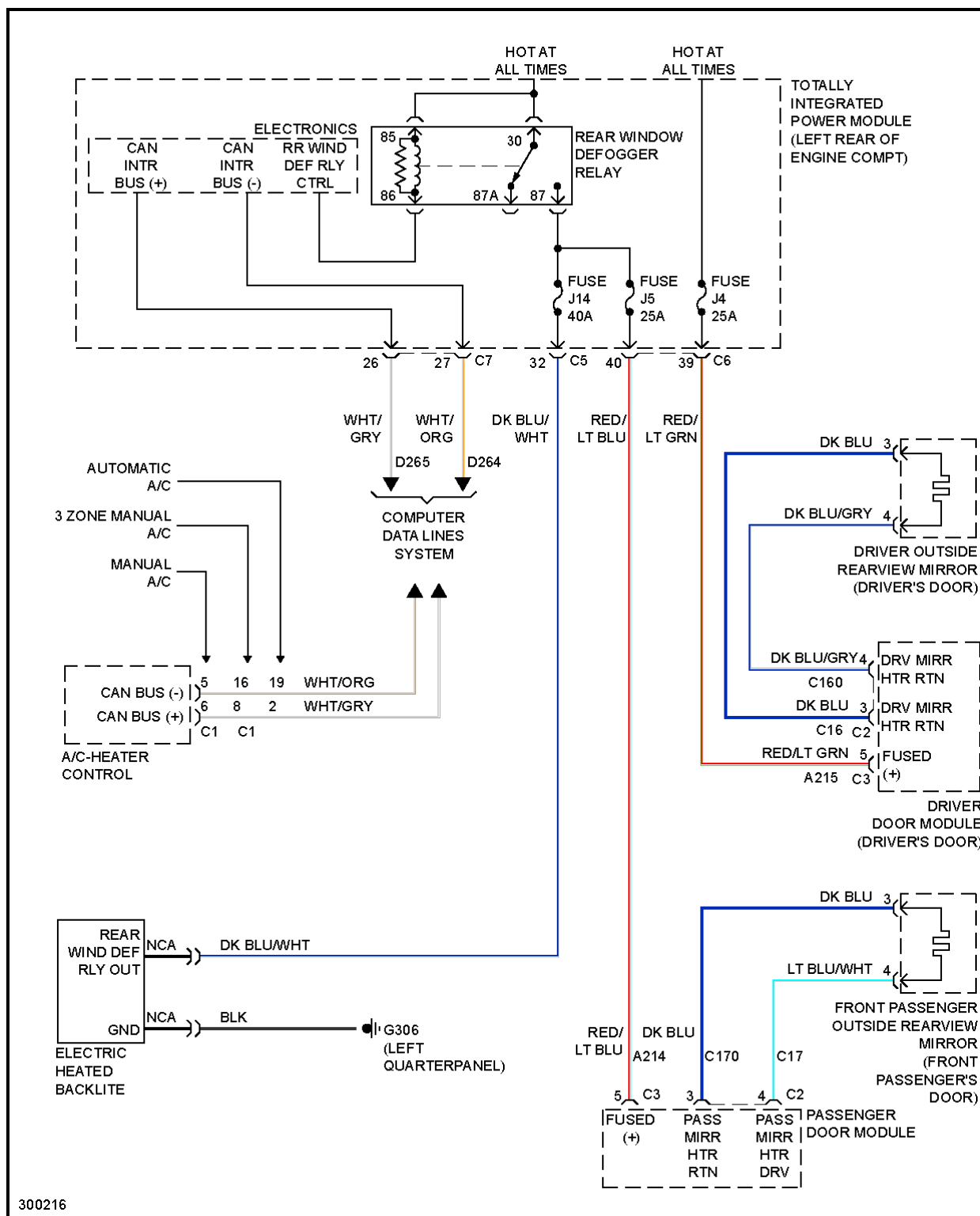
Fig. 14: Defoggers Circuit, W/ Express Up/Down Windows
